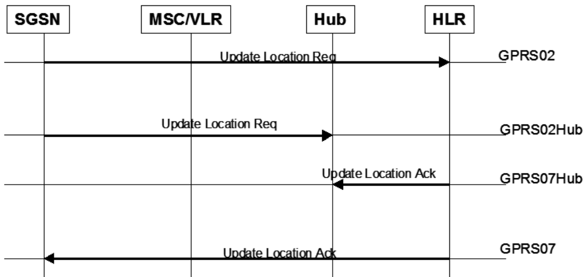
Figure 8: Packet Switch flow for Roaming Hub Provider
