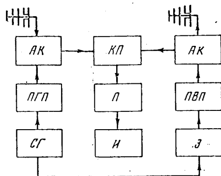
Fig. 4.15. Block-Diagram of a Radar Set Designed for Studying the Resonance Phenomenon During the Scattering of Radio Waves in the Ionized Meteor Trails. A K - antenna switching device; K П - receiver switch; ПГП - transmitter of horizontal polarization; ПВП - transmitter of vertical polarization; П - receiver; СГ - synchrogenerator; И - indicator; З - lag by \tau = 140 microseconds.
