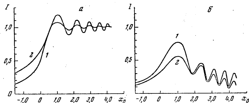
Fig. 4.13. Diffraction Patterns of the Signals Scattered in the Underdense Meteor Trails at Two Positions of the Point of Mirror Image. 1- for the ascending branch of the ionization curve; 2- for the descending branch at 2 values of the parameter \Delta = 8\pi^2 D \sqrt{R/\lambda^3/2} v . a- \Delta = 0 ; b- \Delta = 0.5 .
