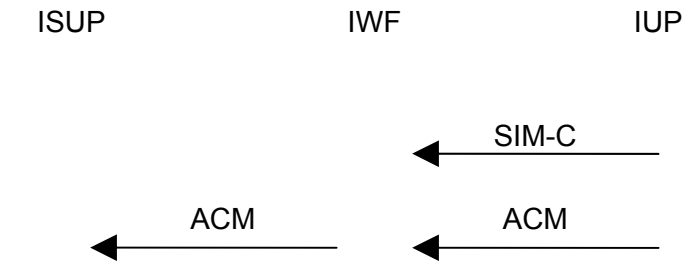
FIGURE 1.12 Mapping IUP ACM to ISUP ACM
