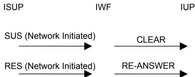
FIGURE 1.16 Mapping of ISUP SUS and RES (Network Initiated) to IUP
