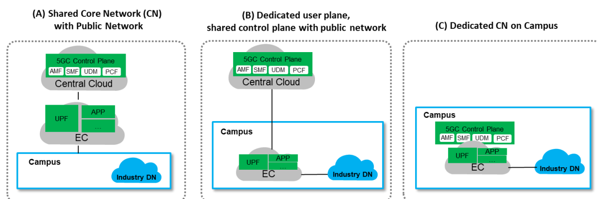
Figure 2: NPN deployment - Core Network Options
