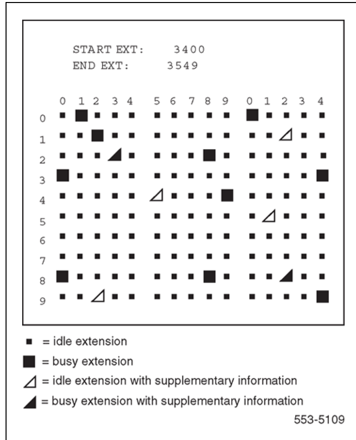
Figure 16 Standard Busy Lamp Field on the BLF/CGM
