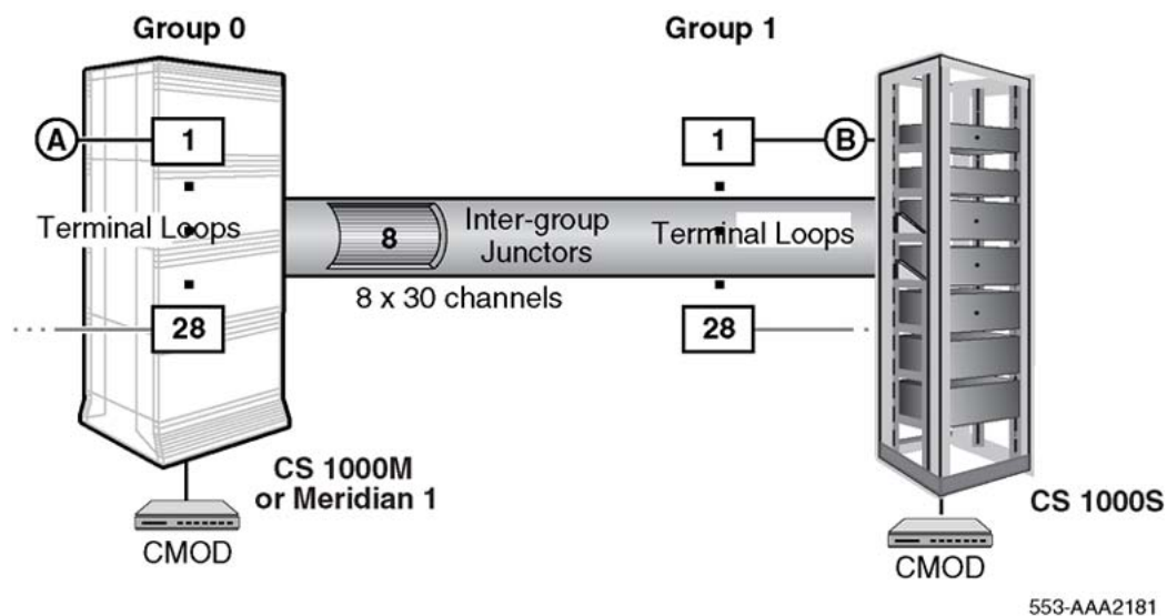
Figure 19: A system with a two-group network
