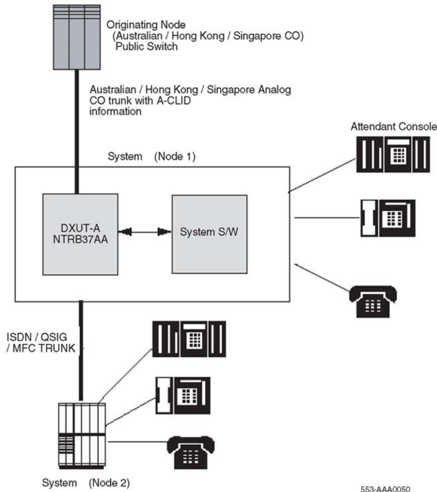
Figure 23: System structure for CLID delivery
