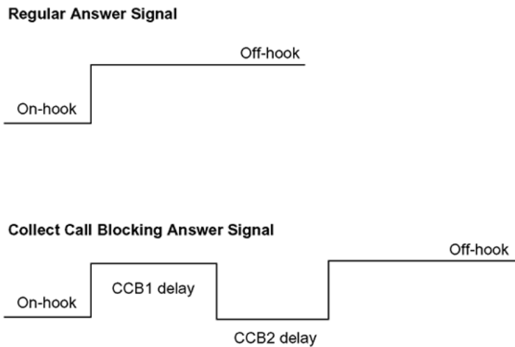
Figure 24: Collect Call Blocking answer signal compared to regular answer signal
