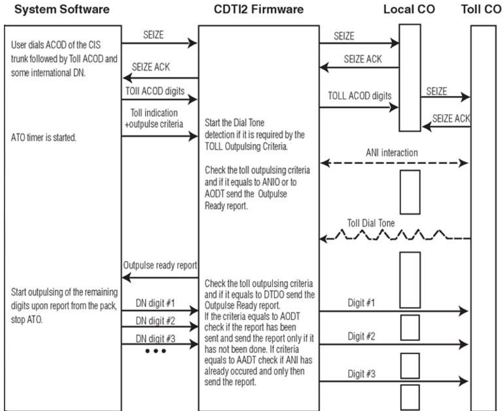
Figure 13: Indirect outgoing toll call with dial tone detection
