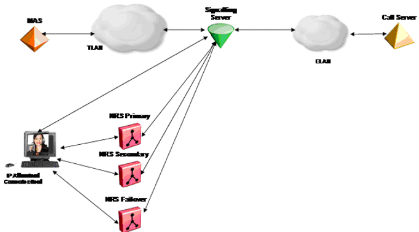
Figure 7: Redirect deployment using 1 NRS, 1 Signaling Server, and 1 Call Server
