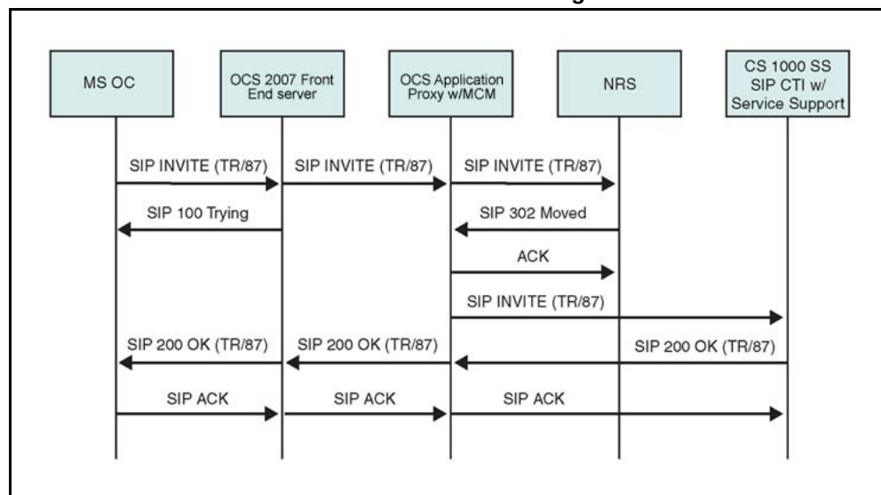
Figure 114 Remote Call Control Session Establishment through SRS
