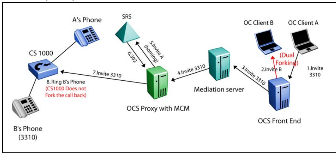
Figure 5 Dual forking example
