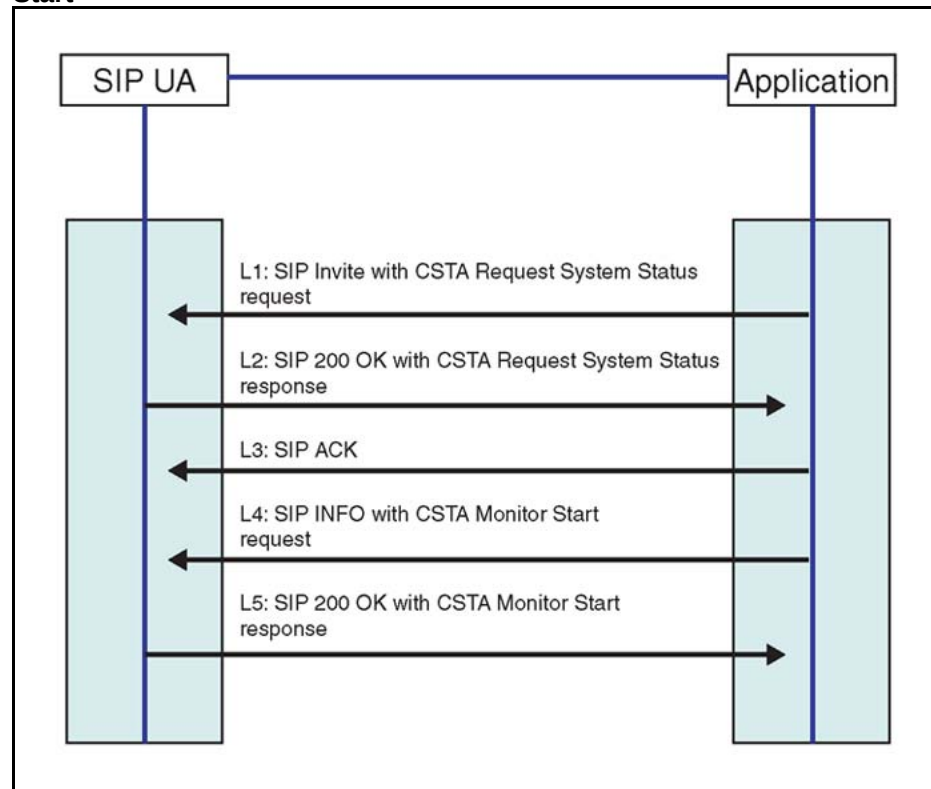
Figure 106 Message sequence diagram - CSTA Session Establishment and Monitor Start
