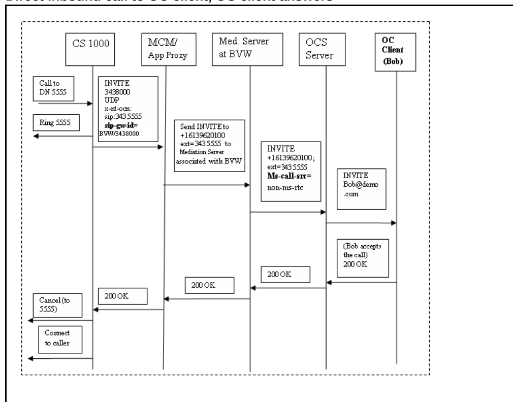
Figure 110 Direct inbound call to OC client, OC client answers
