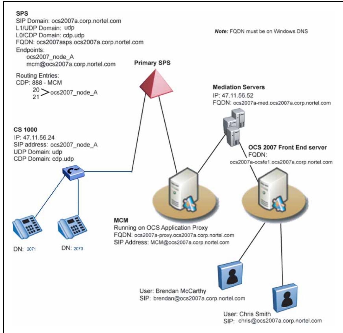
Figure 9 "IP diagram" (page 36) depicts the IP protocol information.
