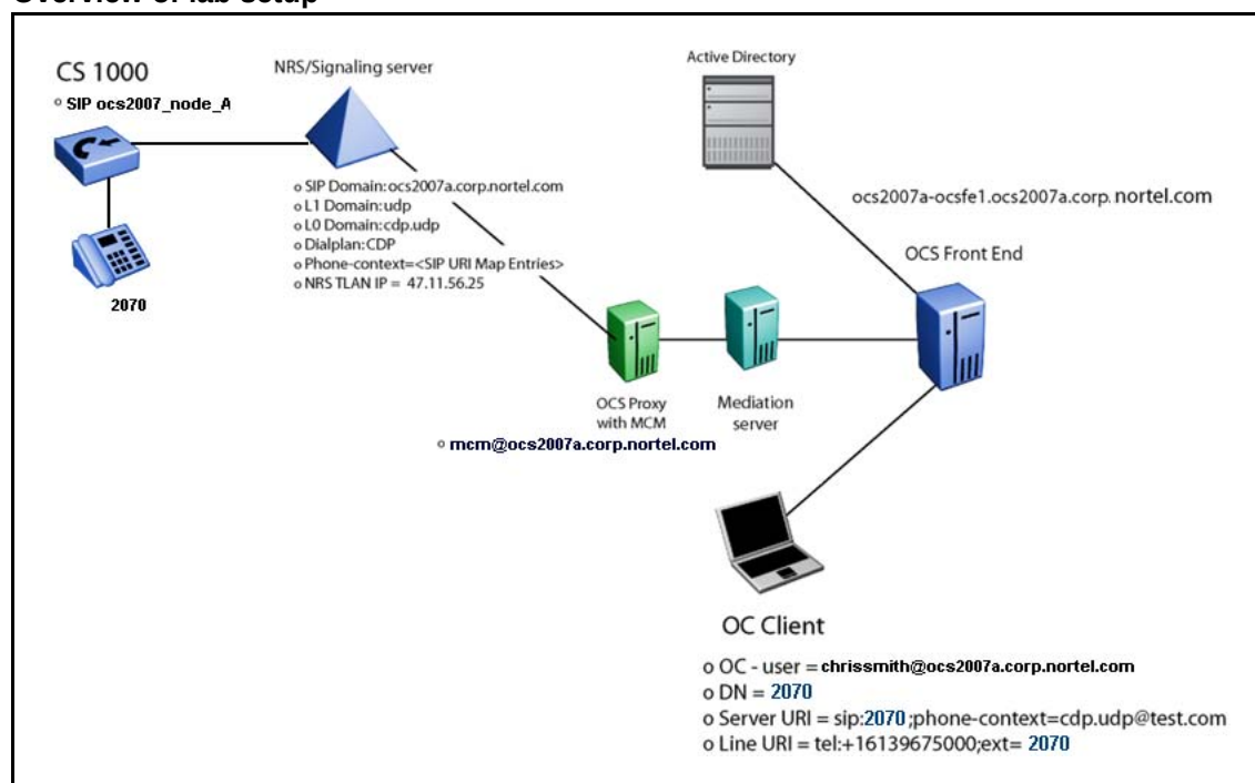
Figure 115 Overview of lab setup
