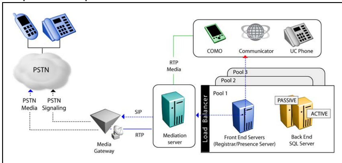
Figure 1 Enterprise Voice components - OCS 2007
