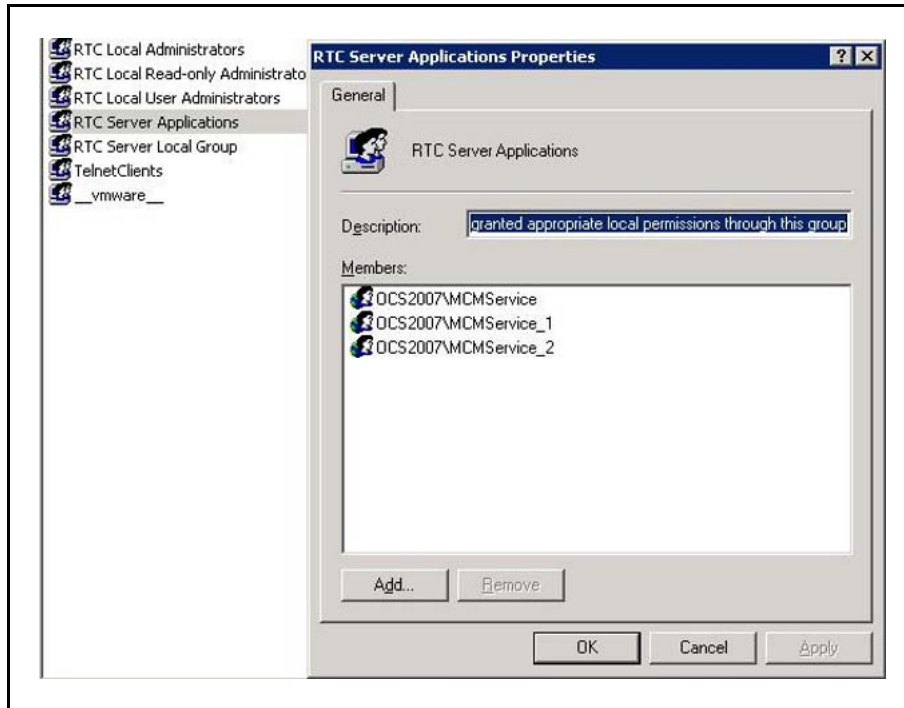
Figure 143 RTC Server Application group
