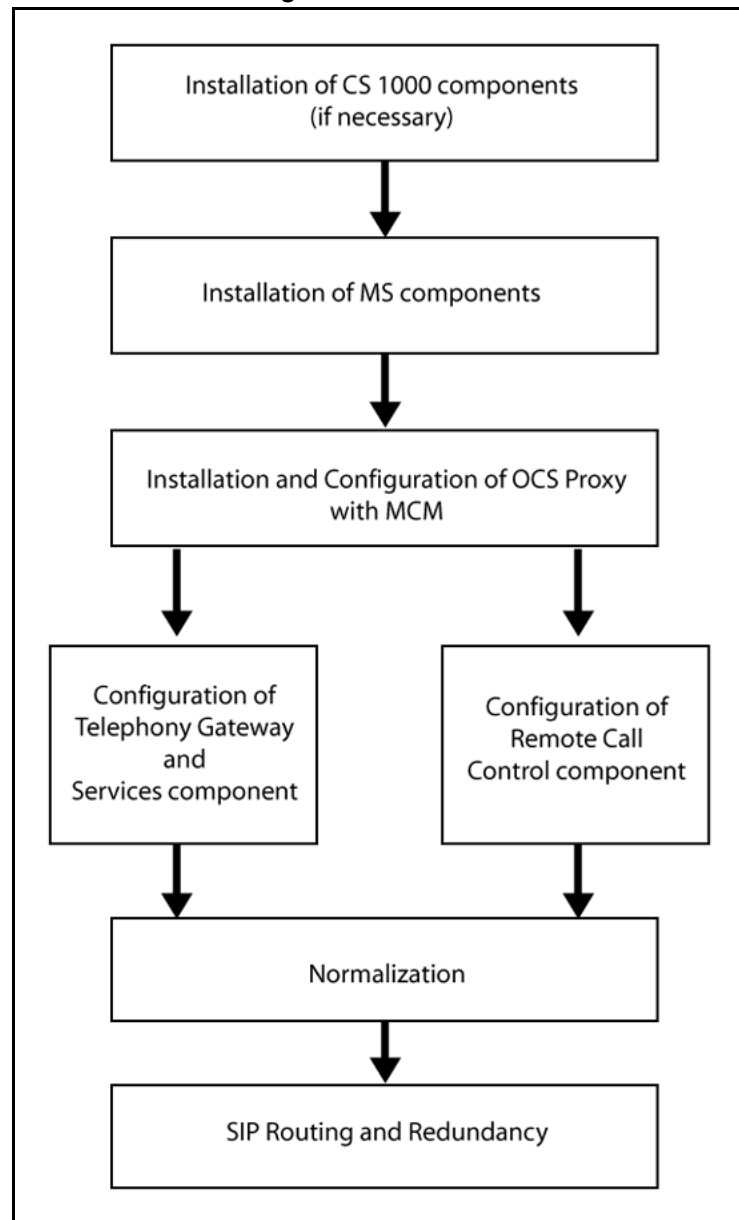
Figure 25 Installation and configuration flow
