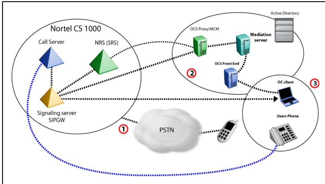
Figure 6 Example call scenario
