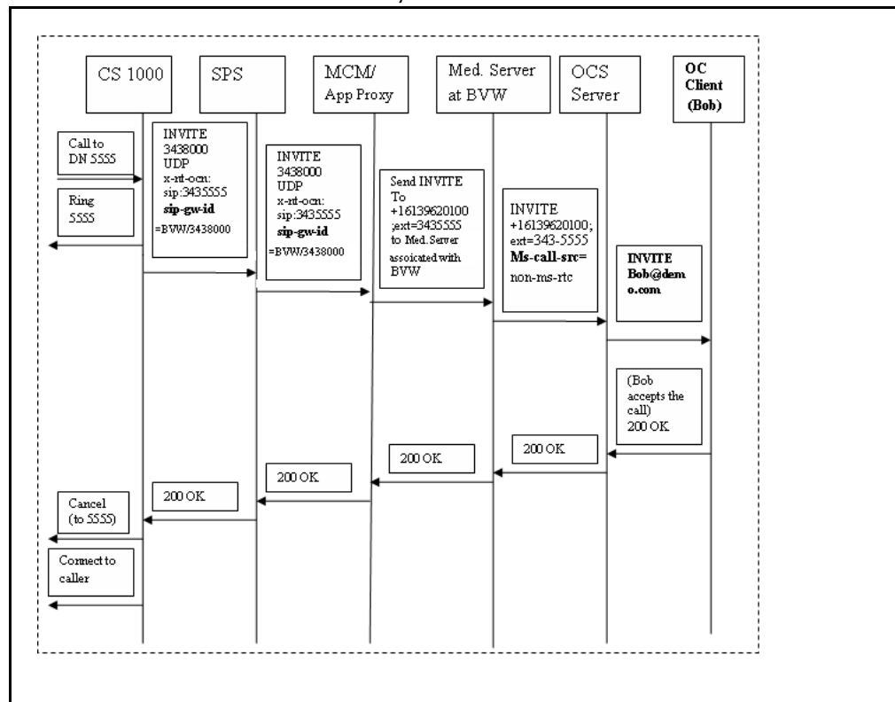
Figure 108 Inbound call to OC client with SPS, OC client answers
