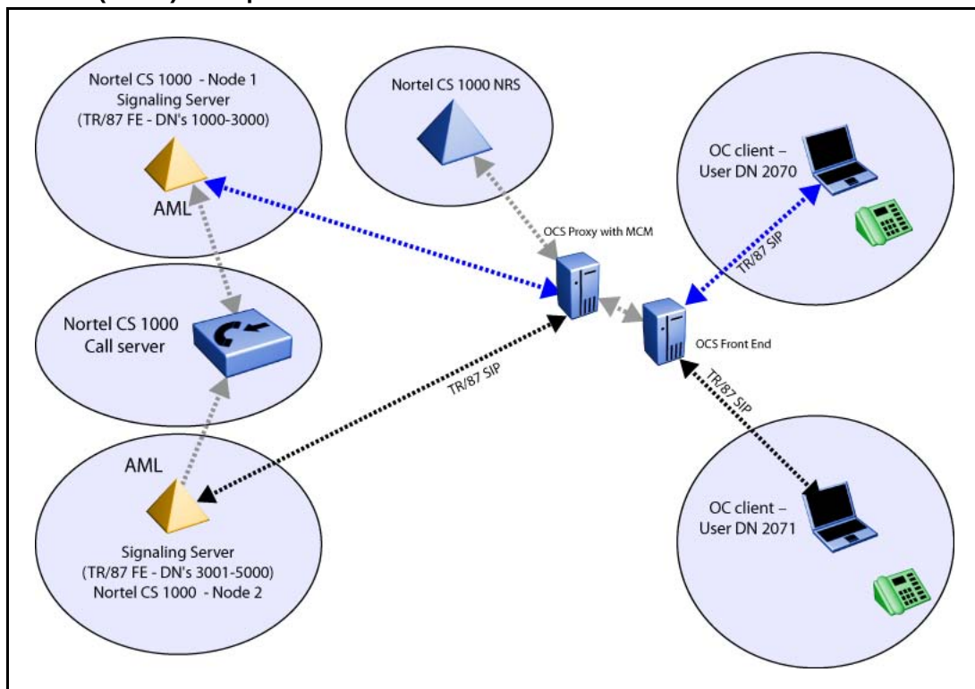
Figure 16 SIP CTI (TR/87) example
