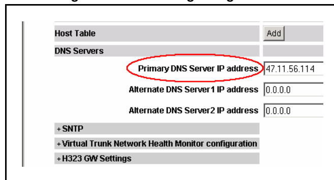
Figure 117 DNS configuration on the Signaling Server
