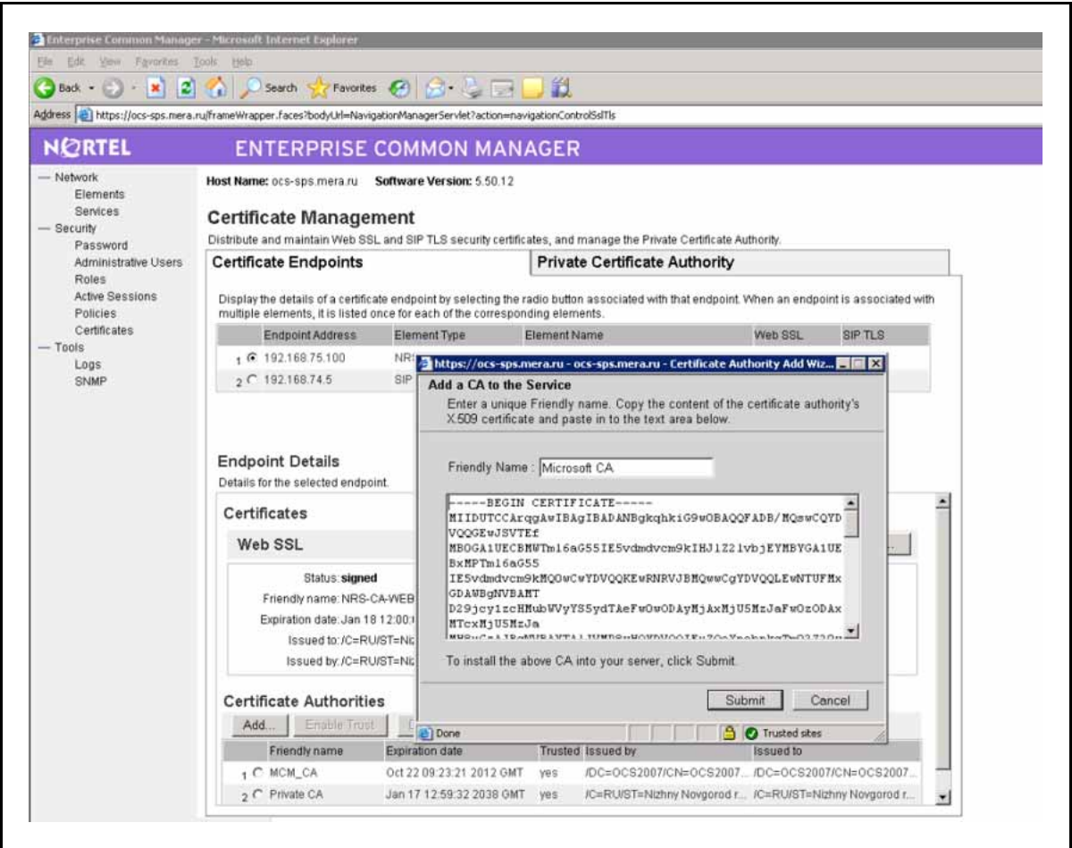
Figure 81 "Certificate Endpoints" (page 213) shows the newly added Certificate Authority.
