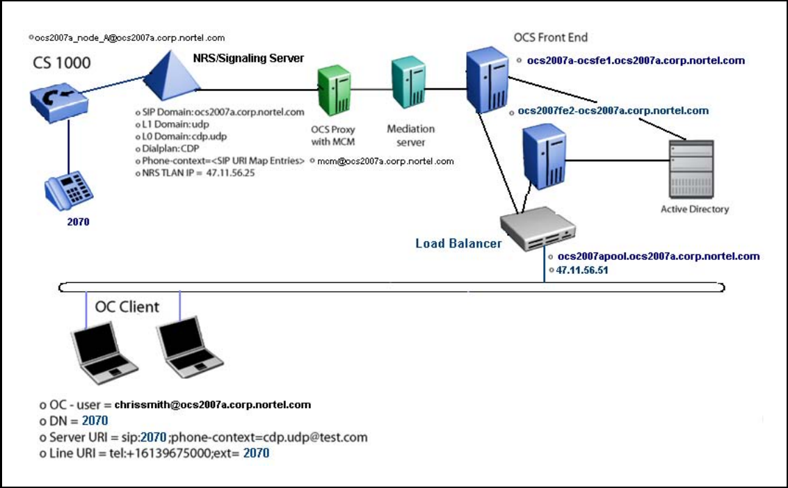
Figure 130 OCS Enterprise Edition General Overview
