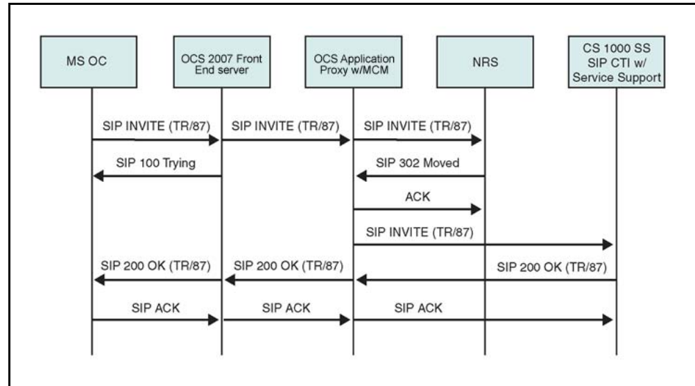
Figure 151 Remote Call Control Session Establishment through SRS
