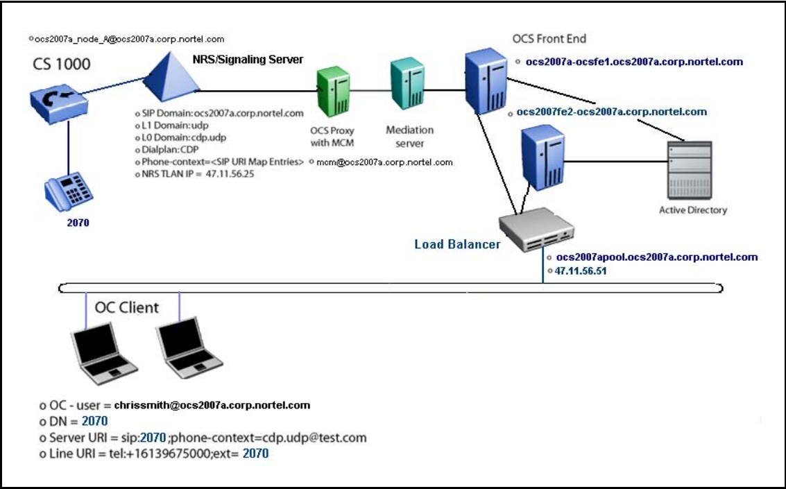
Figure 167 OCS Enterprise Edition General Overview
