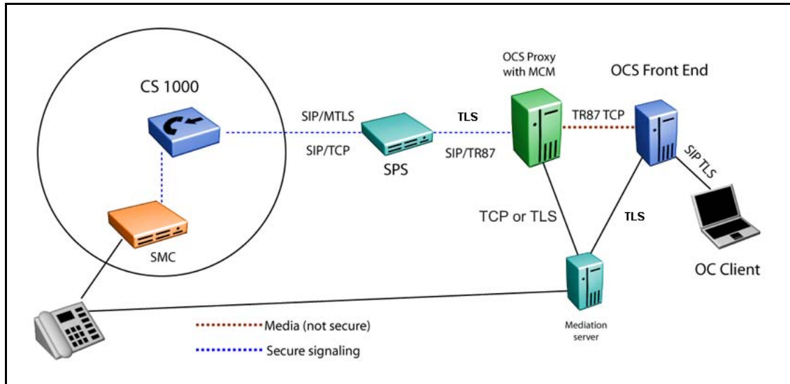
Figure 22 Signaling security with TLS
