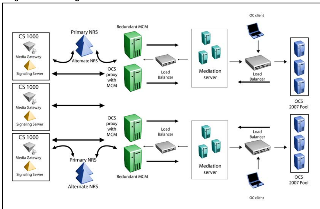
Figure 16 Large network configuration
