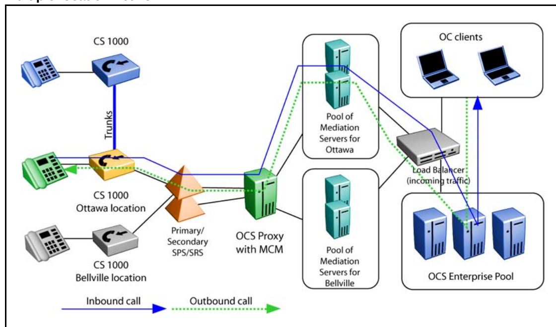
Figure 18 Multiple location network
