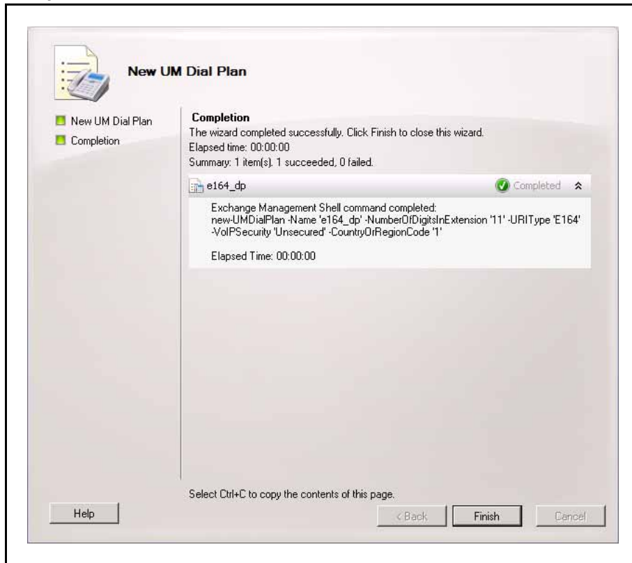
Figure 118 Completion window
