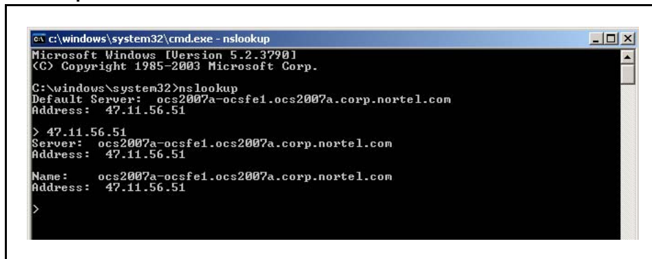
Figure 131 nslookup tool
