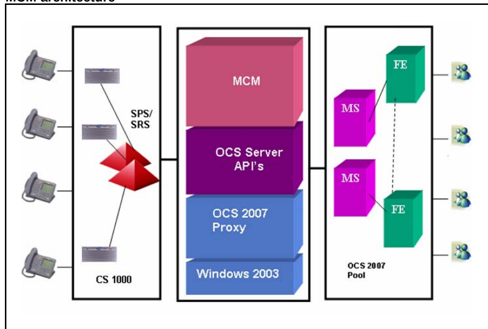
Figure 57 MCM architecture
