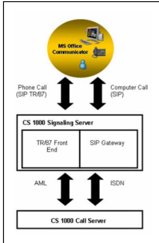
Figure 23 Signaling and media paths
