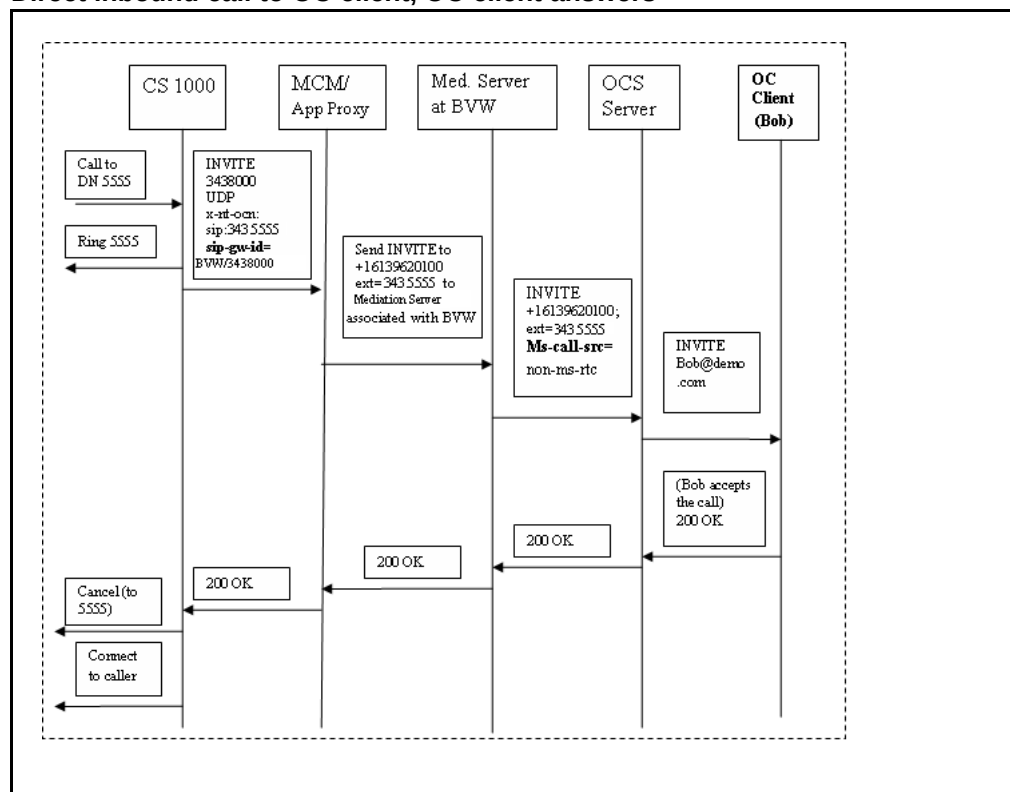
Figure 144 Direct inbound call to OC client, OC client answers
