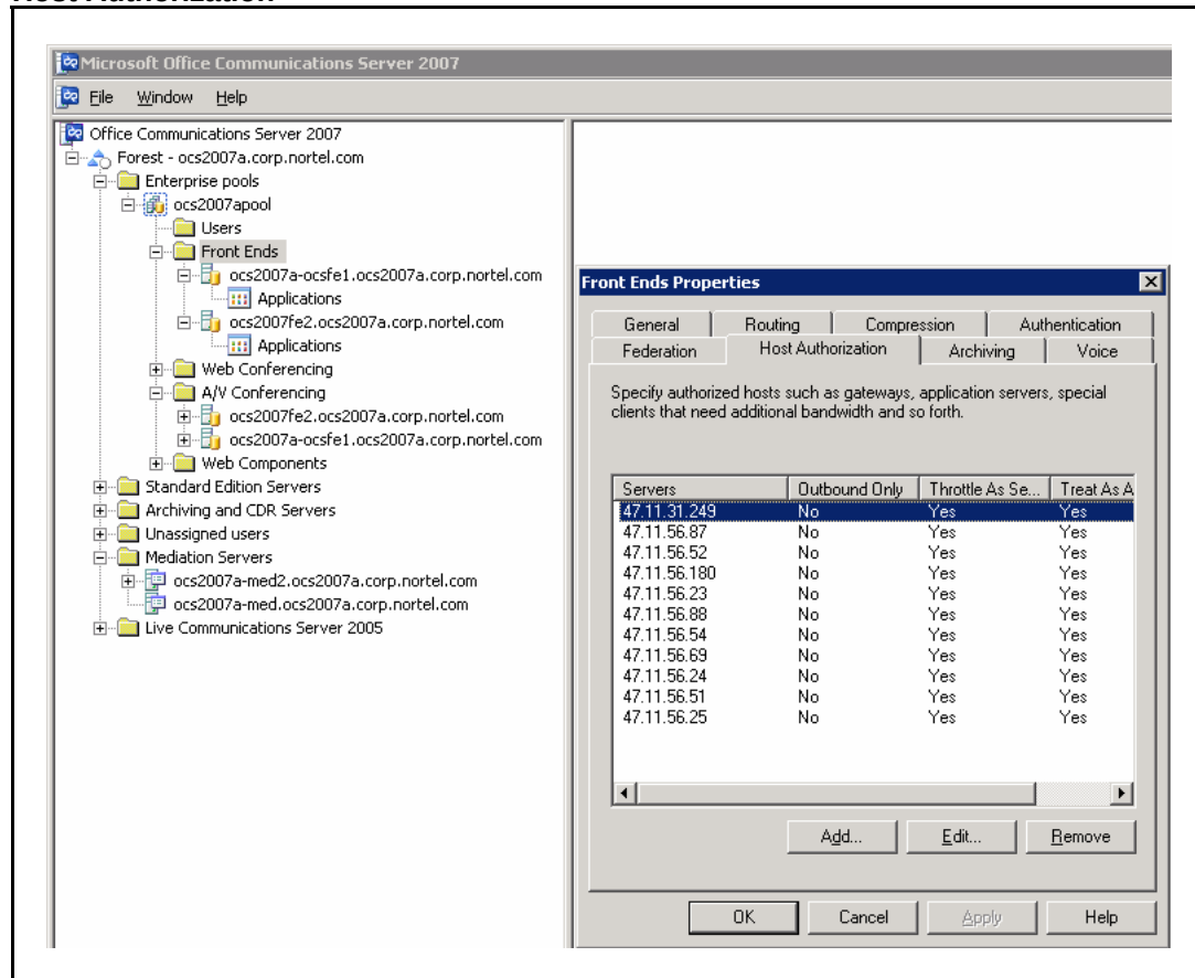
Figure 160 Host Authorization
