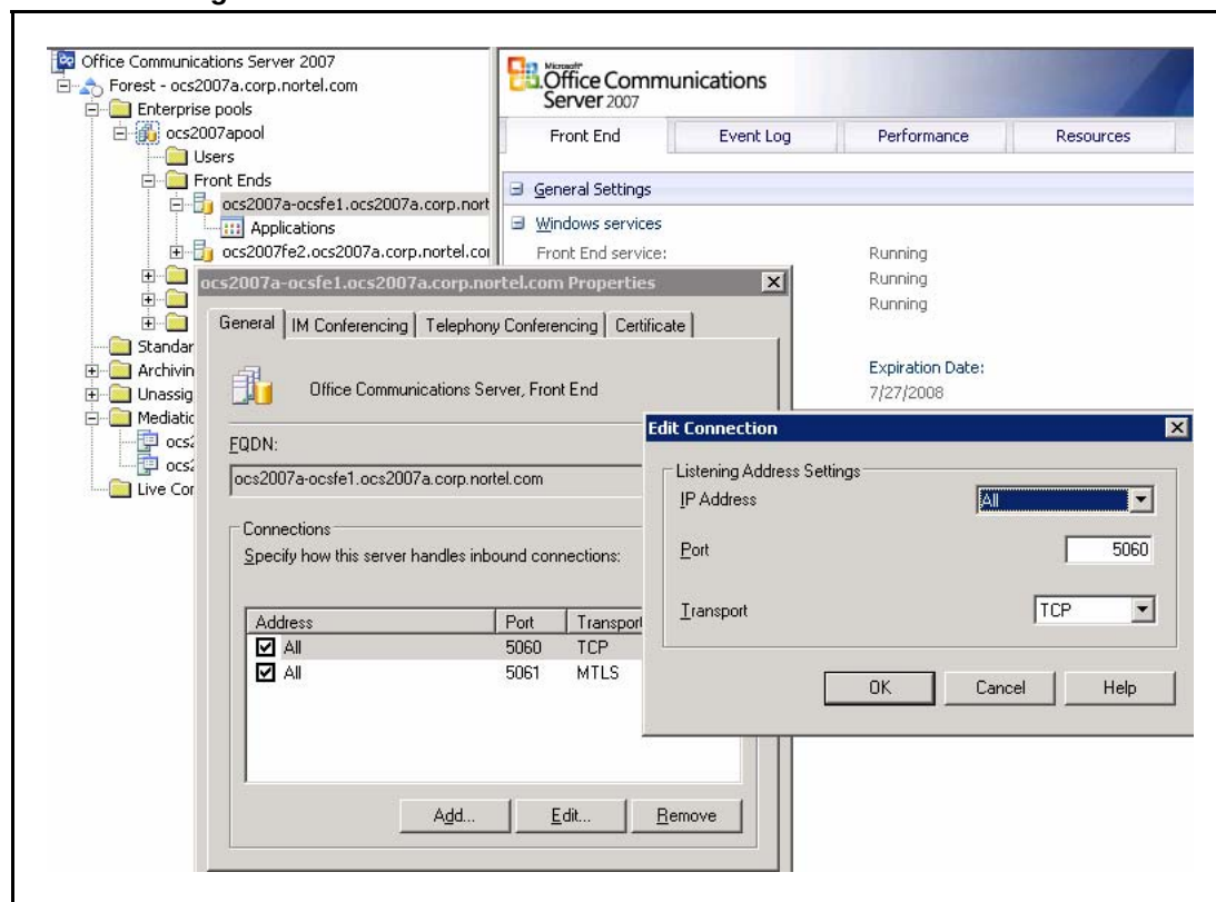
Figure 171 General settings
