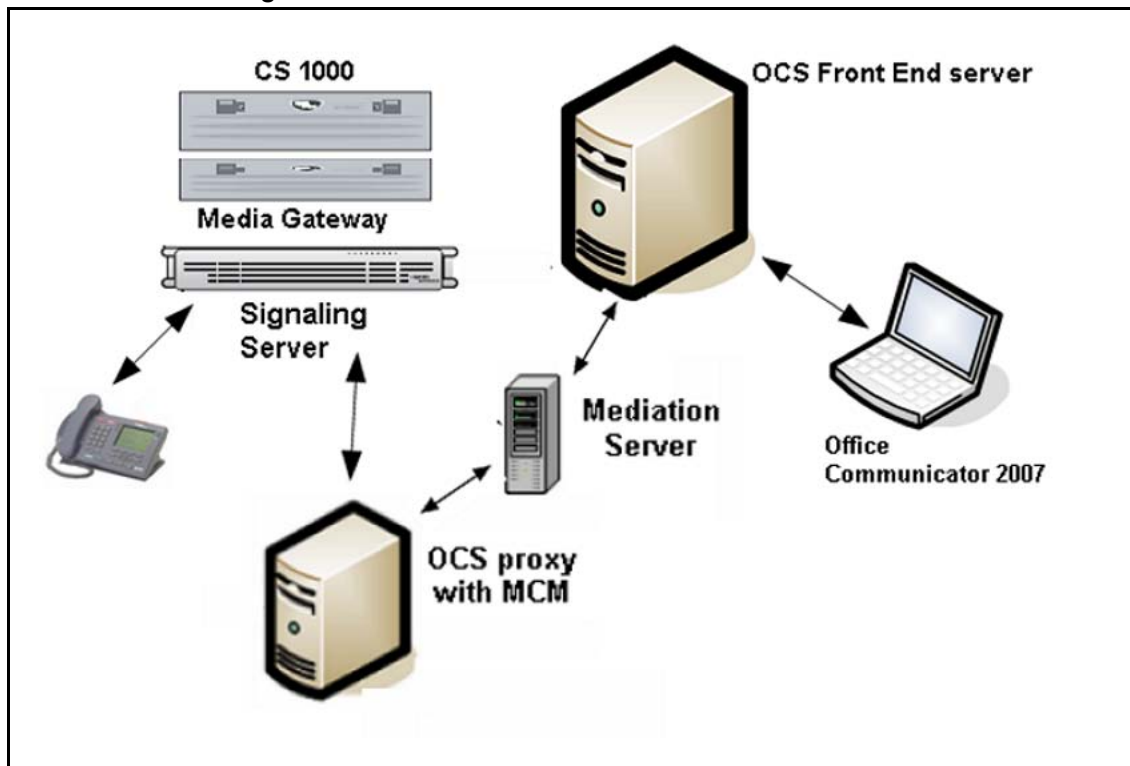
Figure 14 Small network configuration
