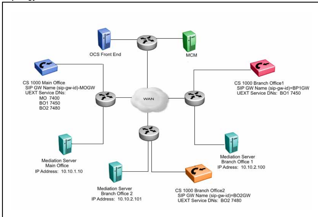
Figure 62 Topology of a main office and two branch offices
