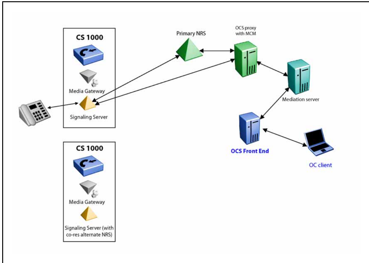
Figure 15 Medium network configuration
