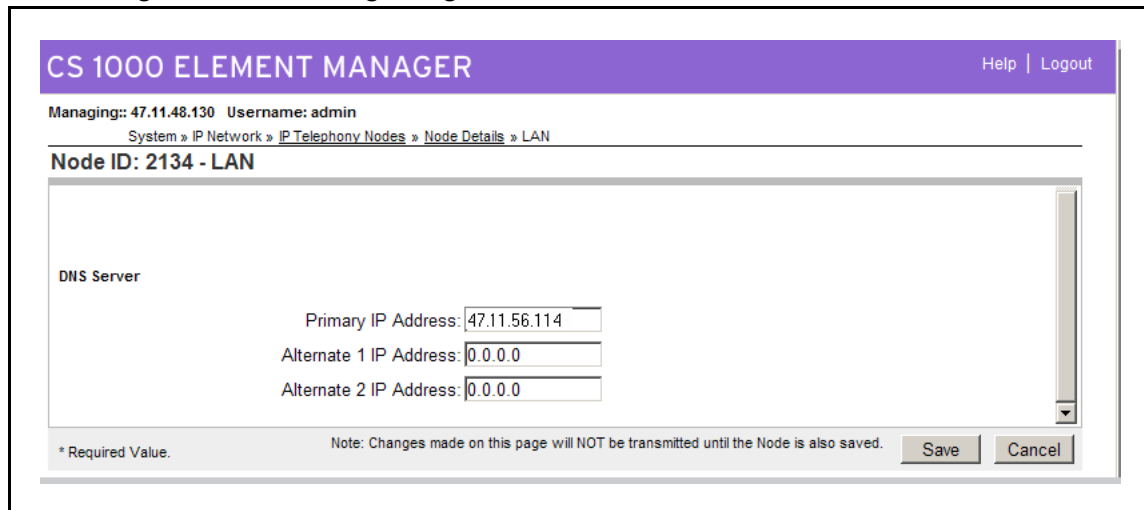
Figure 154 DNS configuration on the Signaling Server
