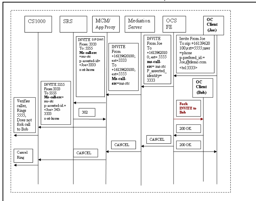
Figure 146 Outbound call from OC client to another OC client, OC client answers
