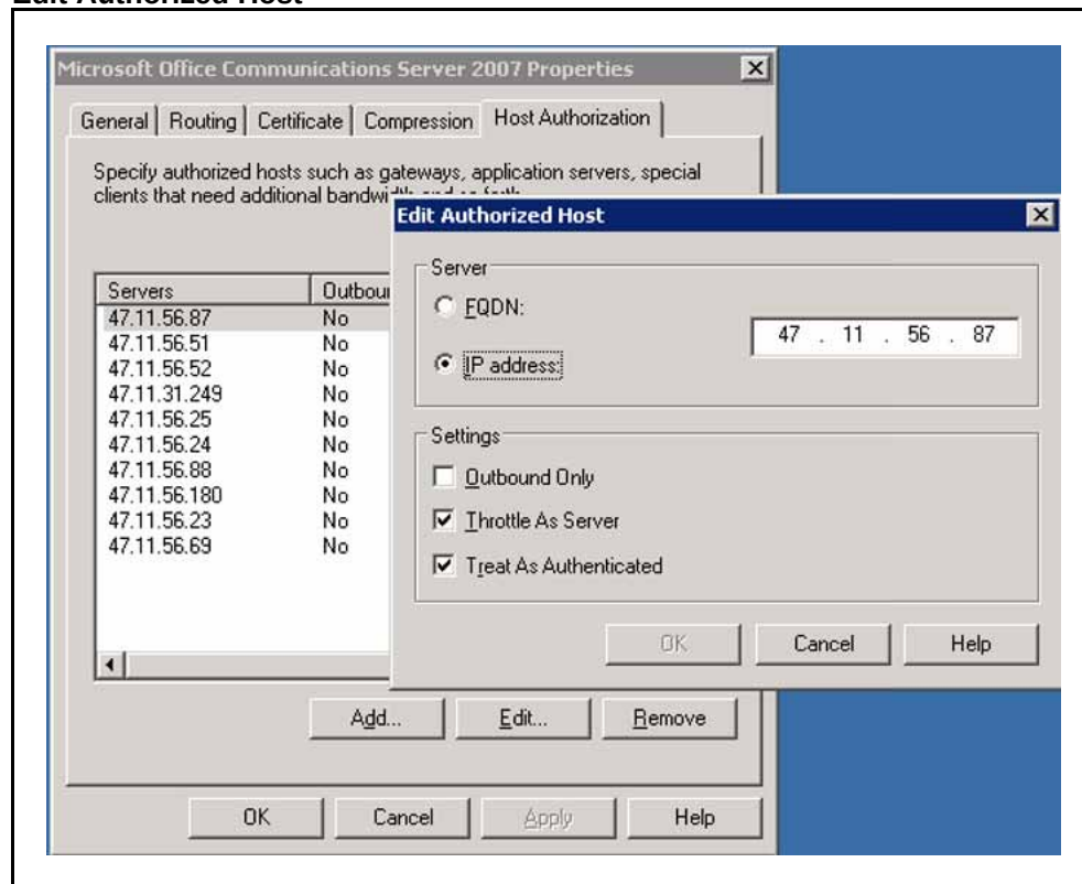
Figure 56 Edit Authorized Host
