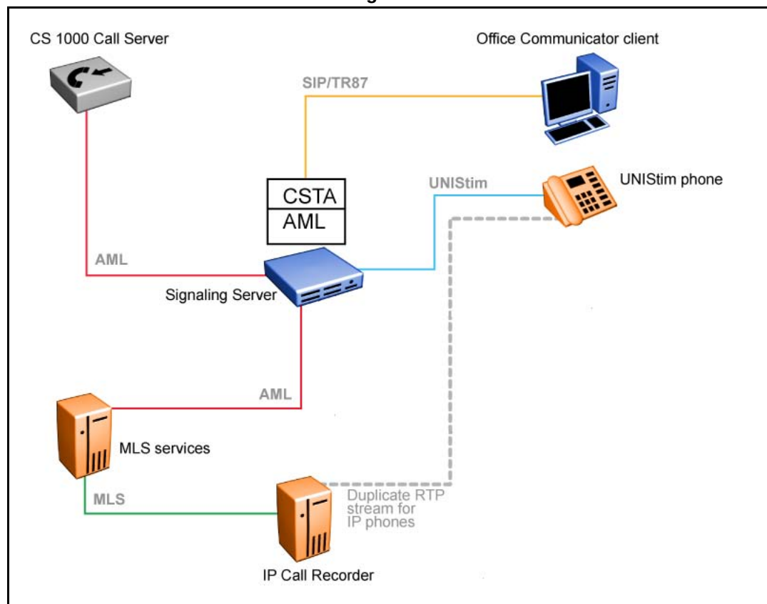
Figure 6 General architecture for IP call recording
