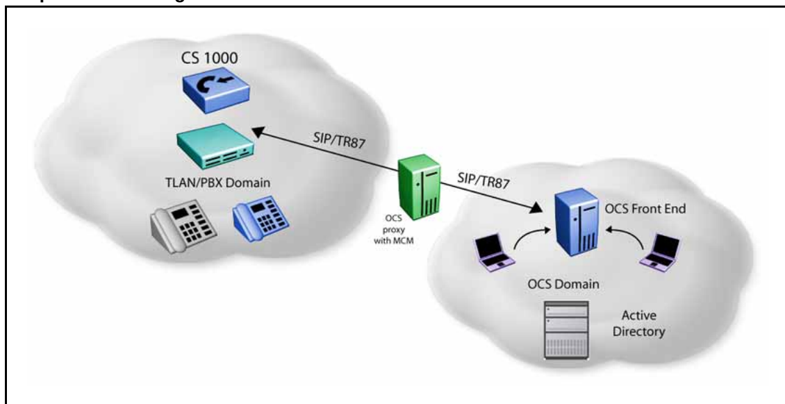
Figure 31 Simple network diagram
