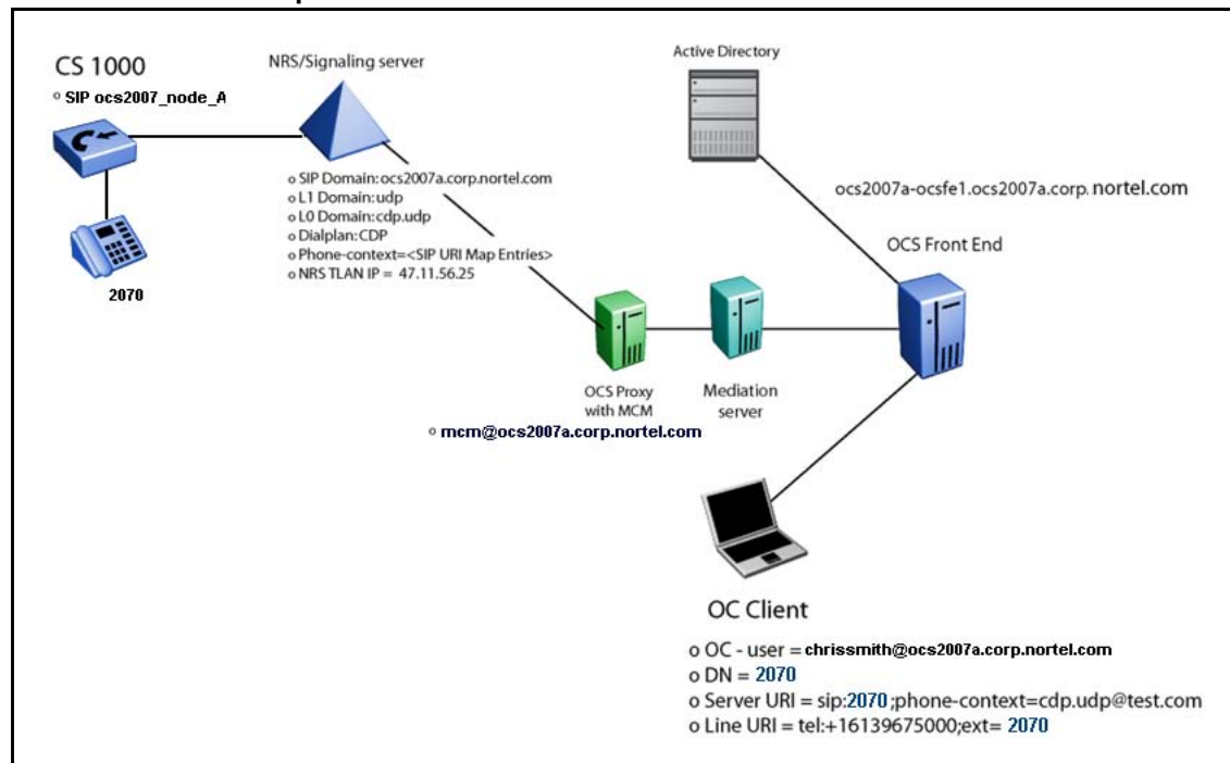
Figure 152 Overview of lab setup
