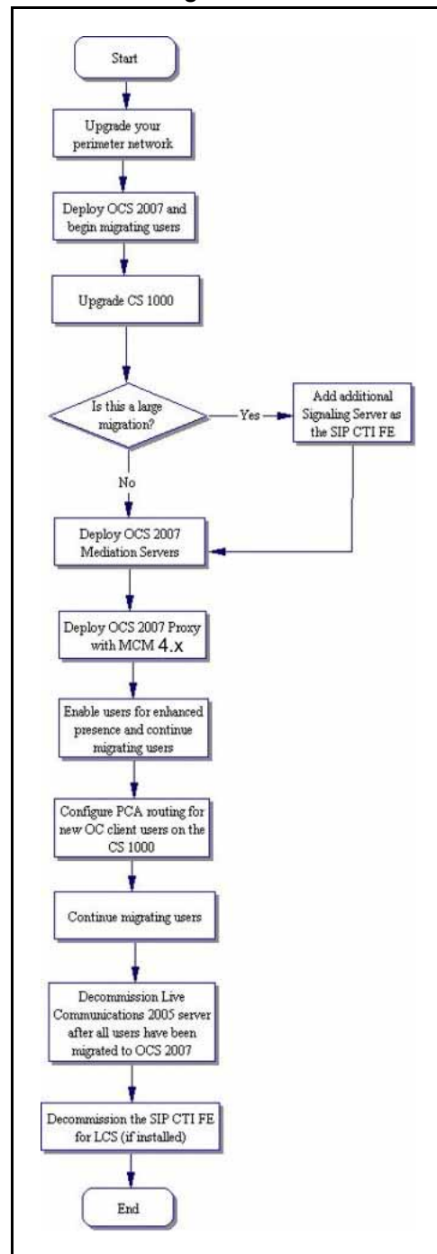
Figure 32 LCS to OCS migration task flow
