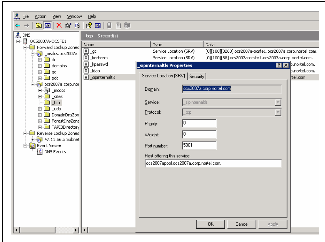
Figure 176 sipinternaltls SRV records
