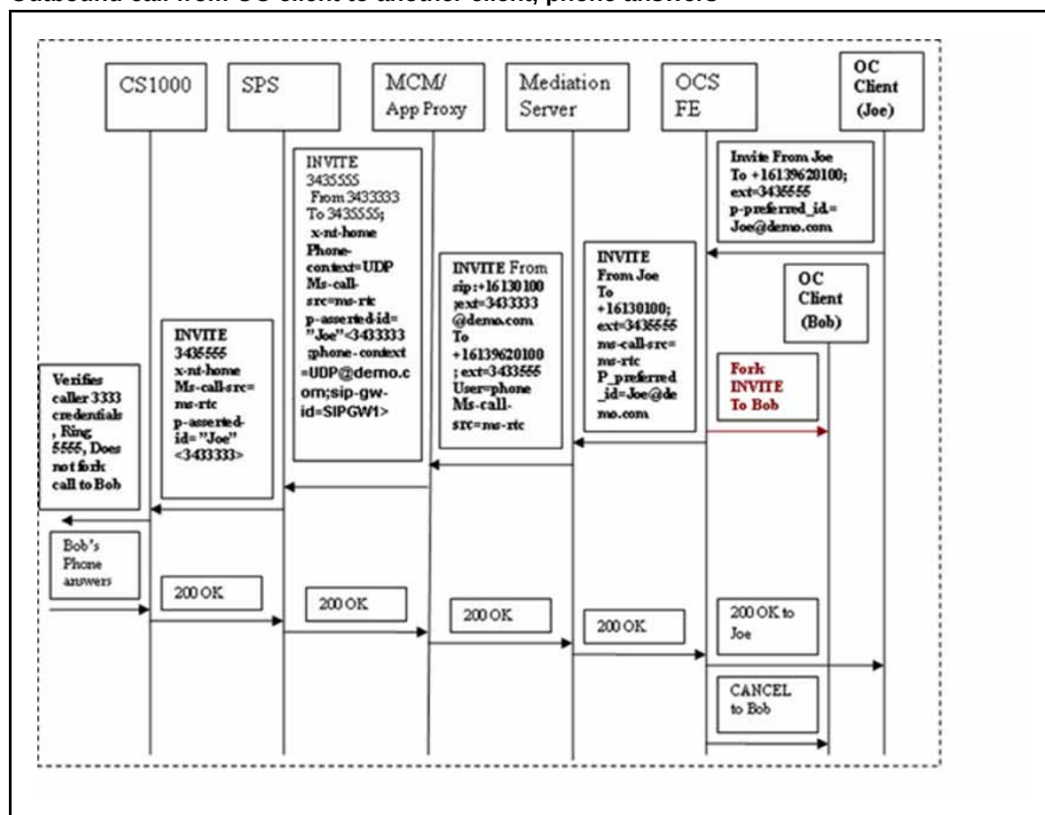
Figure 145 Outbound call from OC client to another client, phone answers
