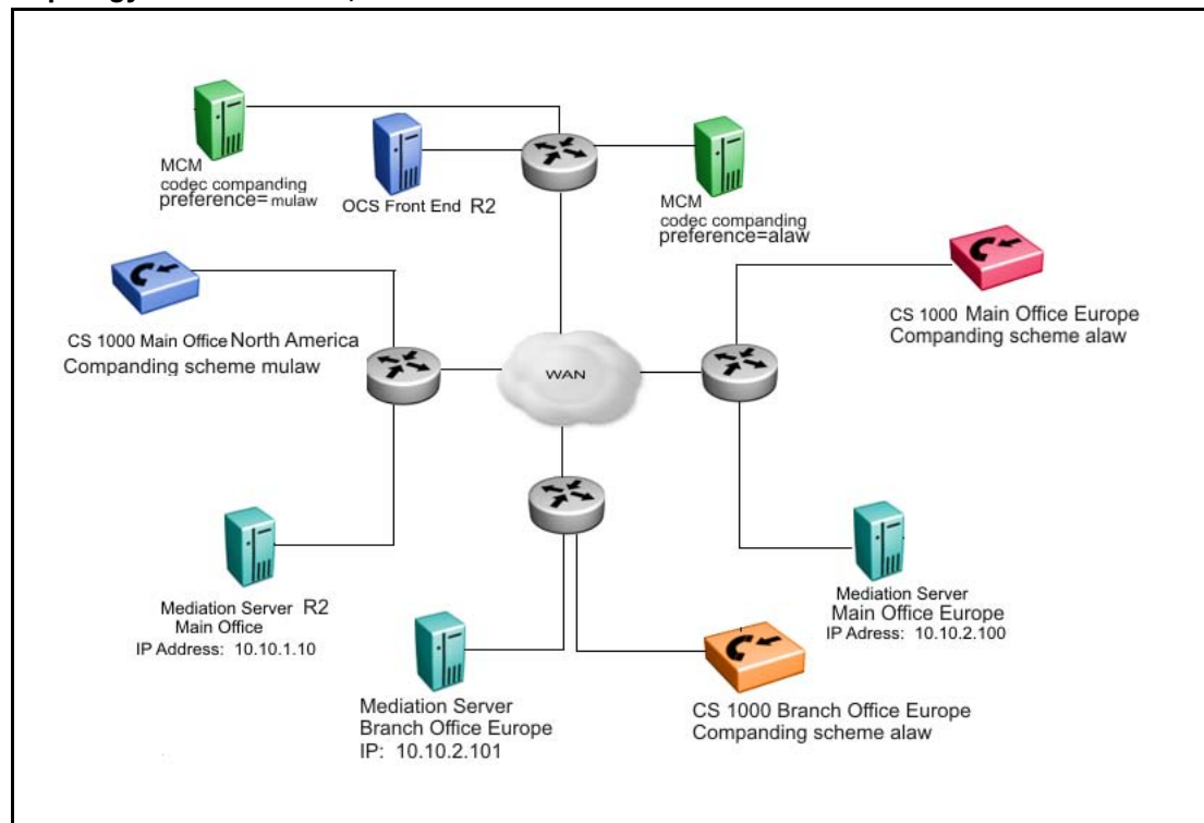
Figure 72 Topology 3—Two MCMs, mixed release of Mediation Servers
