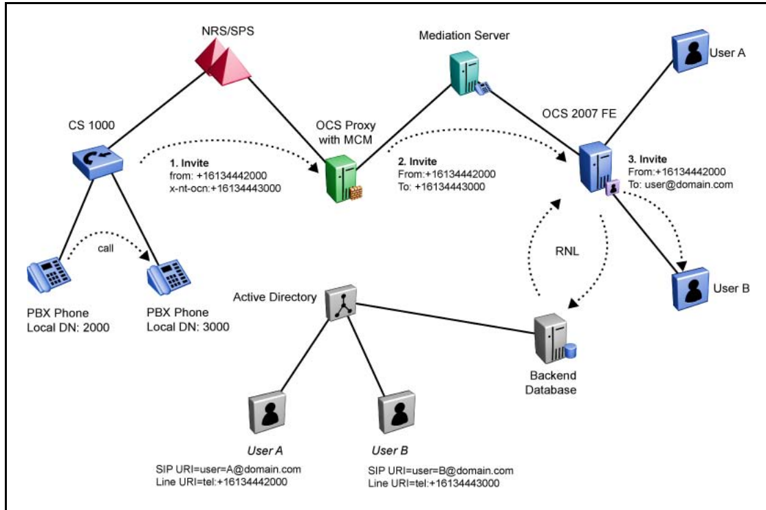
Figure 26 Call between two DID users
