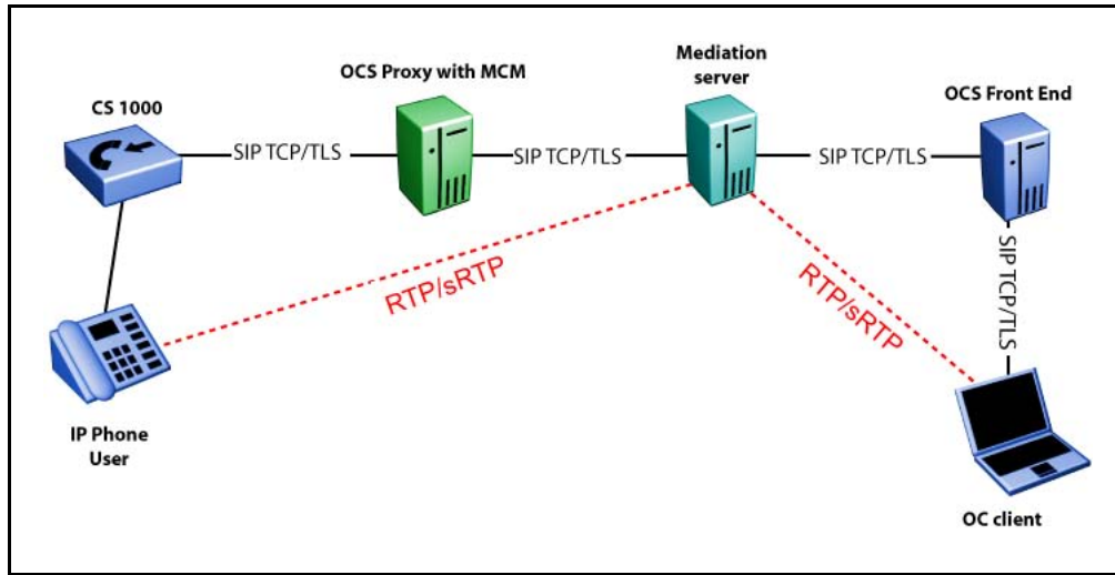
Figure 4 Signaling and media path between OC client and CS 1000
