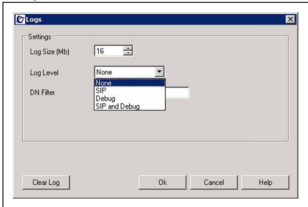
Figure 135 MCM logs
