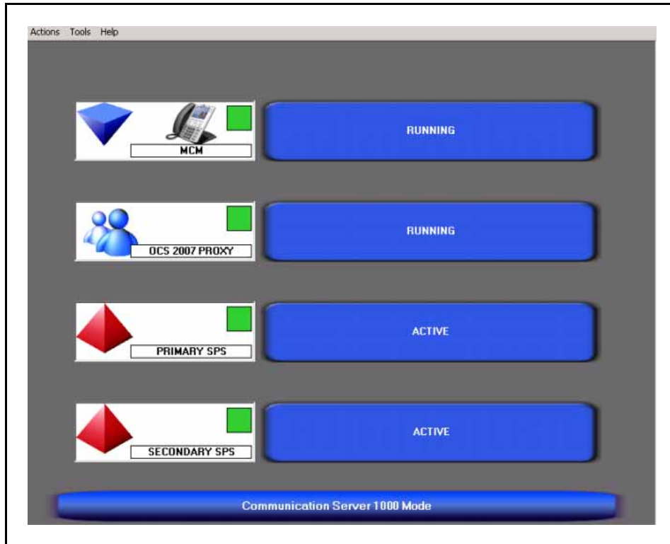
Figure 107 MCM status
