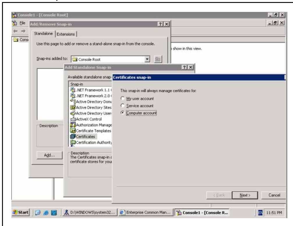
Figure 98 Certificate snap-in
