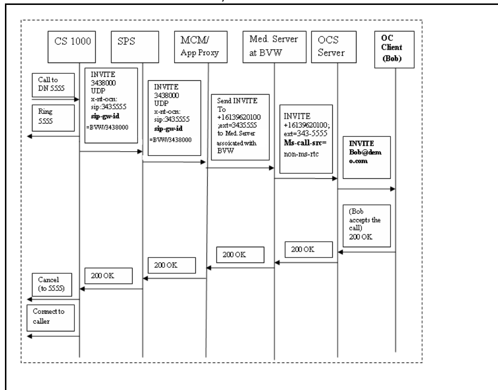
Figure 142 Inbound call to OC client with SPS, OC client answers
