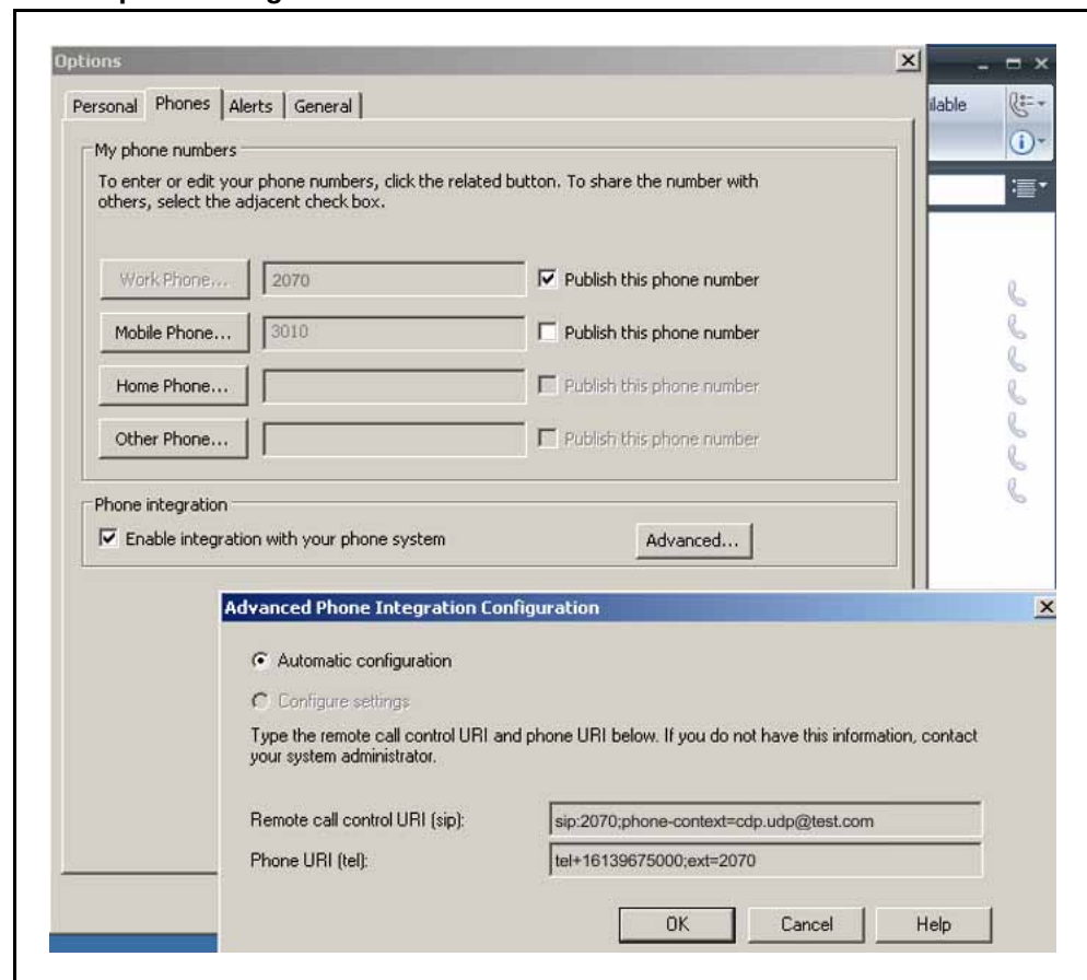
Figure 76 Enable phone integration on the client
