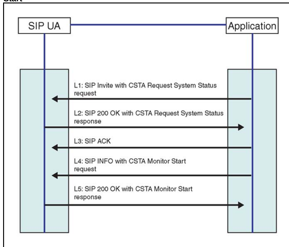
Figure 140 Message sequence diagram - CSTA Session Establishment and Monitor Start
