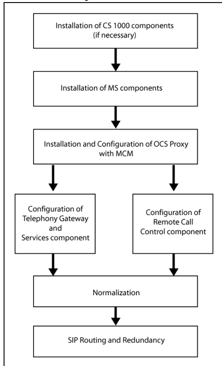
Figure 41 Installation and configuration flow
