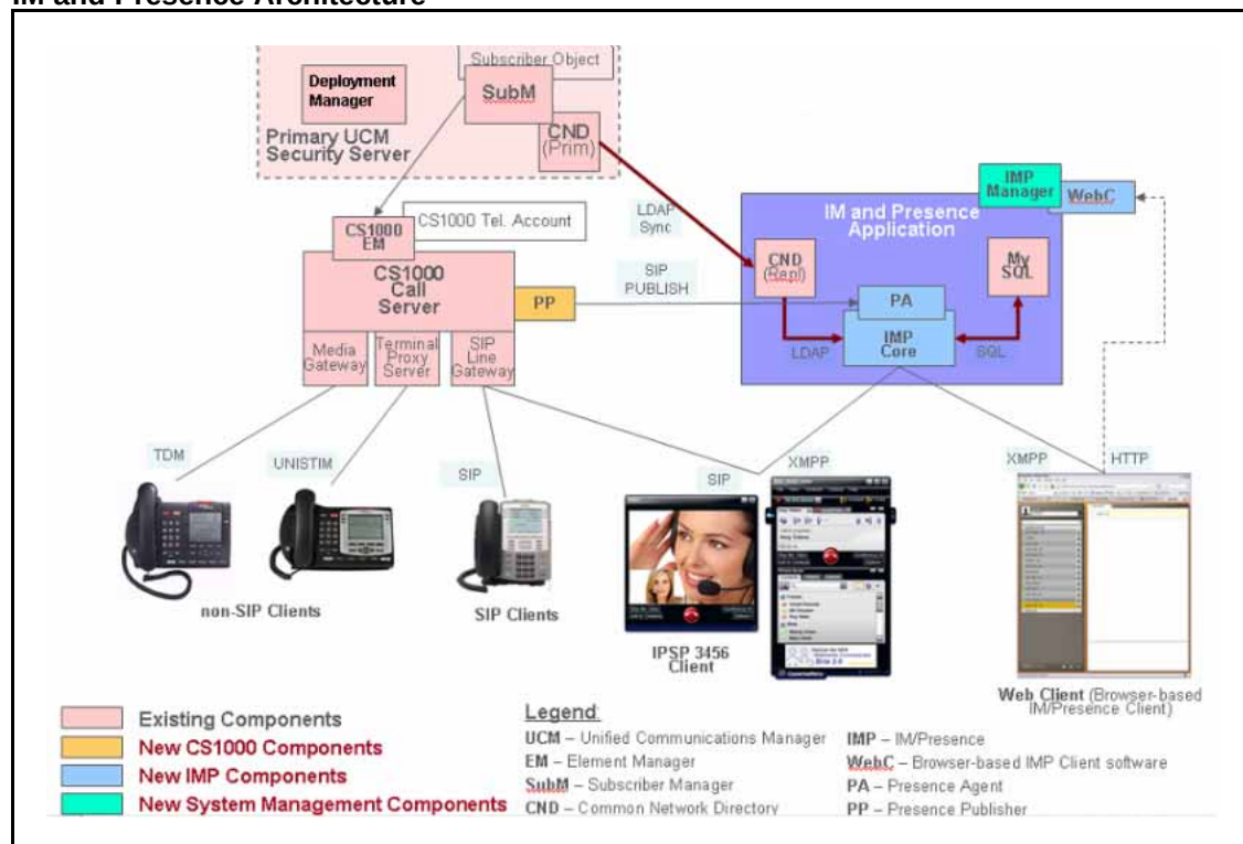
Figure 1 IM and Presence Architecture
