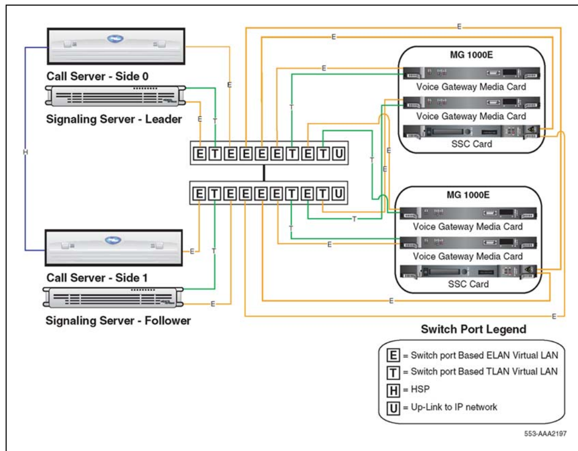
Figure 29 CS 1000E - Physically co-located Side 0 and Side 1
