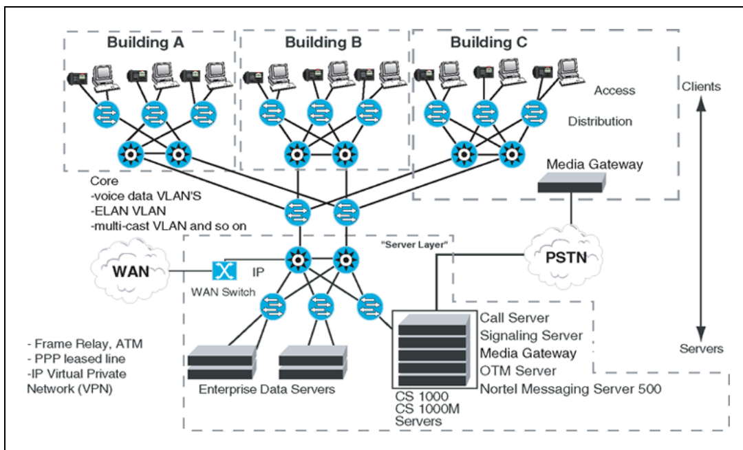
Figure 5 Large campus network example
