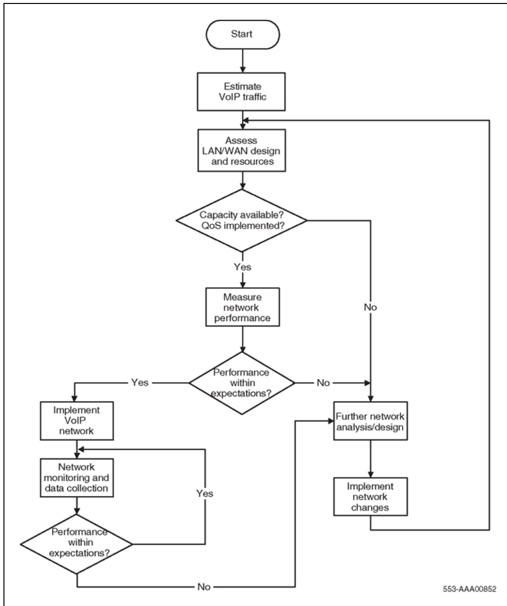
Figure 1 Network assessment flow chart
