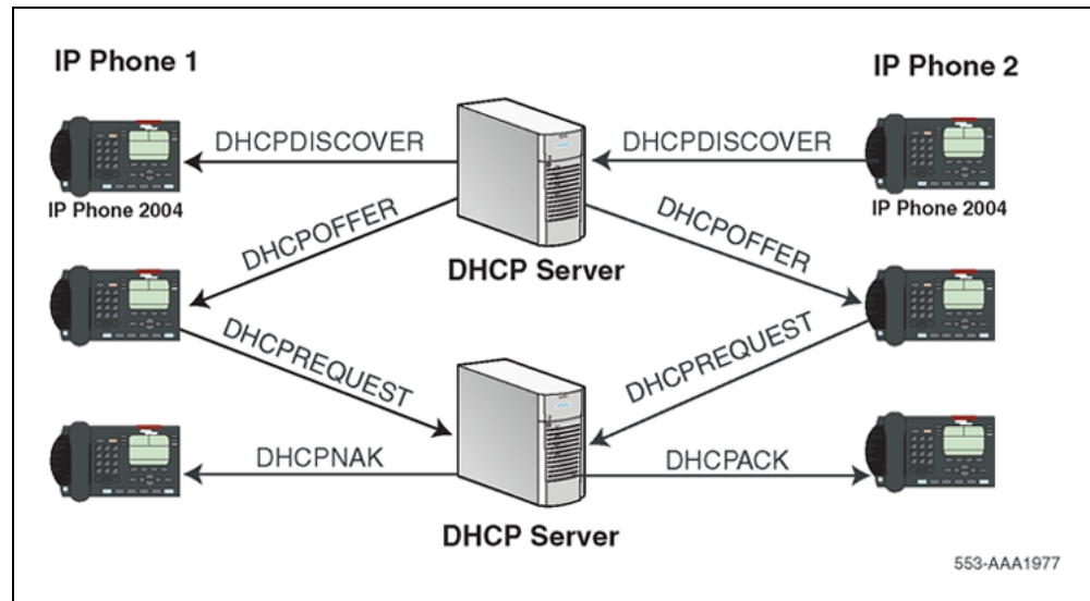
Figure 47 IP acquisition sequence: Case 3
