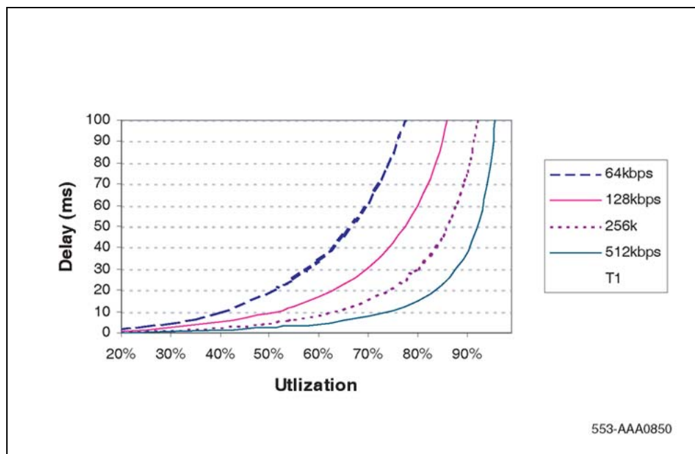
Figure 25 Queuing delay of various links
