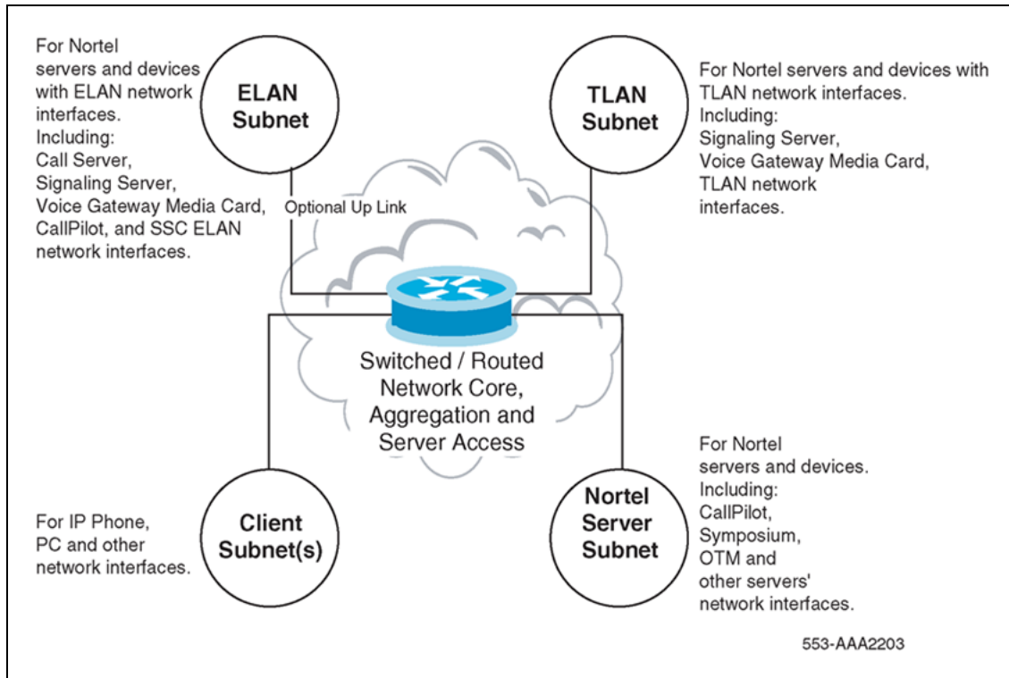
Figure 26 Example: Enterprise IP Network (that is, describing the whole of the data network structure)
