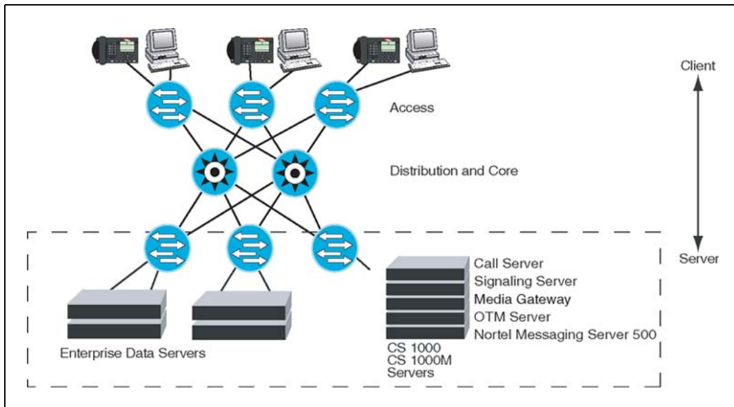
Figure 5 Large campus network example
