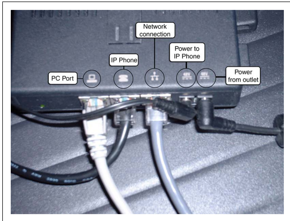
Figure 10 3-port switch
