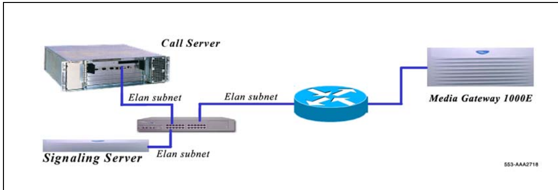
Figure 40 Media Gateway separation from the Call Server by Layer 3 router
