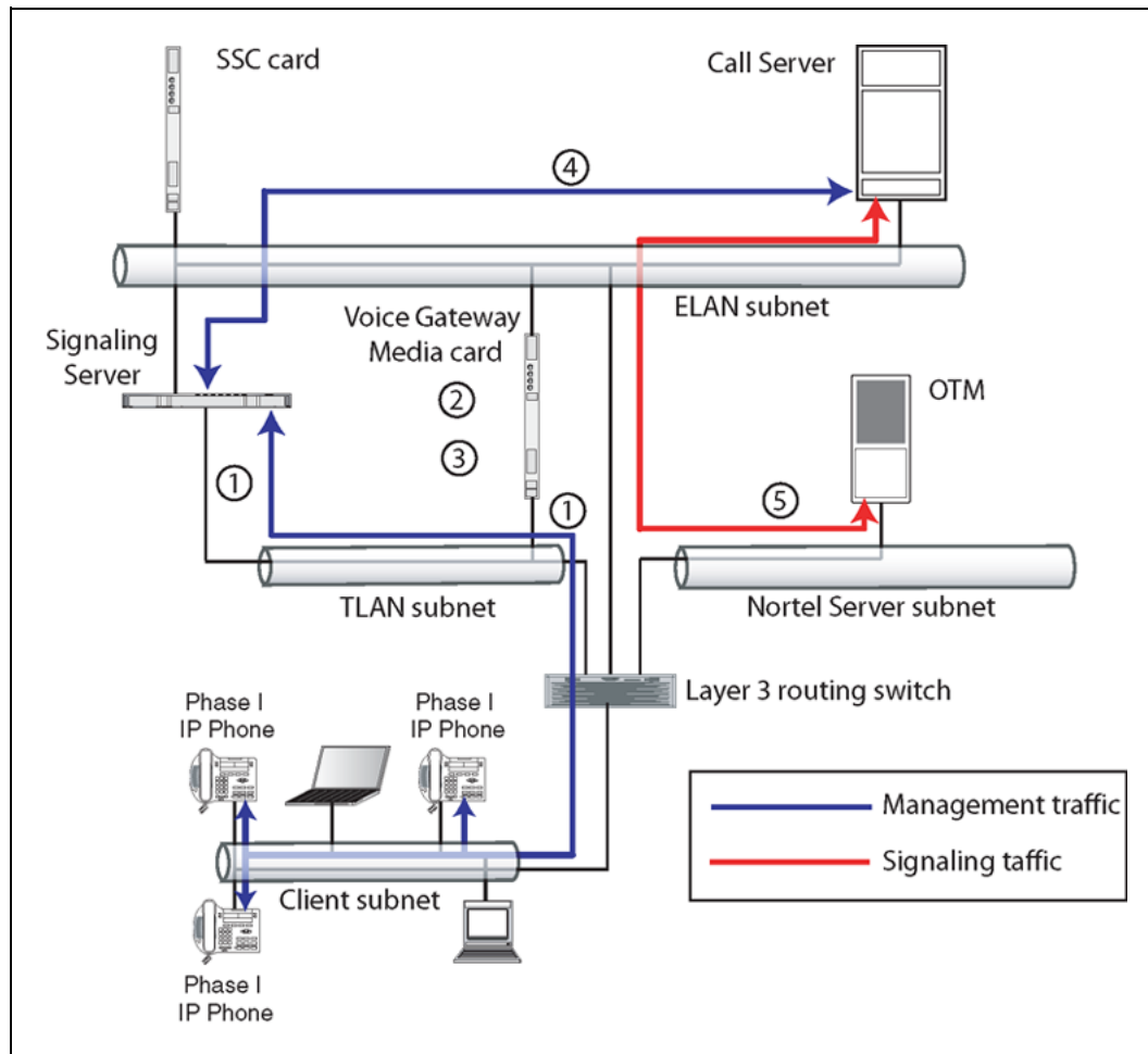
Figure 42 Phase I IP Phones voice quality monitoring flow diagram
