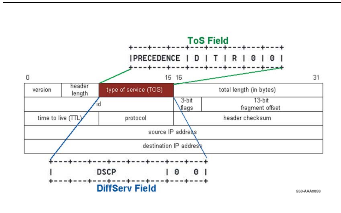
Figure 12 IPv4 header showing DSCP location
