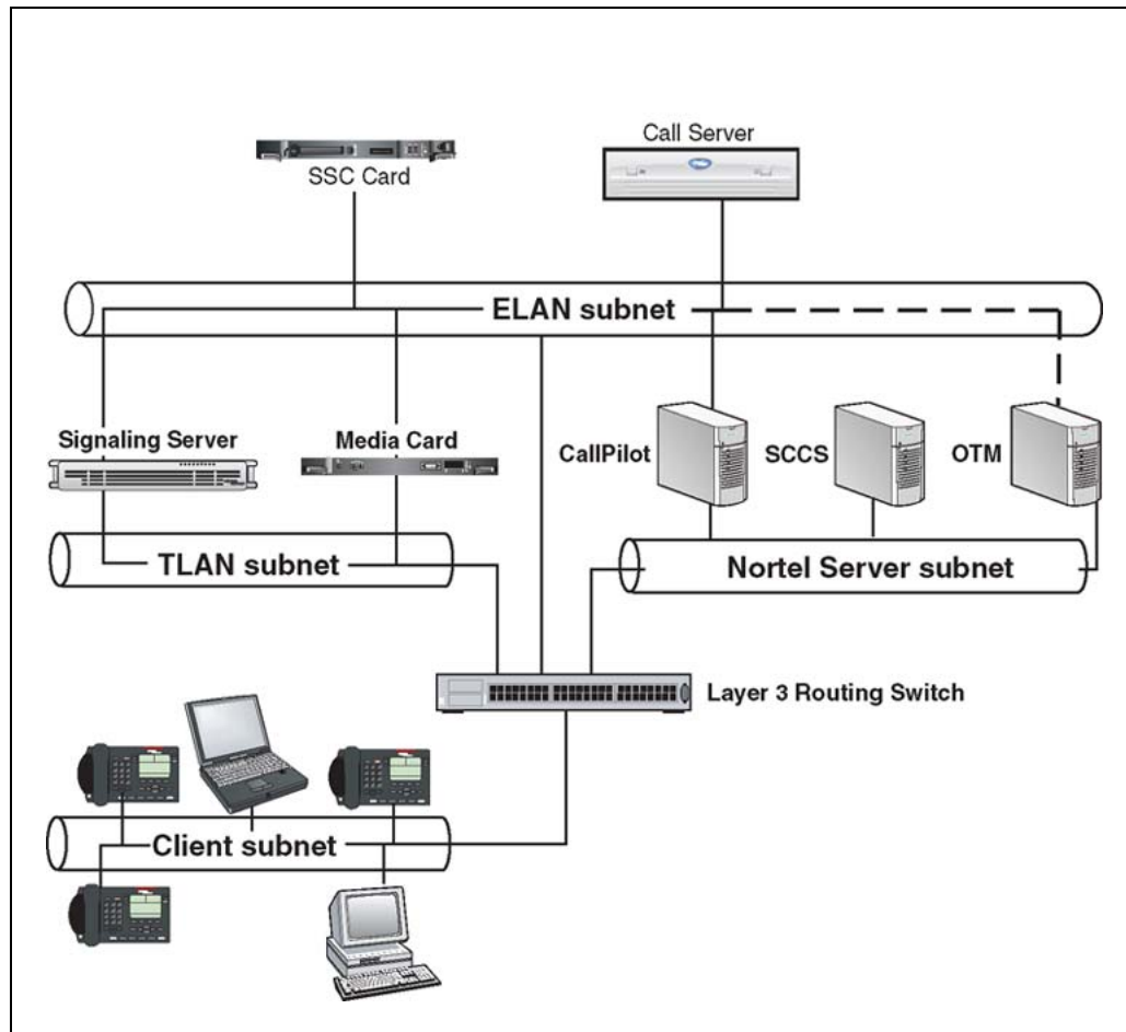
Figure 27 Layer 2 Ethernet connection model
