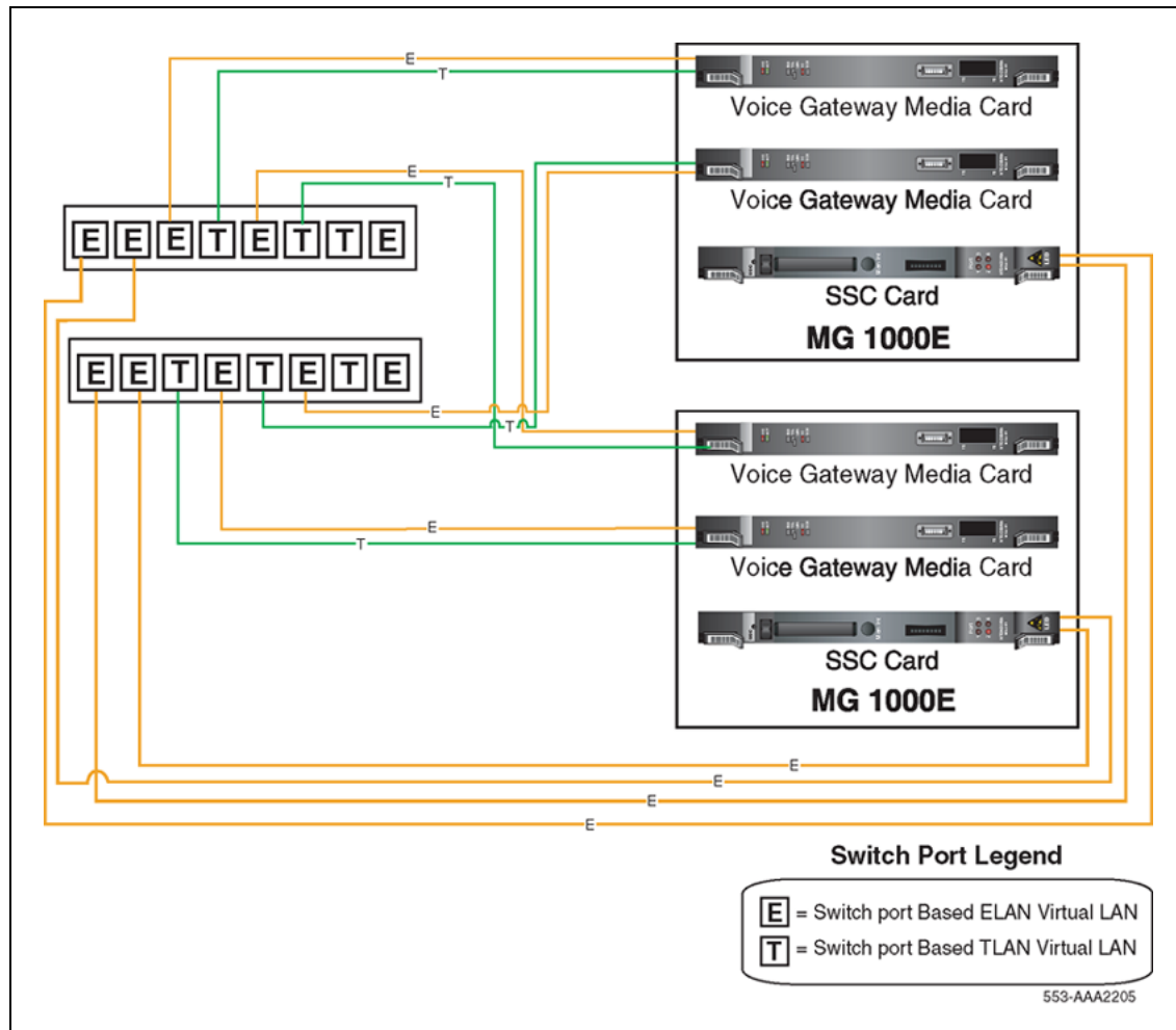
Figure 37 MG 1000E redundancy details
