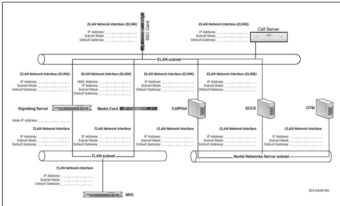
Figure 41 CS 1000S sample system layout
