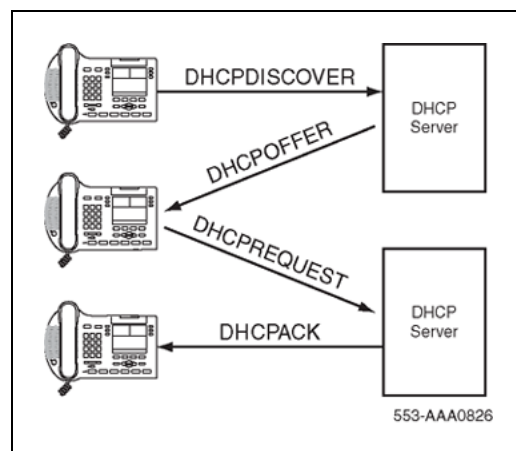
Figure 45 IP acquisition phase: Case 1
