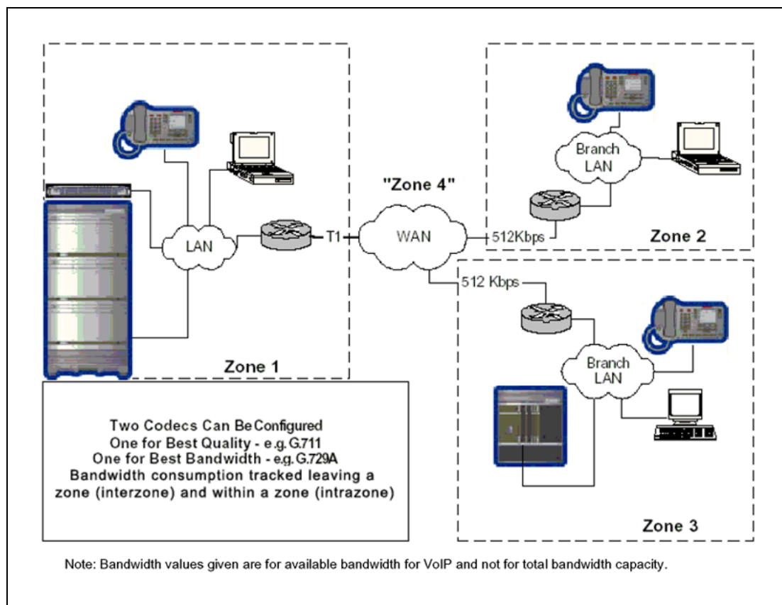
Figure 16 Bandwidth management example
