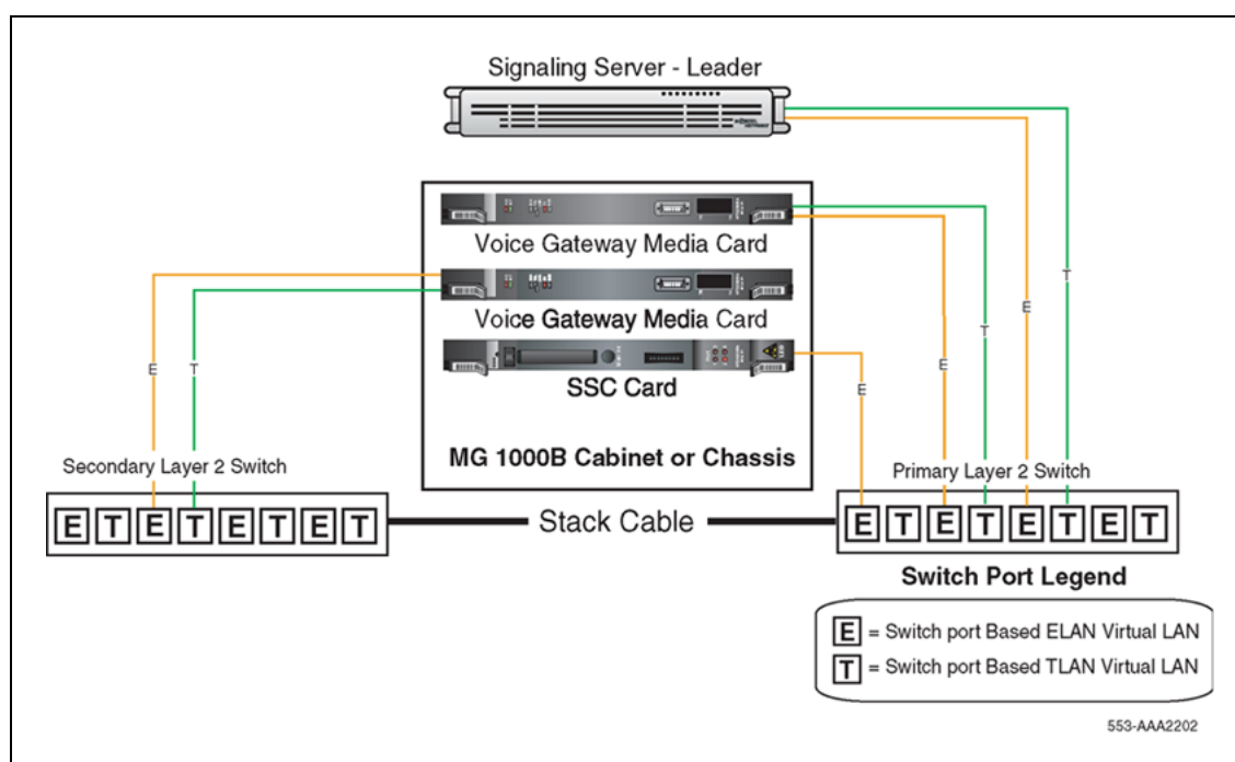
Figure 28 MG 1000B detailed core system connections
