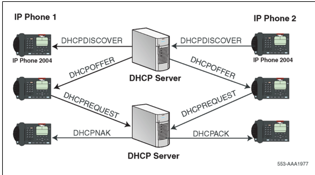
Figure 46 IP acquisition sequence: Case 2
