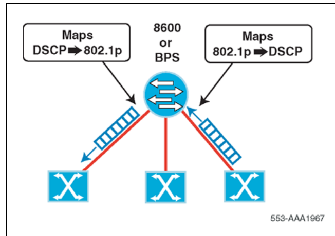
Figure 13 Mapping DSCP to 802.1p
