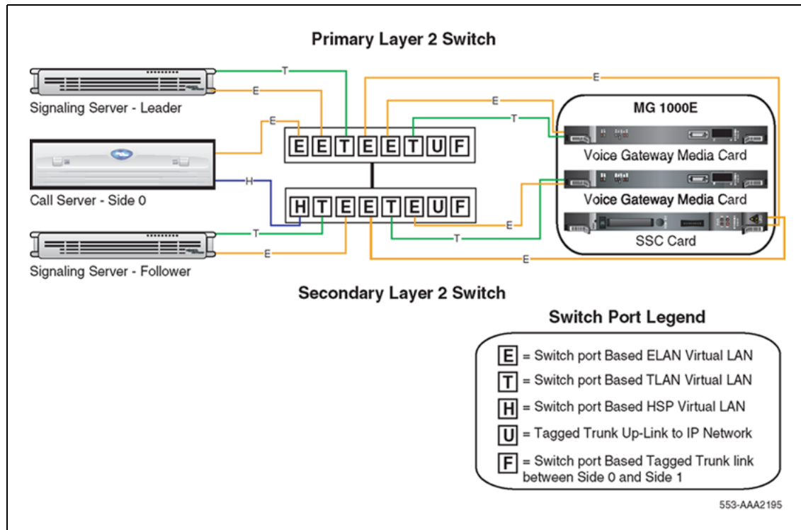
Figure 39 Campus redundancy - Side 0 with VLANs
