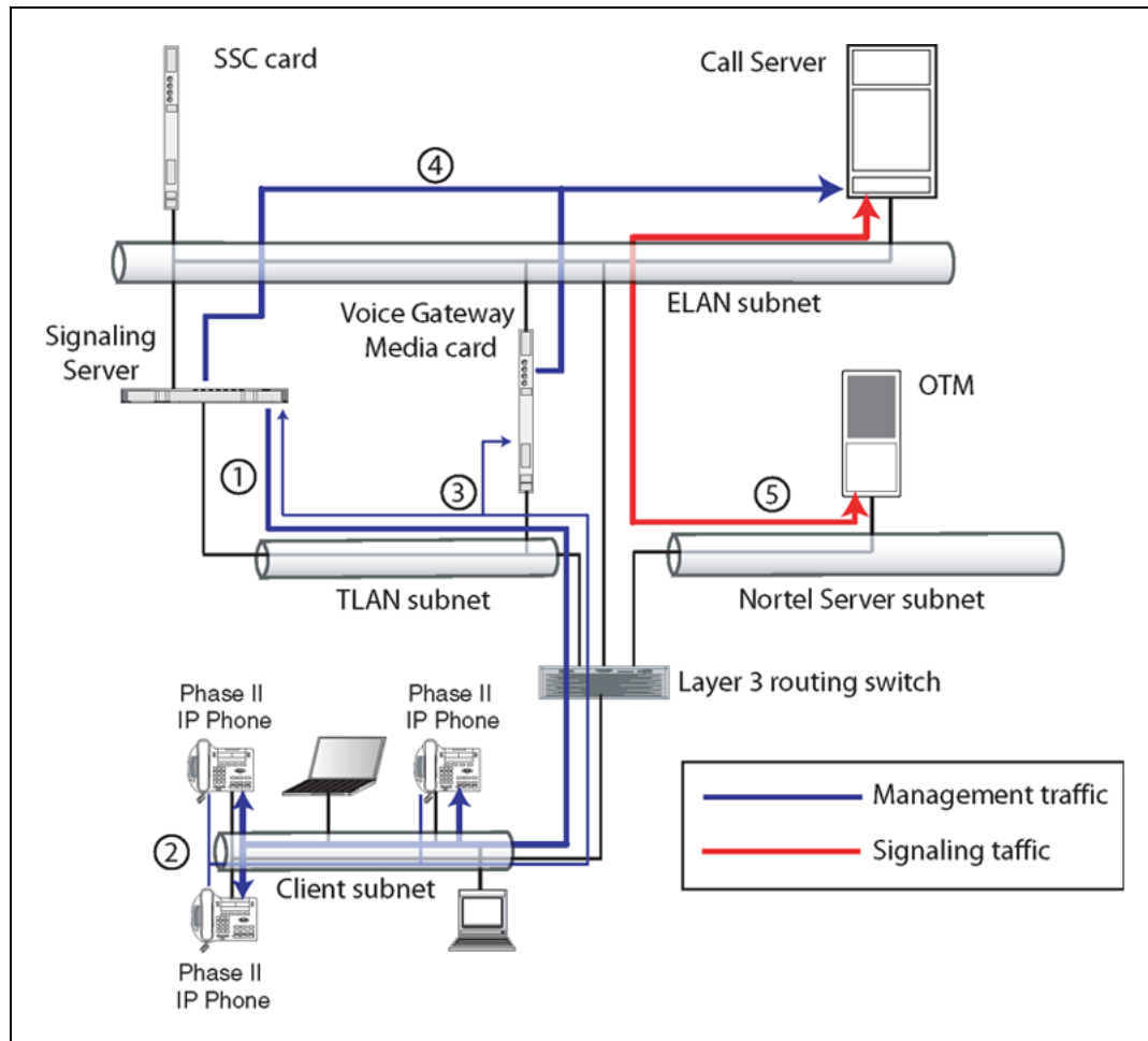
Figure 43 Phase II IP Phones voice quality monitoring flow diagram
