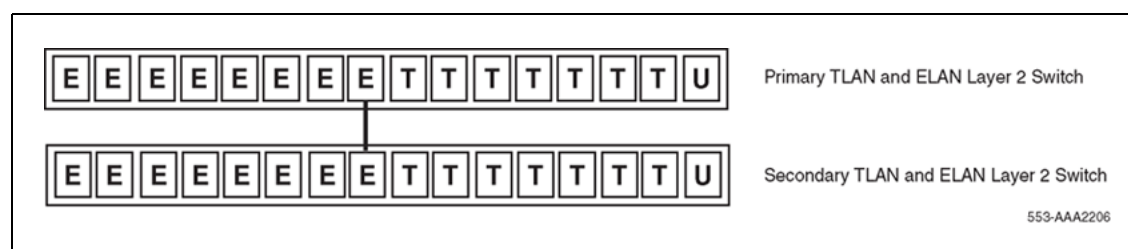
Figure 36 Redundant core network: VLANs on the Layer 2 switch infrastructure
