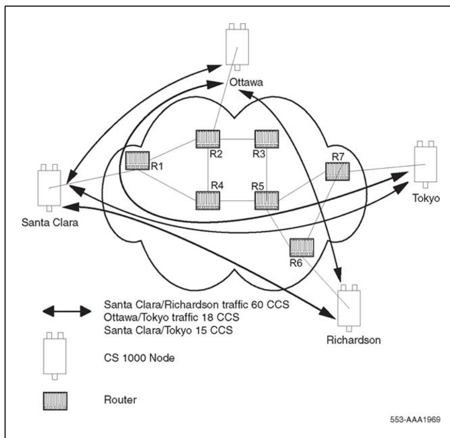
Figure 23 Calculate network load with VoIP traffic
