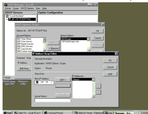
Figure 50 Add standard DHCP options to scope
