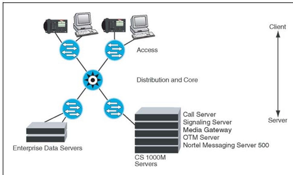
Figure 3 Small campus network example
