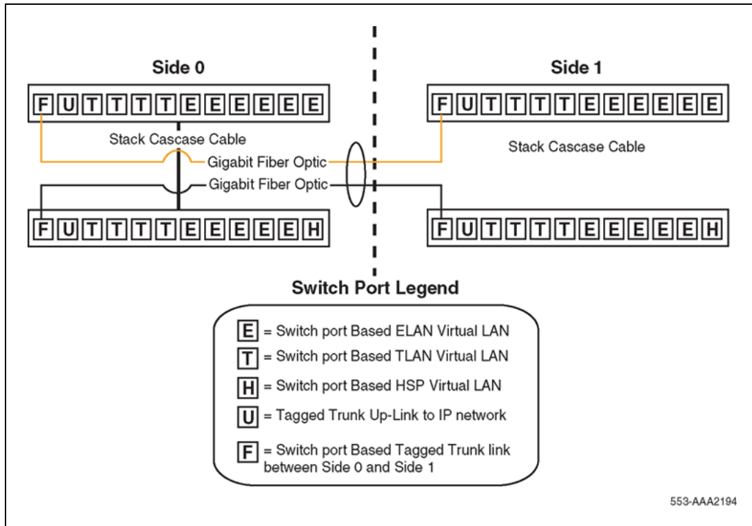
Figure 38 Campus redundancy - Layer 2 switch configuration
