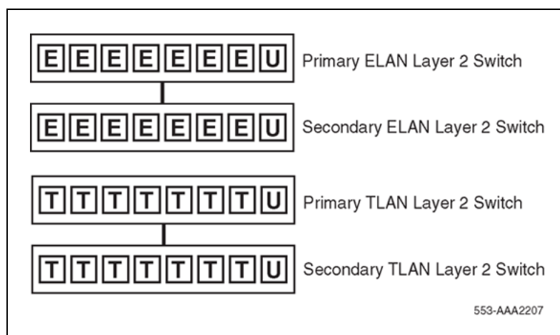
Figure 35 Redundant core network: no VLAN on Layer 2 switch infrastructure
