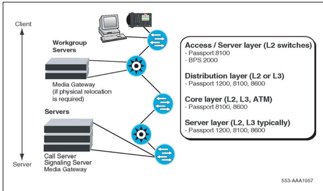
Figure 2 Campus network reference model
