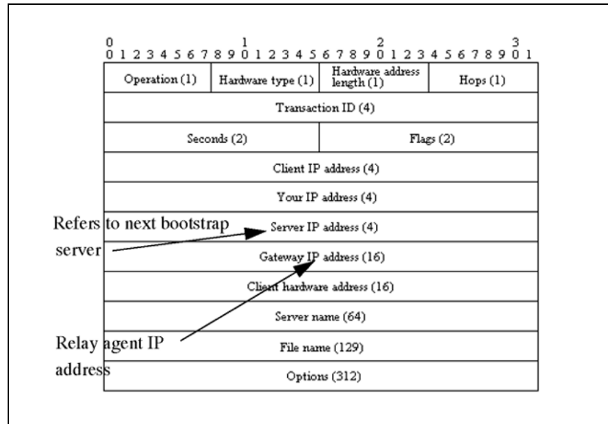
Figure 44 DHCP message format
