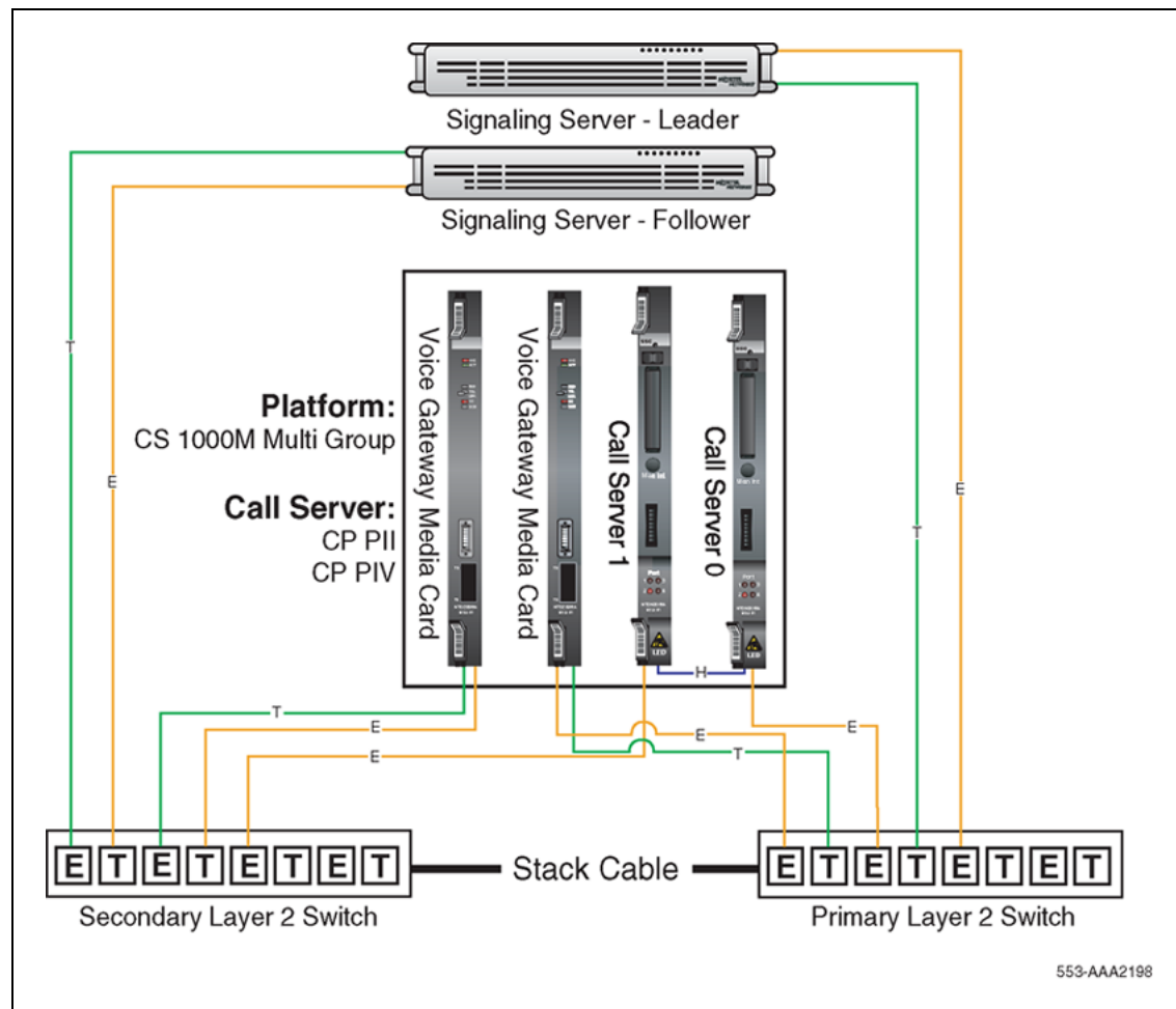
Figure 31 CS 1000M MG with dual CP PII or CP PIV Call Server cards
