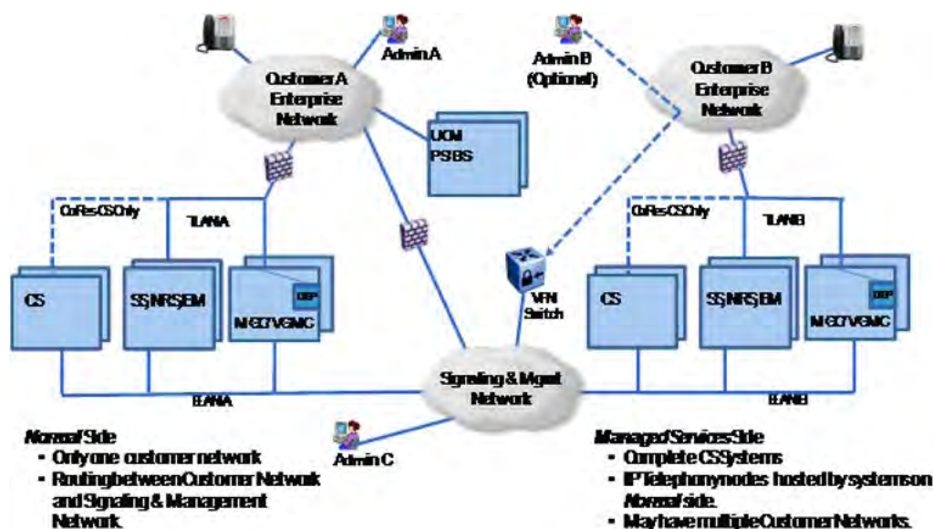
Figure 40: Hybrid Managed Services configuration
