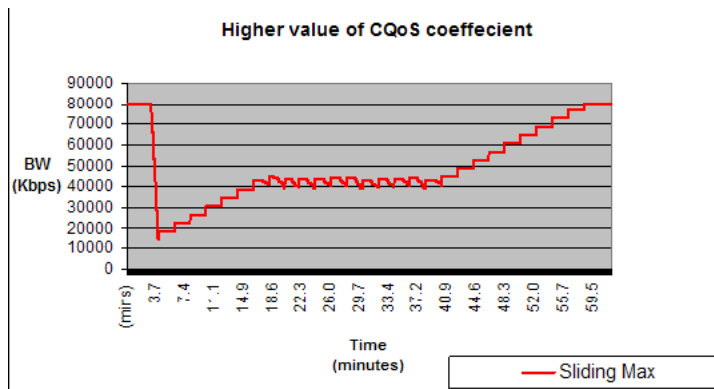
Figure 21: Effect of a high CQoS coefficient
