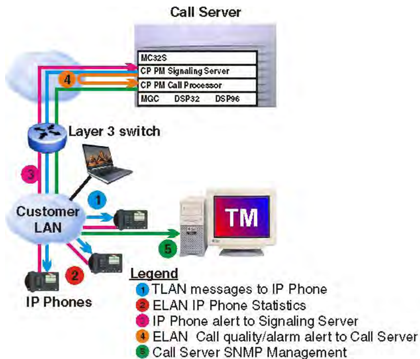
Figure 52: IP Phones voice quality monitoring
