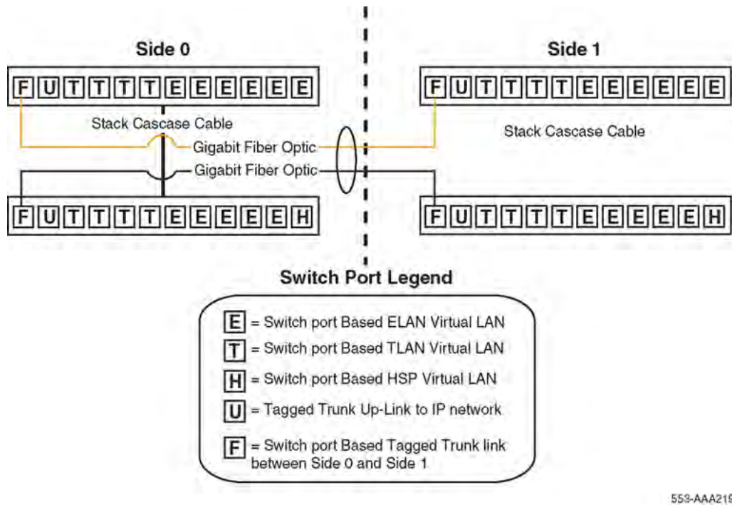
Figure 50: Campus redundancy: Layer 2 switch configuration
