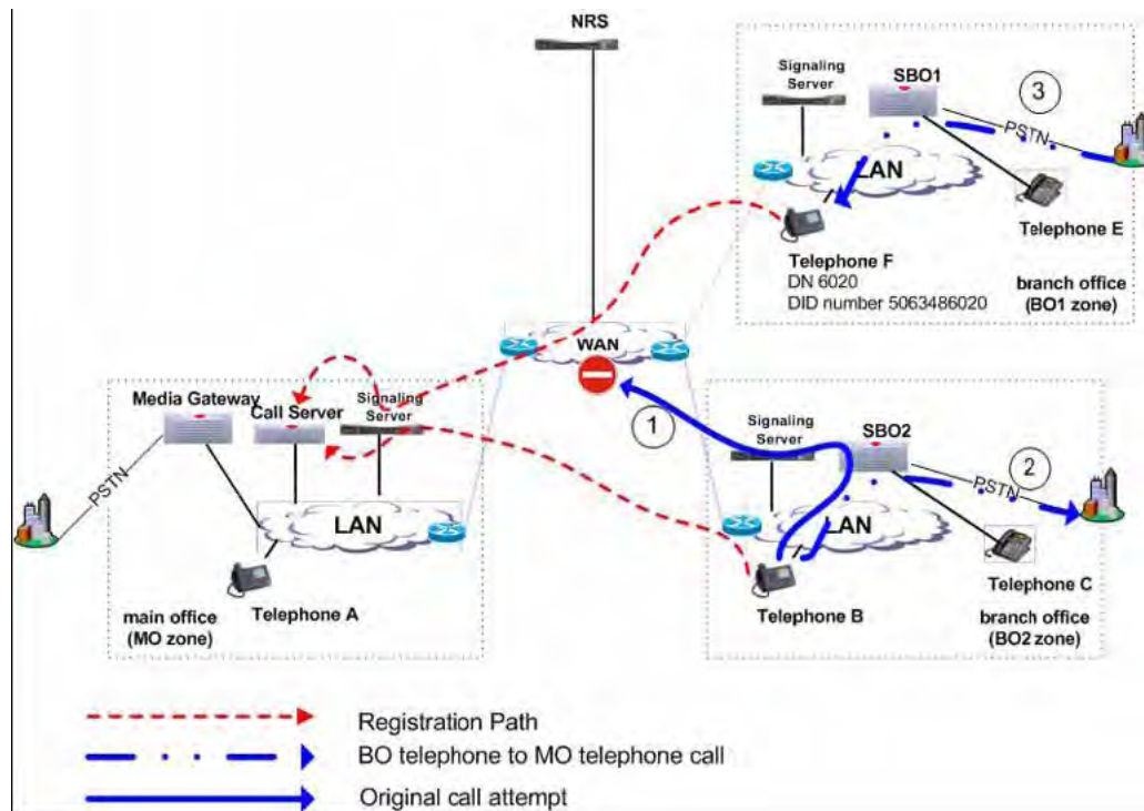
Figure 70: Call between Branch Office telephones
