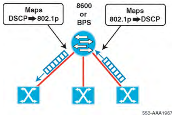
Figure 8: Mapping DSCP to 802.1p
