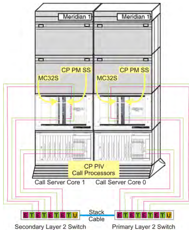
Figure 45: CS 1000M MG with dual CP PIV Call Server cards
