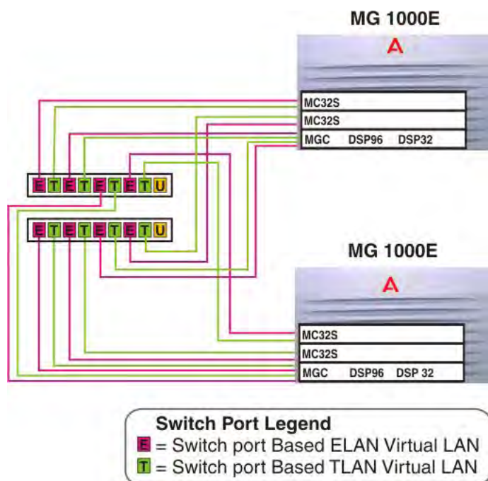
Figure 49: MG 1000E redundancy details
