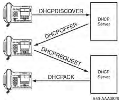
Figure 107: IP acquisition phase: Case 1
