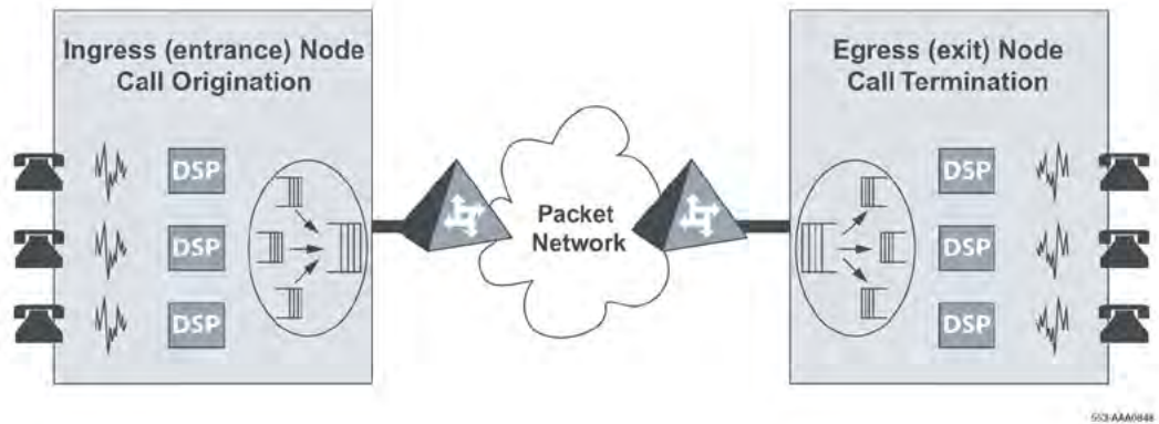
Figure 33: Sources of packet delay
