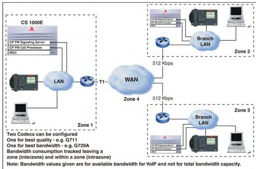
Figure 1: Bandwidth management example
