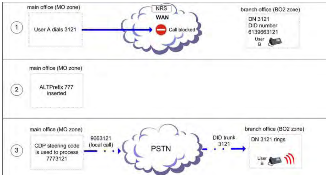
Figure 69: Digits dialed and outpulsed between main and Branch Office
