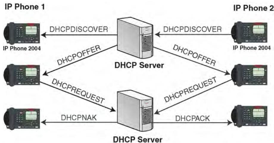
Figure 108: IP acquisition sequence: Case 2
