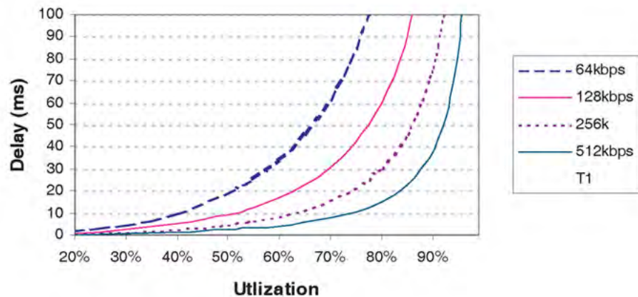
Figure 34: Queueing delay of various links
