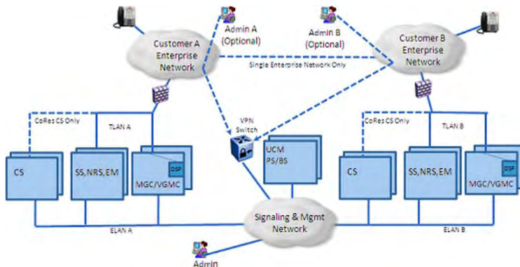
Figure 39: Managed services configuration
