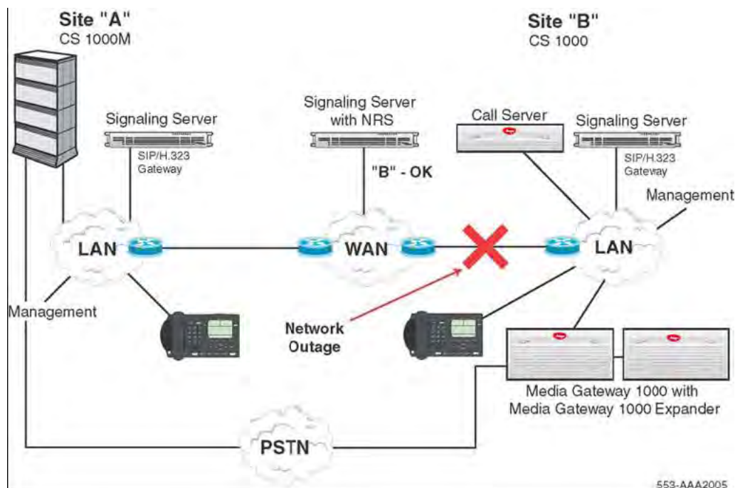
Figure 10: IP network outage at Site B
