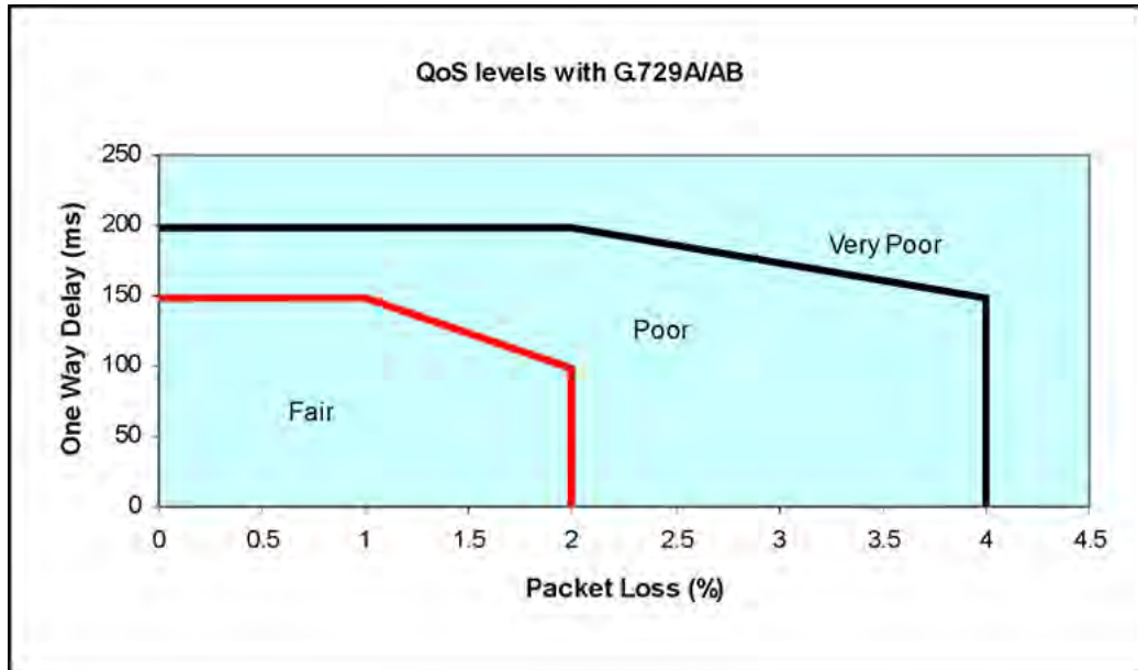
Figure 29: QoS levels with G.729A/AB codec
