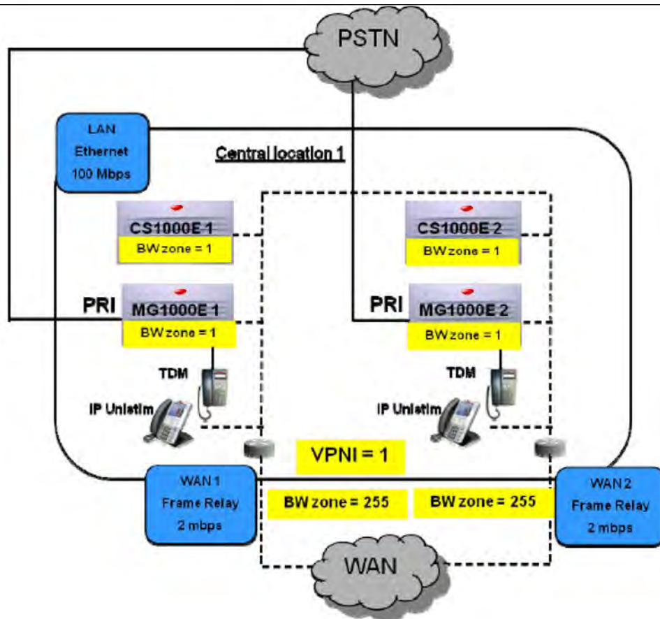
Figure 98: CS 1000 to CS 1000 on the same LAN
