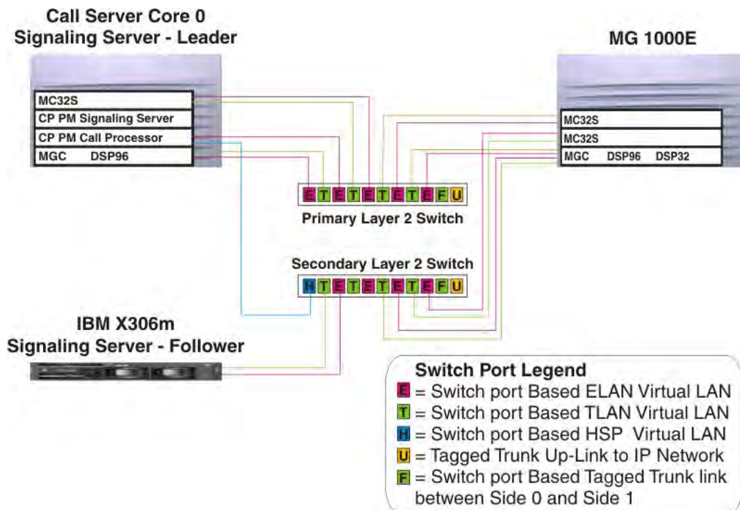
Figure 51: Campus redundancy: Side 0 with VLANs
