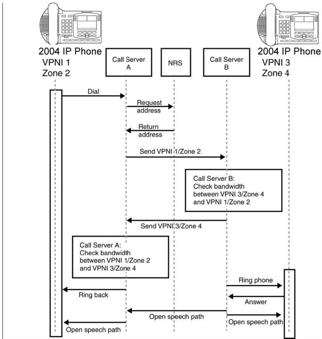
Figure 18: Call Progress with Adaptive Network Bandwidth Management
