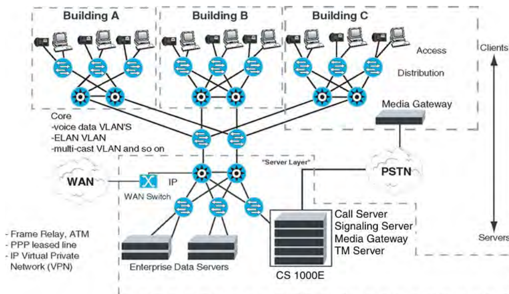
Figure 27: Large campus network example
