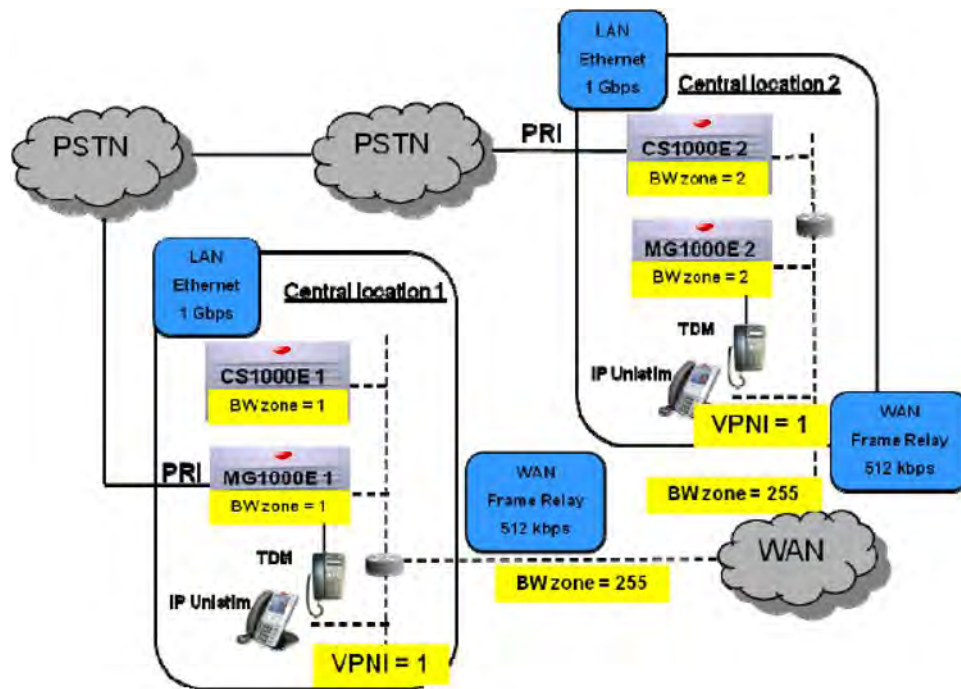
Figure 101: Network Wide Virtual Office
