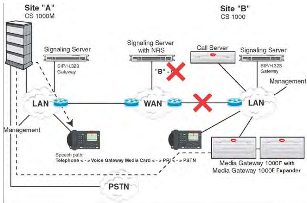
Figure 17: Call is terminated over PSTN
