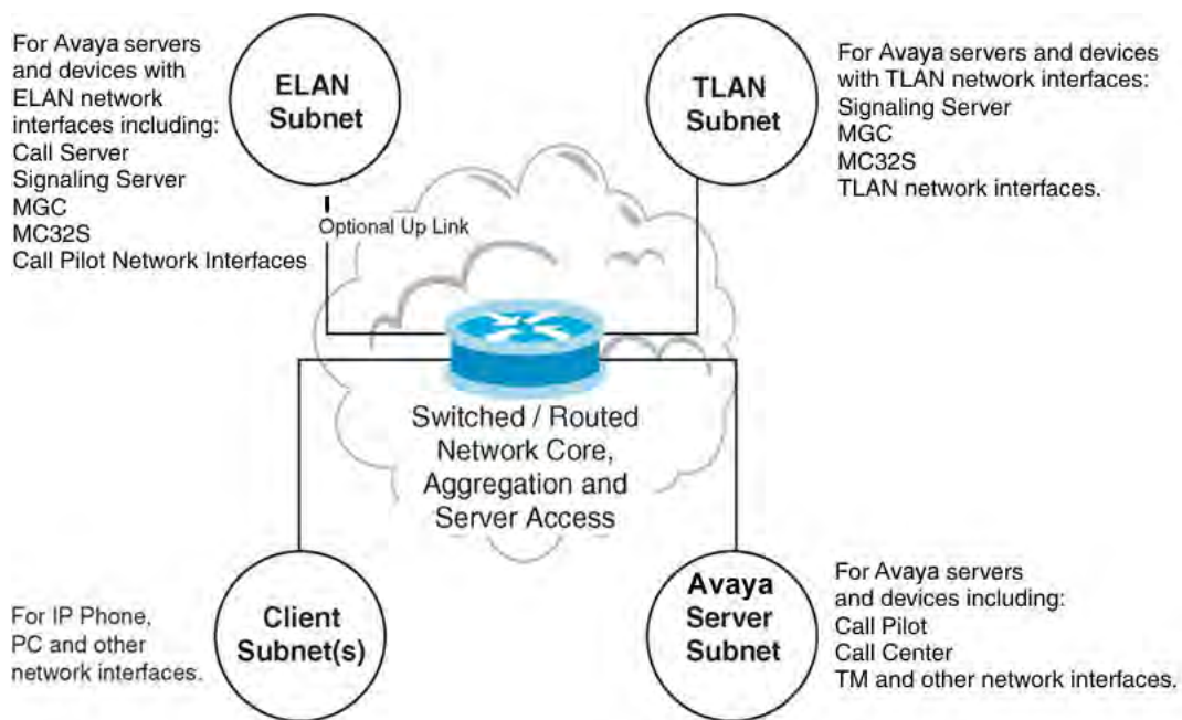
Figure 41: Example: Enterprise IP Network
