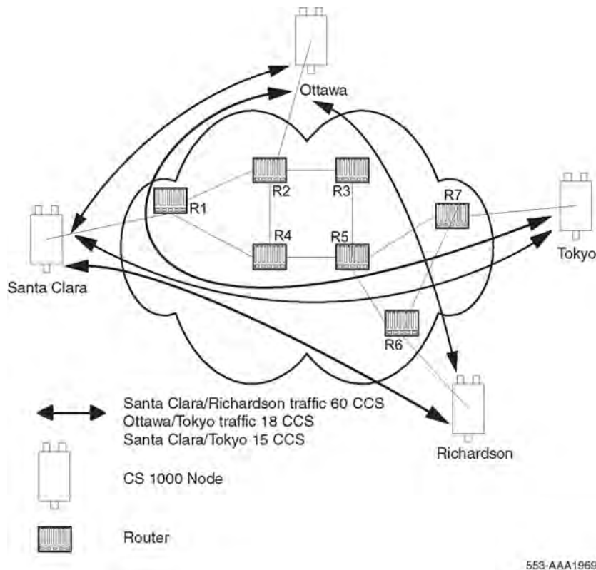
Figure 32: Network load with VoIP traffic
