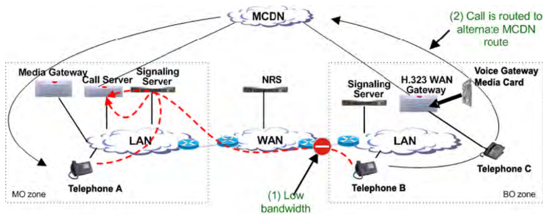
Figure 65: Example of Alternate Call Routing
