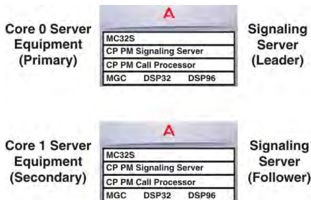
Figure 46: Primary and secondary equipment groups
