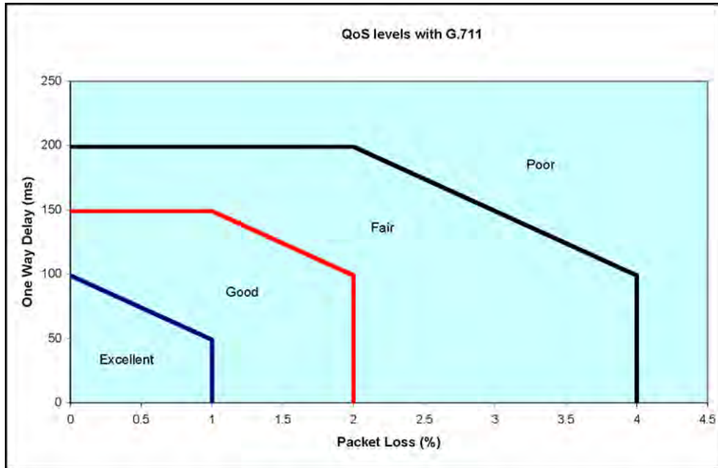
Figure 30: QoS level with G.711 codec
