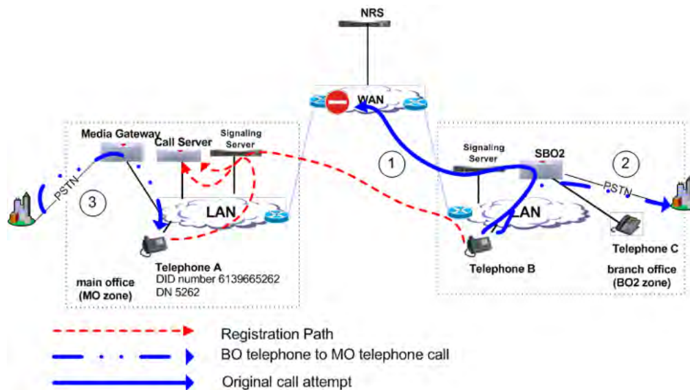
Figure 66: Call from a branch office telephone in normal mode to a main office telephone
