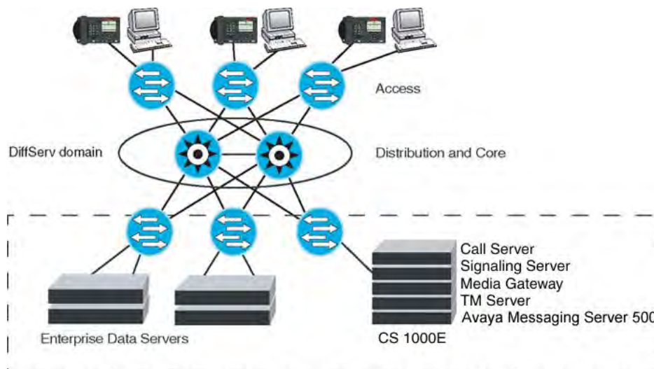
Figure 6: DiffServ-based QoS architecture
