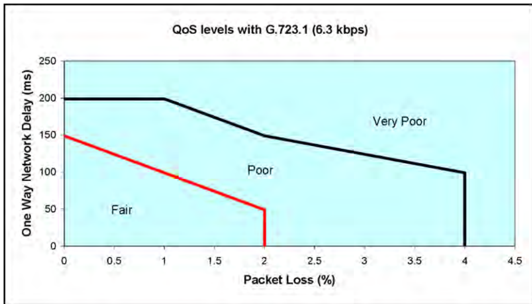
Figure 31: QoS level with G.723 codec
