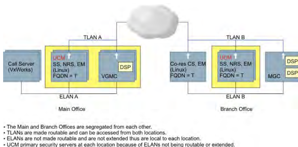
Figure 36: Release 6.0 and later customer network configuration
