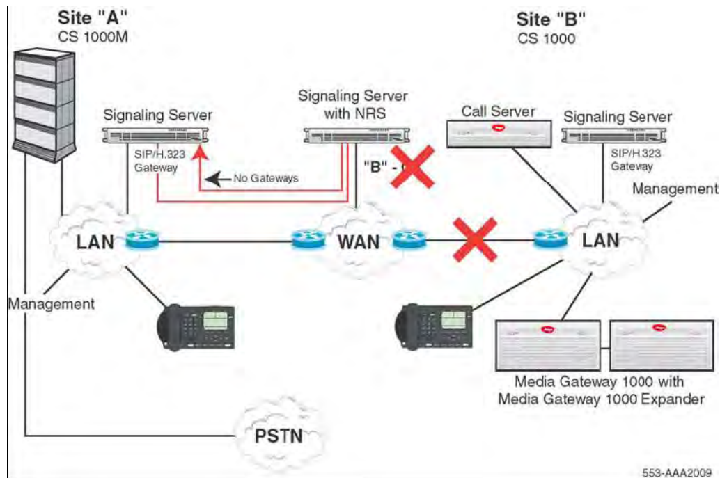
Figure 14: No SIP/H.323 Gateways are available for the dialed DN
