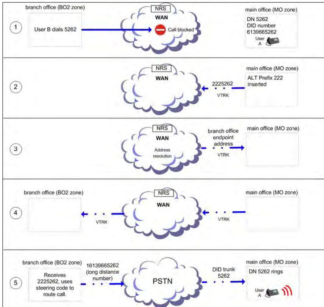
Figure 67: Digits dialed and outpulsed between Branch Office and main office
