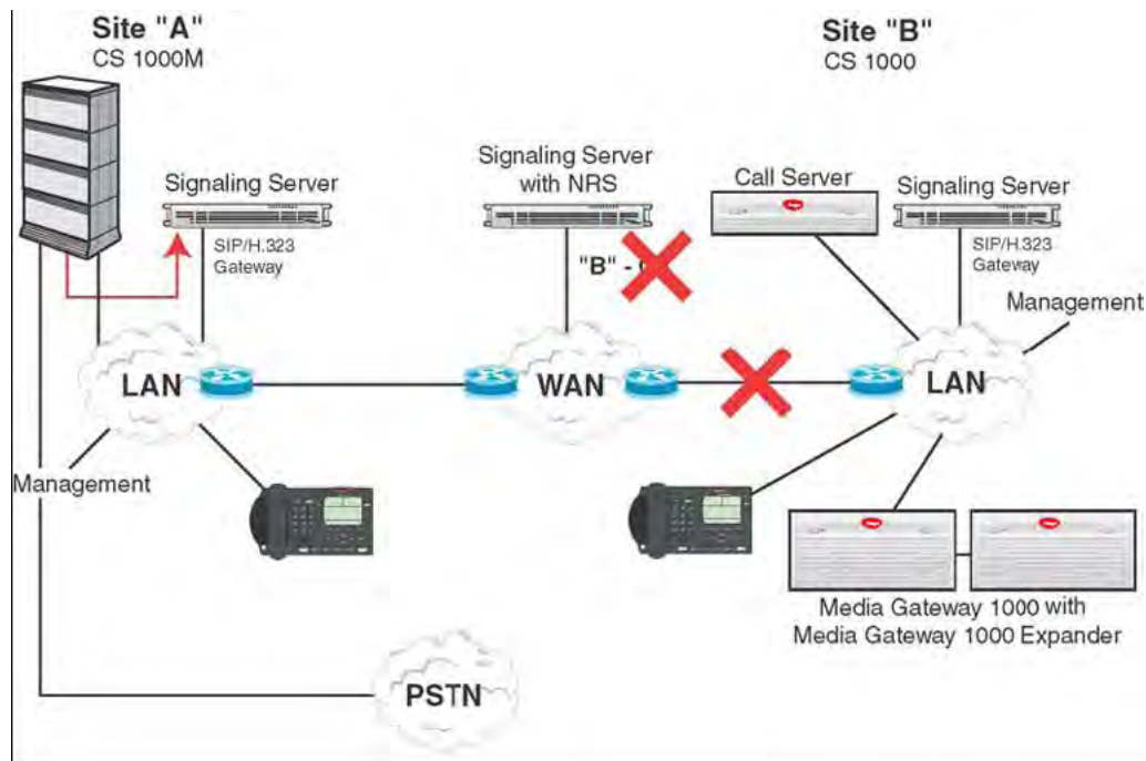
Figure 13: Call Server A routes the call to the IP network
