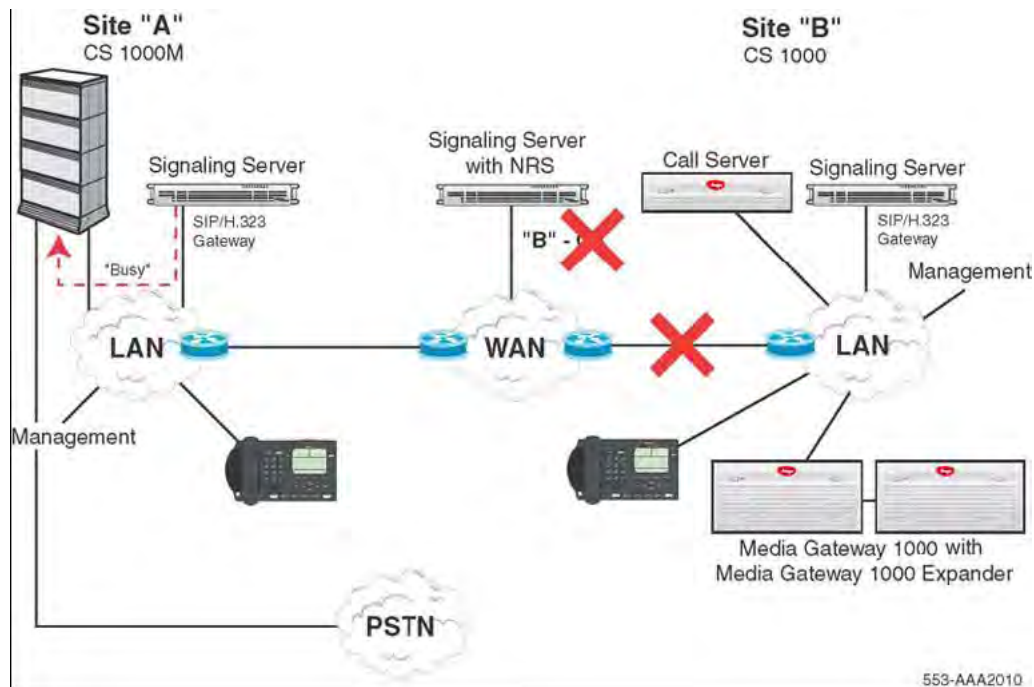
Figure 15: SIP/H.323 Gateway A replies to Call Server A
