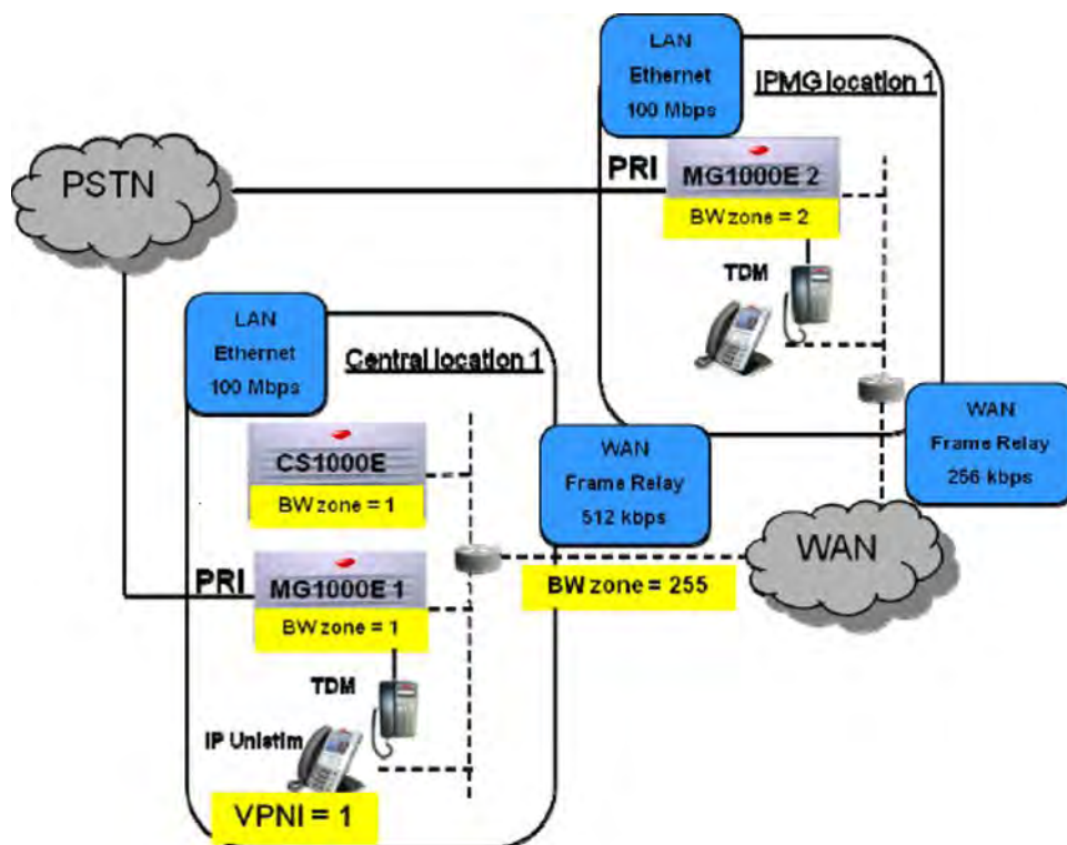
Figure 91: Distributed Media Gateway
