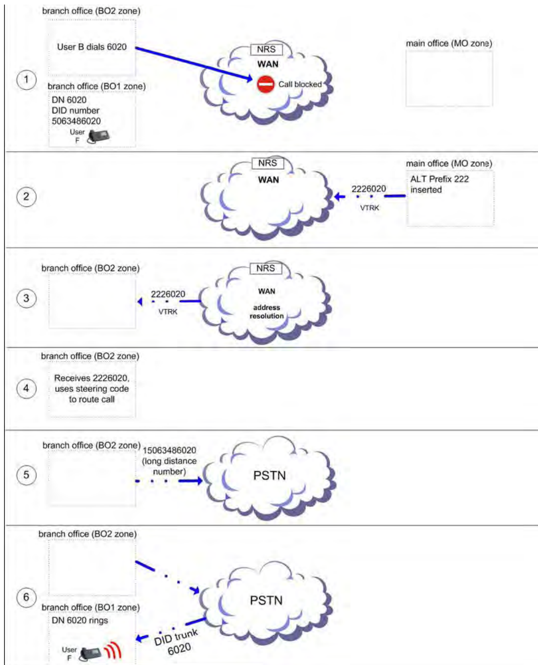
Figure 71: Digits dialed and outpulsed between two Branch offices
