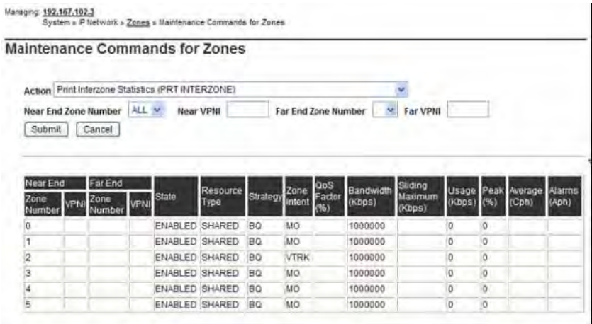
Figure 56: Intrazone statistics example
