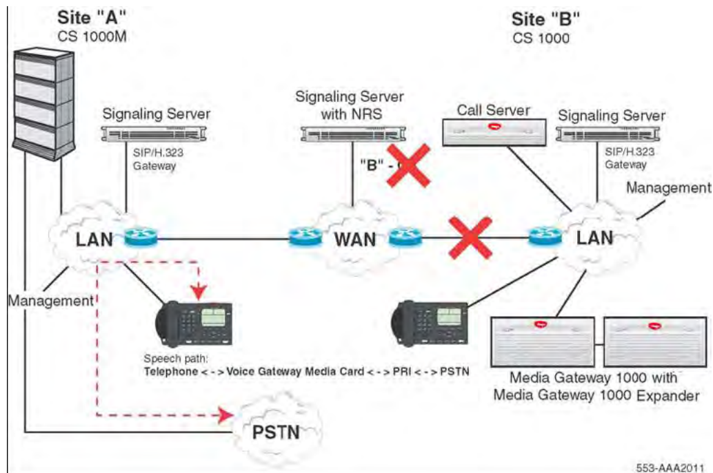
Figure 16: Call Server A chooses the next route in the Route List Data Block
