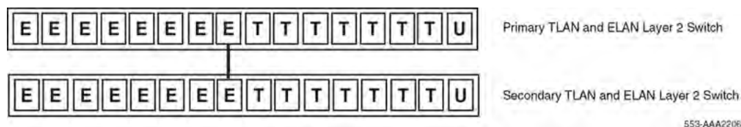
Figure 48: Redundant core network: VLANs on the Layer 2 switch infrastructure
