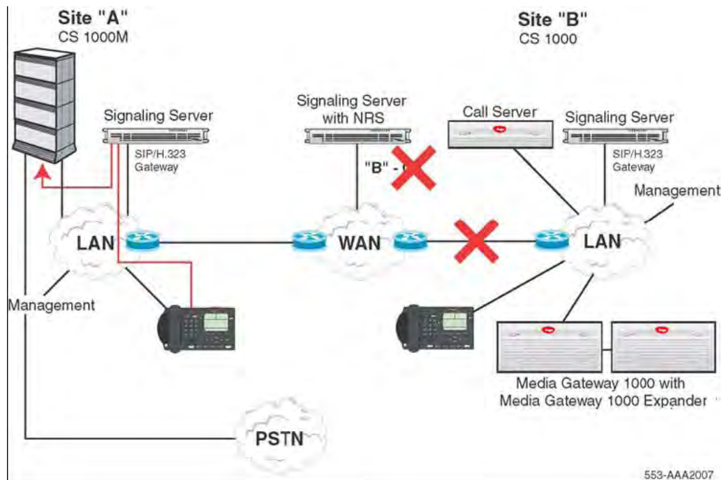
Figure 12: User A dials User B
