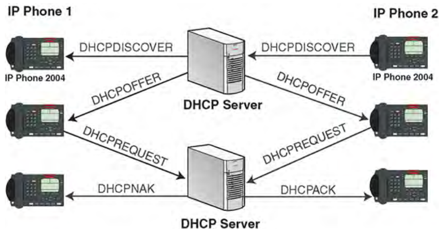
Figure 109: IP acquisition sequence: Case 3
