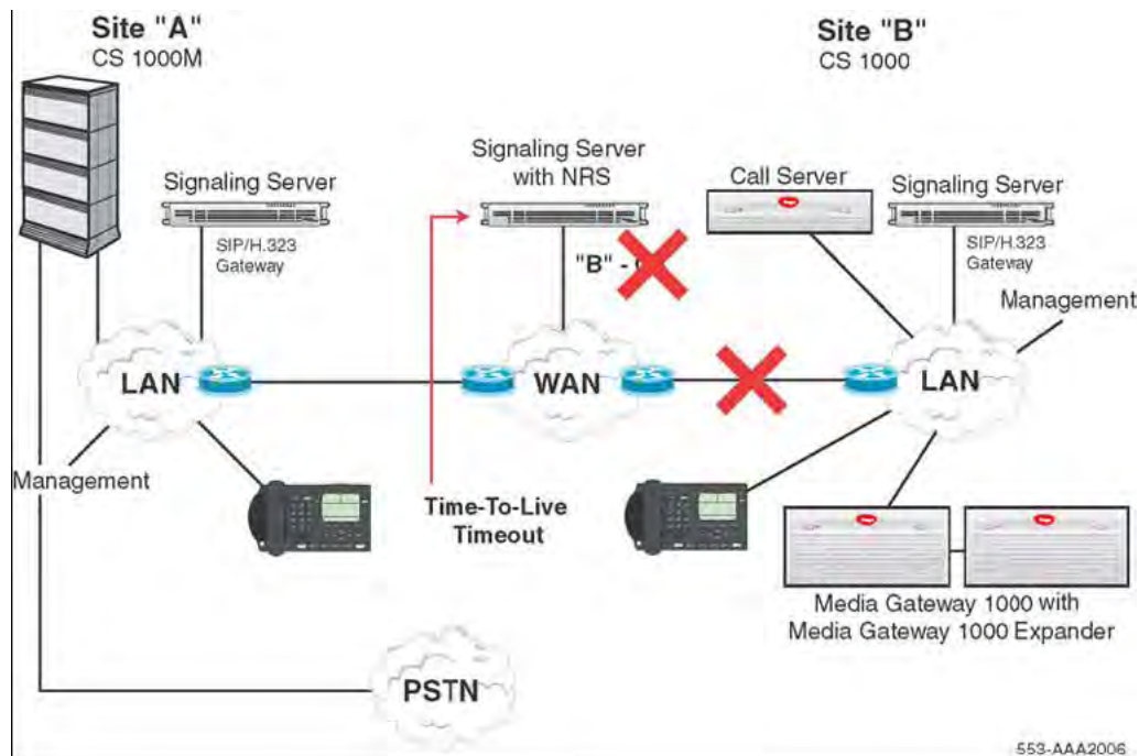
Figure 11: Registration at Site B times out
