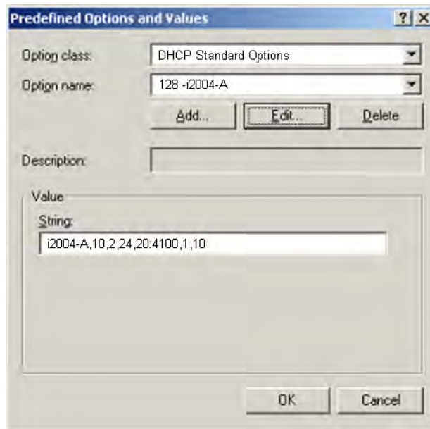
Figure 113: Predefined Options and Values with data entered
