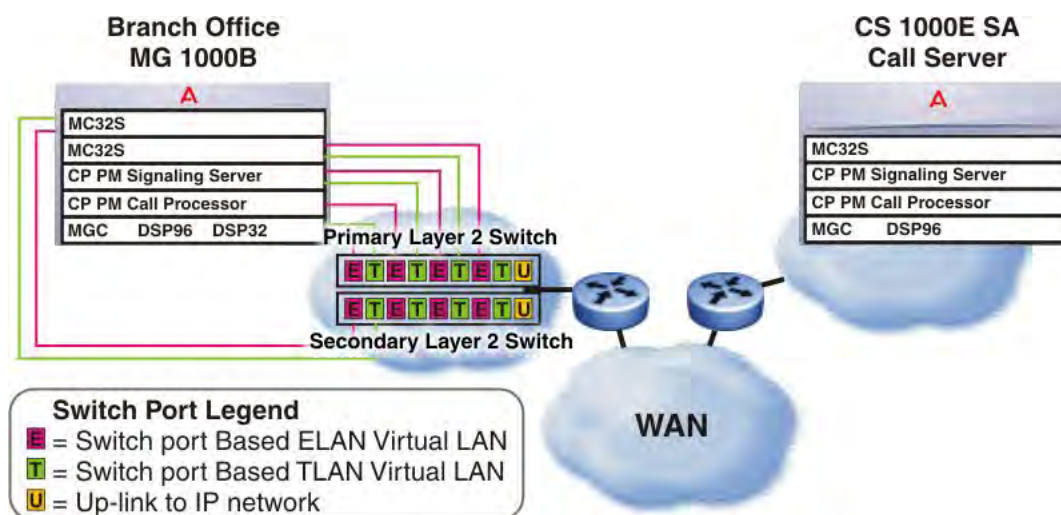
Figure 43: MG 1000B detailed core system connections
