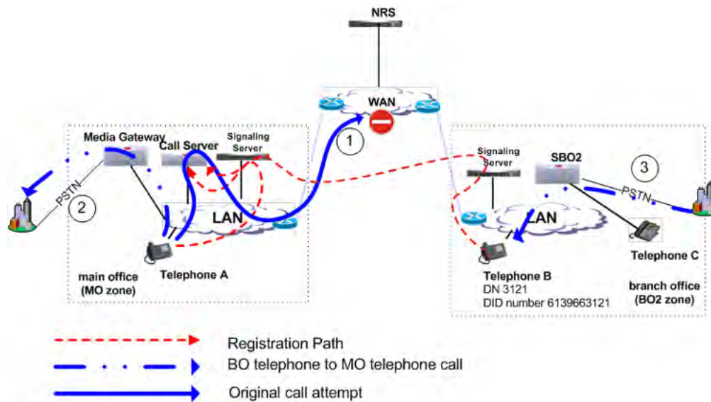
Figure 68: Call from a main to a branch office telephone
