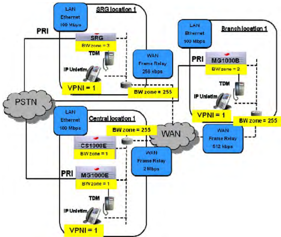
Figure 95: Main Office with MG 1000B and SRG
