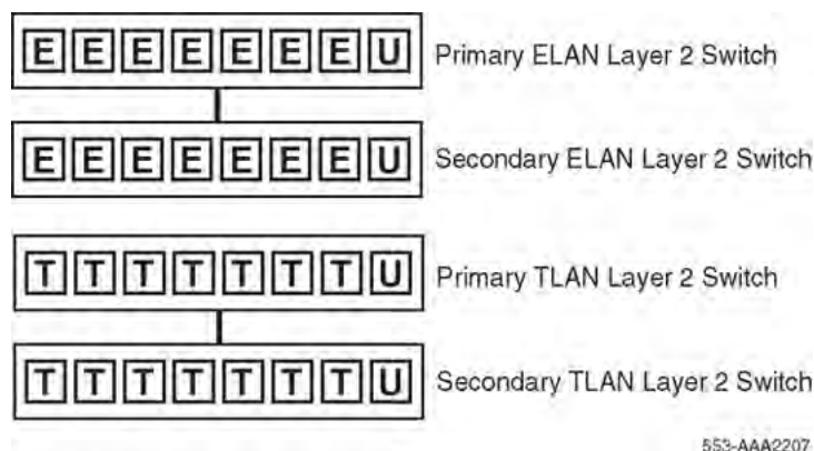
Figure 47: Redundant core network: no VLAN on Layer 2 switch infrastructure
