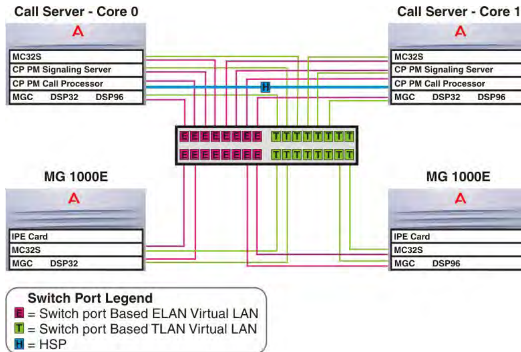
Figure 44: Communication Server 1000E: Physically collocated Side 0 and Side 1
