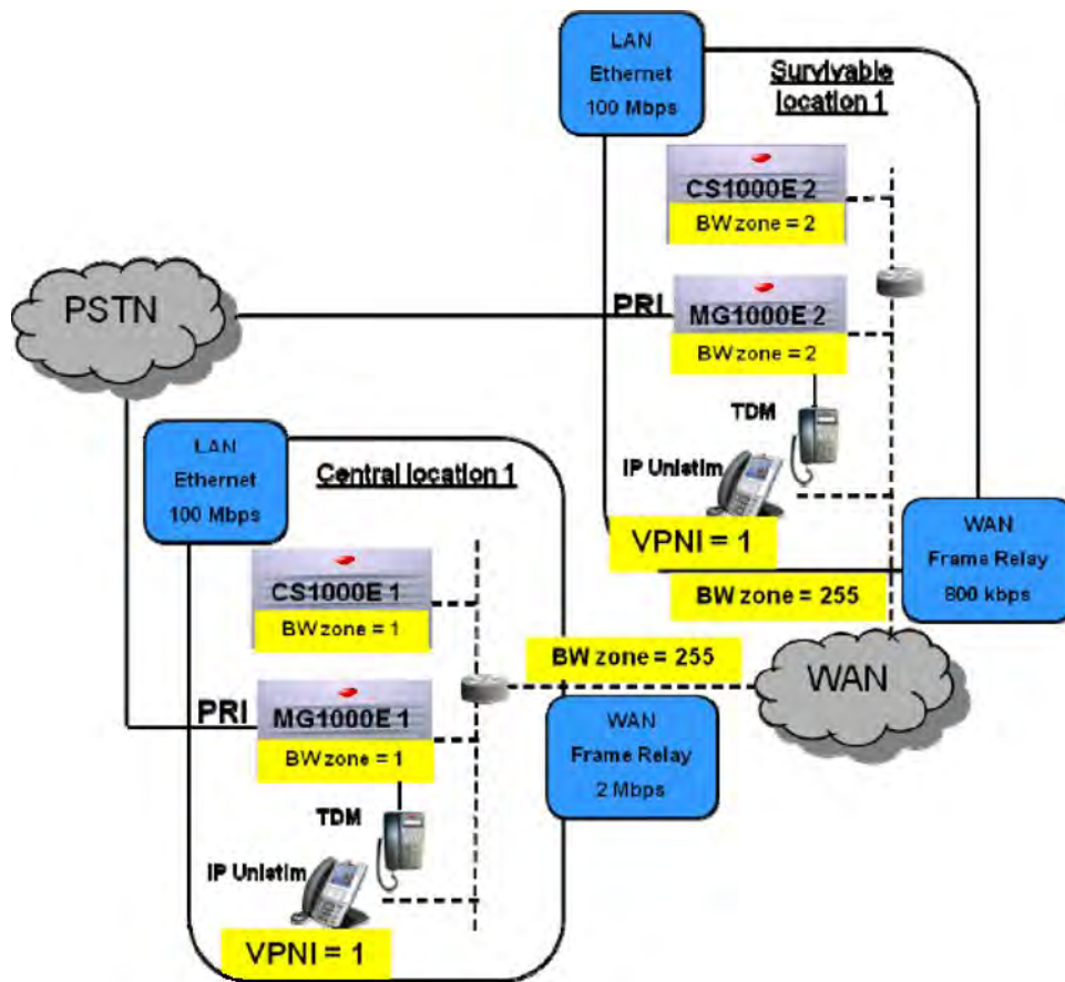
Figure 93: CS 1000 with Survivable Media Gateway
