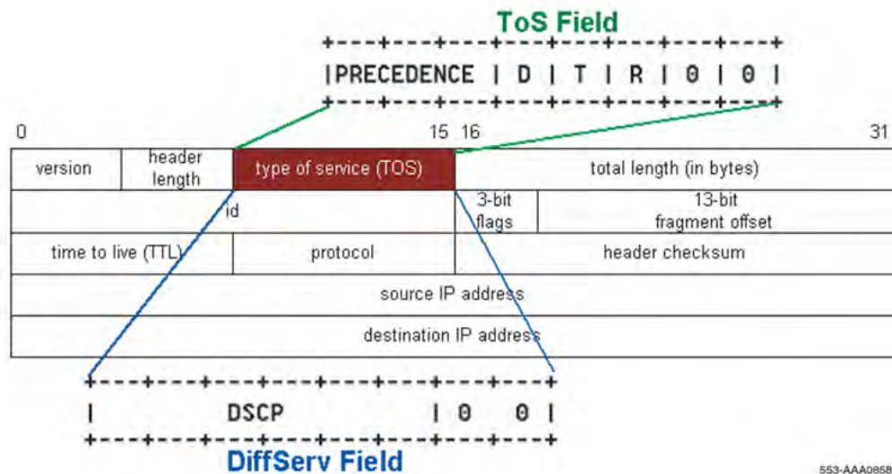
Figure 7: IPv4 header showing DSCP location
