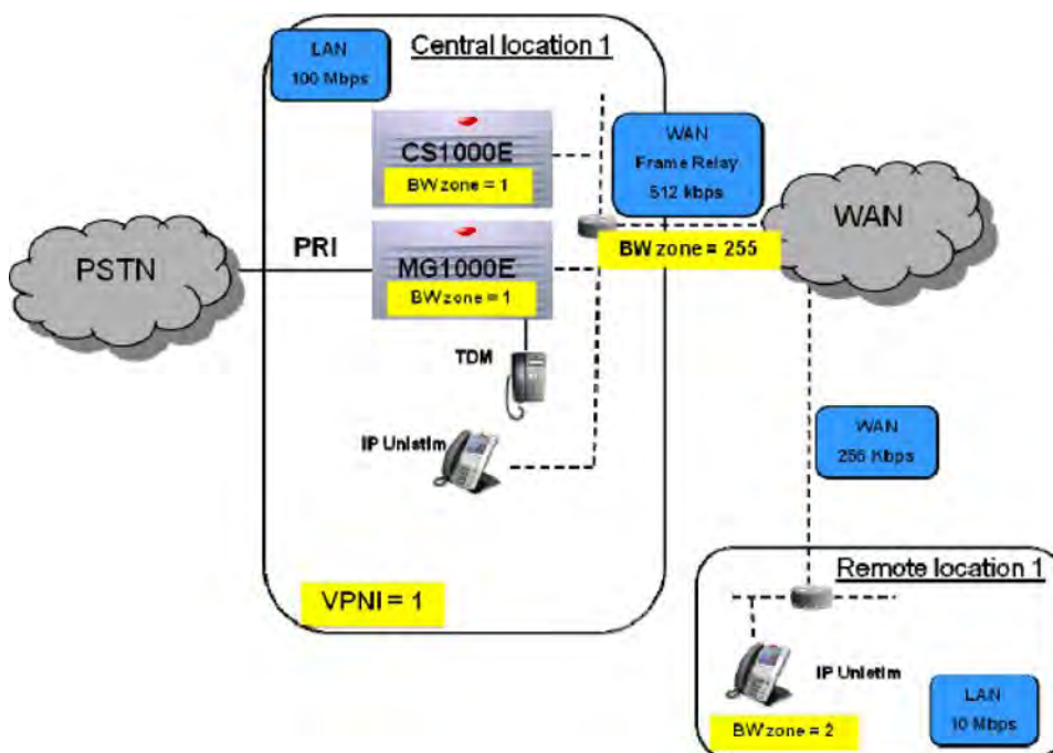
Figure 104: CS 1000 with remote location consisting of IP Phones only
