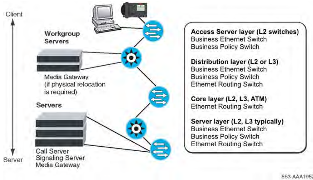
Figure 24: Campus network reference model
