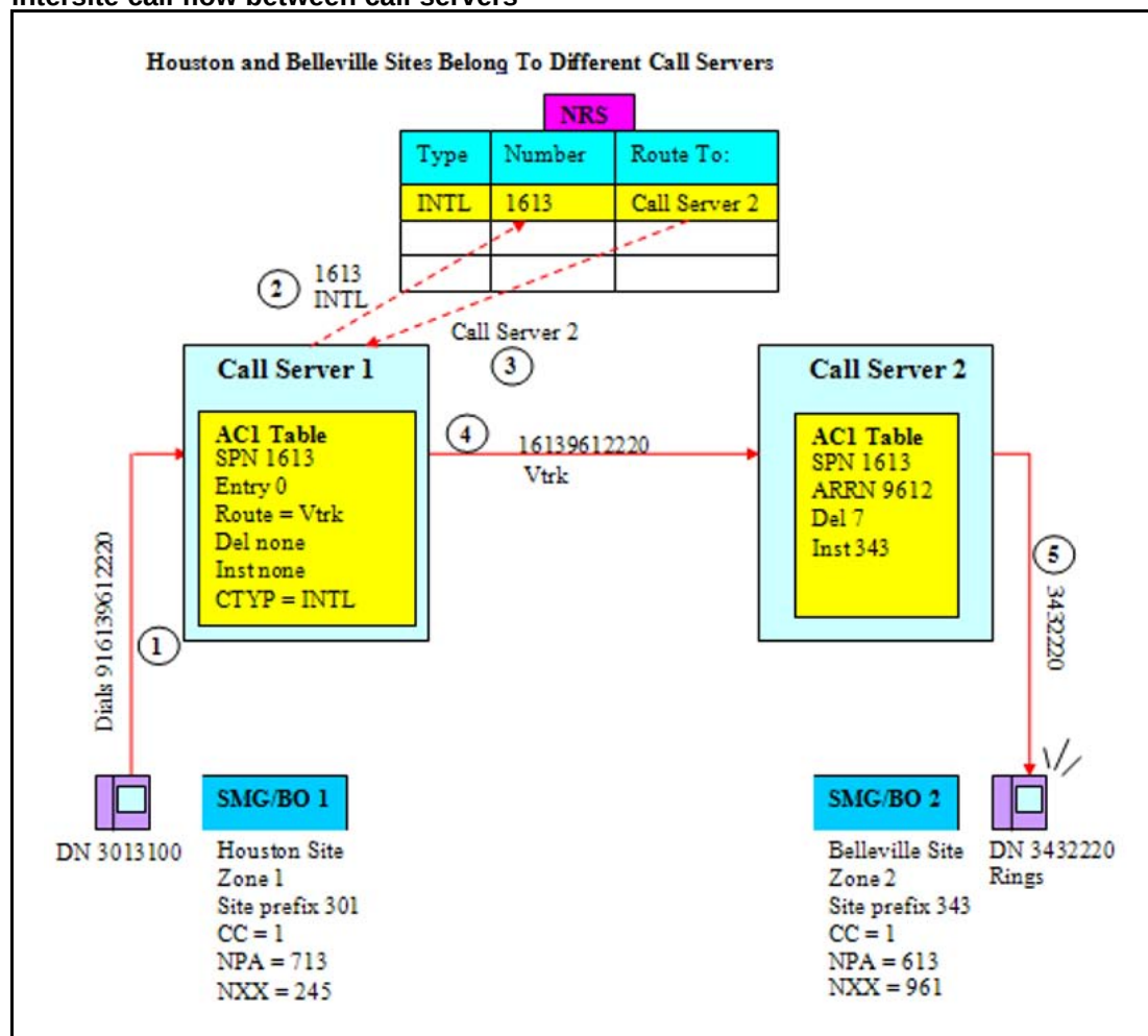
Figure 23 intersite call flow between call servers
