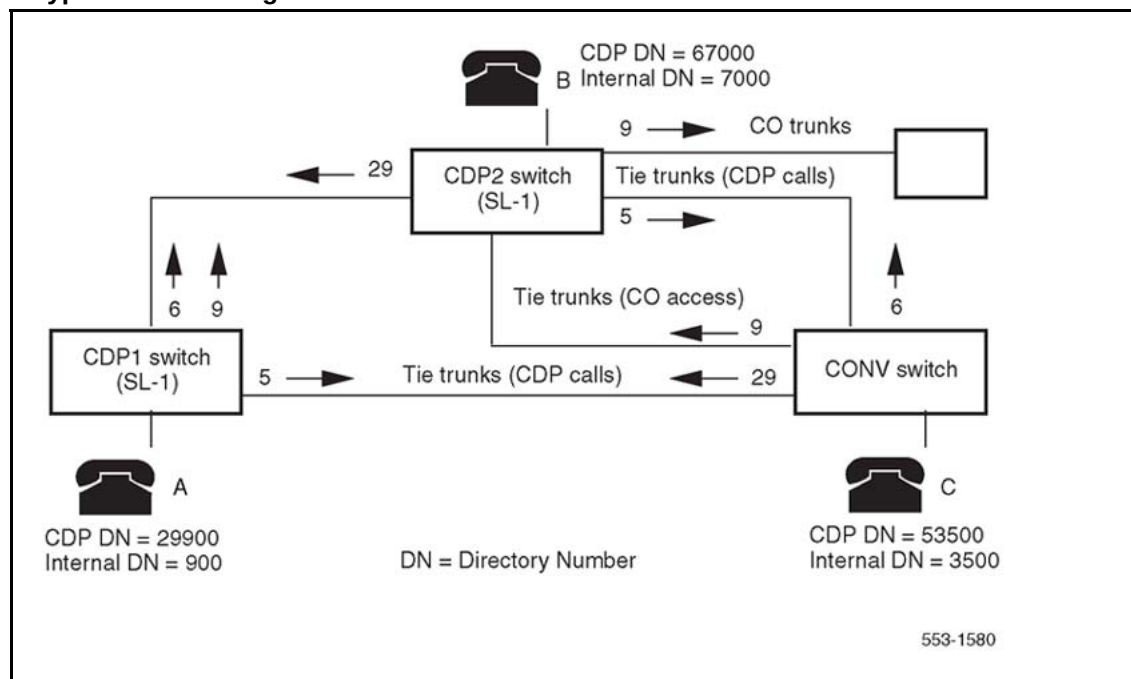
Figure 2 A typical CDP Configuration
