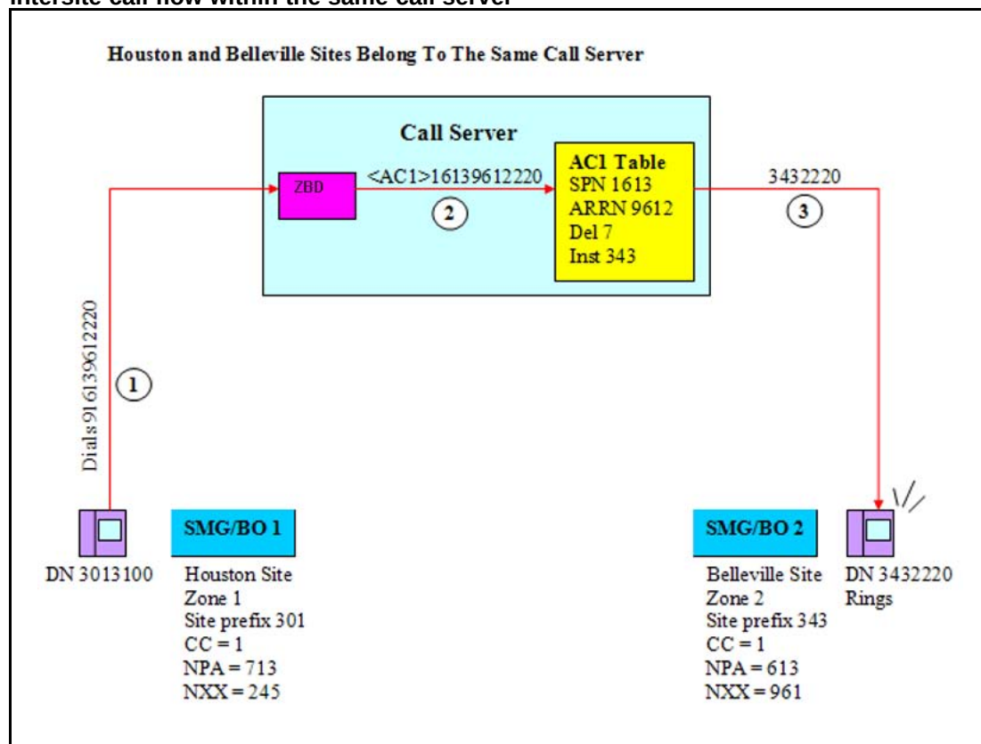
Figure 22 intersite call flow within the same call server
