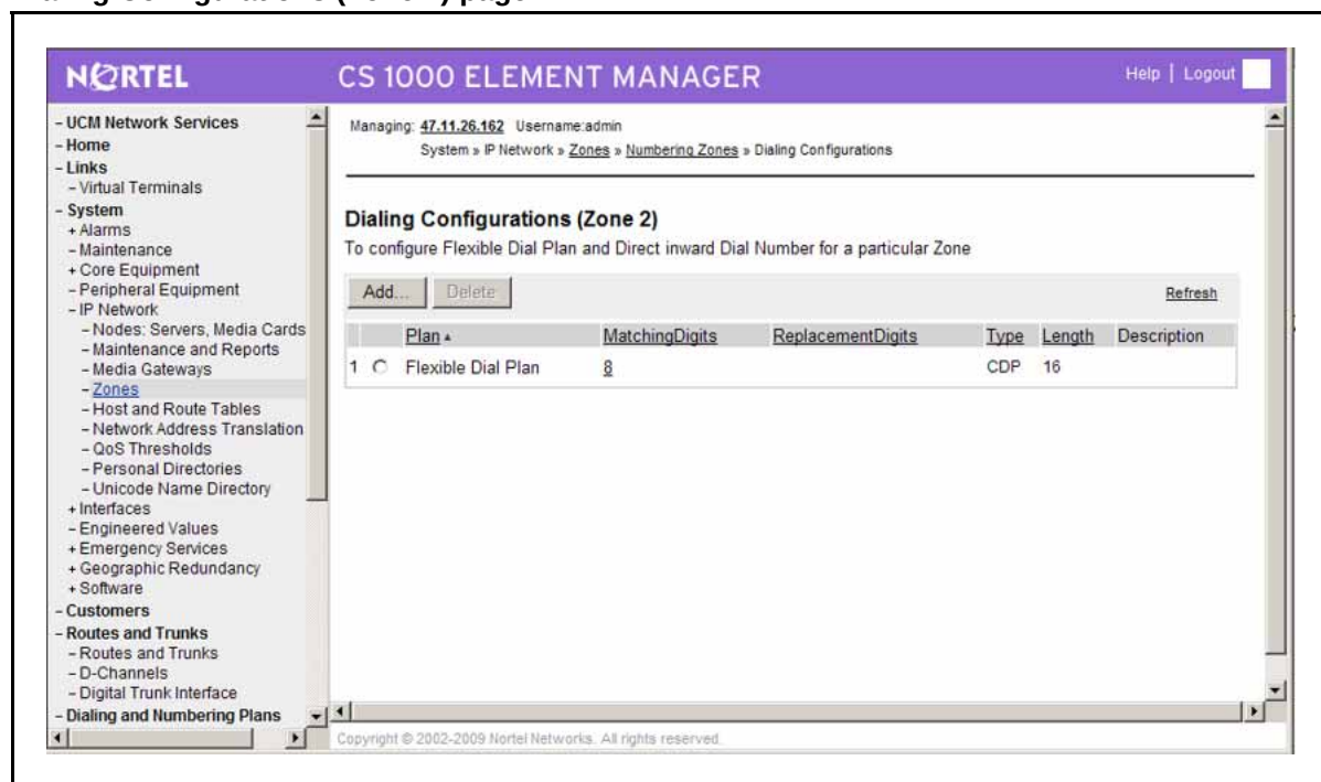
Figure 16 Dialing Configurations (Zone x) page
