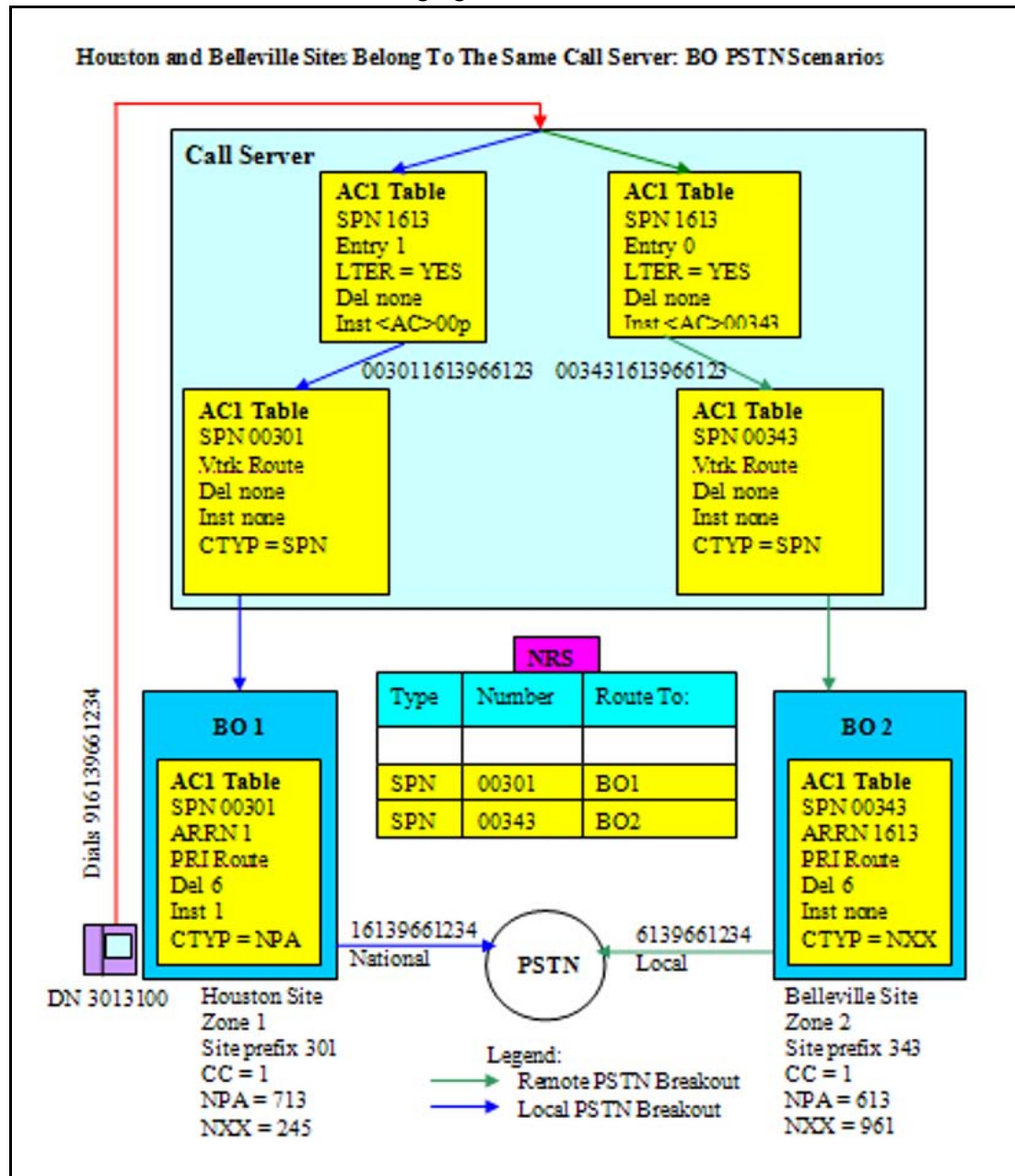
Figure 25 PSTN call flow with BO sites belonging to the same call server
