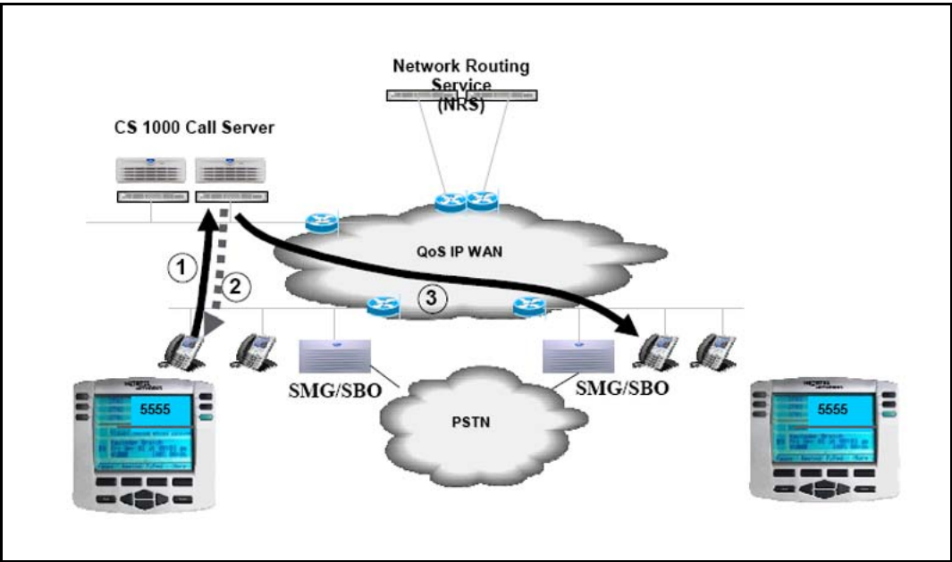
Configuration Example: Call Server: Numbering zone (LD 117)
