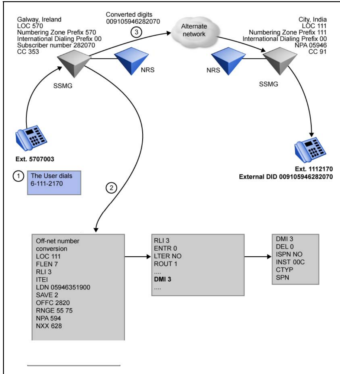
Figure 36 Call flow for Private dialing during WAN outage
