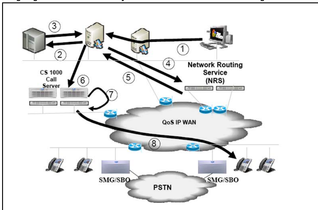
Figure 32 Outgoing OC client SIP Gateway call to On-Net Private number using IP WAN
