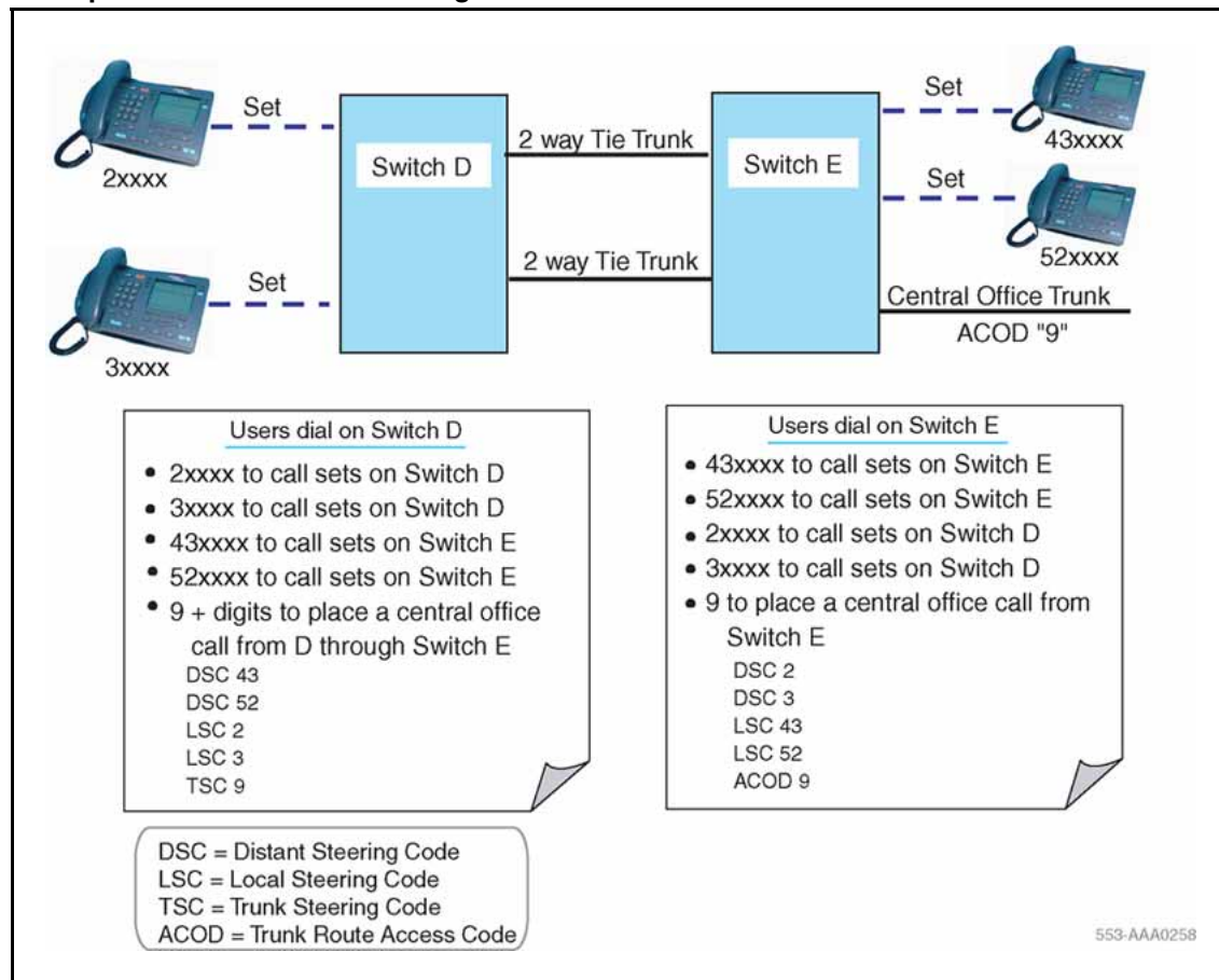
Figure 1 Example of a Coordinated Dialing Plan
