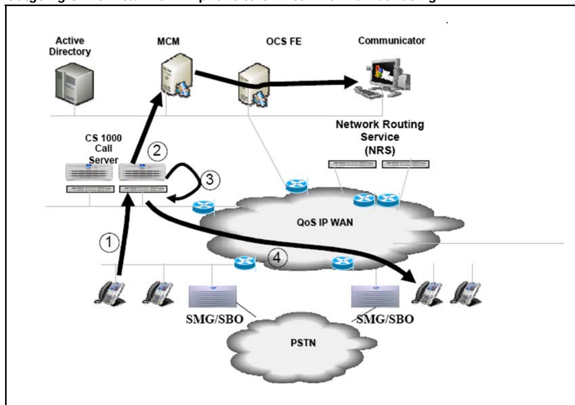
Figure 28 Outgoing SIP CTI call from IP phone to On-net E.164 number using IP WAN
