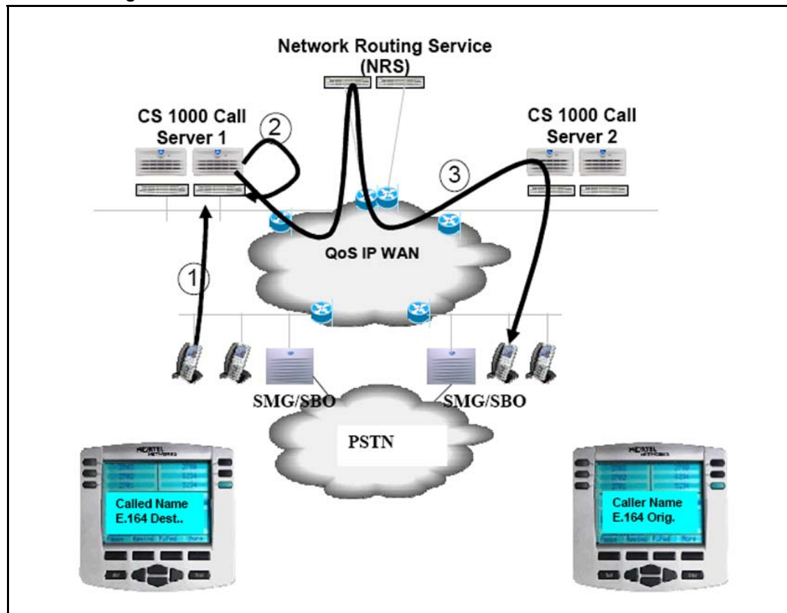
Figure 31 On-Net Dialing with Private Numbers across different Call Servers
