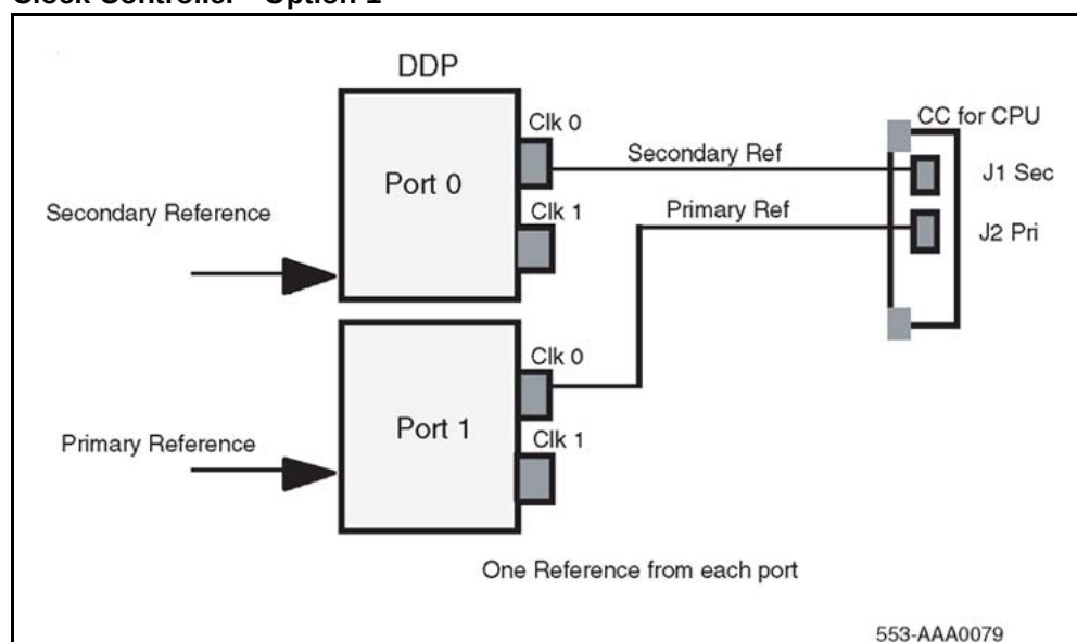
Figure 31 Clock Controller - Option 1
