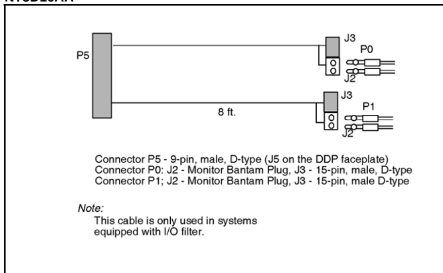
Figure 25 NT5D16AA
