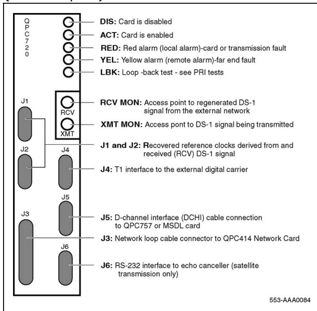
Figure 7 QPC720 PRI faceplate layout
