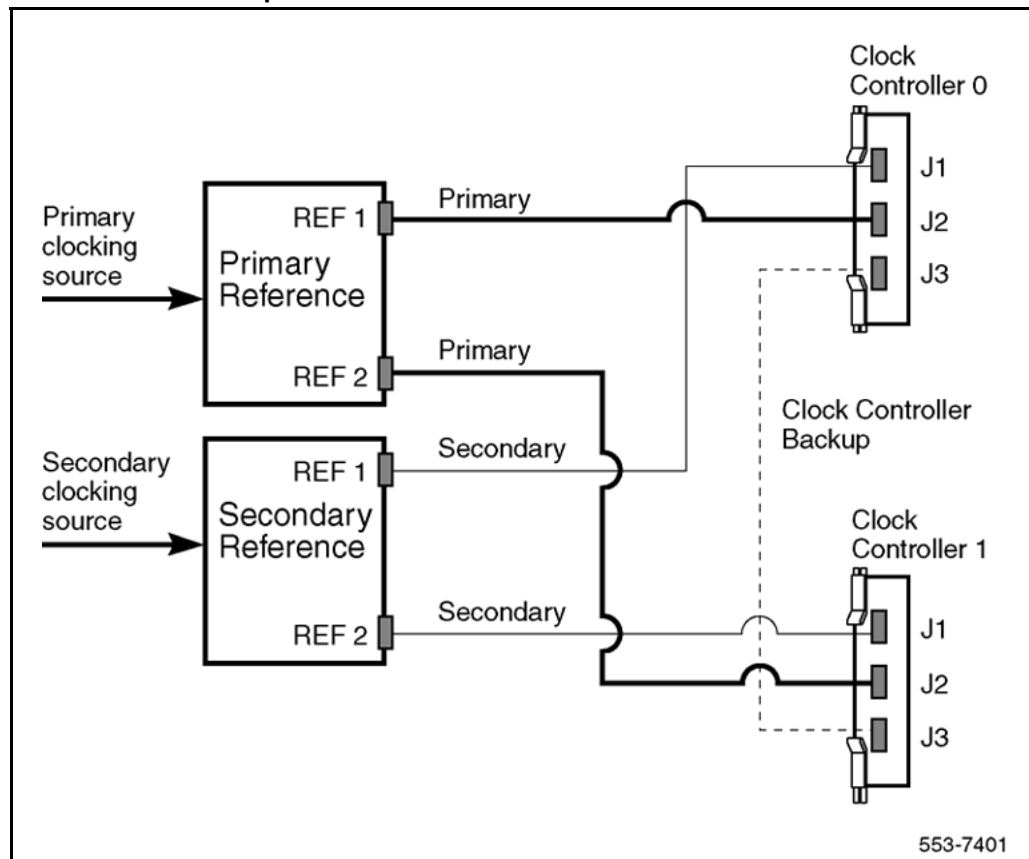
Figure 19 Clock Controller - Option 1
