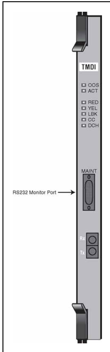
Figure 76 NTRB21 TMDI card faceplate
