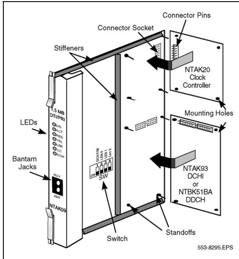
Figure 79 Daughterboard installation on the NTA09
