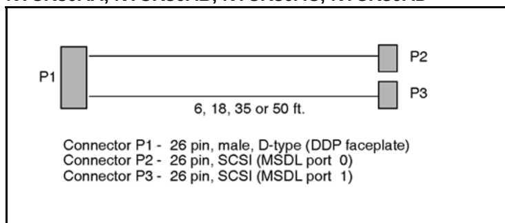
Figure 28 NTCK80AA, NTCK80AB, NTCK80AC, NTCK80AD
