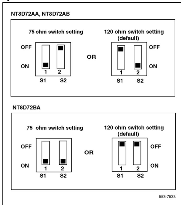
Figure 53 NT8D72AA, NT8D72AB, NT8D72BA PRI DIP switch settings for Large Systems
