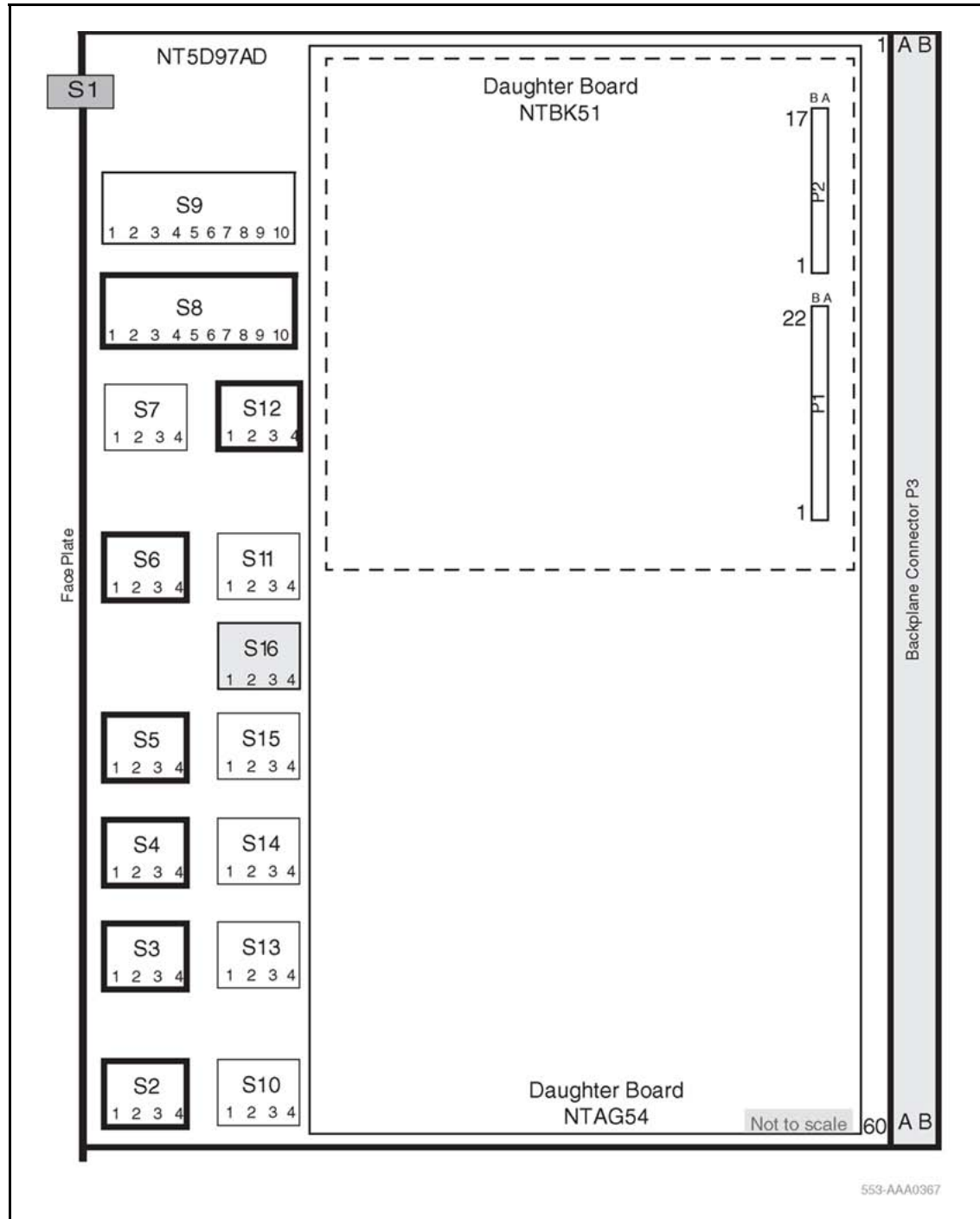
Figure 56 Dip switches locations for NT5D97AD
