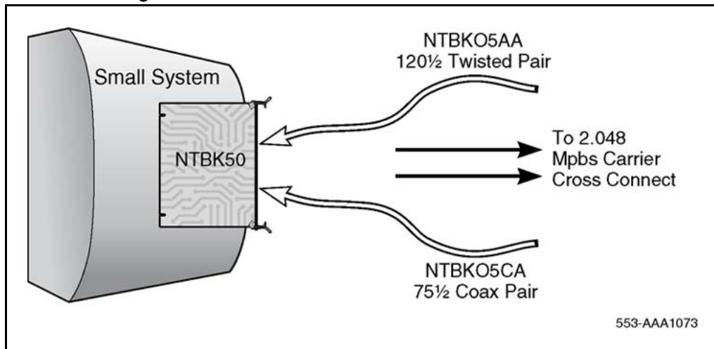
Figure 87 NTBK50 cabling
