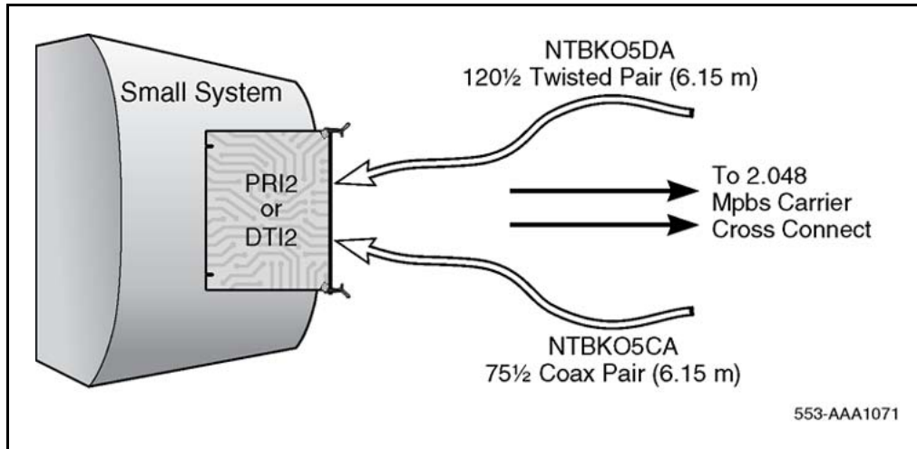
Figure 82 2.0 Mb DTI cabling
