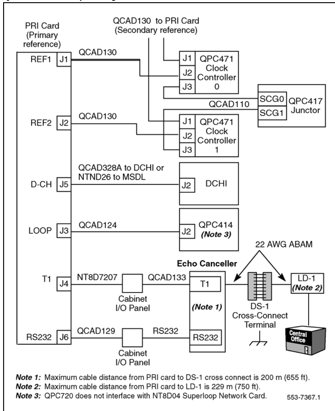
Figure 52 QPC720 Multi Group cabling with an echo canceller
