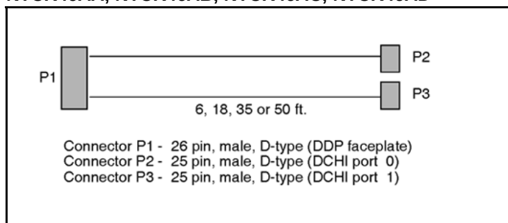
Figure 27 NTCK46AA, NTCK46AB, NTCK46AC, NTCK46AD
