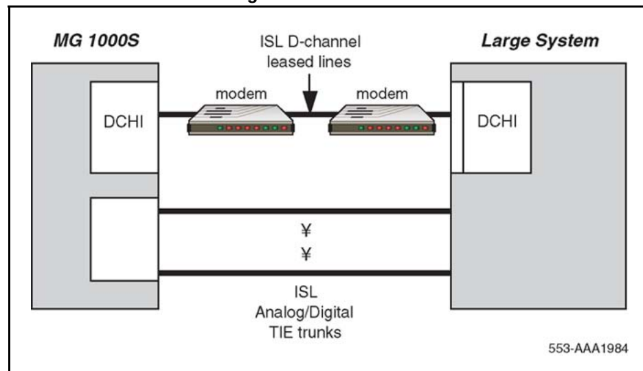
Figure 80 ISL in dedicated mode using leased line
