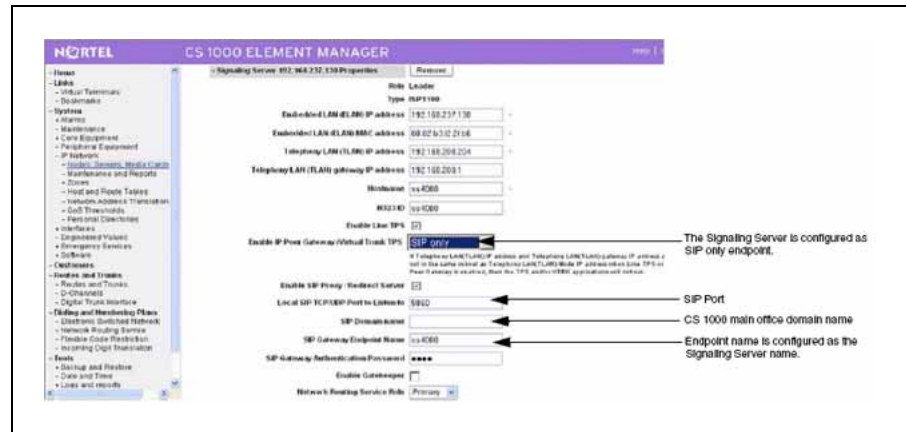
Figure 5 SIP Trunk configuration in Element Manager
