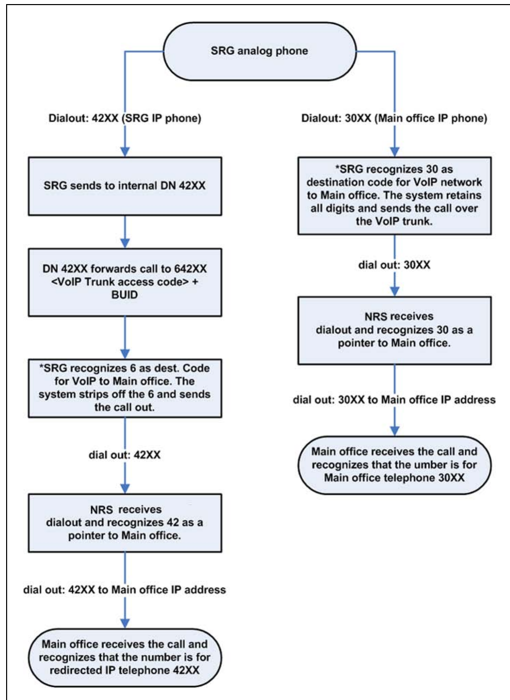
Figure 18 Calls to an SRG IP Phone and a main office IP Phone registered to the main office
