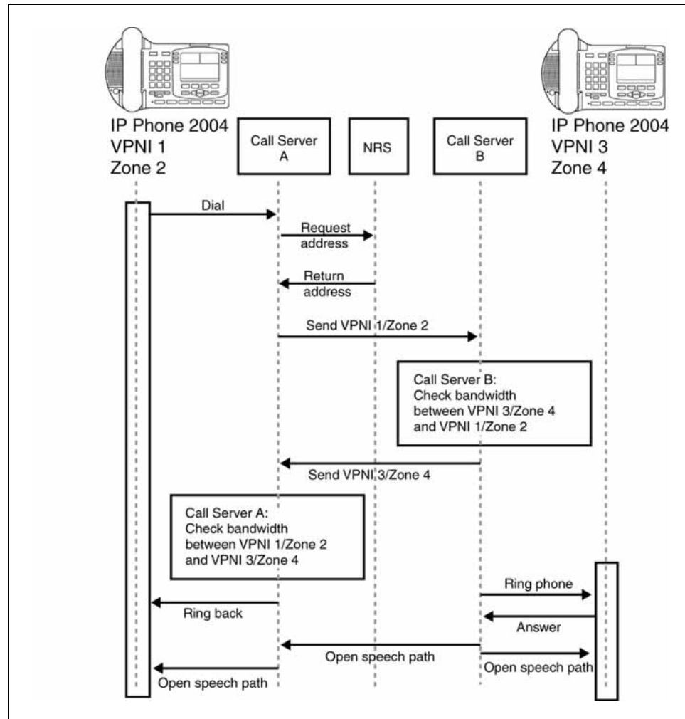
Figure 34 Call Progress with Adaptive Network Bandwidth Management
