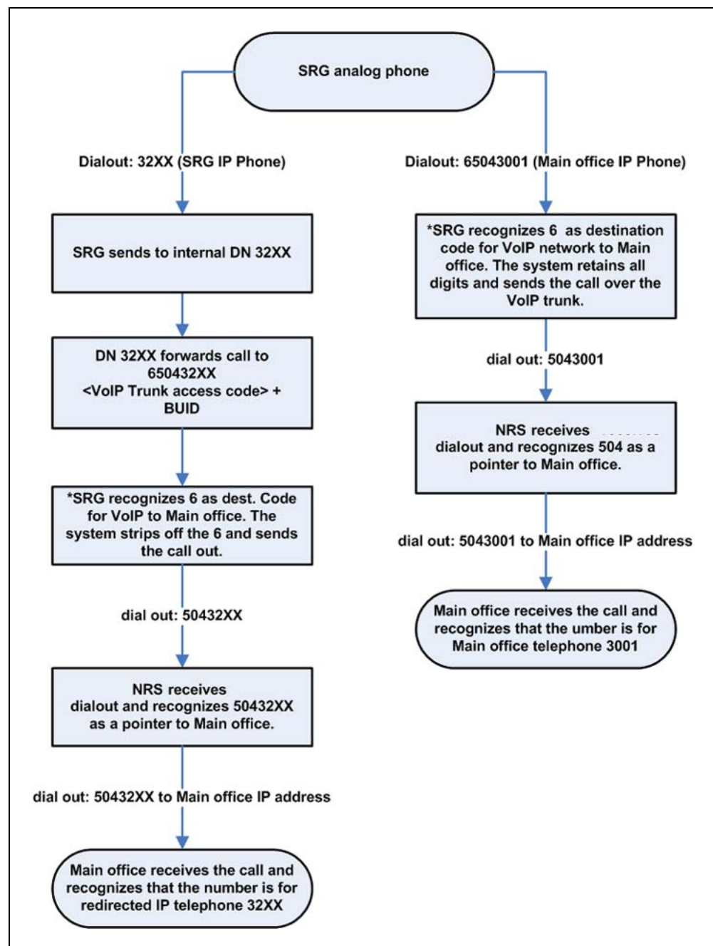
Figure 27 SRG analog phone calls an SRG IP Phone and a main office IP Phone registered to the main office
