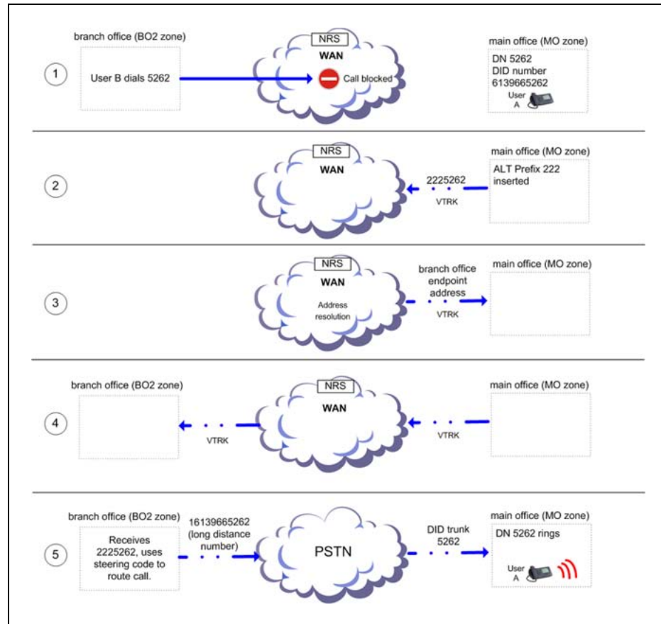
Figure 67 Digits dialed and outpulsed with Alternative Call Routing for NBWM
