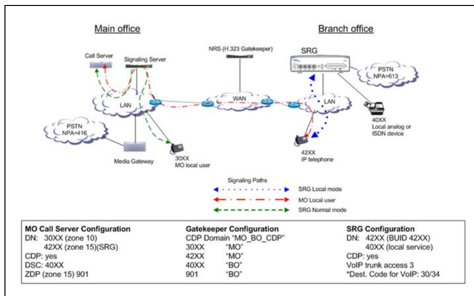
Figure 17 CDP Option 1
