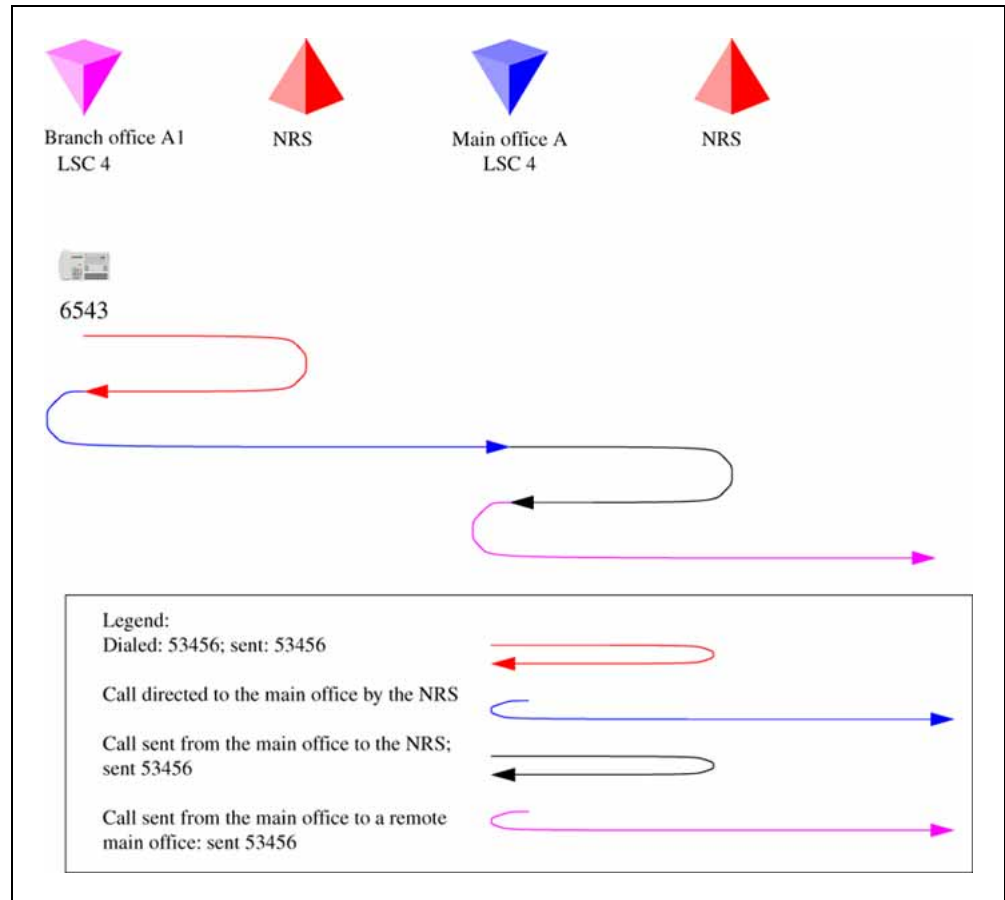
Figure 52 Call to remote branch office on the originator side
