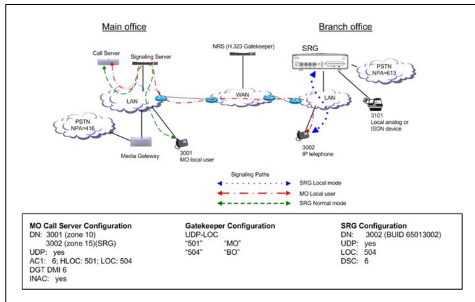
Figure 25 UDP using location codes
