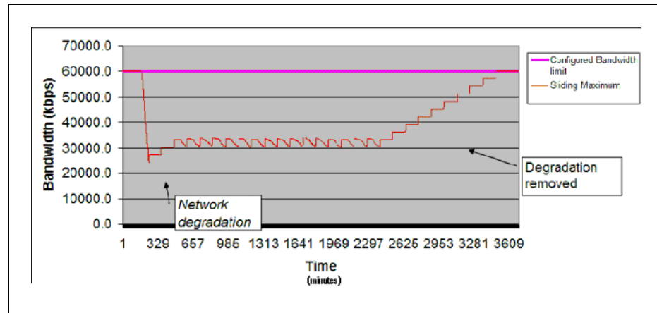
Figure 35 Adaptive Network Bandwidth Management graph
