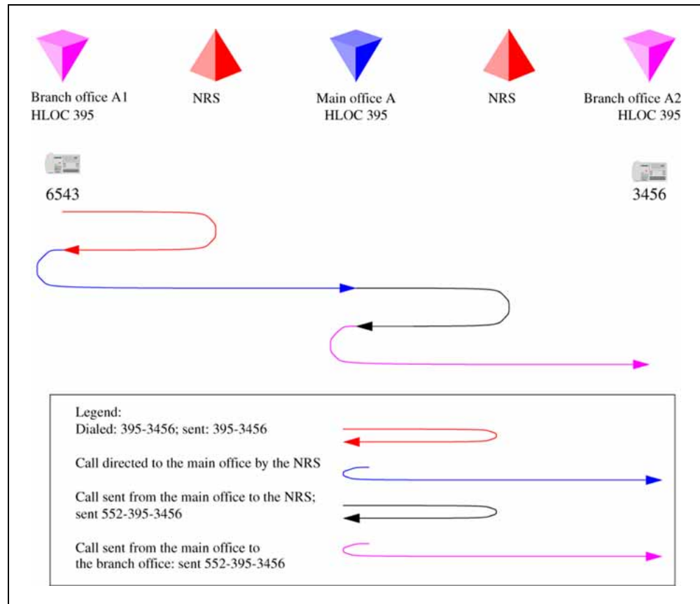
Figure 60 Call to remote branch office on the destination side
