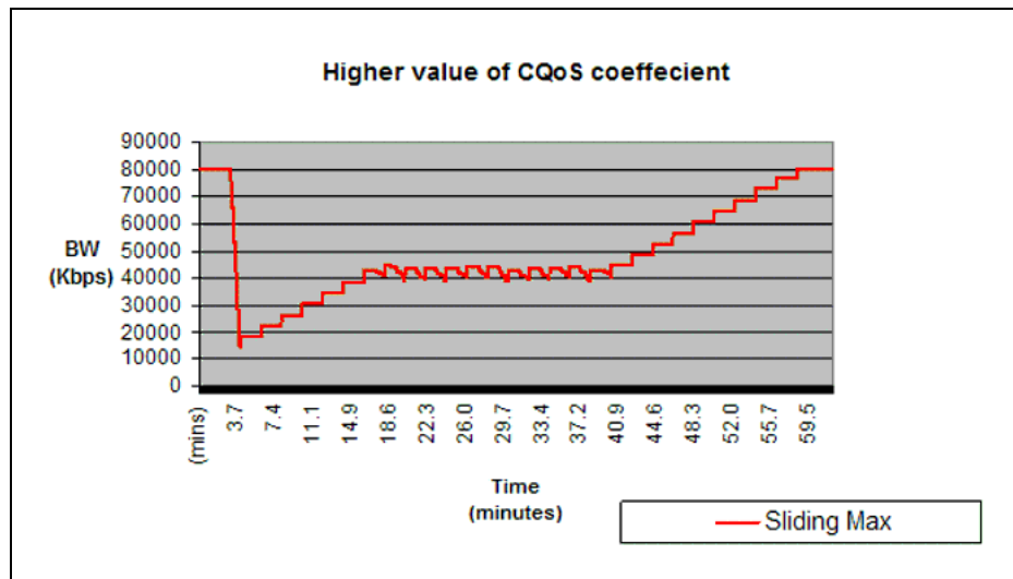
Figure 37 Effect of a higher CQoS Coefficient
