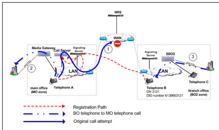
Figure 68 Call between a main office telephone and a branch office telephone
