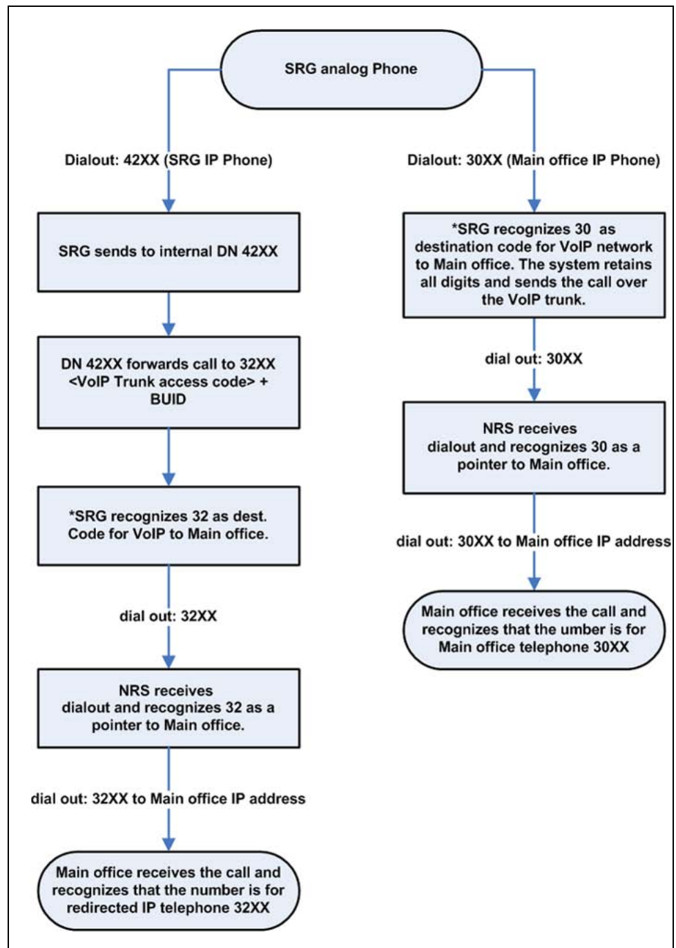
Figure 24 SRG analog phone calls an SRG IP Phone and a main office IP Phone registered to the main office
