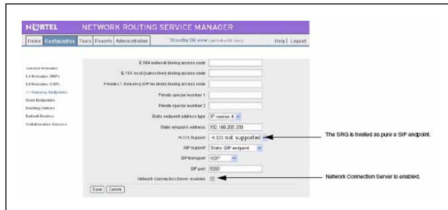
Figure 6 SIP Trunk configuration in NRS
