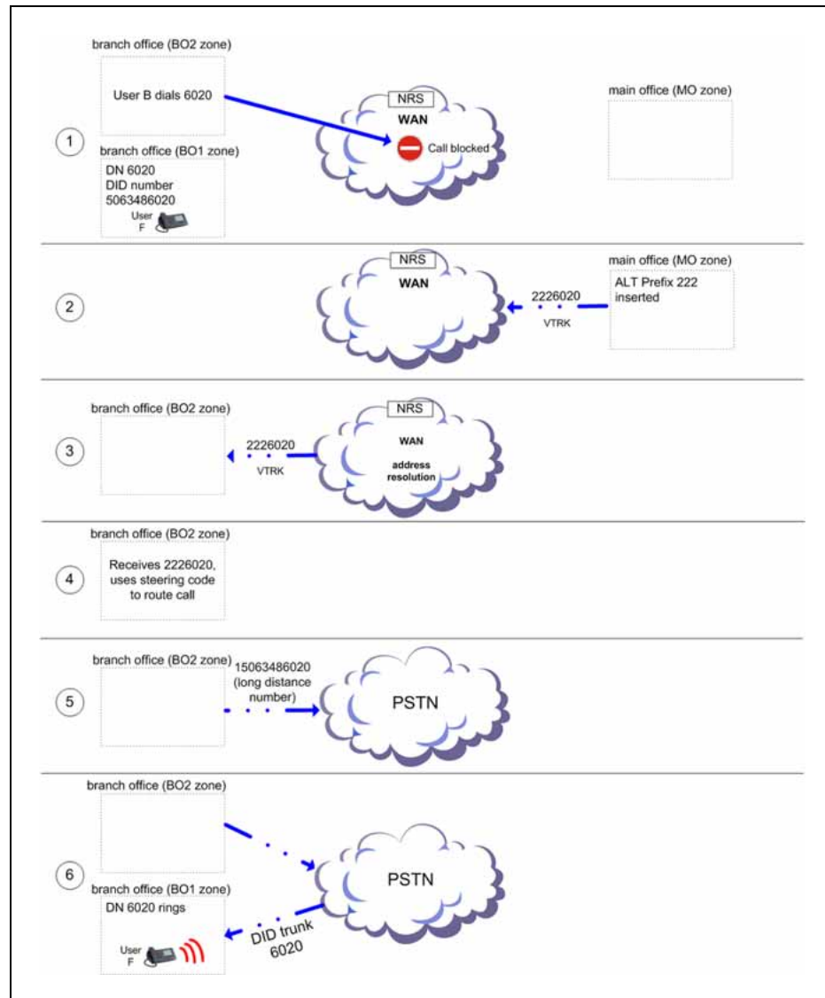
Figure 71 Digits dialed and outpulsed with Alternative Call Routing for NBWM
