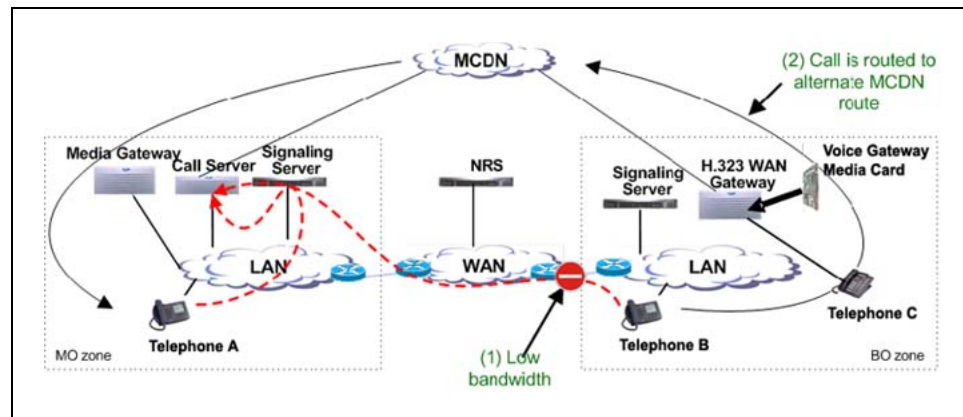
Figure 65 Example of Alternative Call Routing for NBWM in operation
