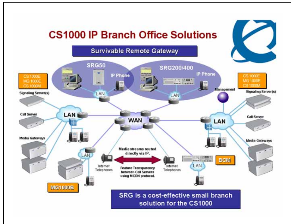
Figure 1 SRG network
