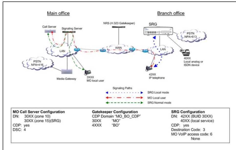
Figure 23 CDP Option 3
