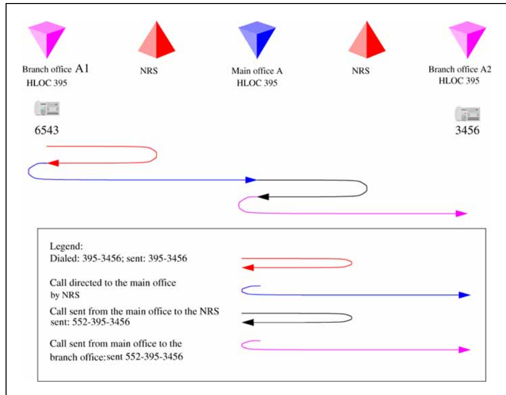
Figure 45 Call flow for Scenario 1 - local call
