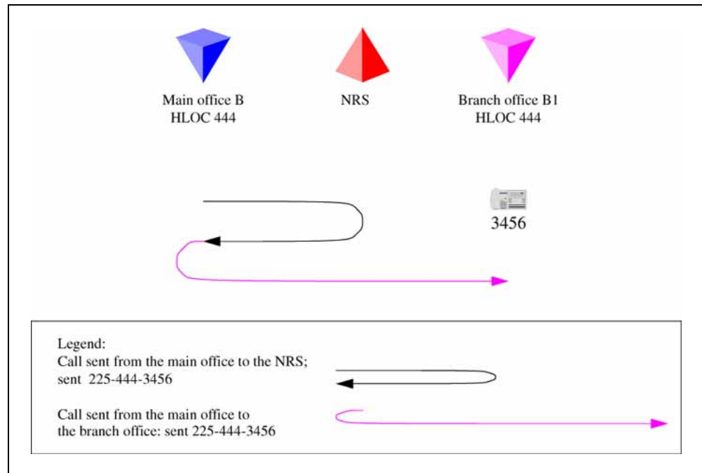
Figure 49 Call to remote branch office on the destination side
