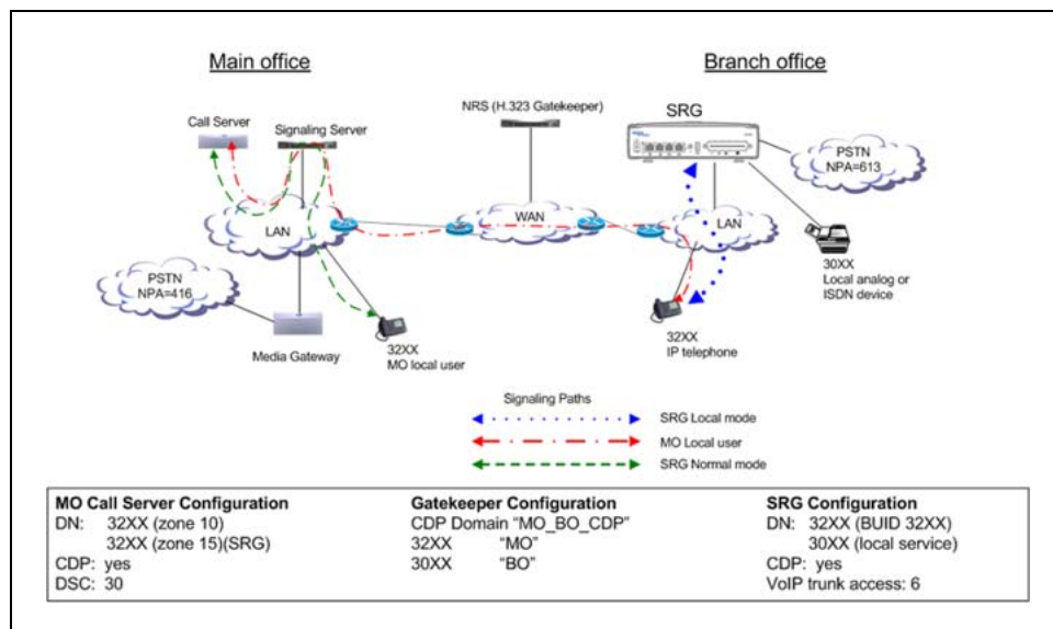
Figure 20 CDP Option 2
