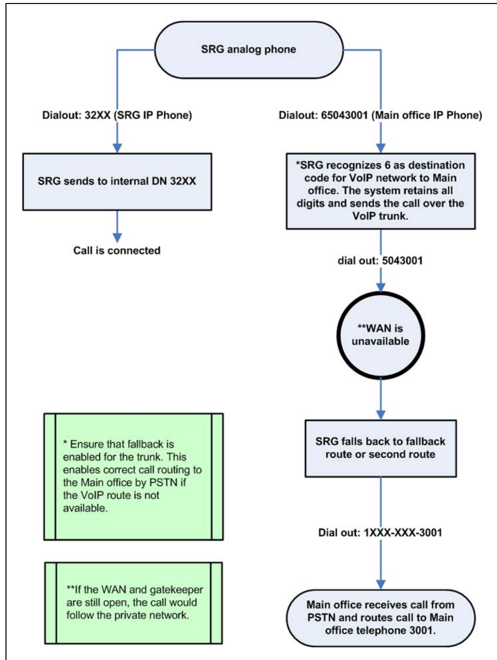
Figure 28 SRG analog phone calls an IP Phone and a main office IP Phone registered to the SRG
