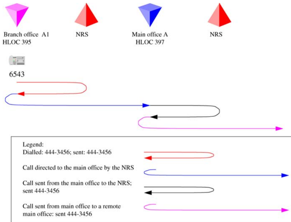
Figure 42: Provisioning example
