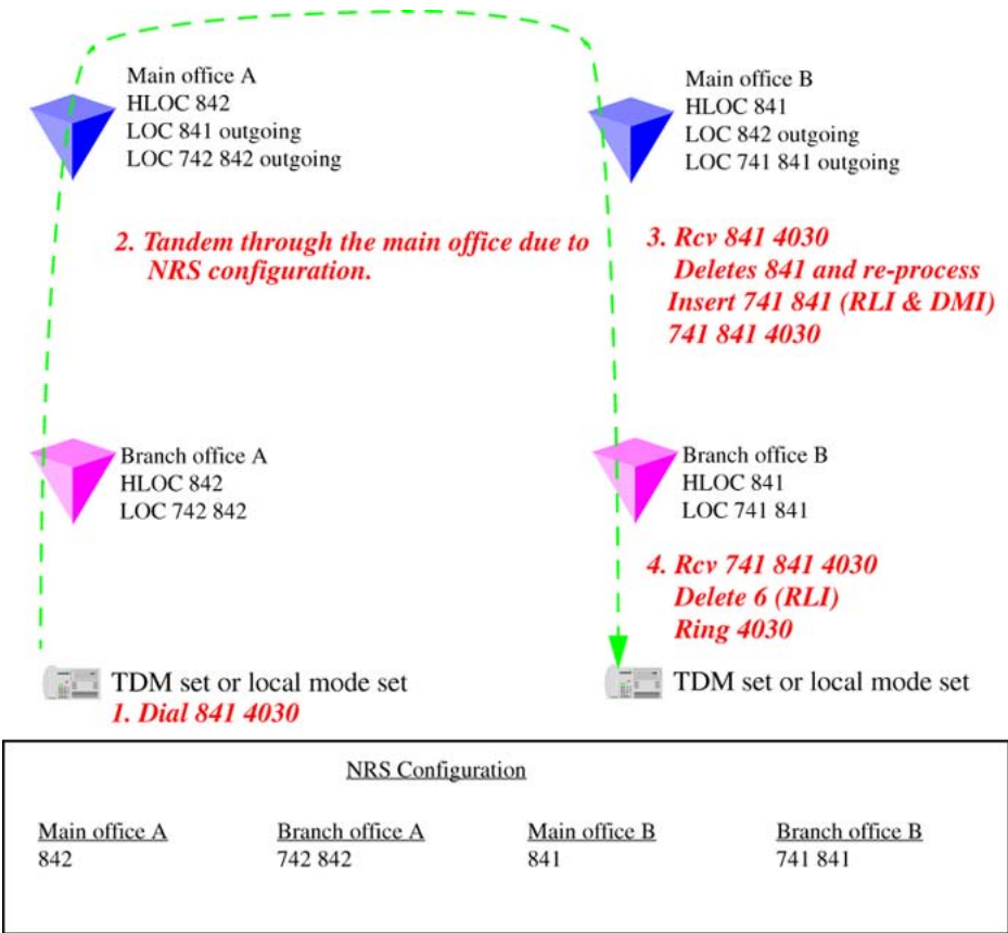
Figure 44: UDP between main offices and CDP inside the main office region
