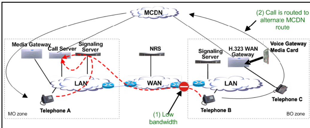
Figure 62 Example of Alternative Call Routing for NBWM in operation
