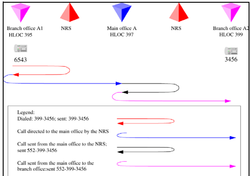
Figure 44 Call flow for Scenario 1- local call
