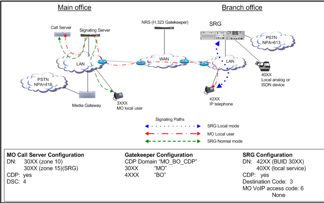
Figure 20 CDP Option 3: DNs of SRG IP Phone and DNs in the main office overlap in Normal Mode but are unique in Local Mode
