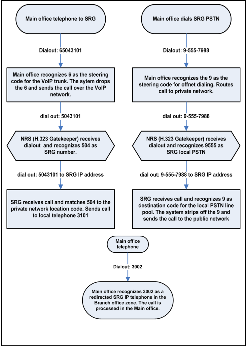
Figure 23 Calling from the main office to the SRG and SRG PSTN, in Normal Mode
