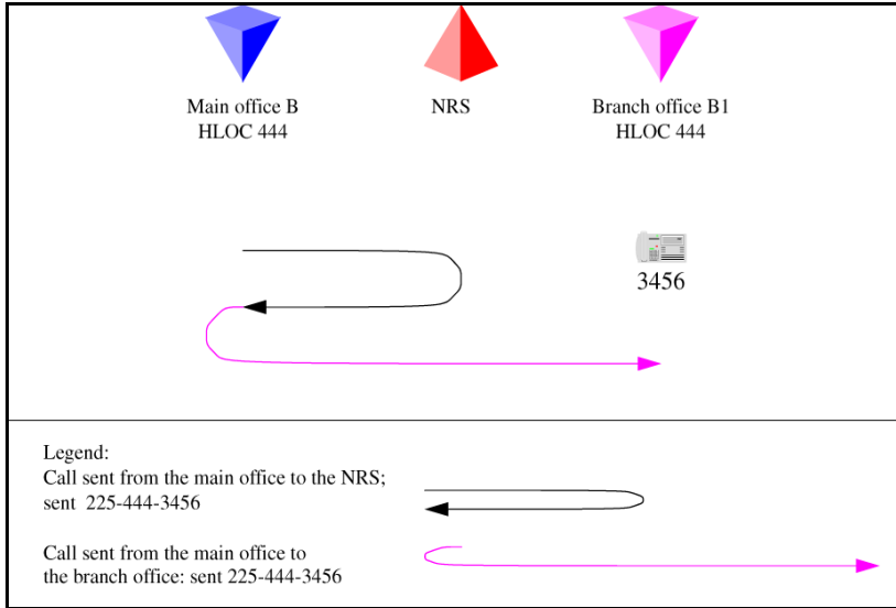
Figure 46 Call flow for Scenario 1 - call to remote branch office (destination side)
