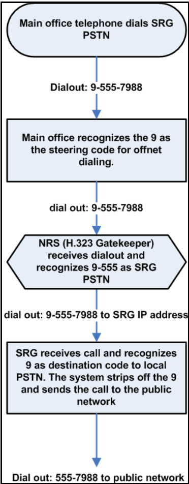
Figure 11 Normal Mode: Main office telephone makes a call over the PSTN through the SRG
