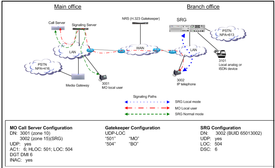
Figure 22 UDP using location codes
