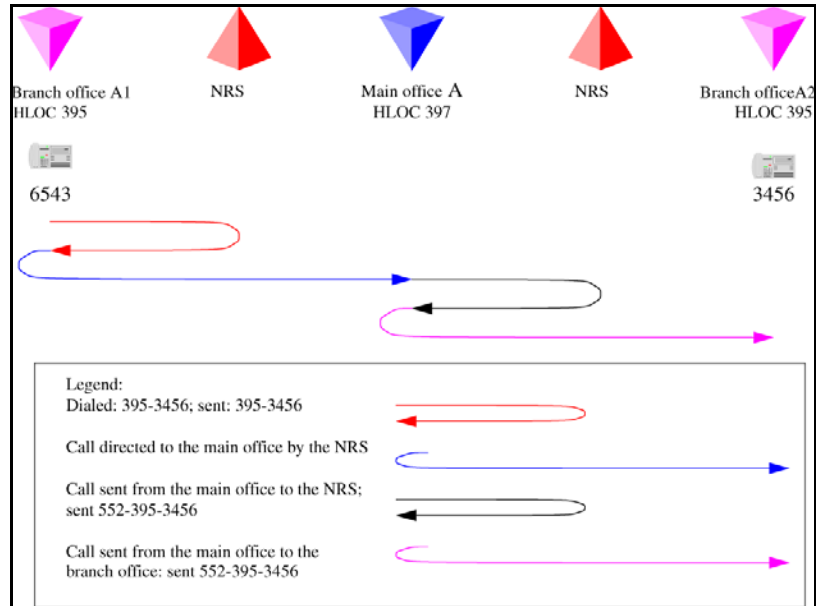
Figure 43 Call flow for Scenario 1 - local call
