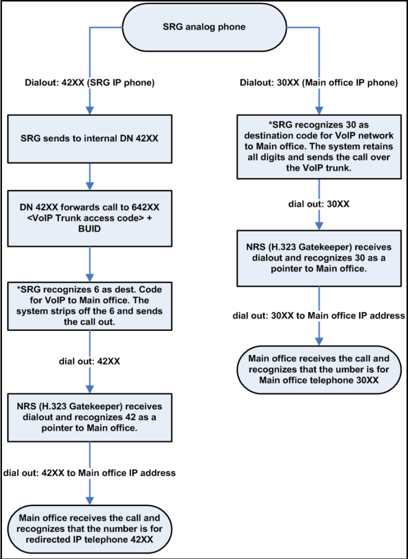
Figure 15 WAN is up. SRG analog phone calls an SRG IP Phone and a main office IP Phone registered to the main office (Normal Mode)
