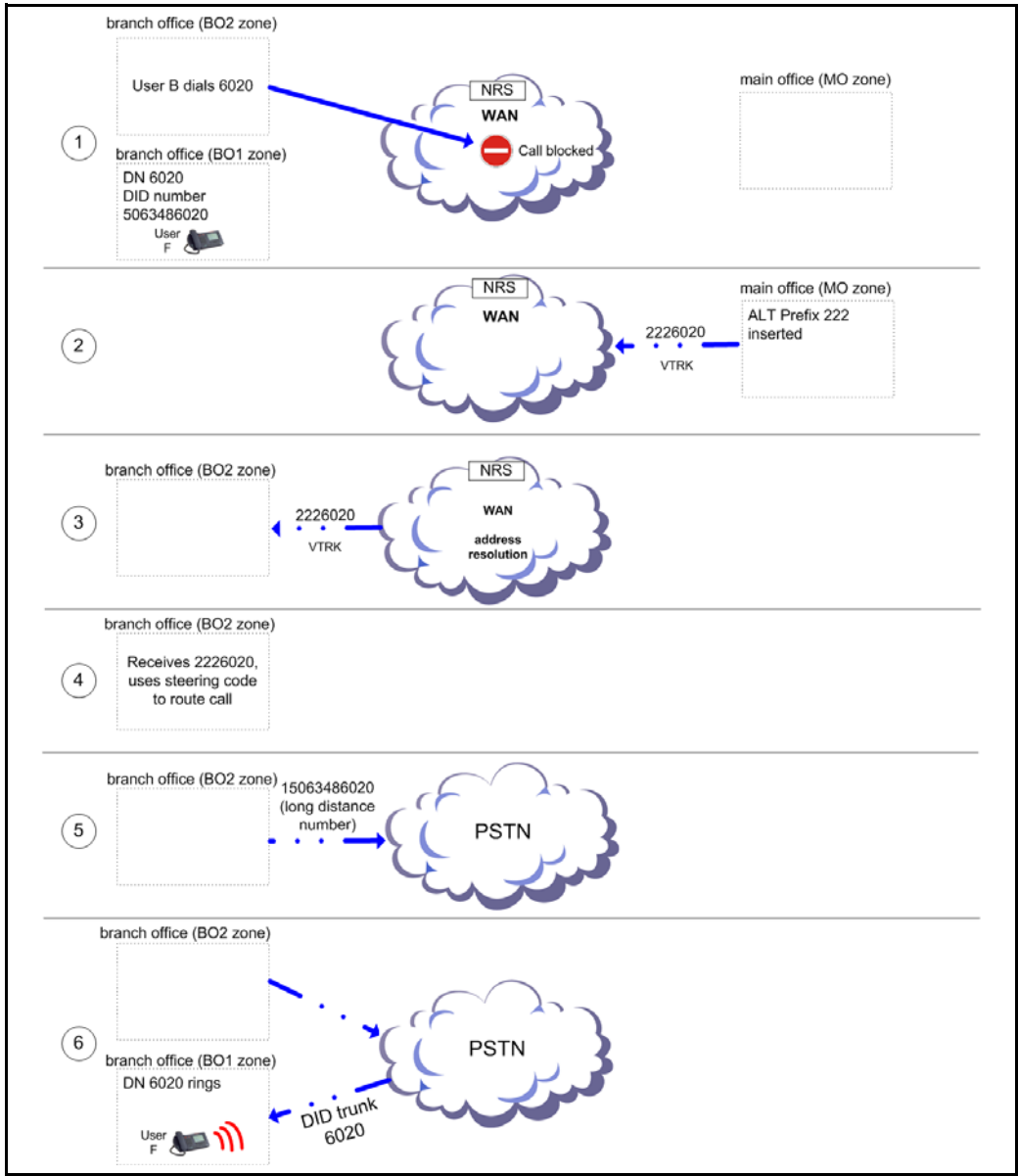
Figure 68 Illustration showing digits dialed and outpulsed with Alternative Call Routing for NBWM
