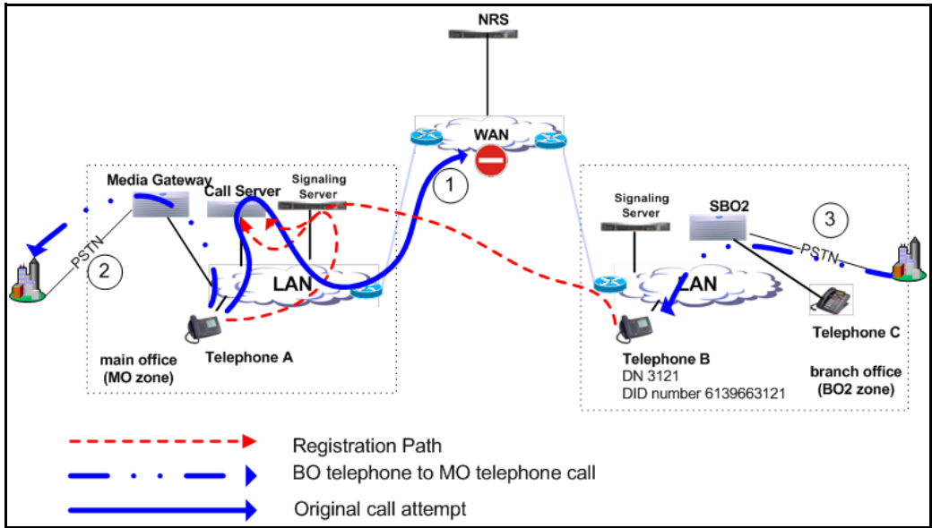
Figure 65 Example of an alternately routed call between a main office telephone and a branch office telephone
