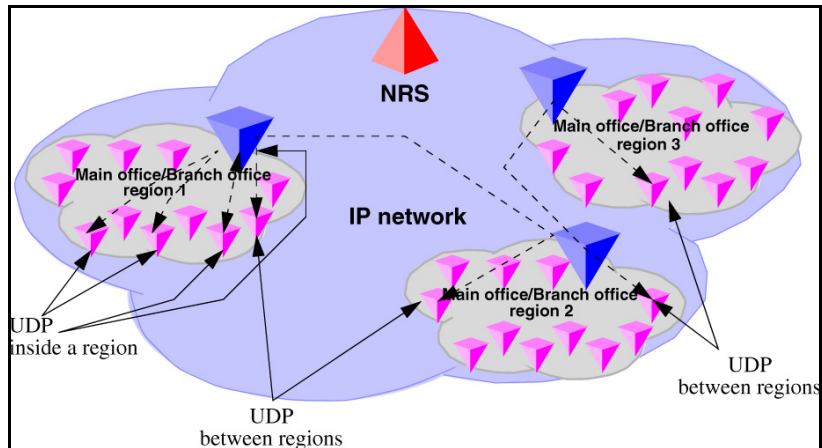
Figure 41 Scenario 1: UDP throughout the network
