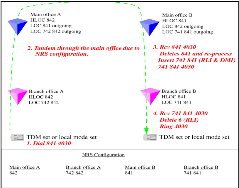
Figure 53 Scenario 2 - UDP between main offices, CDP inside the main office region
