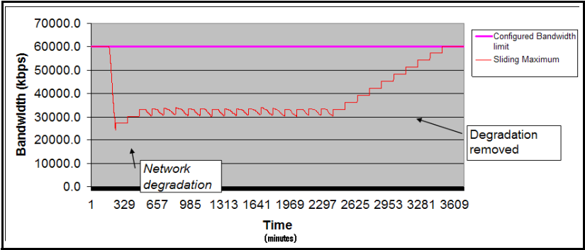
Figure 32 Adaptive Network Bandwidth Management graph
