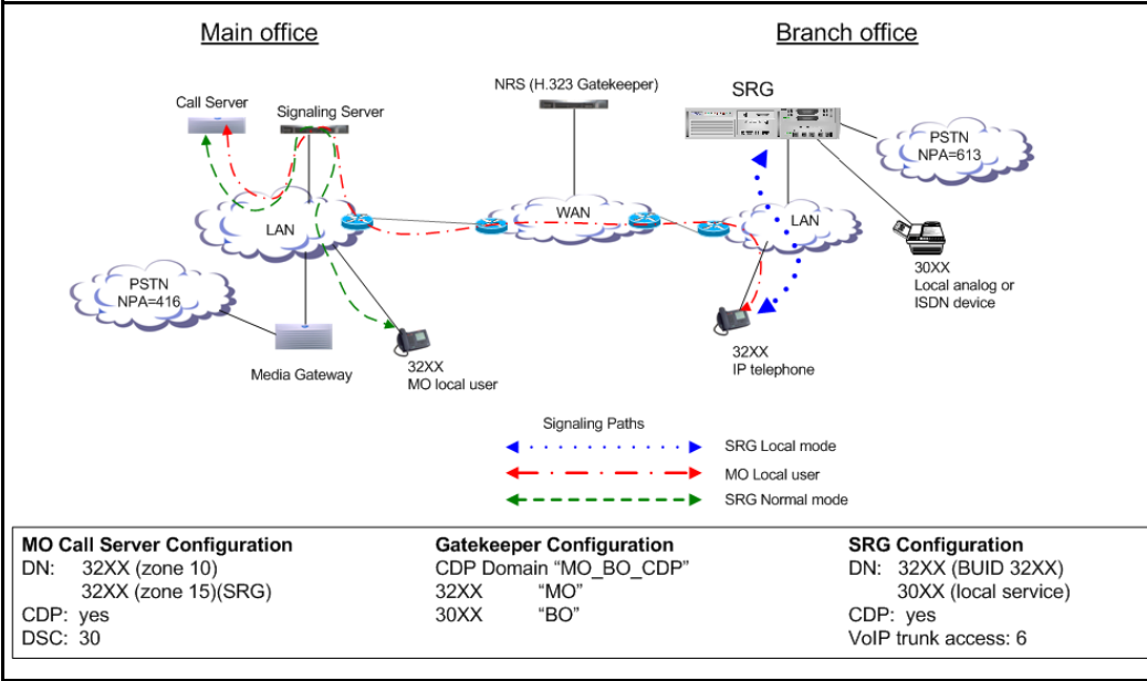
Figure 17 CDP Option 2: Main office and SRG DN ranges overlap; SRG IP Phone DNs are the same in Normal and Local Mode
