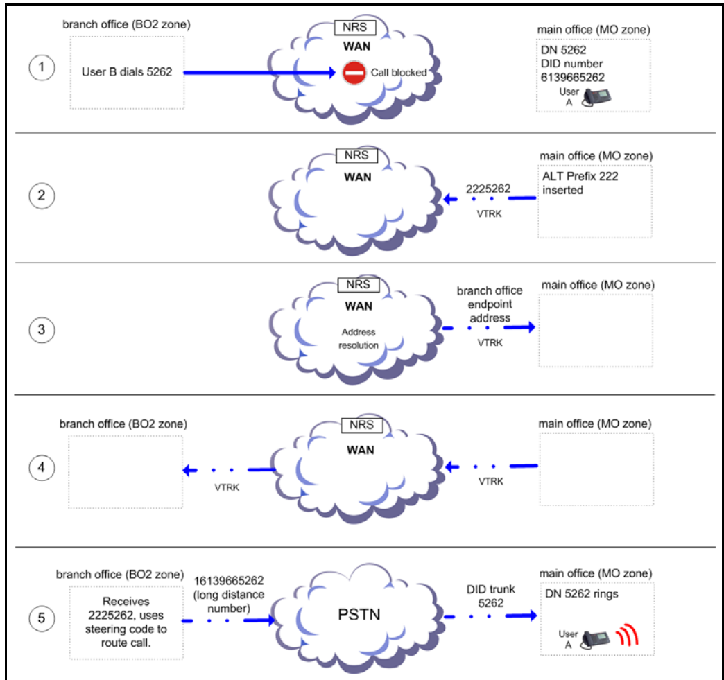
Figure 64 Illustration showing digits dialed and outpulsed with Alternative Call Routing for NBWM
