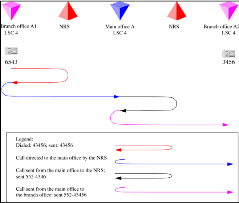
Figure 61 Call flow for Scenario 3- calls to remote branch office (destination side)
