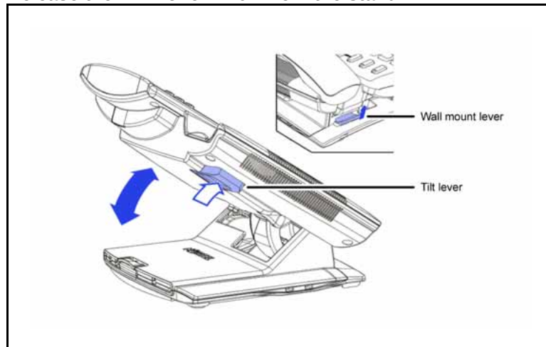
Release the IP Phone 1120E from the stand
