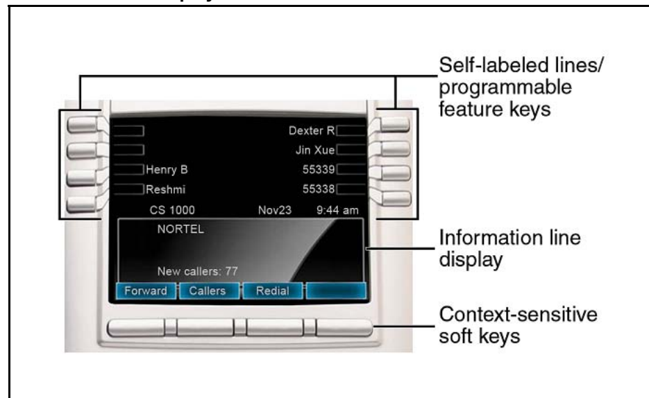
Figure 66 IP Phone 1165E display screen
