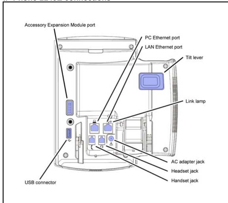
IP Phone 1140E connections
