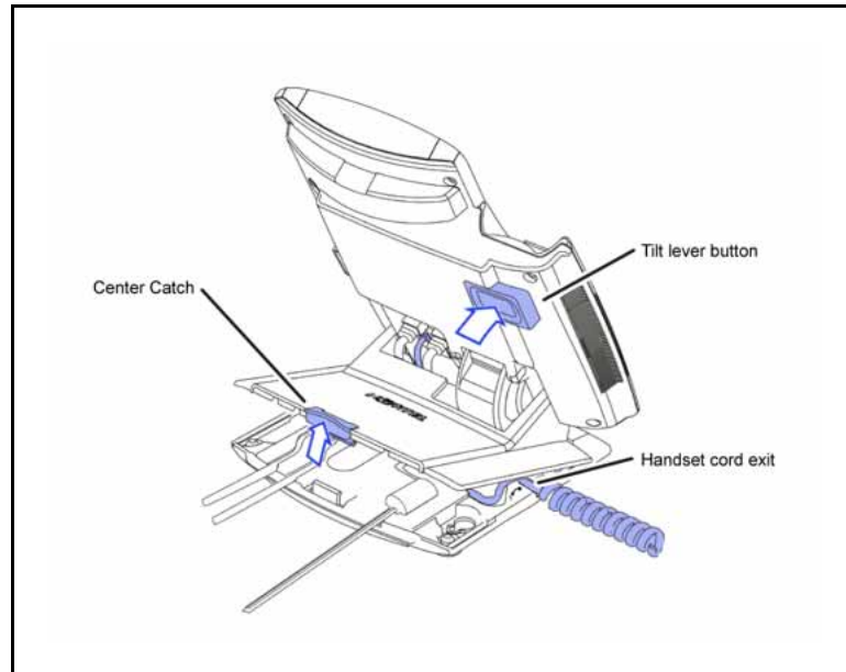
Figure 49 Stand cover removed
