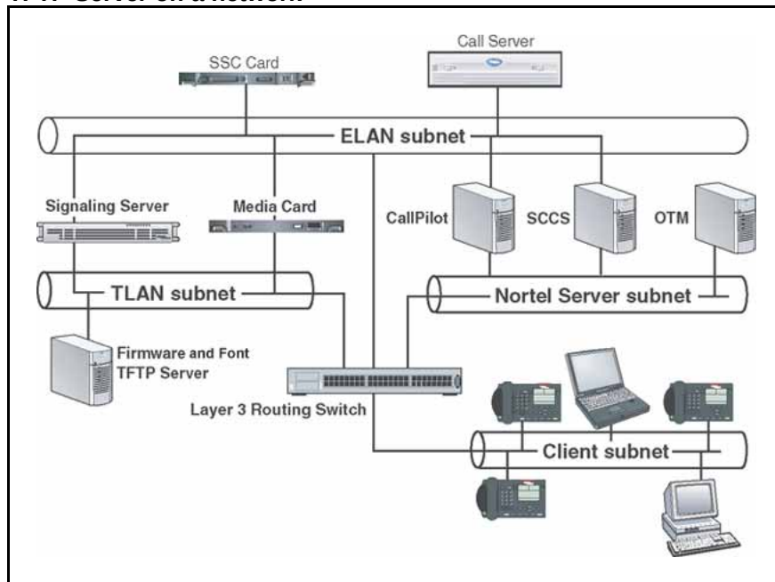
Figure 126 TFTP Server on a network
