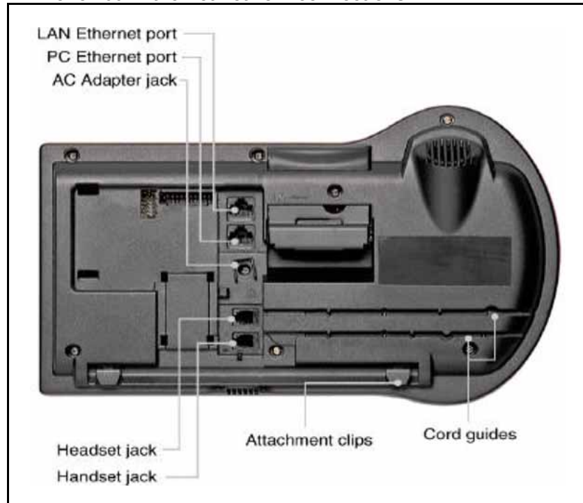
IP Phone 2004 Ethernet network connections
