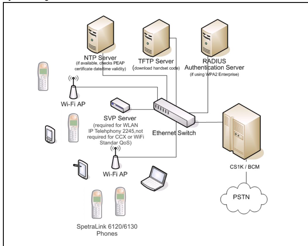
Figure 3 System diagram
