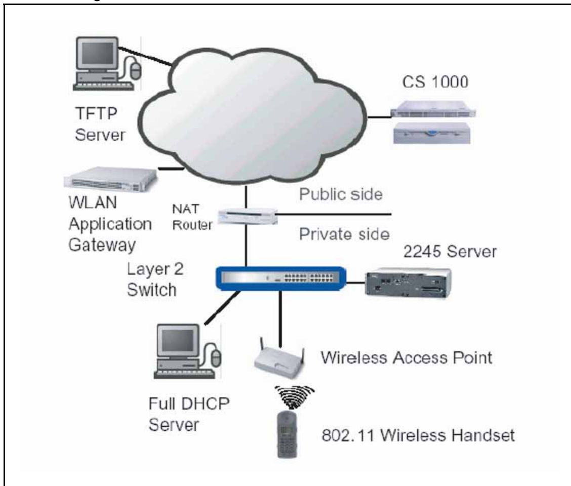
Figure 23 Network configuration 3 with Full DHCP Server
