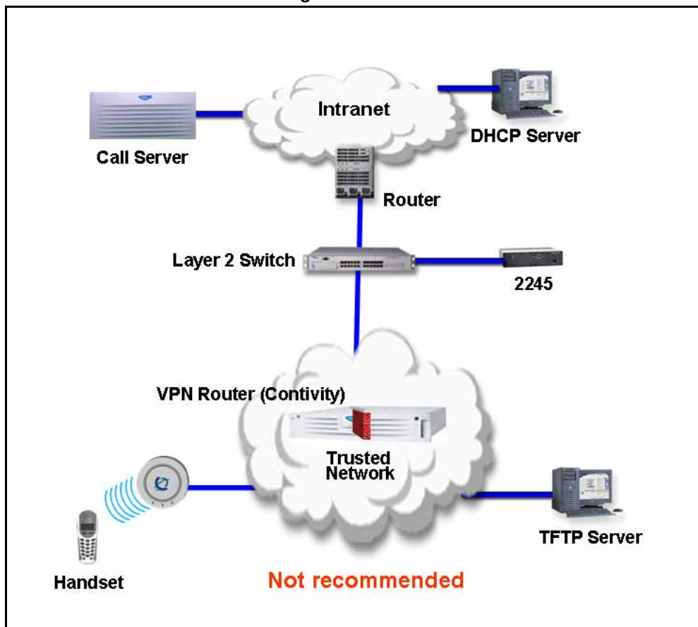
Figure 22 Not recommended VoWLAN design
