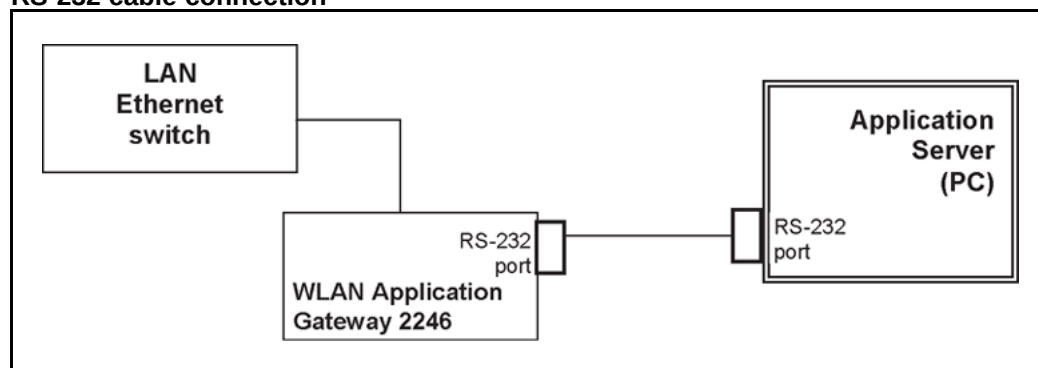
Figure 28 RS-232 cable connection
