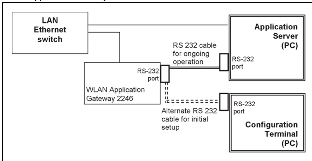
Figure 25 WLAN Application Gateway 2246 connections
