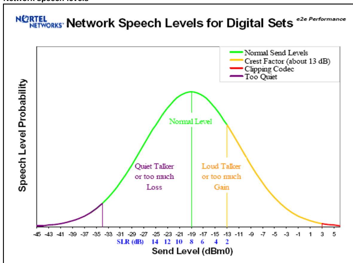
Figure 37 Network speech levels
