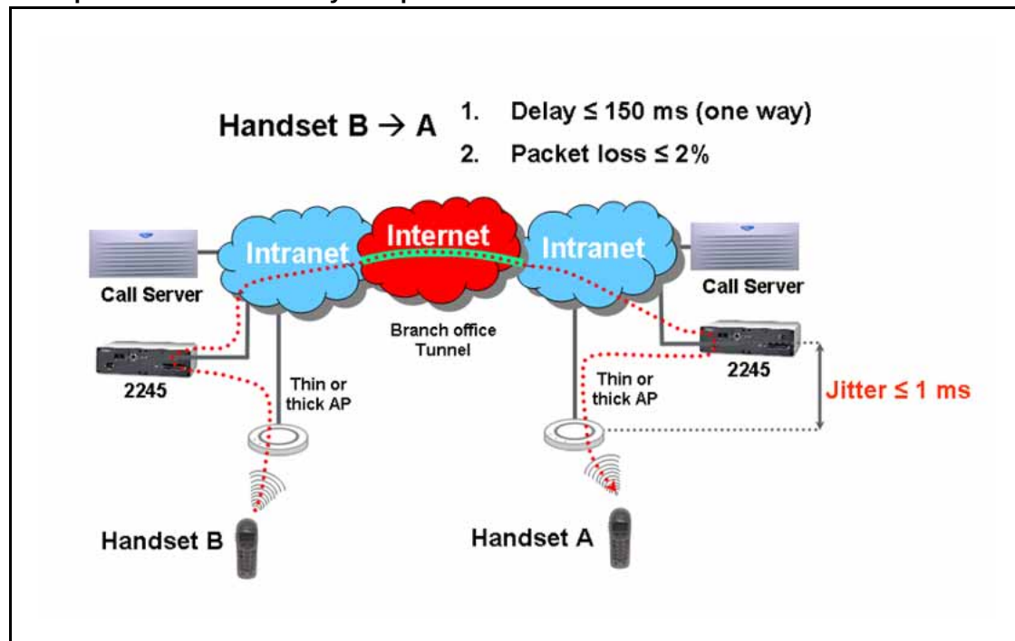
Figure 15 Example 2: End-to-end delay and packet loss for a WAN
