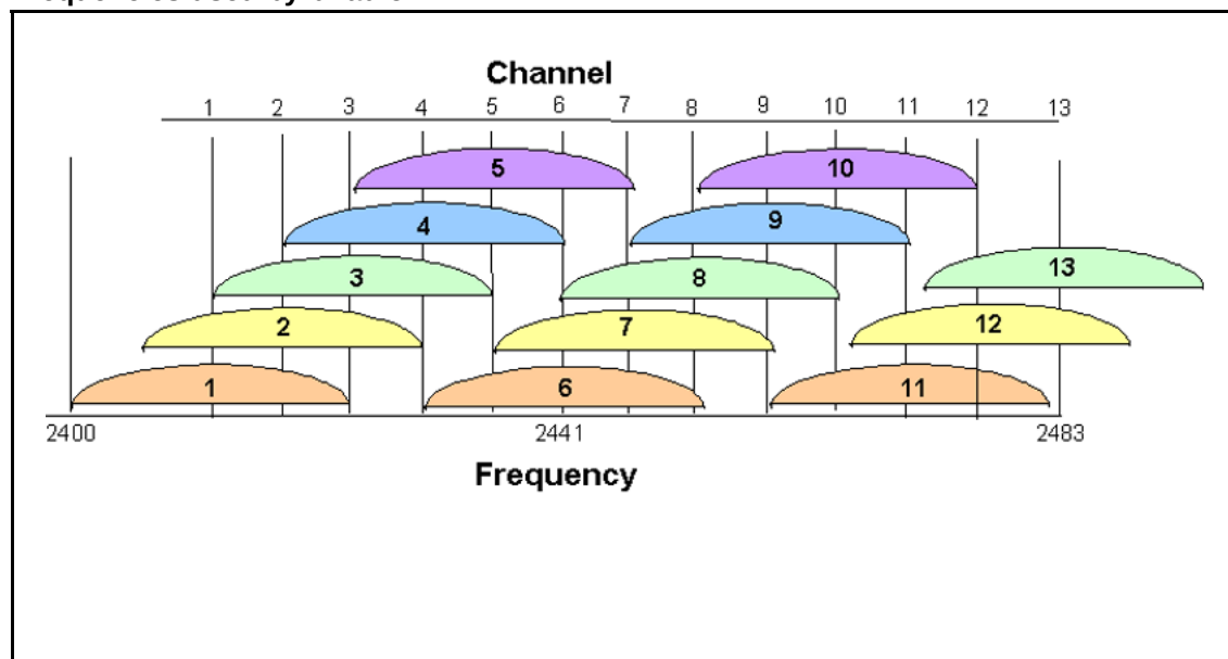
Figure 5 Frequencies used by b radio
