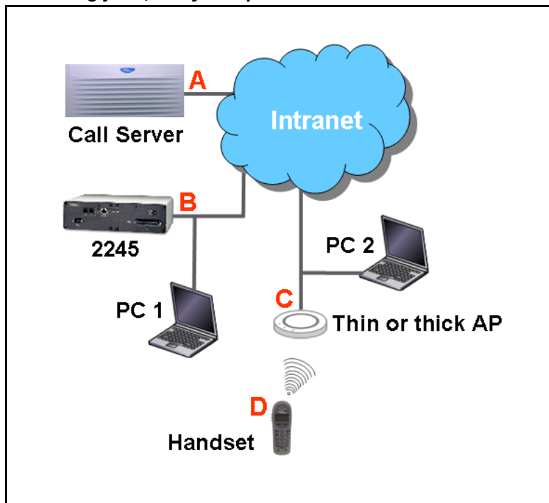
Figure 17 Measuring jitter, delay and packet loss
