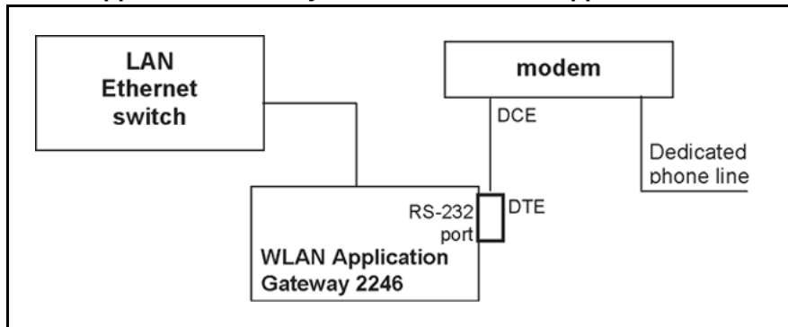
Figure 30 WLAN Application Gateway 2246 connection to Application Server through a modem
