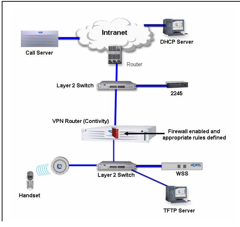
Figure 20 VPN design over a Layer 2 network
