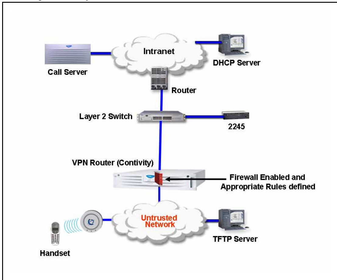
Figure 21 VPN design over a Layer 3 network
