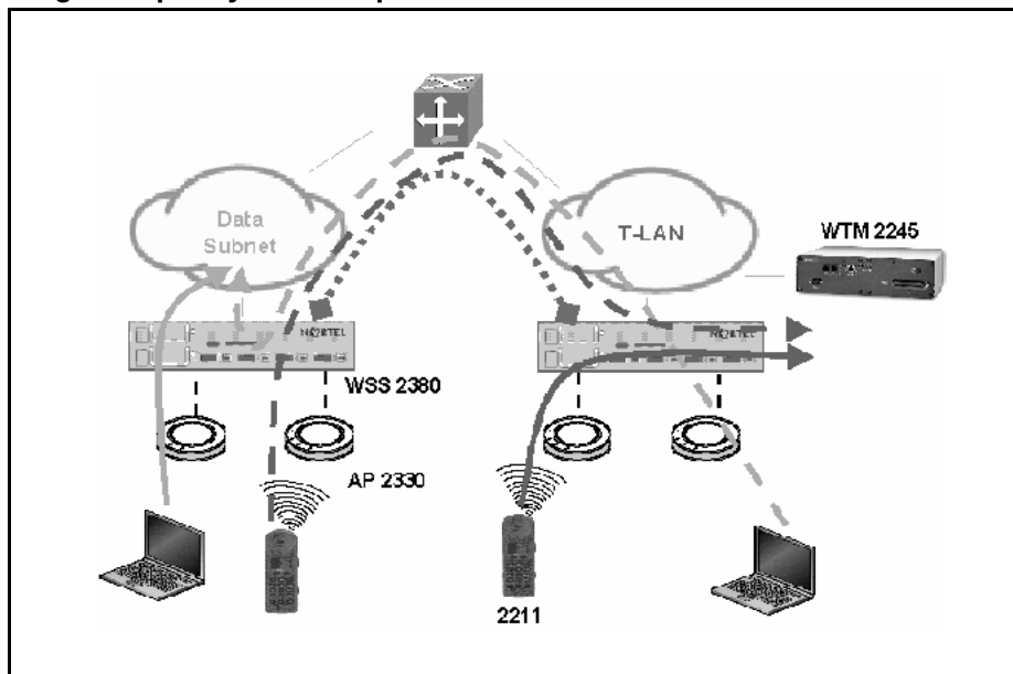
Figure 11 Single telephony VLAN implementation
