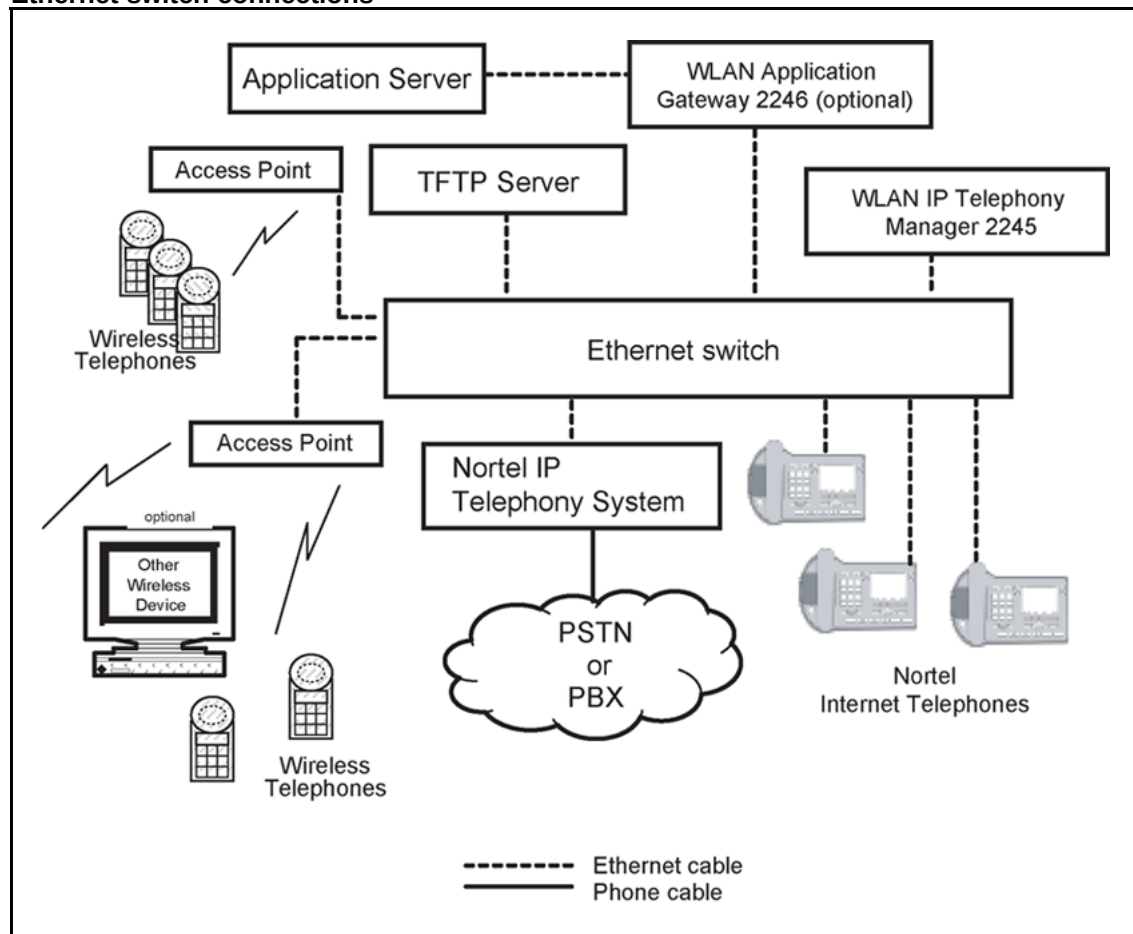
Figure 26 Ethernet switch connections
