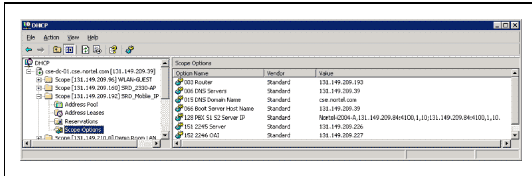
Figure 4 Sample DHCP reservation showing assigned parameters
