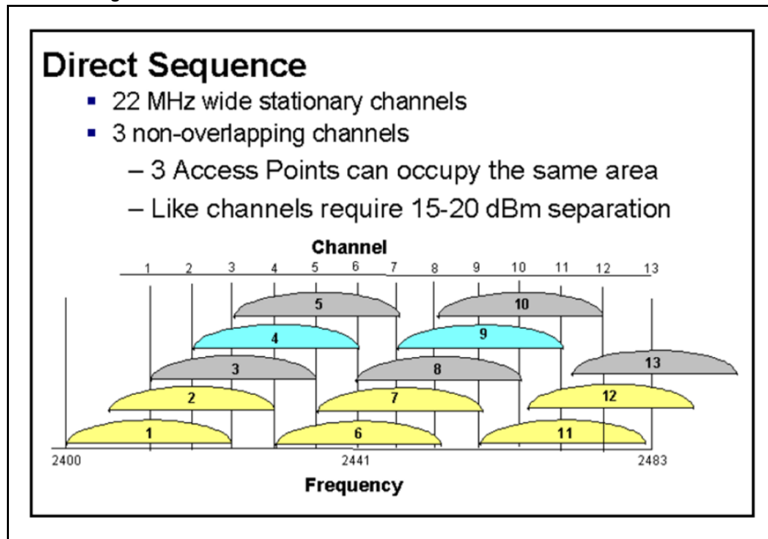
Figure 7 b radio assignment
