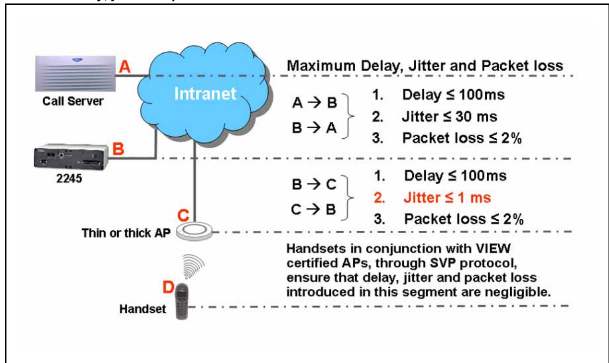
Figure 12 Maximum delay, jitter and packet loss
