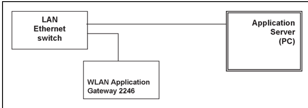
Figure 29 WLAN Application Gateway 2246 connection to Application Server through the LAN
