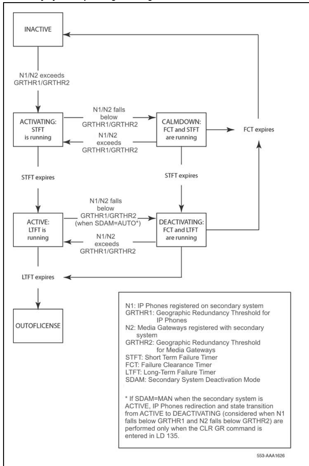
Figure 5 Secondary system operating state logic
