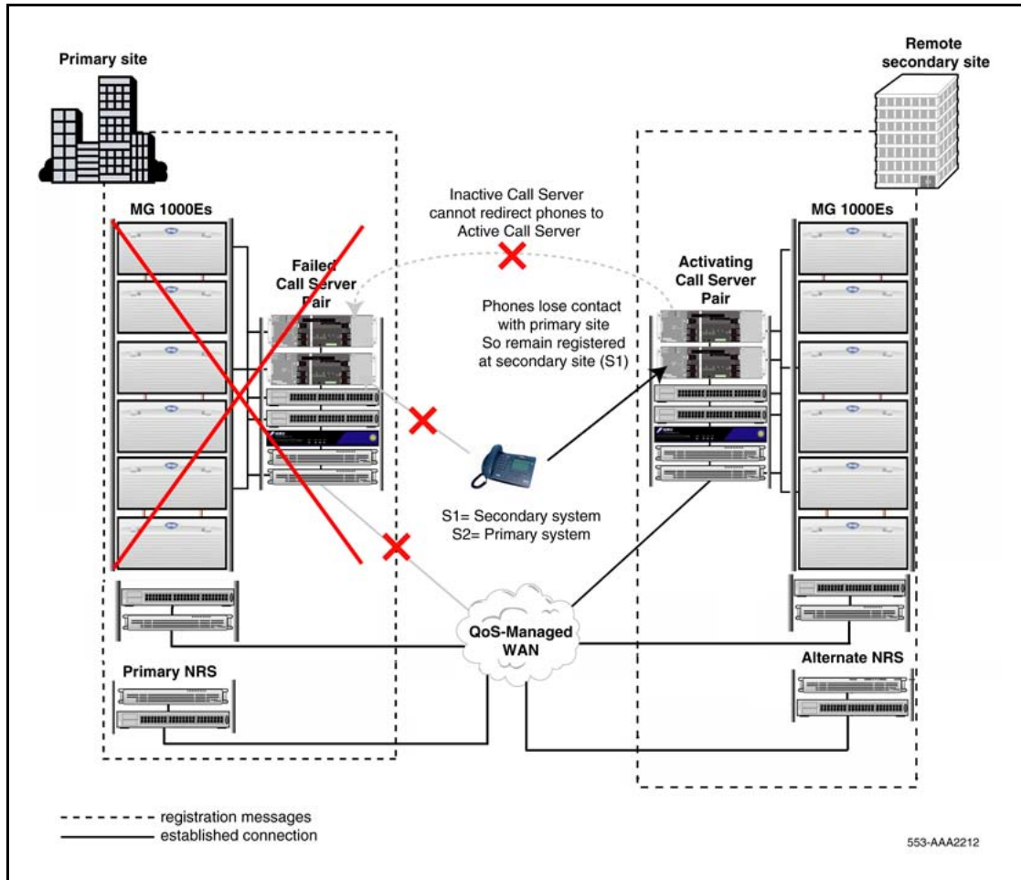
Figure 26 IP Phone redirection: Primary site failure
