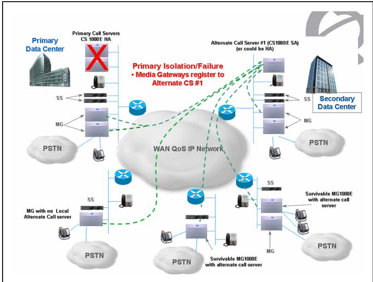
Figure 3 Survivable Media Gateway: Primary Call Server Failure or Loss of Network Connectivity
