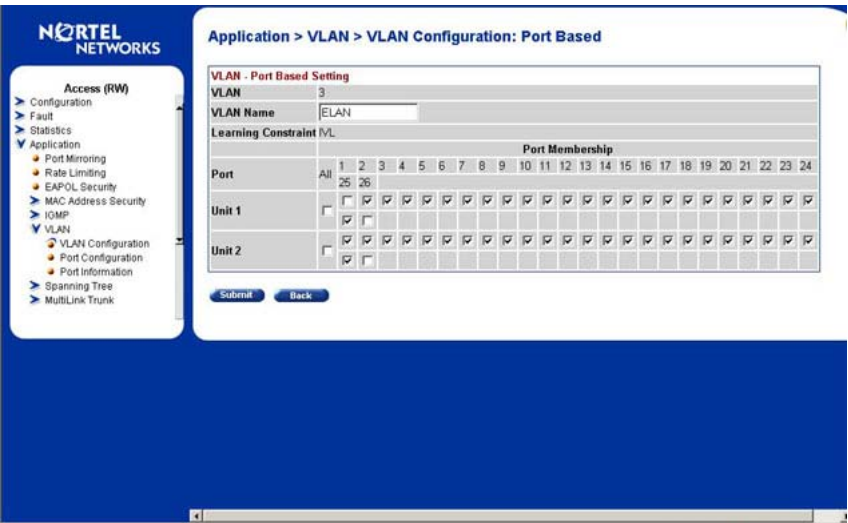
Figure 51 ELAN VLAN port membership configuration
