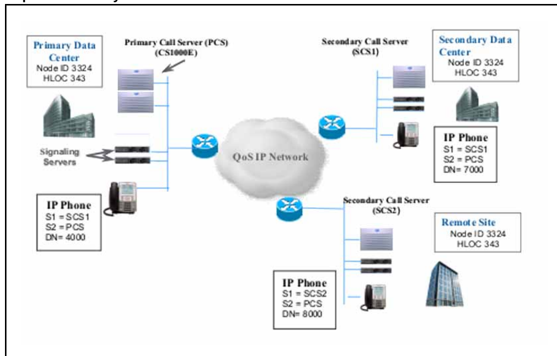
Figure 32 Triple redundancy
