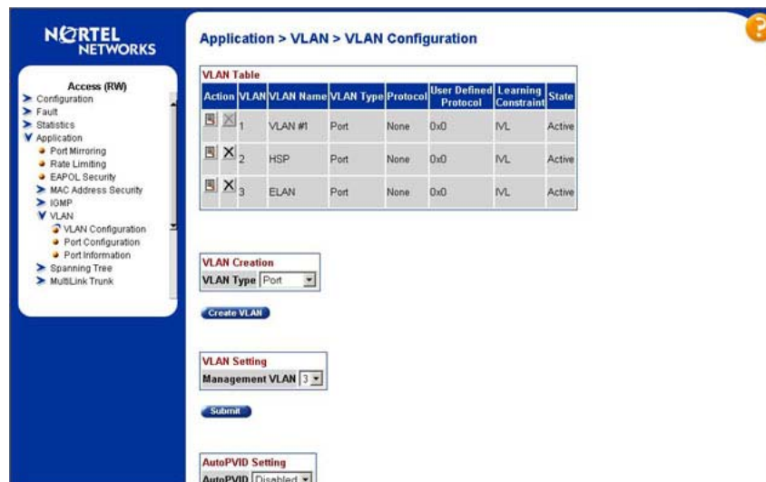
Figure 44 VLAN configuration
