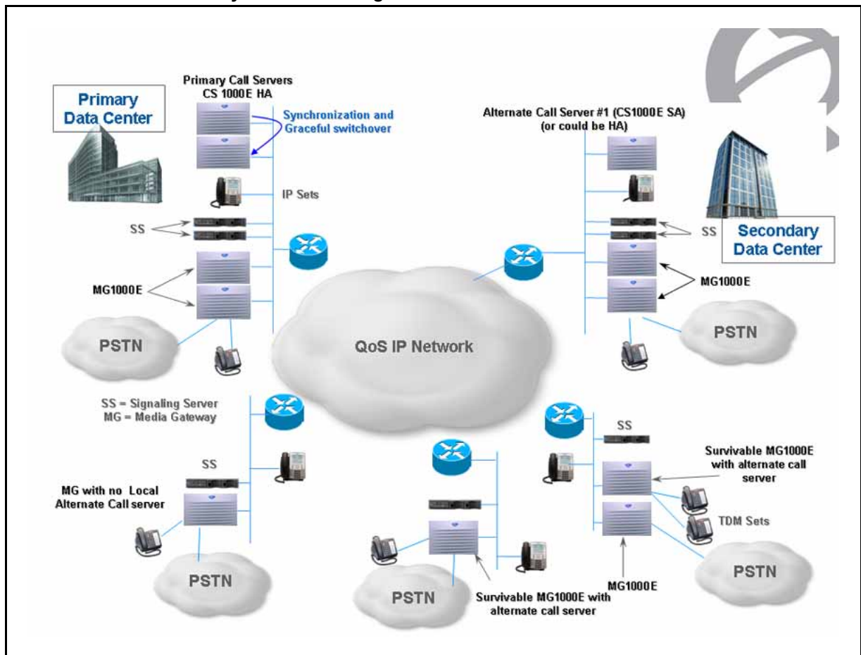
Figure 1 Survivable Media Gateway: Normal Configuration
