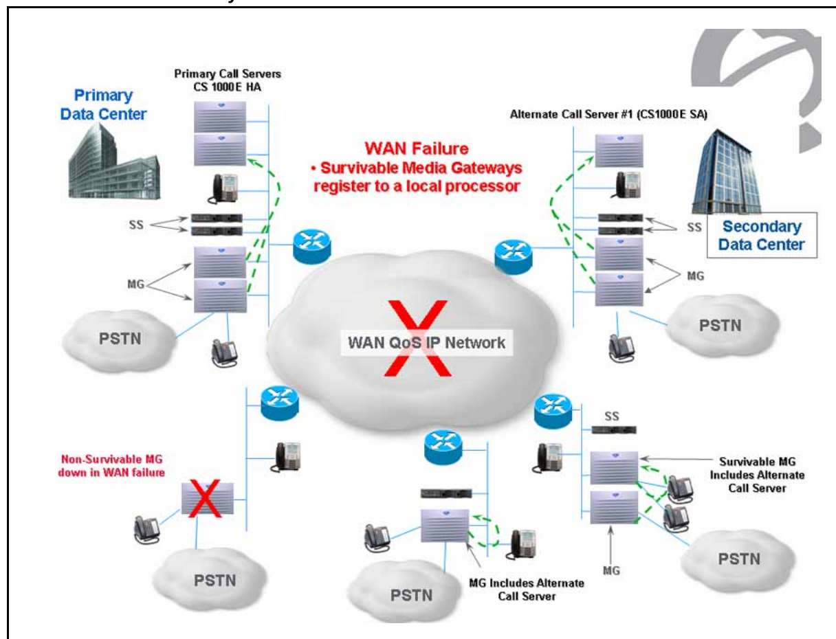
Figure 4 Survivable Media Gateway: WAN Failure
