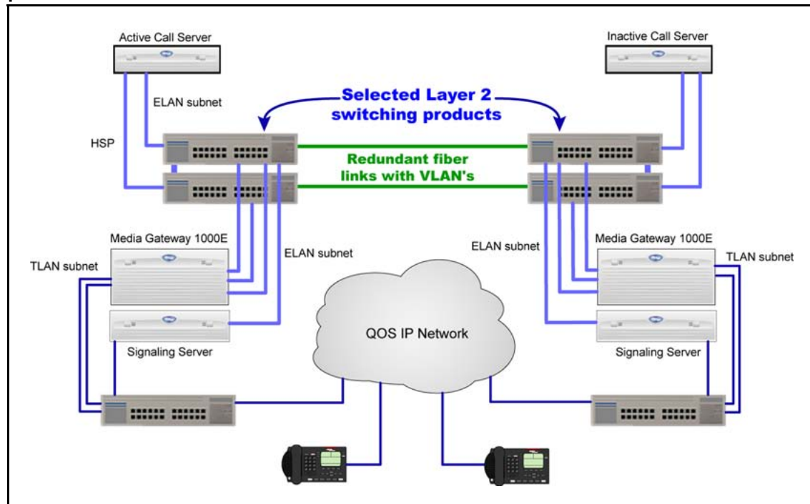
Figure 38 Call Server and Signaling Server (HSP and ELAN subnet) separated with Layer 2 switching products
