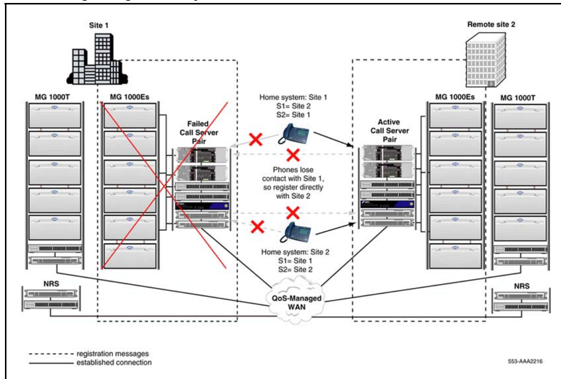
Figure 35 Load-sharing configuration: system failure at Site 1
