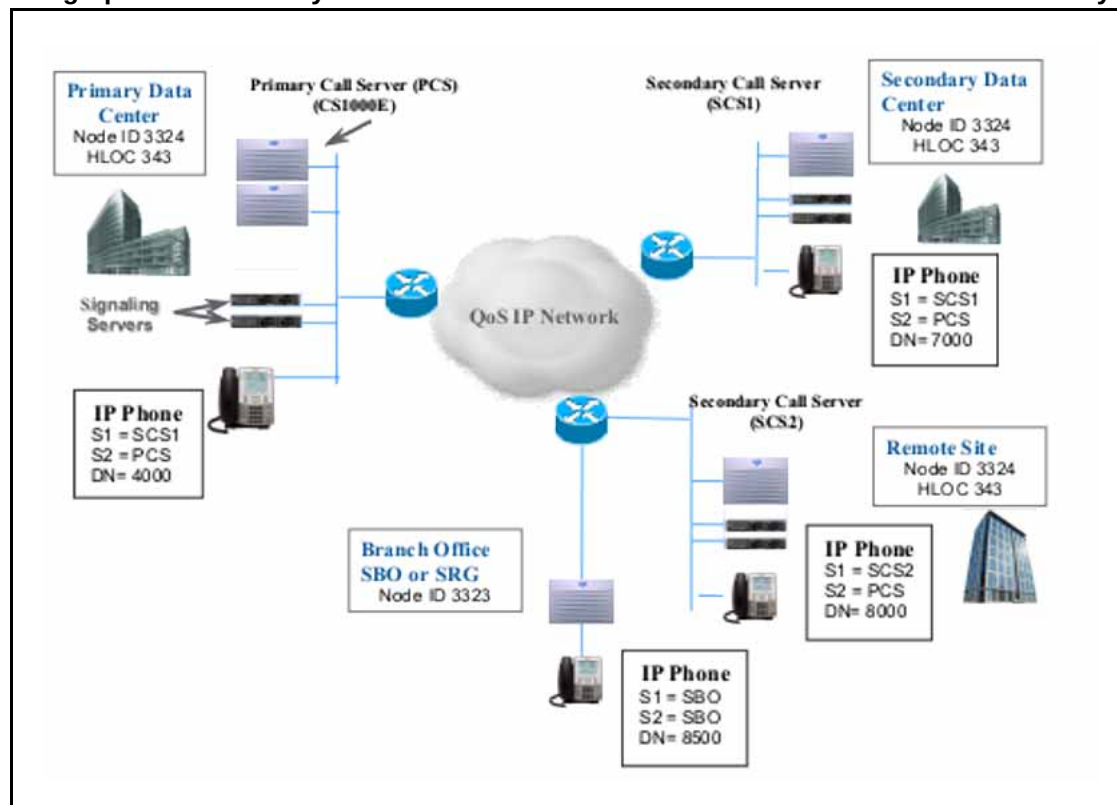
Figure 33 Geographic Redundancy with Survivable Branch Office or Survivable Remote Gateway
