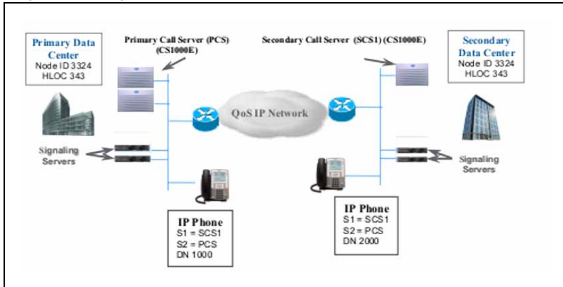
Figure 30 Simple redundancy
