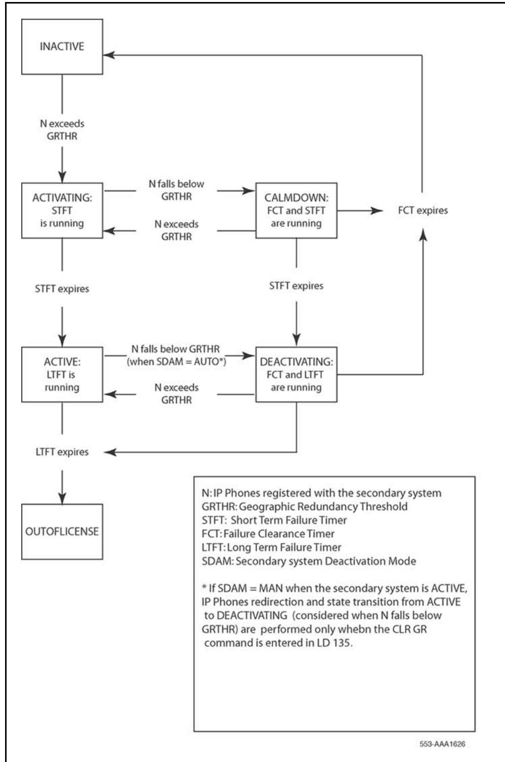
Figure 27 Secondary system operating state logic
