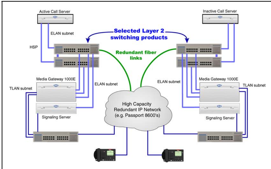
Figure 39 Call Server and Signaling Server (ELAN subnet and HSP) separated by high capacity network
