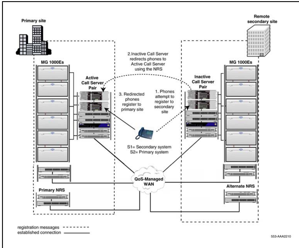
Figure 25 IP Phone redirection: Normal operation
