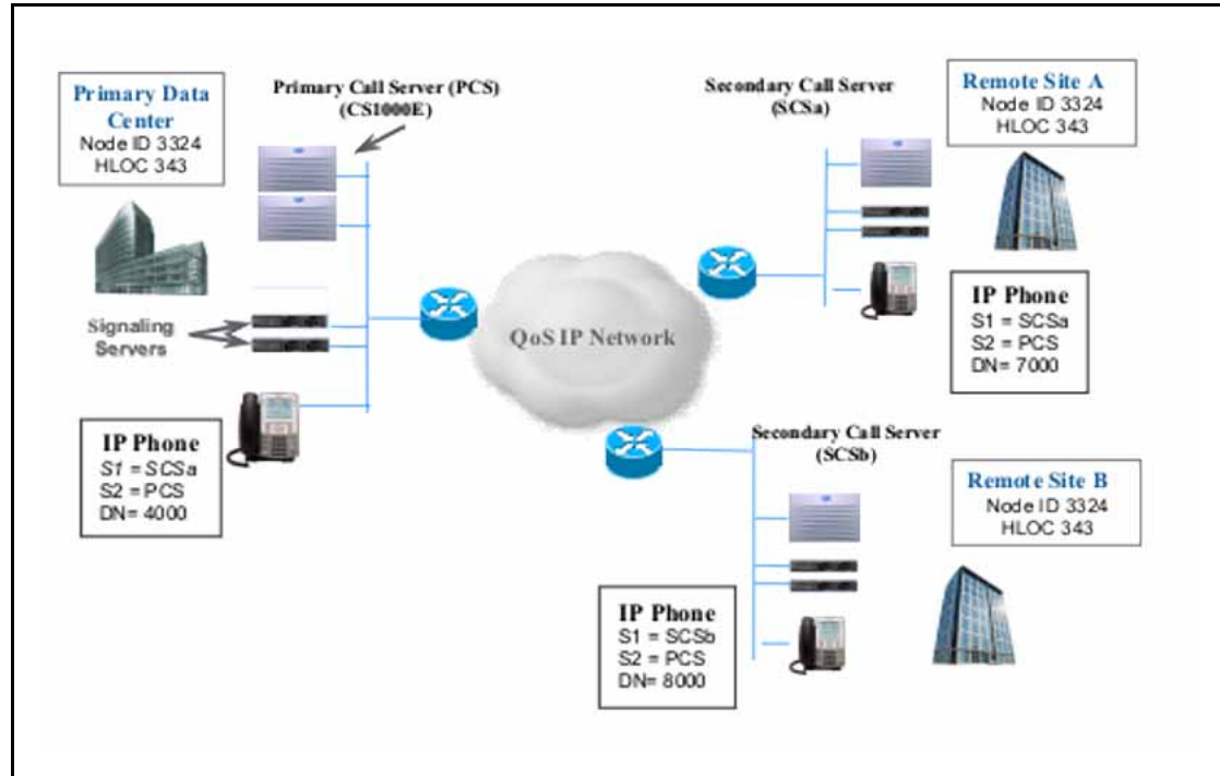
Figure 31 Multiple site redundancy
