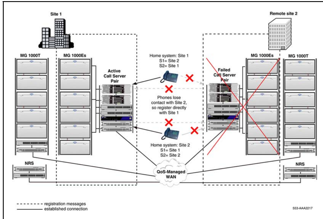
Figure 36 Controlled Load-sharing configuration: system failure at Site 2
