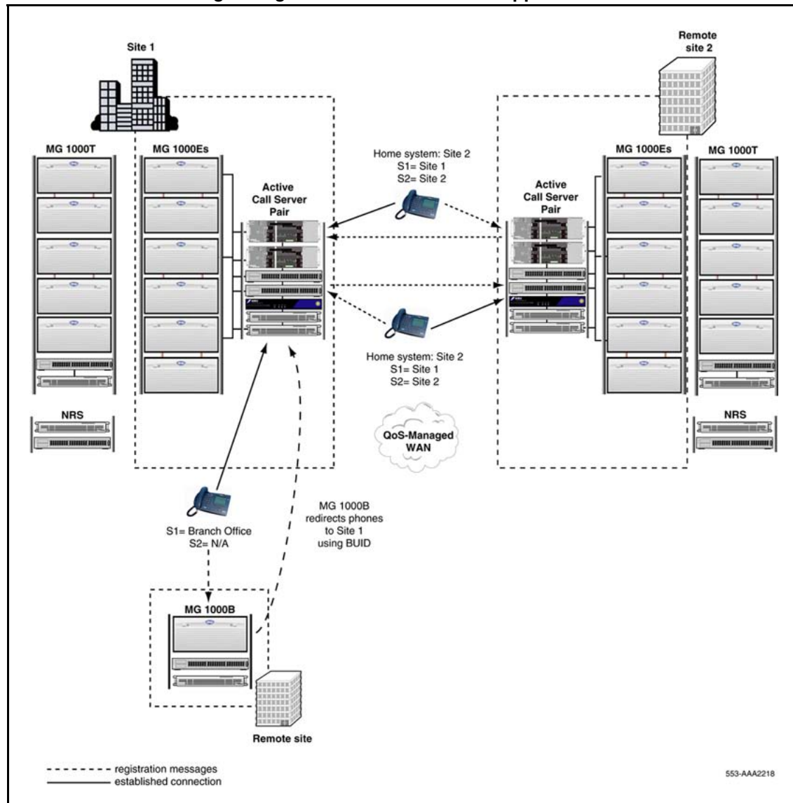
Figure 37 Controlled Load-sharing configuration: Branch Office support
