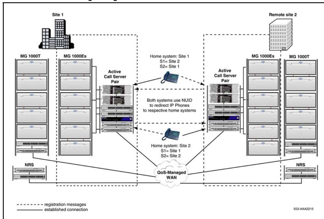
Figure 34 Controlled Load-Sharing configuration
