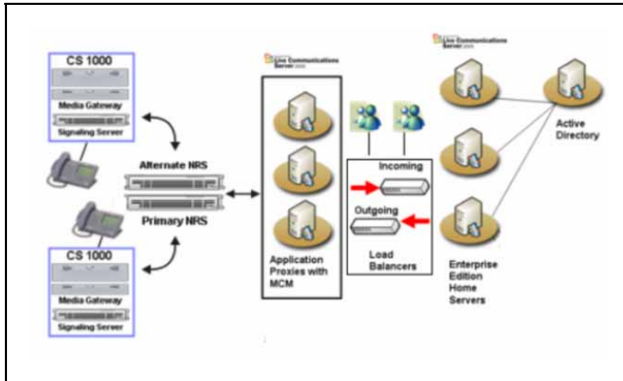
Figure 34 Redundancy with Load Balancers
