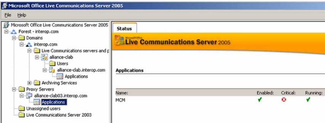
Figure 153 MCM Application
