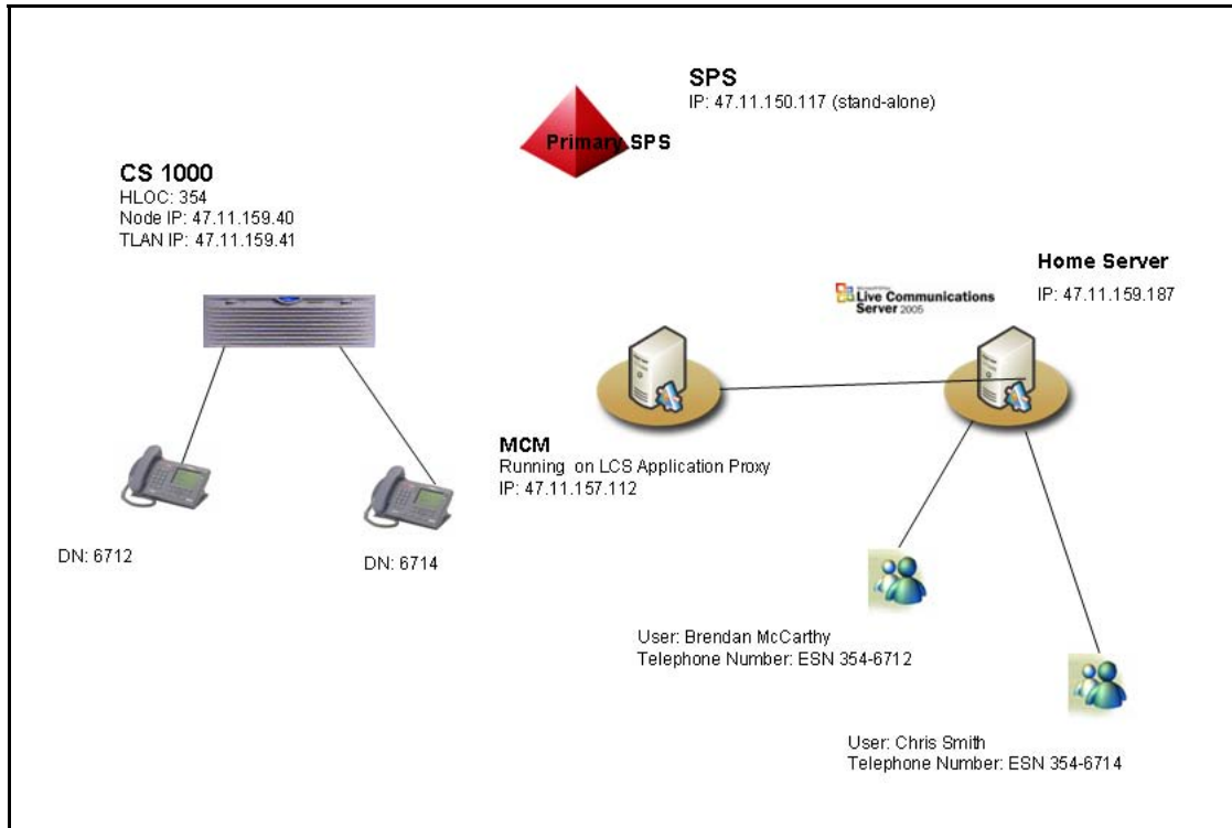
Figure 5 IP diagram
