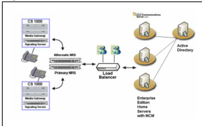
Figure 33 Single Load Balancer
