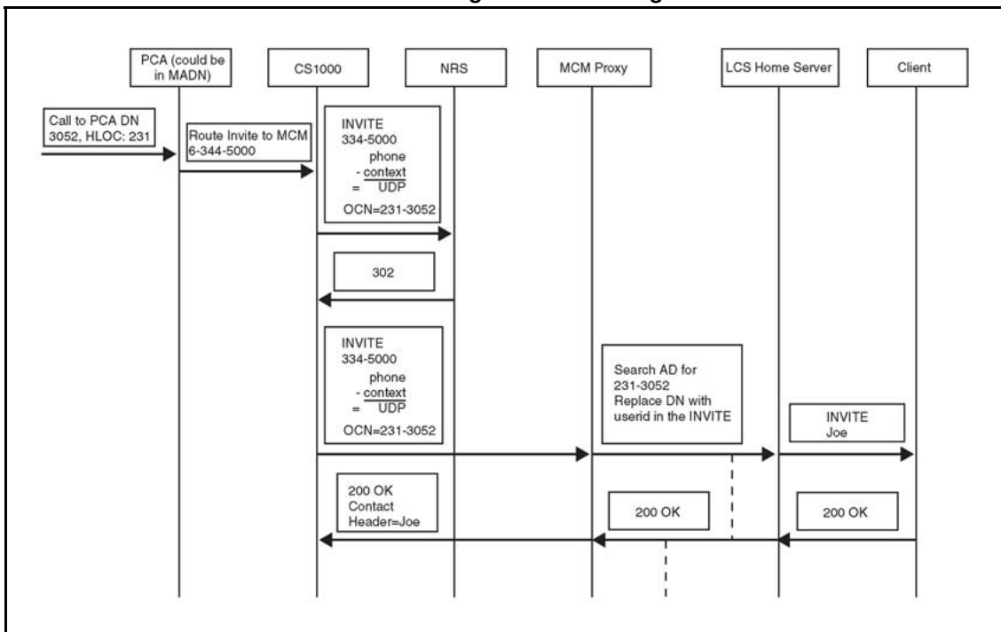
Figure 132 Microsoft® Office Communicator Incoming Call Flow using PCA
