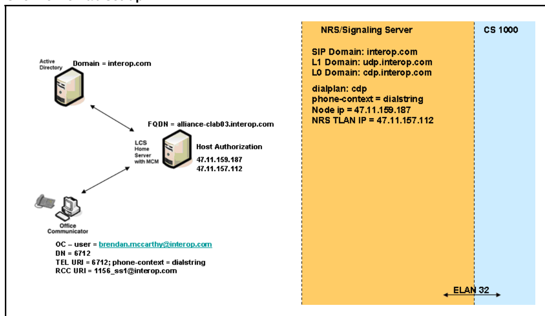
Figure 133 Overview of lab set-up
