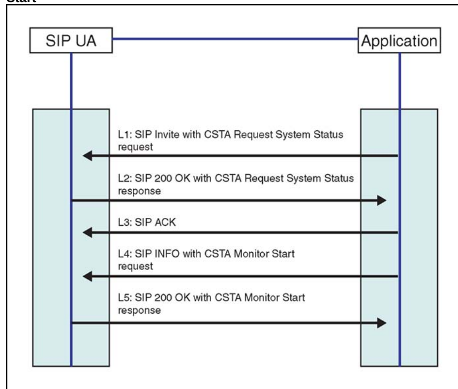
Figure 127 Message sequence diagram - CSTA Session Establishment and Monitor Start
