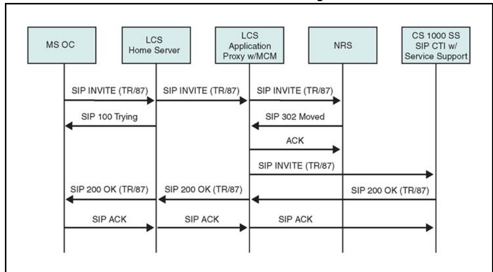
Figure 129 Remote Call Control Session Establishment through SRS
