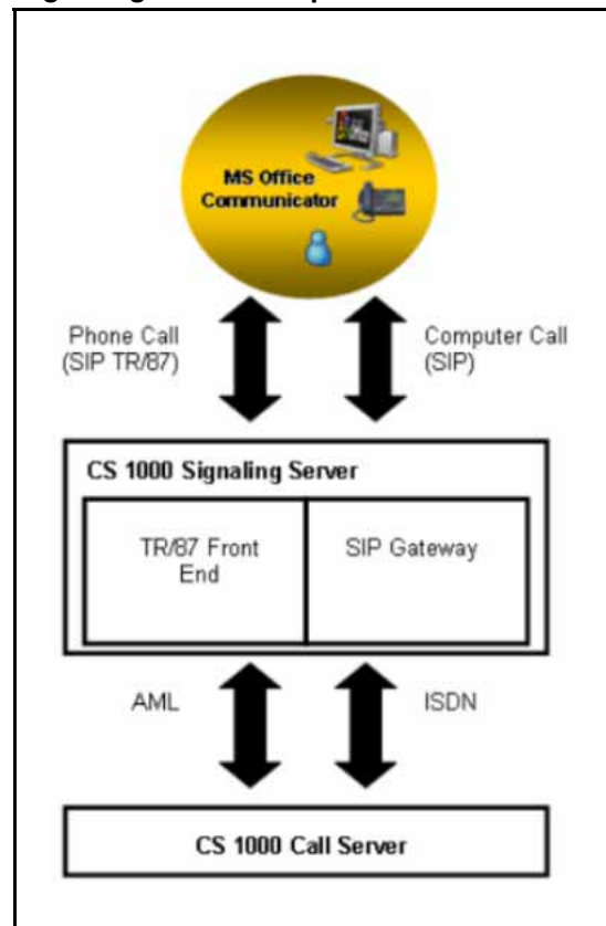
Figure 38 Signaling and media paths
