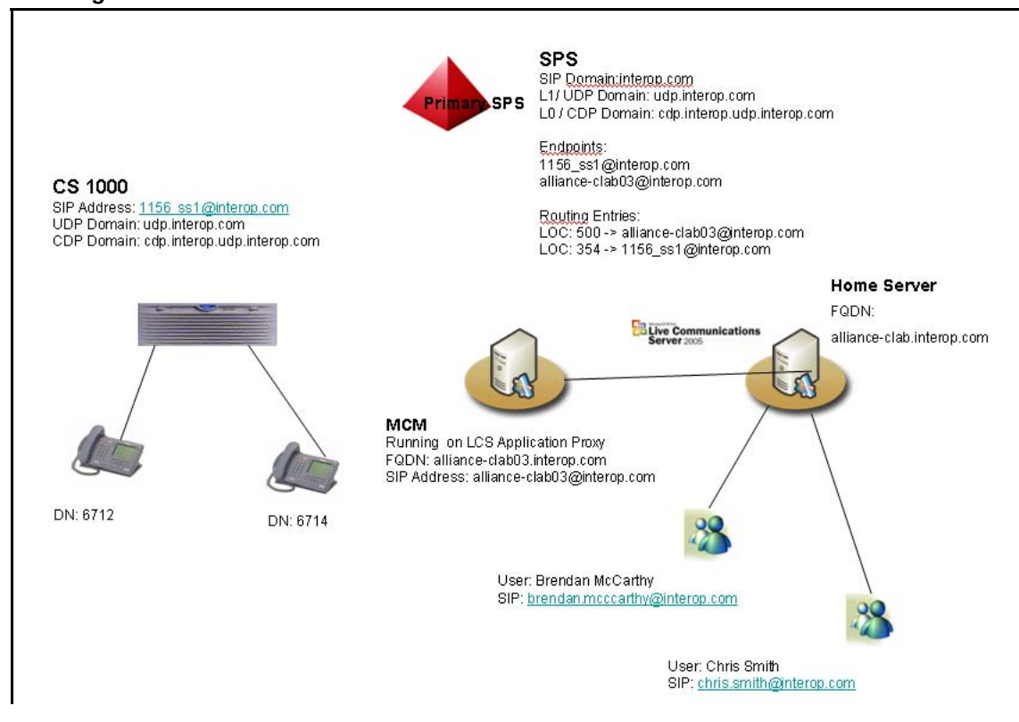
Figure 4 SIP diagram
