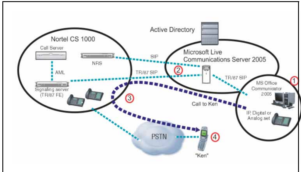
Figure 1 Remote Call Control with SIP CTI (TR/87)
