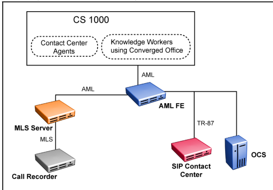
Figure 15 Call Recording for Knowledge Workers with Converged Office and Call Recording for SIP Contact Center Agents
