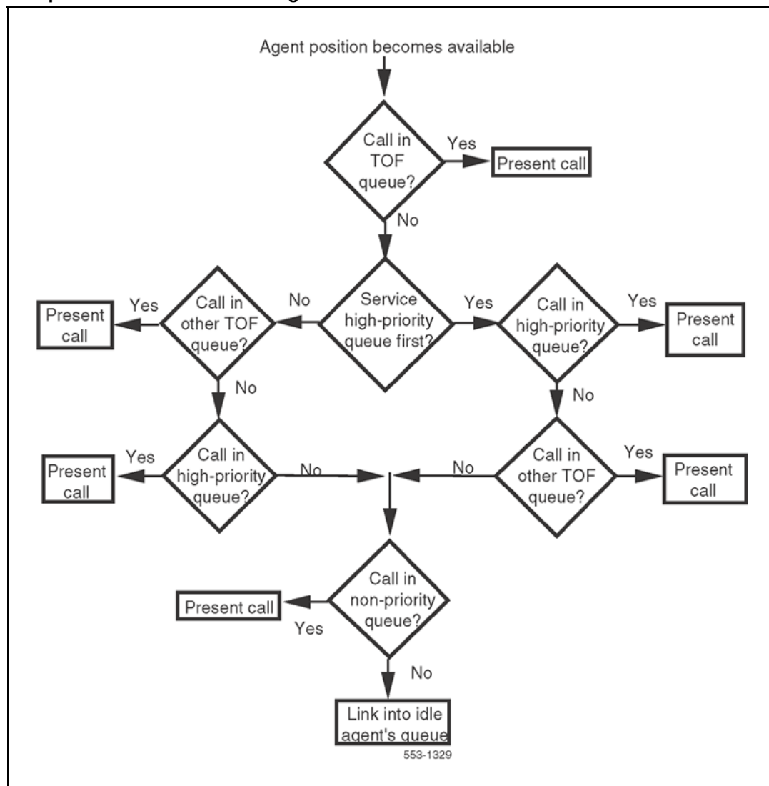
Figure 18 Call presentation to available agent
