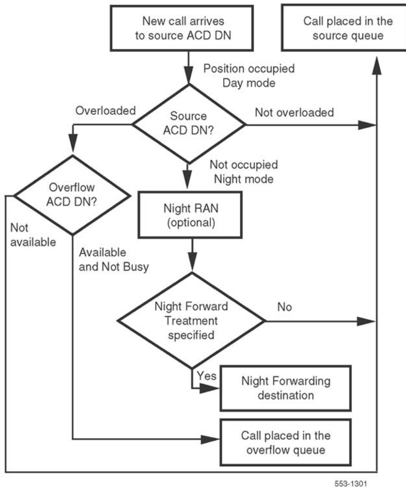
Figure 3: Automatic Overflow decision process
