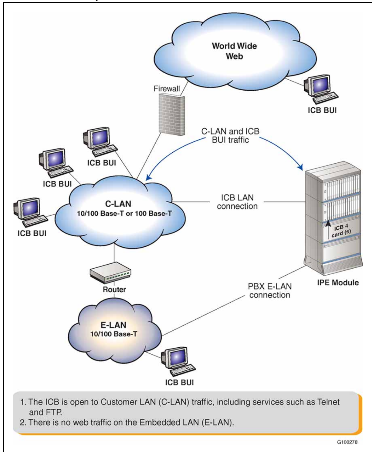
Figure 8 "LAN/intranet access only - E-LAN connection" (page 43) shows an example of the E-LAN connection.
