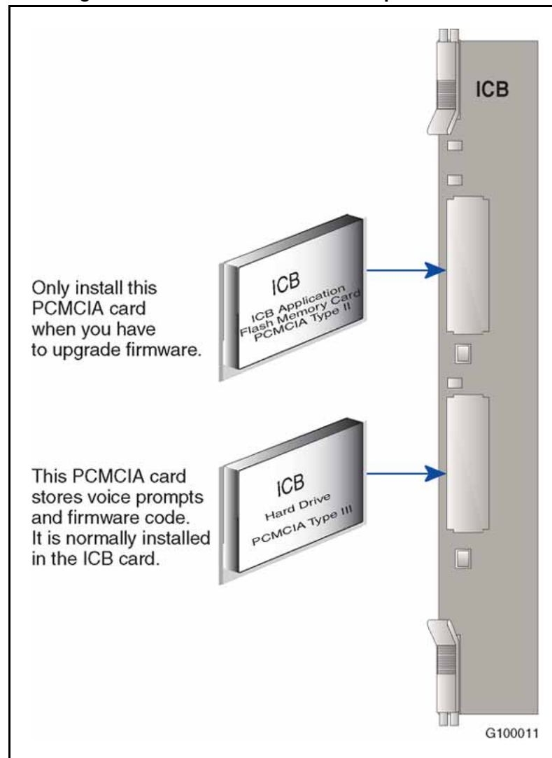
Figure 92 Installing a PCMCIA card into the ICB faceplate slot
