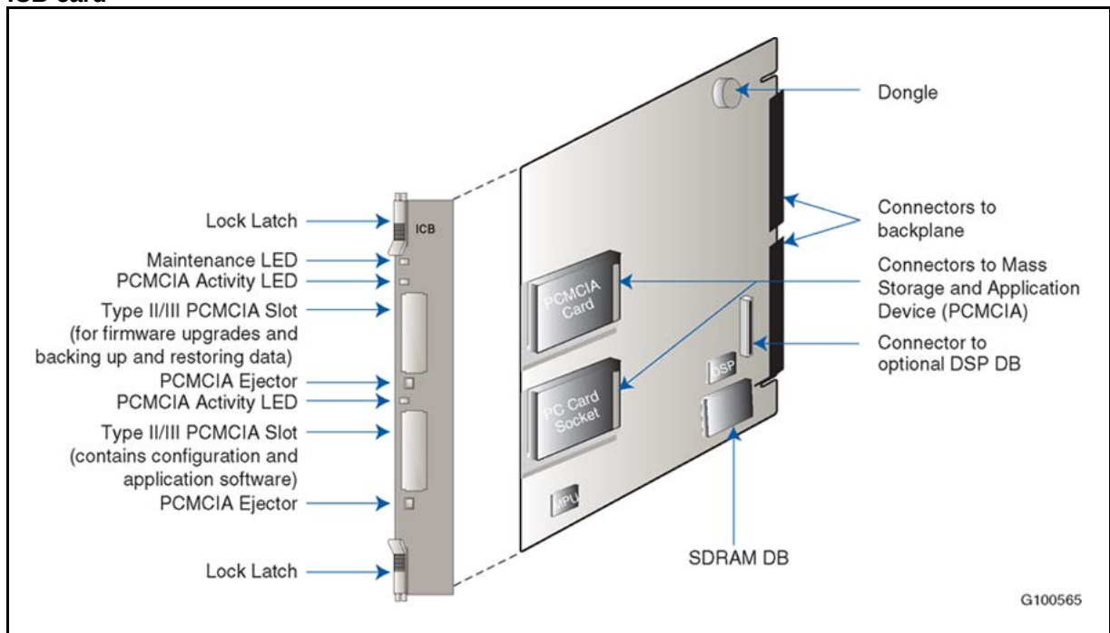
Figure 2 ICB card
