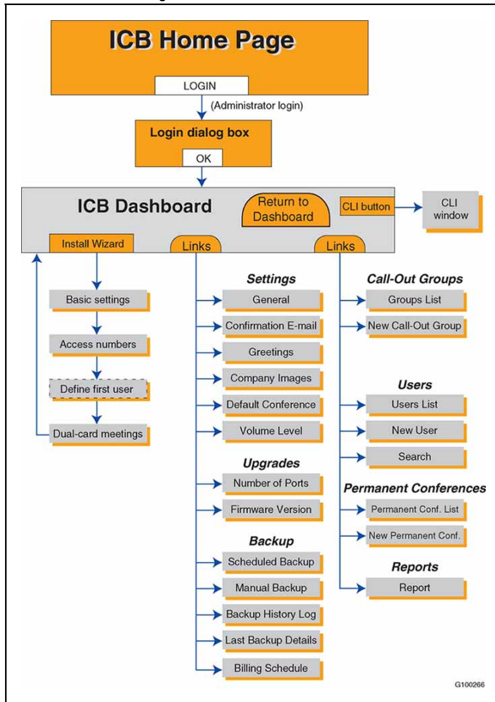
Figure 51 Administration BUI navigation flowchart
