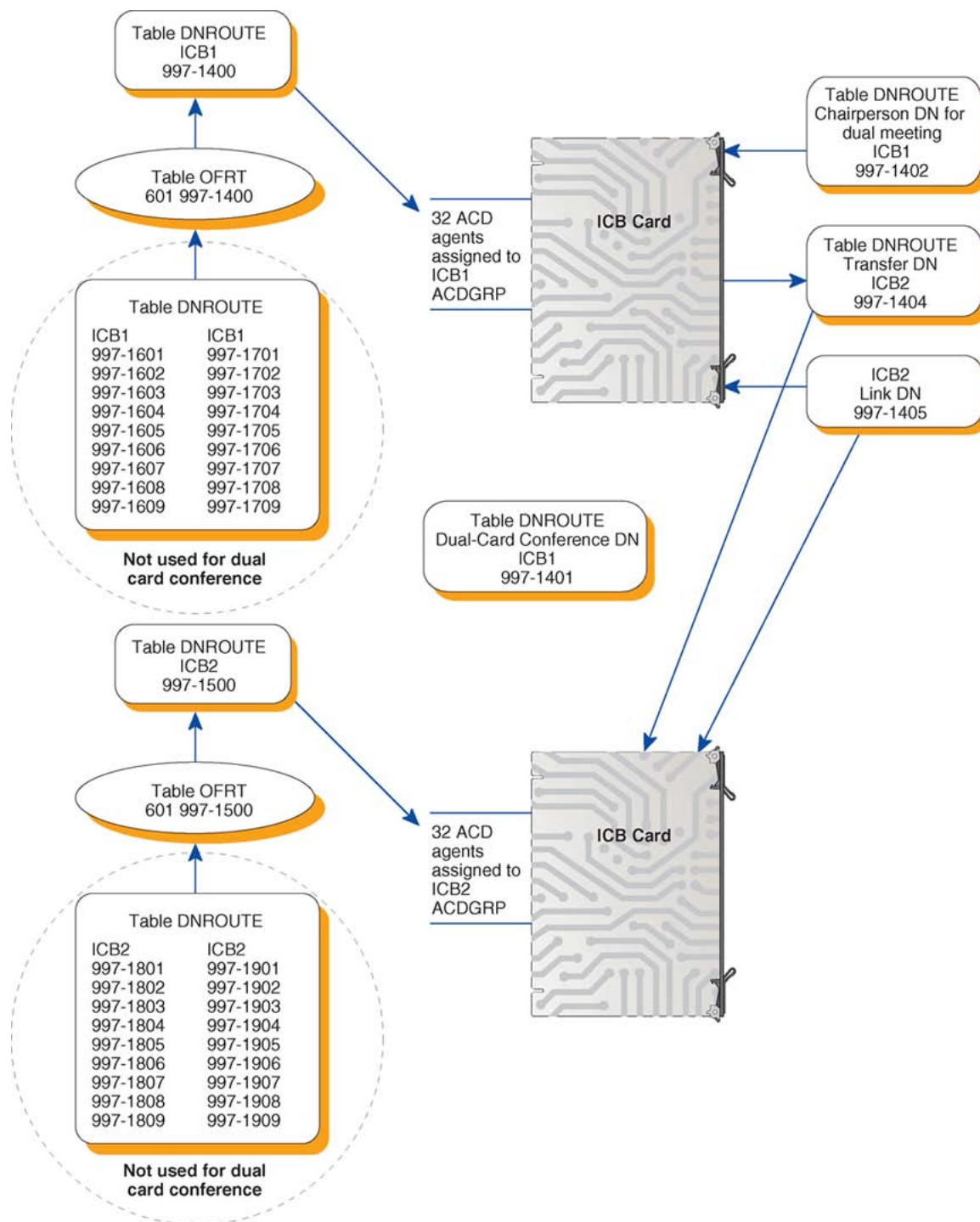
Figure 20: Dual-card conference, 1 conference, 62 ports
