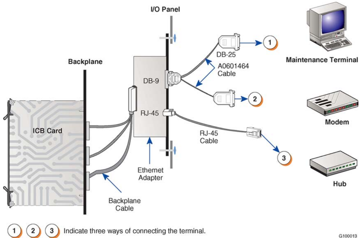
Figure 27: Terminal connection through the Ethernet Adapter
