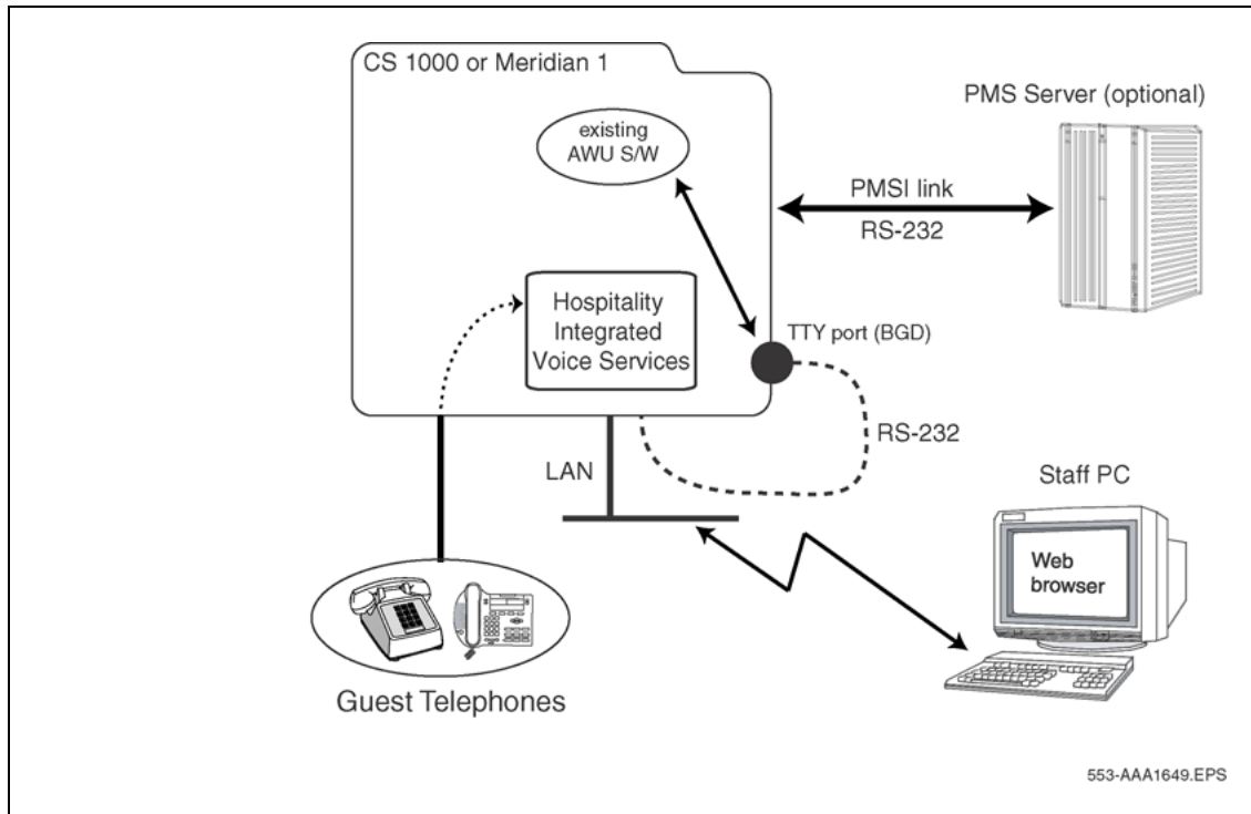
Figure 1 Hospitality Integrated Voice Services in the system
