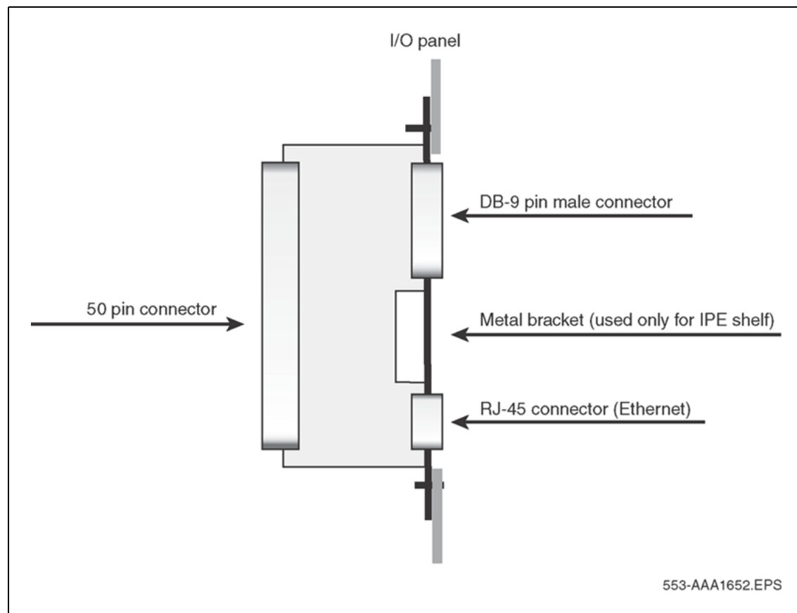
Figure 4 NT5D52BC Ethernet adapter
