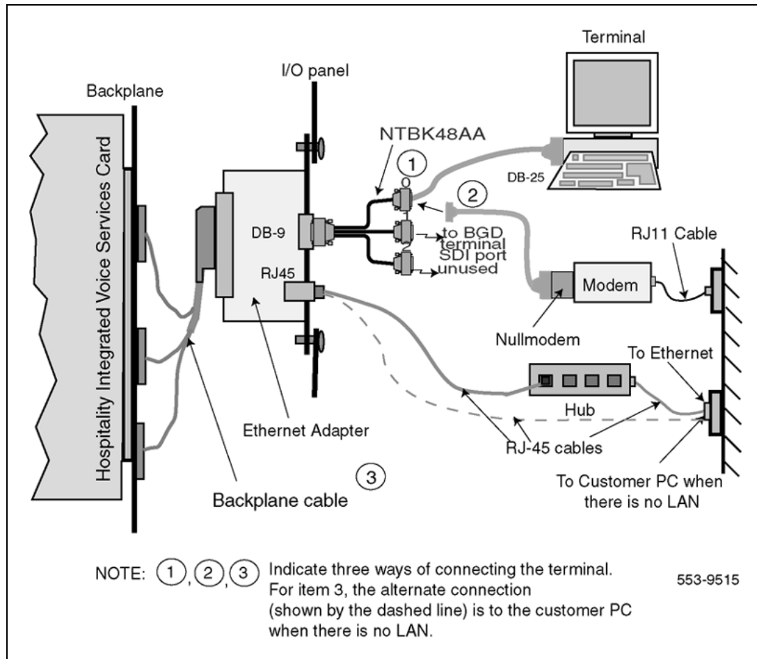
Figure 7 I/O connector bracket connection
