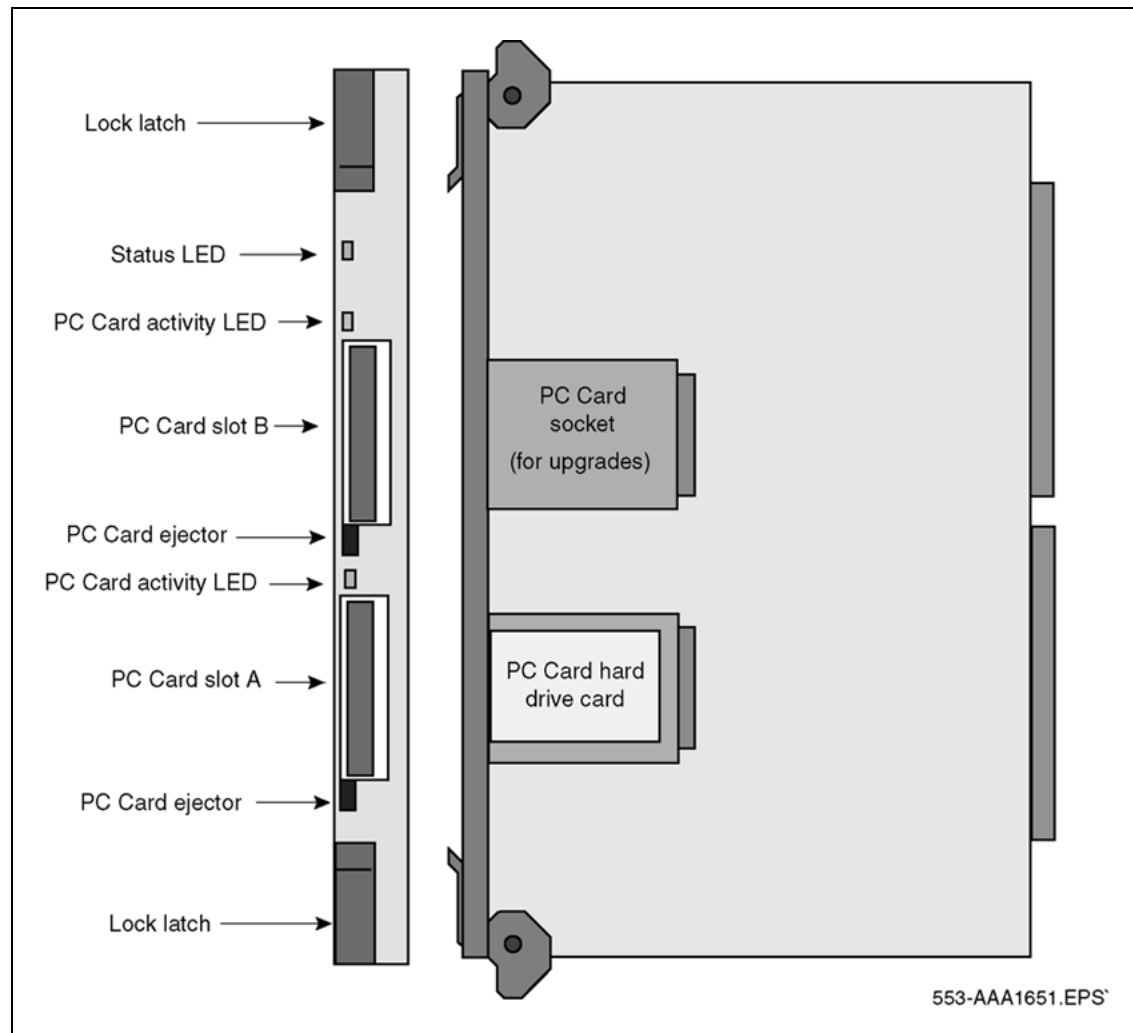
Figure 3 Hospitality Integrated Voice Services card
