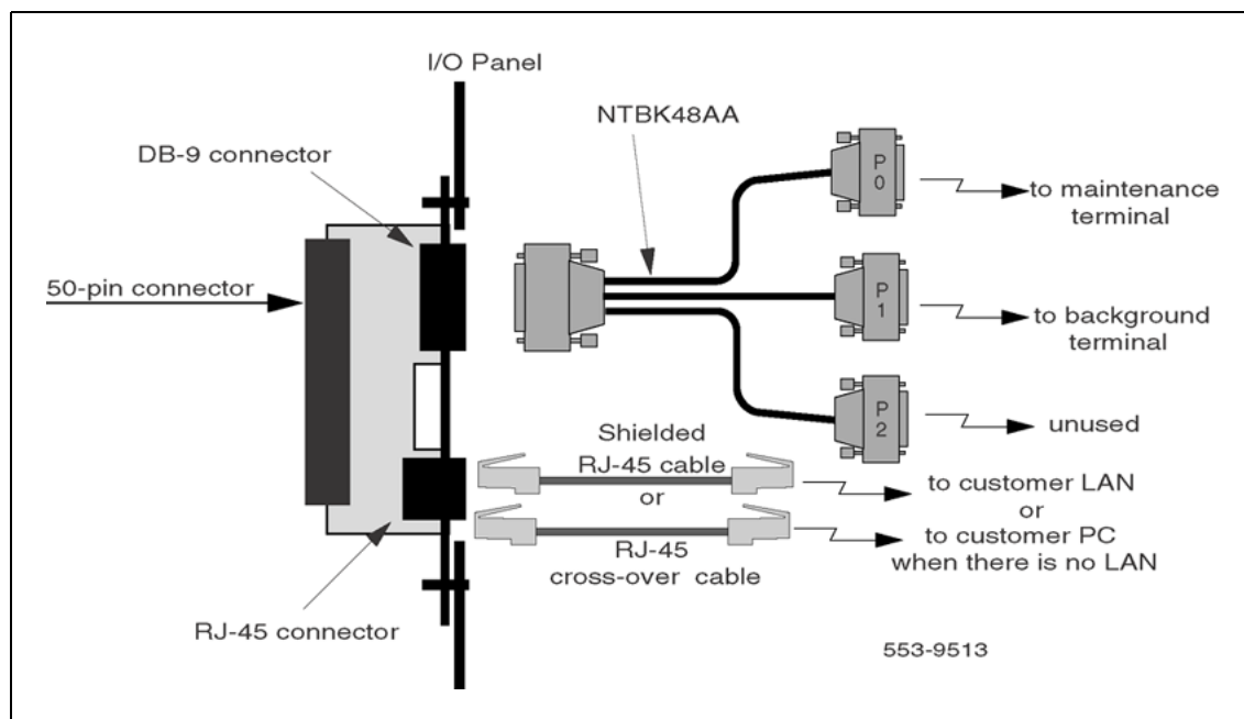
Figure 6 The Ethernet adapter and the NTB48AA cable
