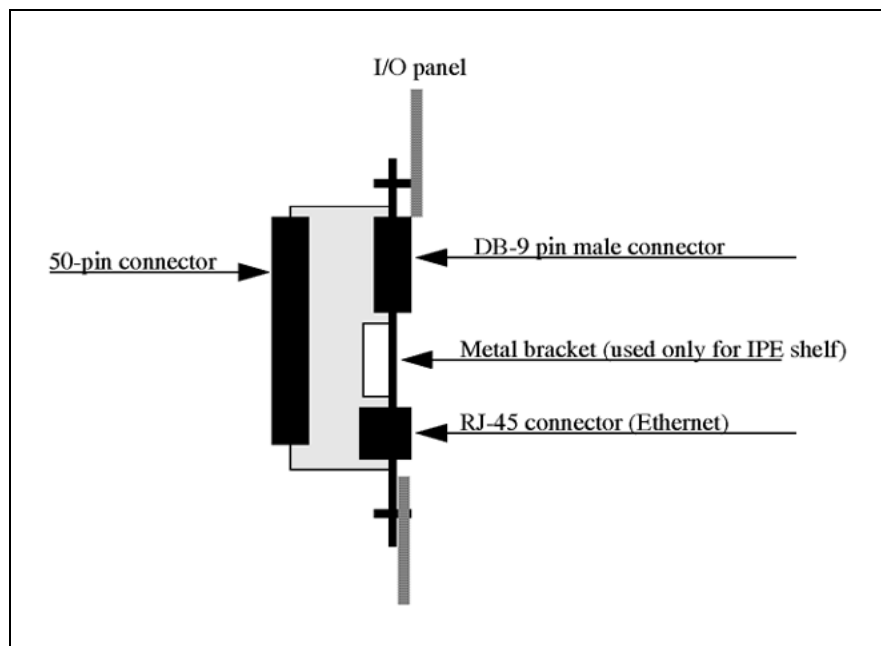
Figure 5 NT5D52AC Ethernet adapter
