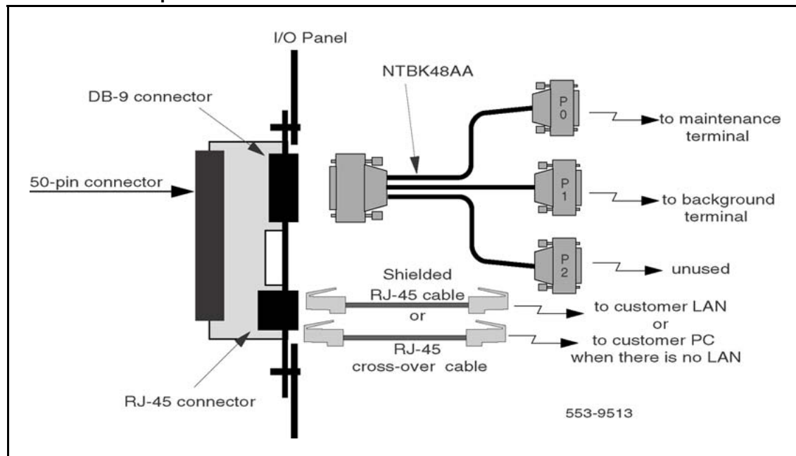
Figure 6 The Ethernet adapter and the NTBK48AA cable
