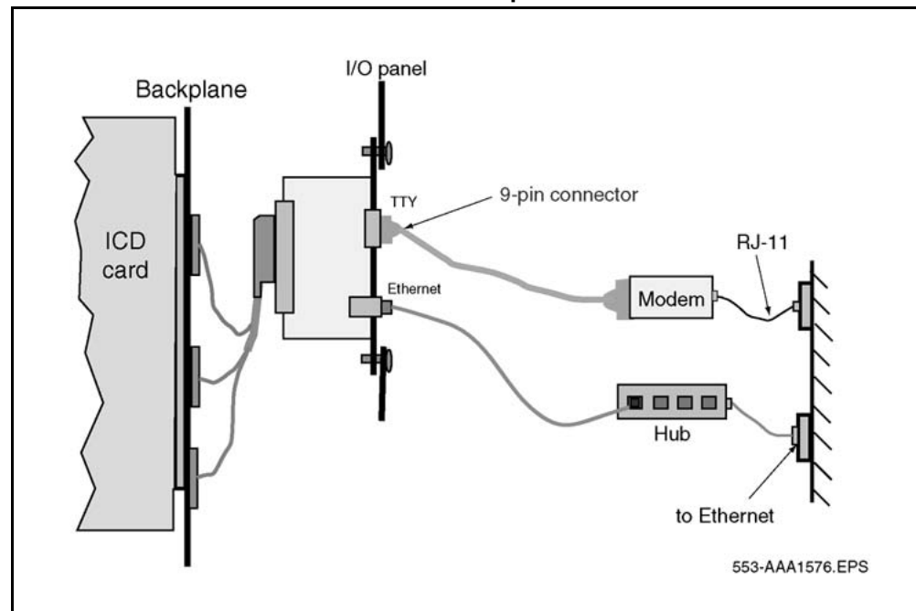
Figure 15 ICD modem and Ethernet connection example
