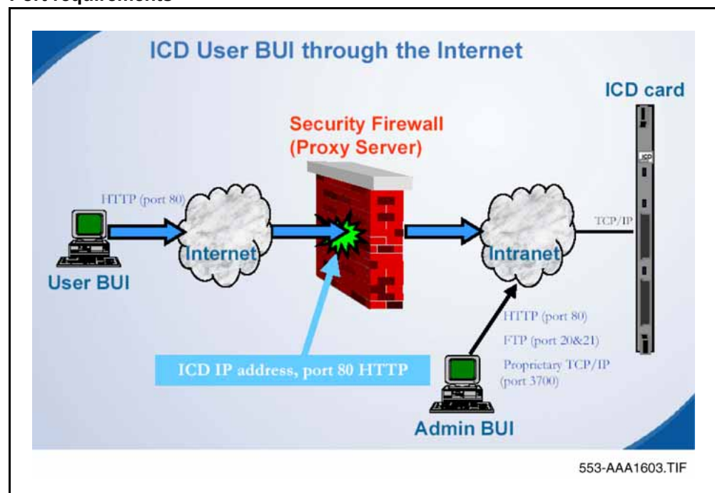
Figure 2 Port requirements
