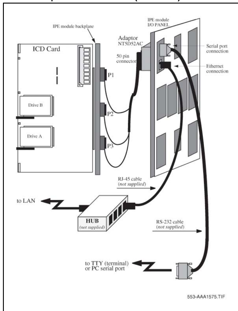
Figure 14 Ethernet adaptor in an IPE module (NT5D52AC)
