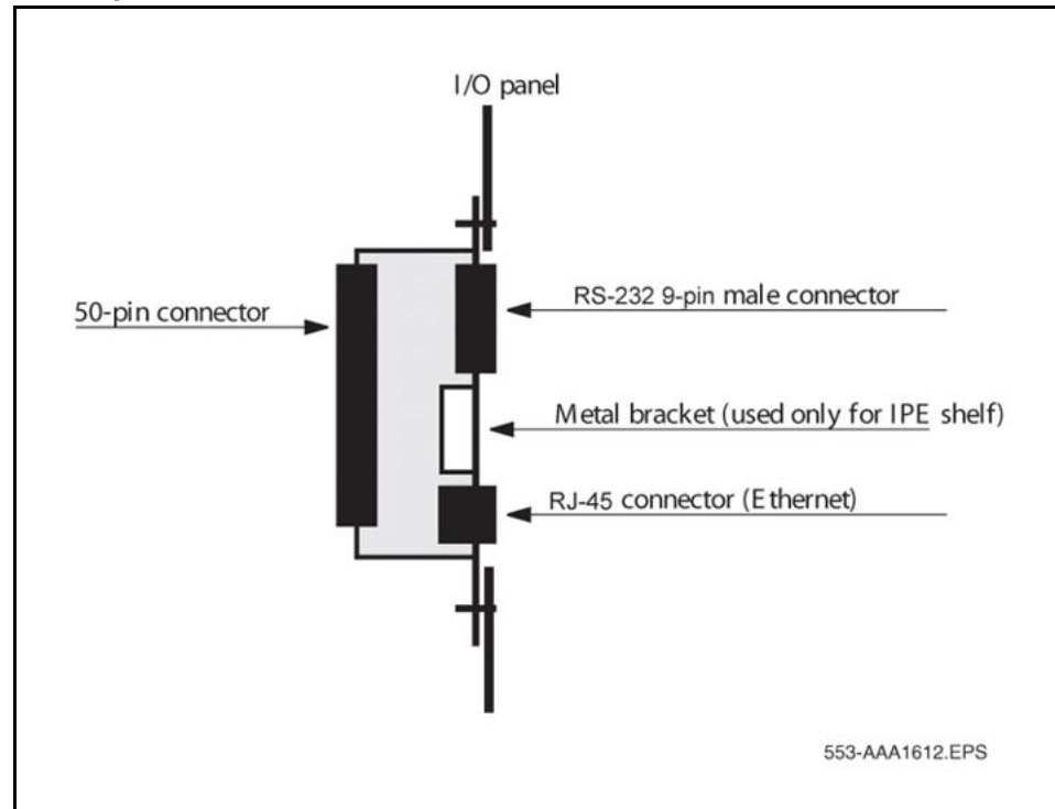
Figure 4 I/O adaptors
