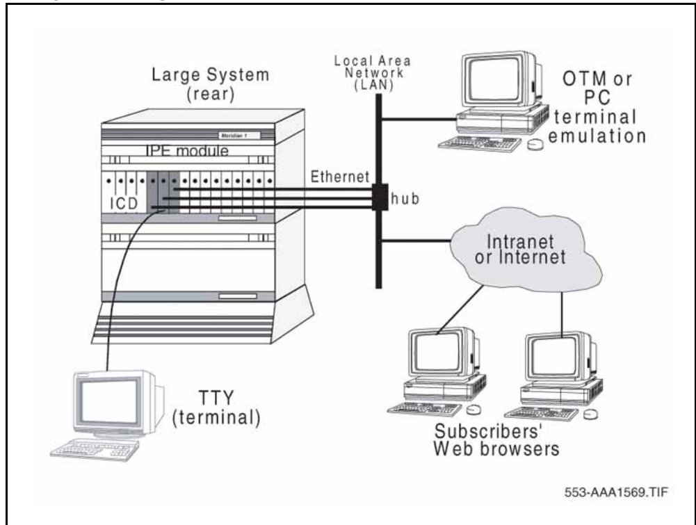
Figure 1 ICD system configuration
