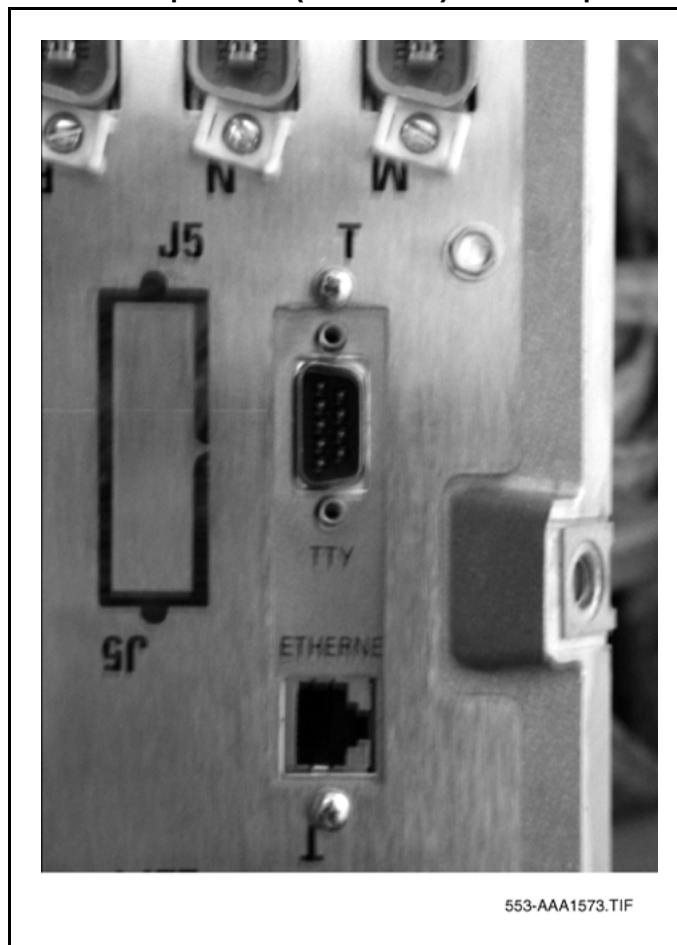
Figure 12 Ethernet adaptor card (NT5D52AC) in IPE I/O panel
