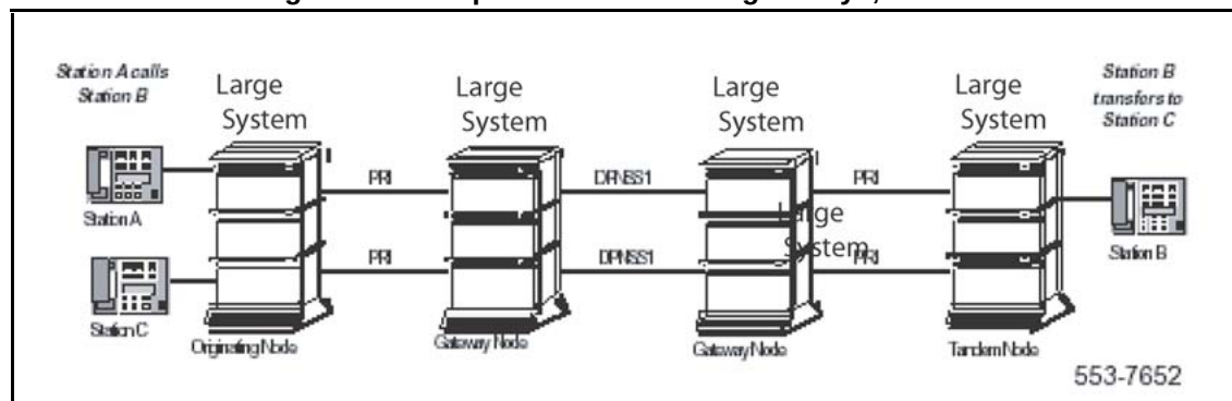
Figure 73 RO/TAT Interworking within multiple DPNSS1/MCDN gateways, before RO/TAT
