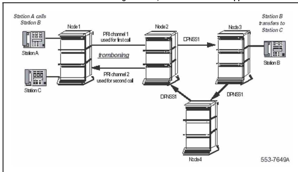
Figure 70 MCDN/DPNSS1 RO/TAT Interworking scenario, before RO has been applied
