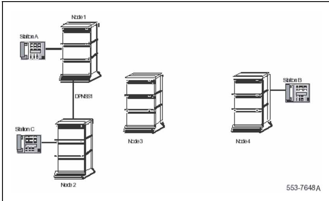
Figure 69 DPNSS1/MCDN RO/TAT Interworking scenario, after RO has been applied
