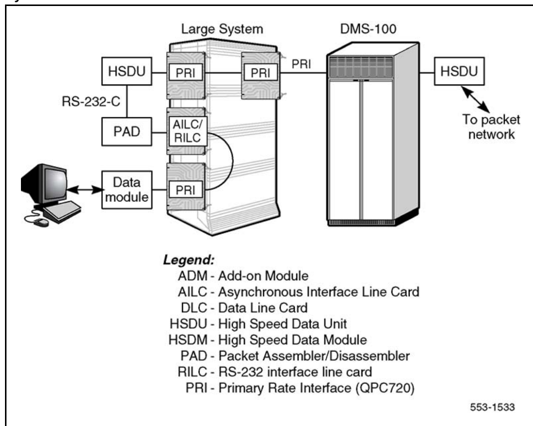
Figure 64 System PRI to DMS-100 Data Packet Network
