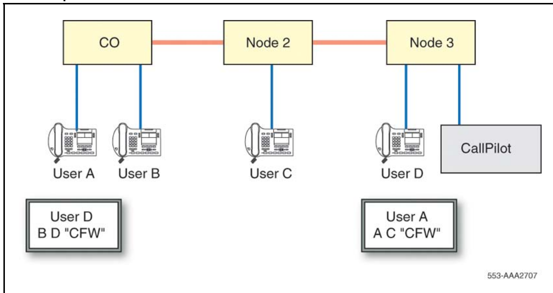
Figure 55 Feature operation with ARDN = RPO
