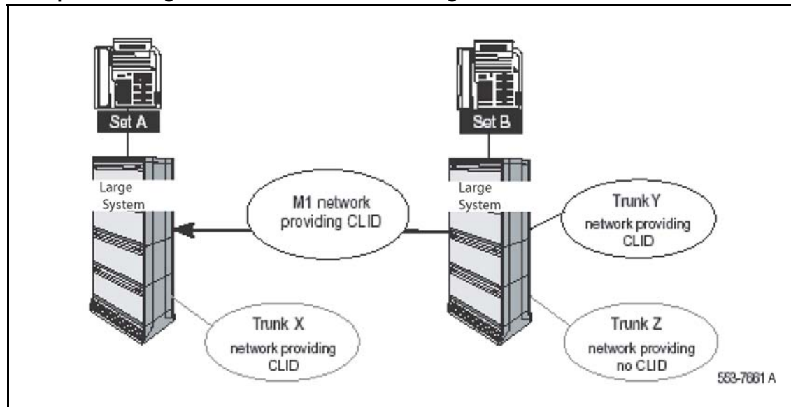
Figure 46 Example of Calling Line Identification for Incoming Calls
