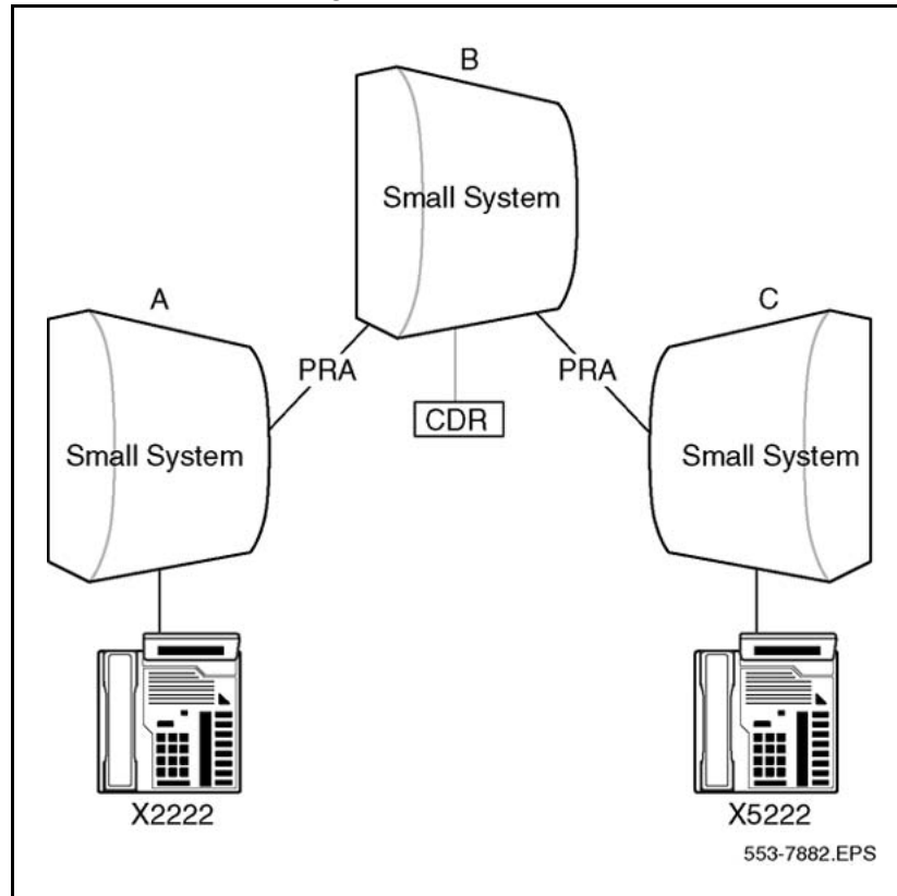
Figure 47 CDR in Multi-site Configuration
