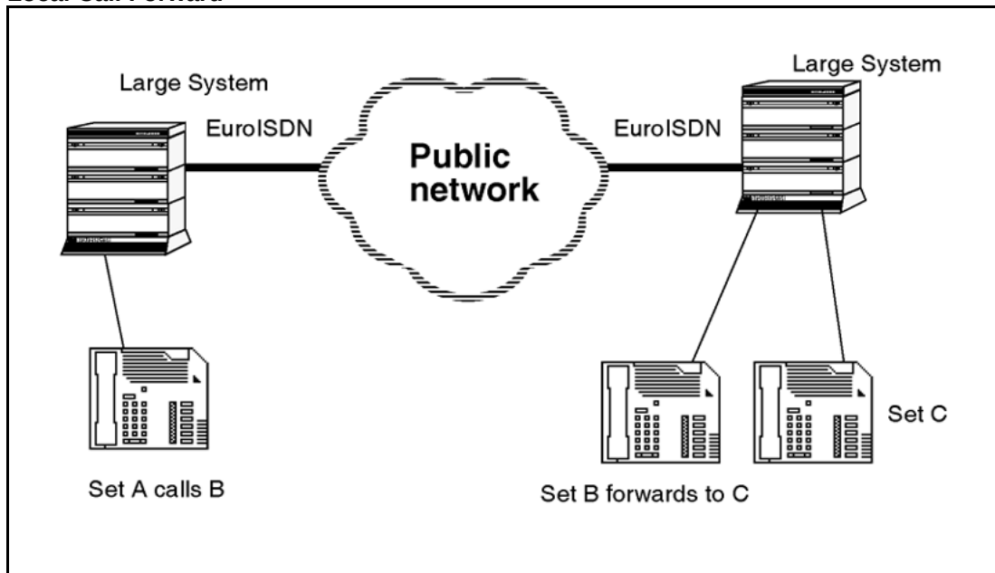
Figure 40 Local Call Forward
