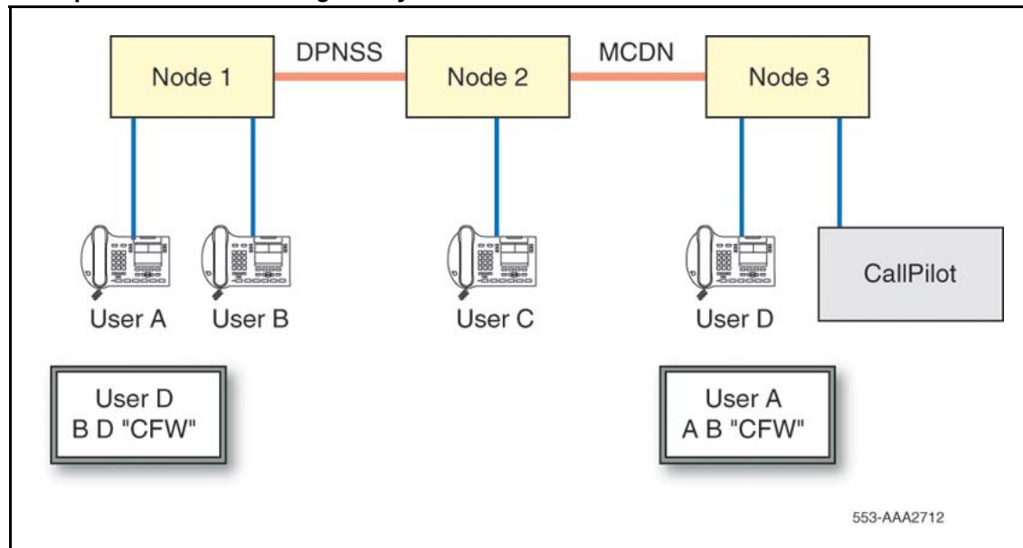
Figure 59 Example of DPNSS-MCDN gateway interaction with ARDN = RPO or NO
