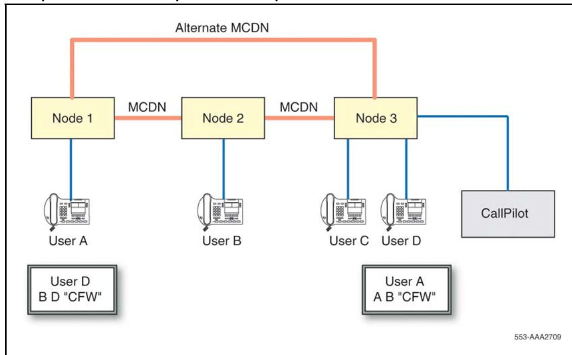
Figure 62 Example of Trunk Route Optimization in operation and ARDN = YES
