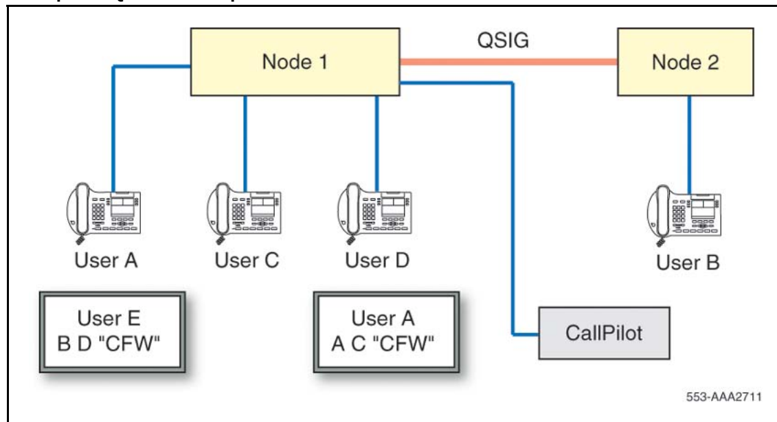
Figure 60 Example of QSIG Path Replacement interaction with ARDN= YES
