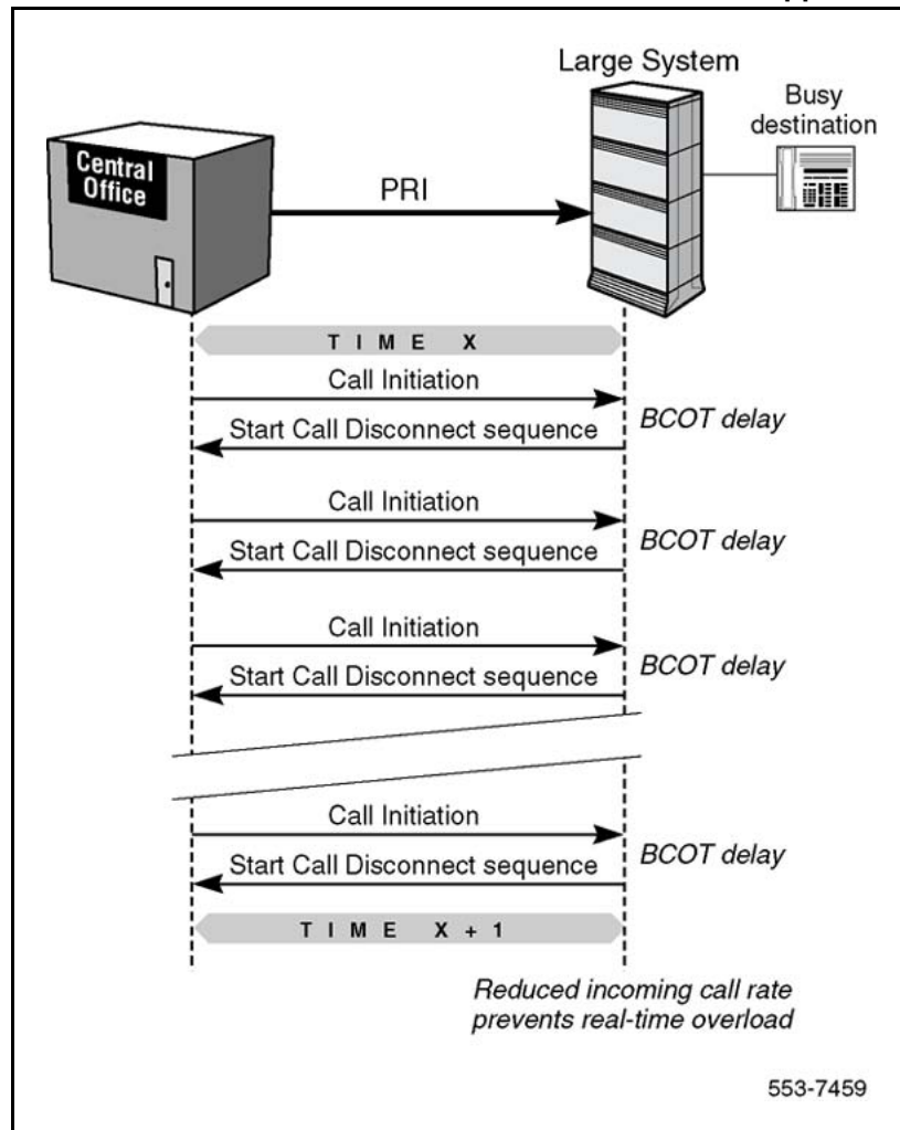
Figure 8 After the B-channel Overload Control Timer has been applied
