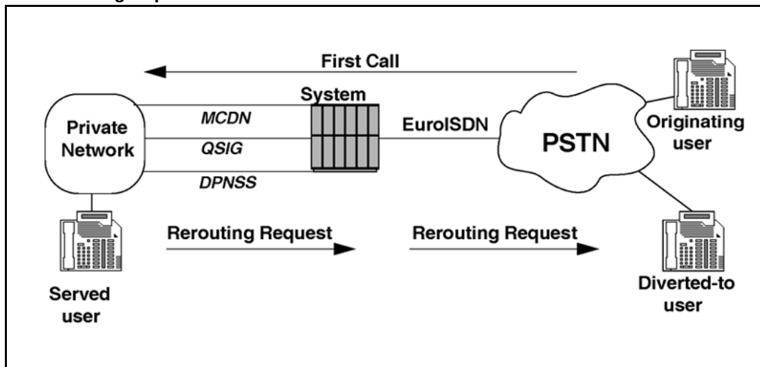
Figure 21 Call rerouting request sent to the CO.
