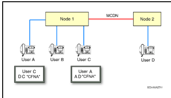
Figure 63 Example of TRO-BA in operation and ARDN = YES or NO
