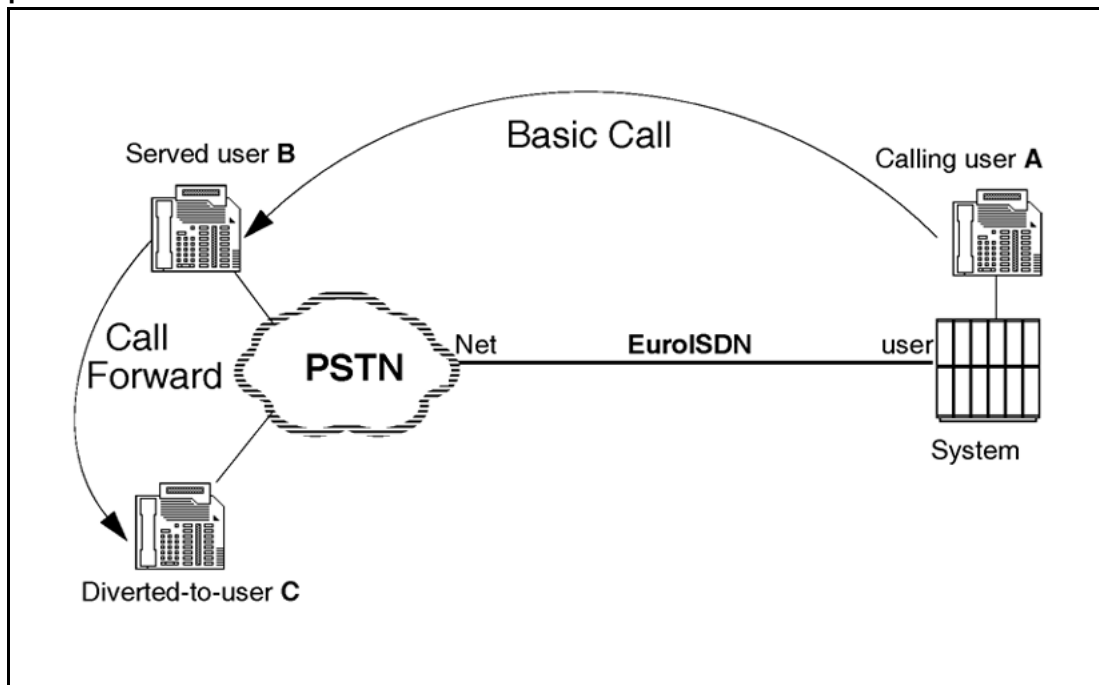
Figure 18 The calling user is on the system and the served user and the diverted-to-users are in the public network
