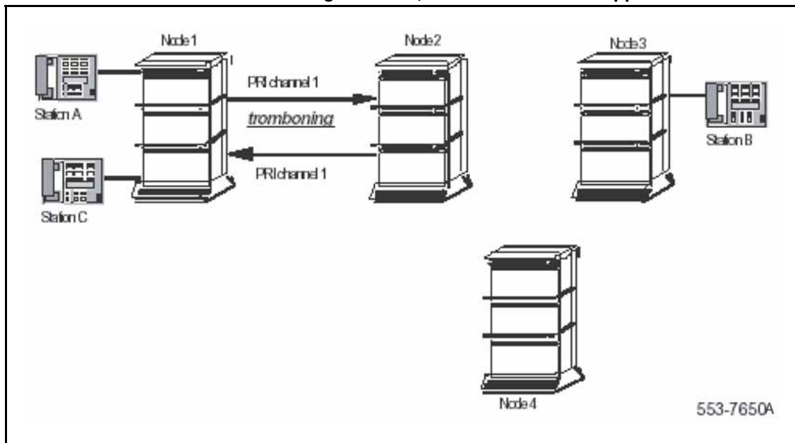
Figure 72 MCDN/DPNSS1 RO/TAT Interworking scenario, after TAT has been applied
