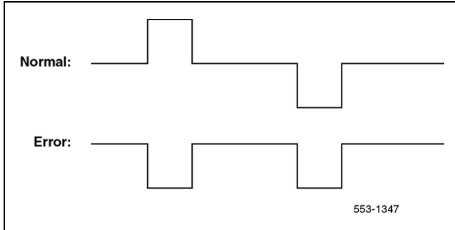
Figure 1 Bipolar violations
