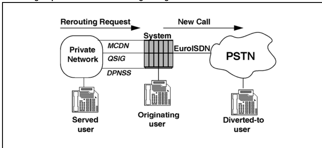
Figure 20 Rerouting request received at the originating node.
