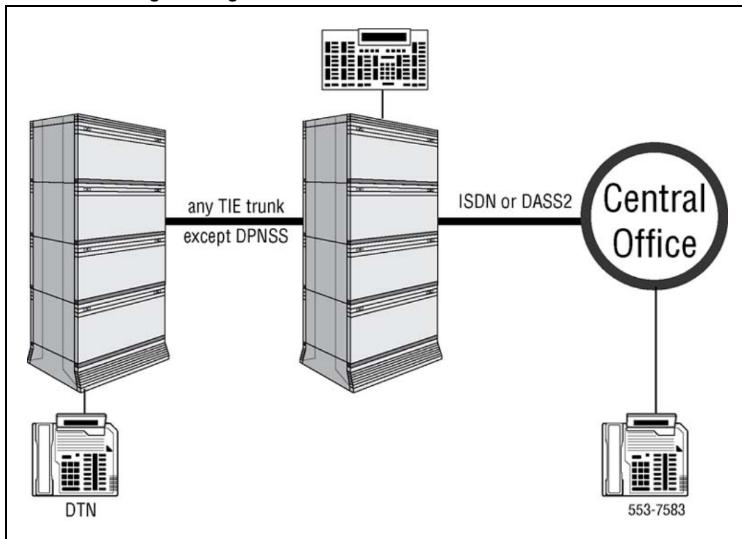
Figure 6 Attendant Through Dialing Networkwide
