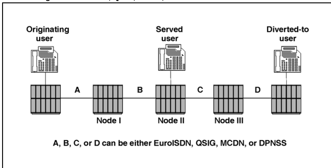
Figure 19 Interworking with EuroISDN, QSIG, MCDN, or DPNSS
