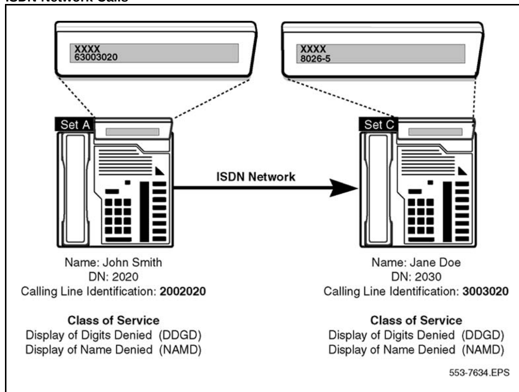
Figure 66 ISDN Network Calls
