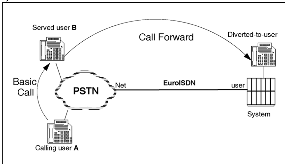
Figure 16 The calling and served users are in the public network and the diverted-to-user is on the system
