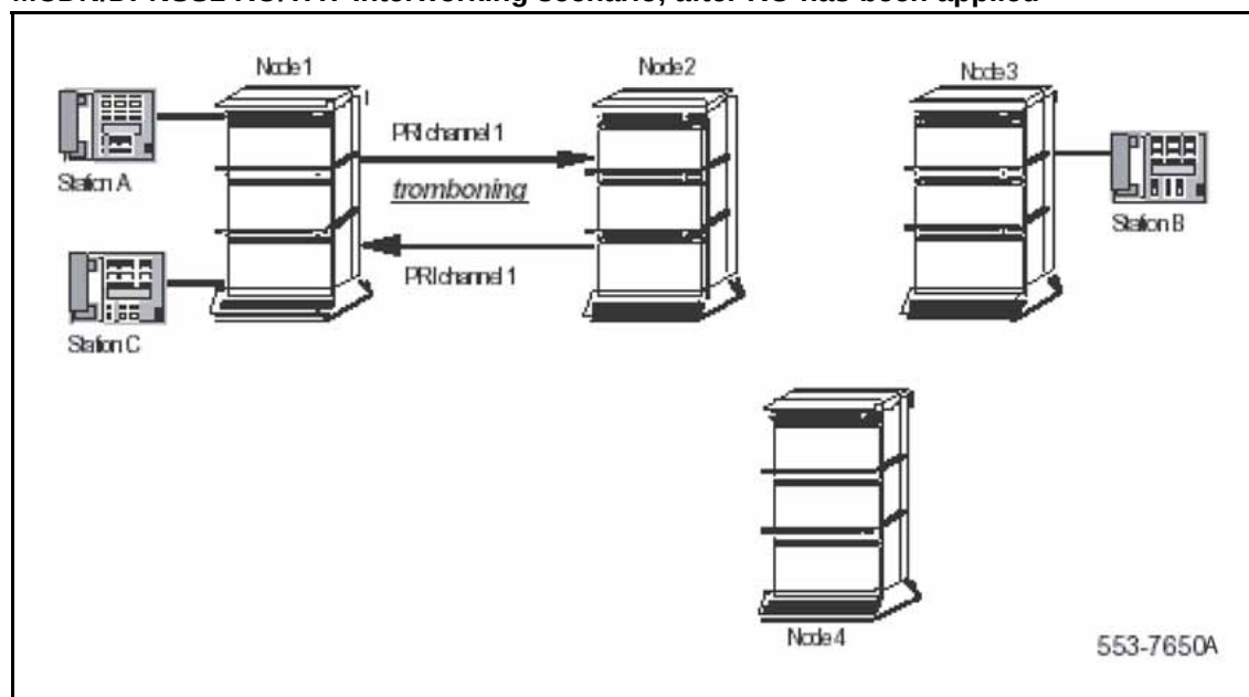
Figure 71 MCDN/DPNSS1 RO/TAT Interworking scenario, after RO has been applied
