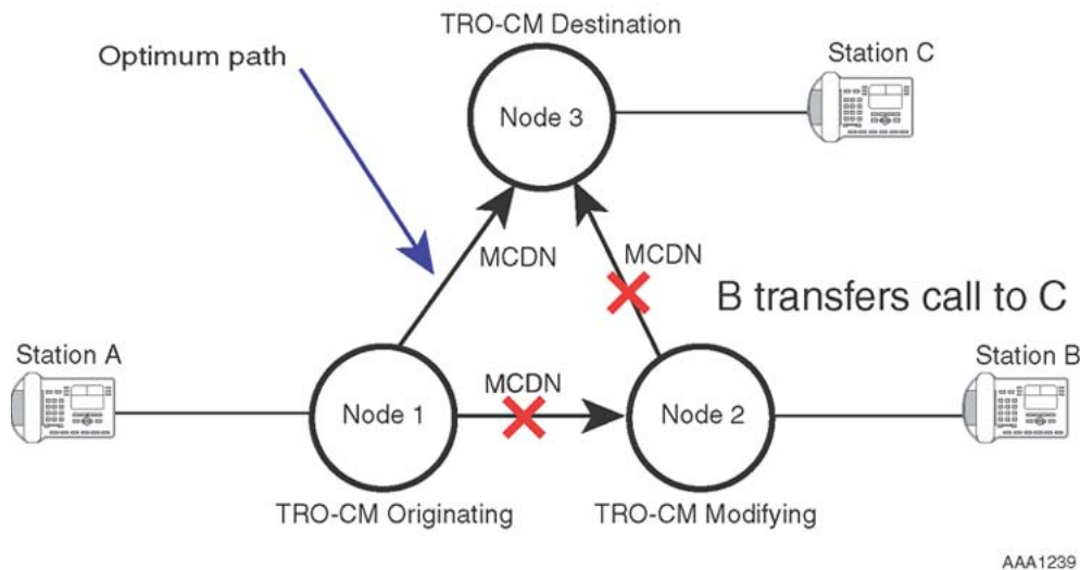
Figure 72: TRO-CM basic operation
