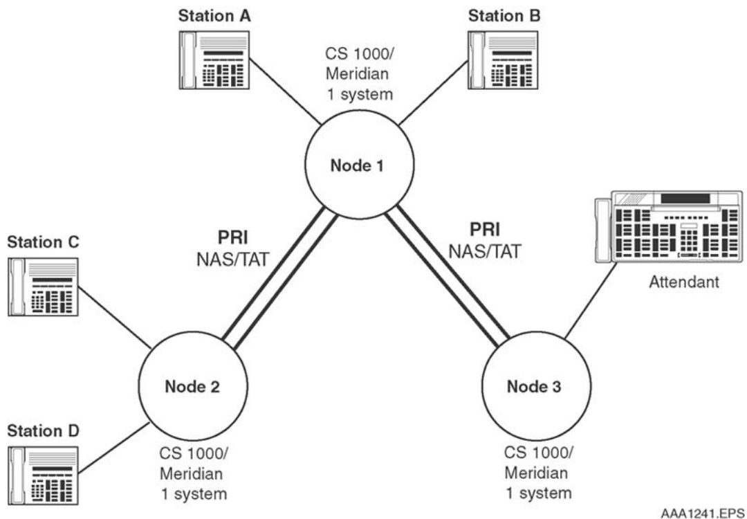
Figure 103: NAS and TAT interworking
