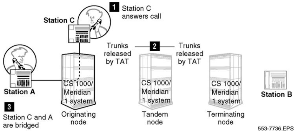
Figure 82: Results of anti-tromboning for Network Call Transfer - system/system
