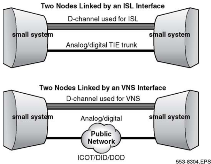
Figure 120: VNS Interface/ISL Interface Comparison
