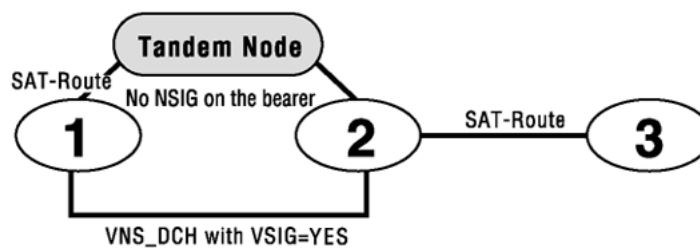
Figure 35: SAT-count is not updated when NSIG is not configured on the bearer (VSIG = YES and SIGO is set to STD)
