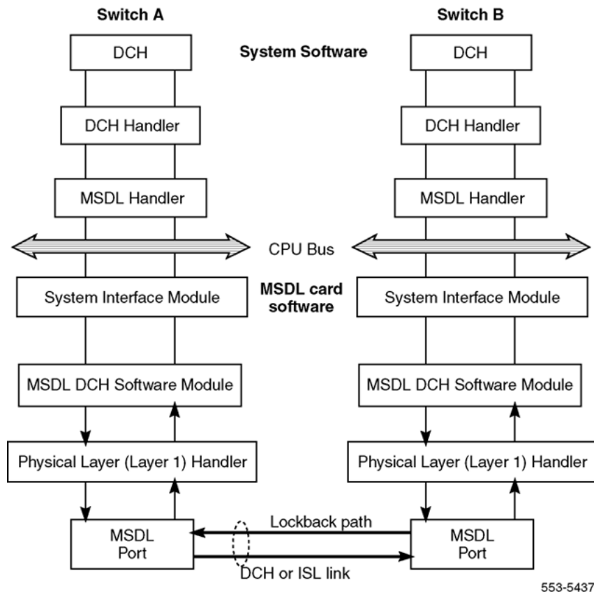
Figure 133: Remote loopback tests (NT6D80)
