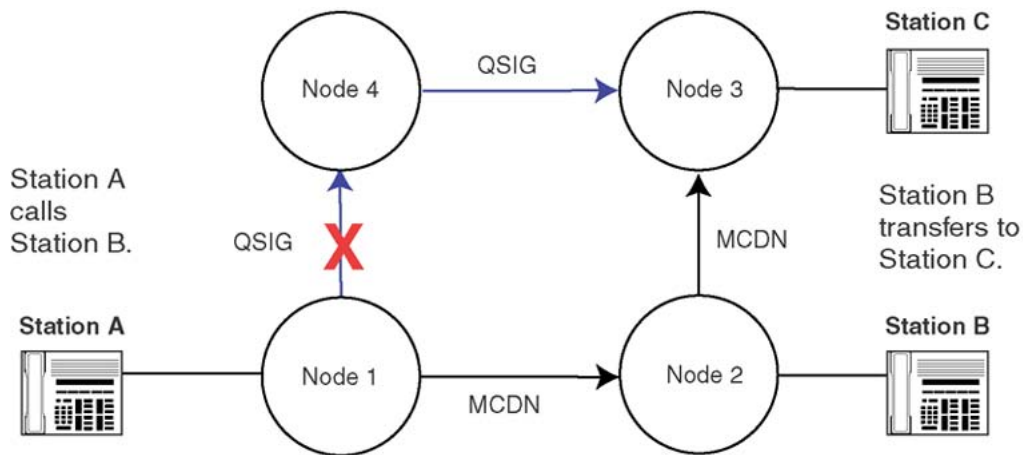
Figure 91: TRO-CM fails when the optimum path is not an MCDN trunk
