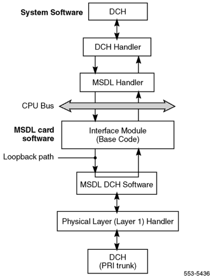
Figure 132: Local loopback test (NT6D80)
