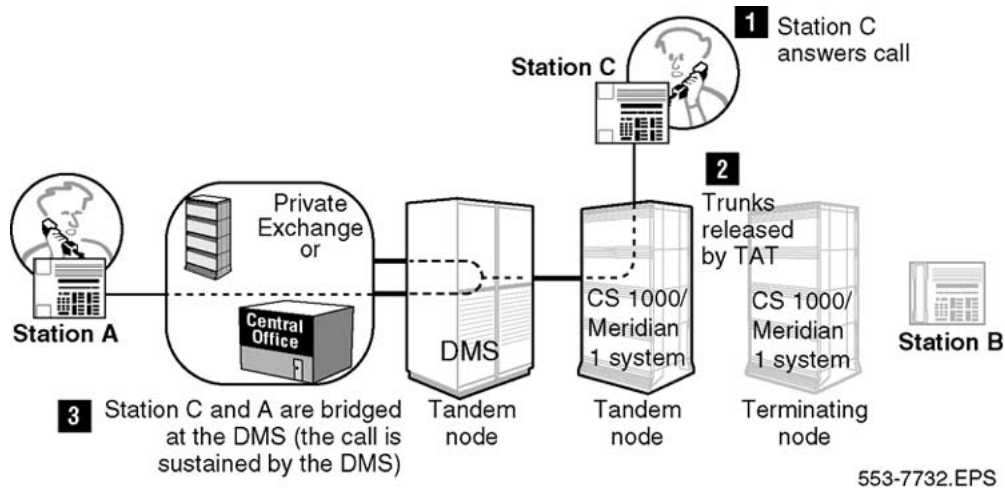
Figure 78: Results of anti-tromboning for NCRD (case 2) - system interworking with DMS
