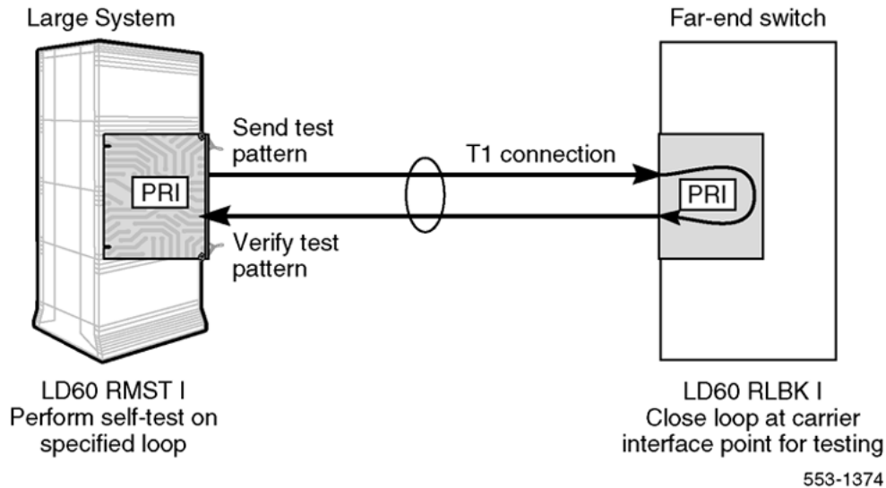
Figure 129: PRI remote loop-back and link diagnostic tests
