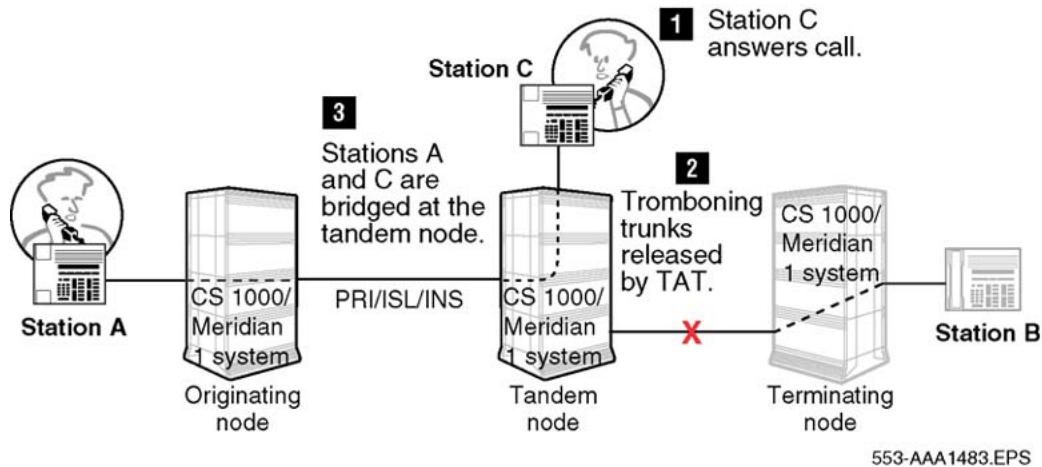
Figure 107: NCRD after TAT
