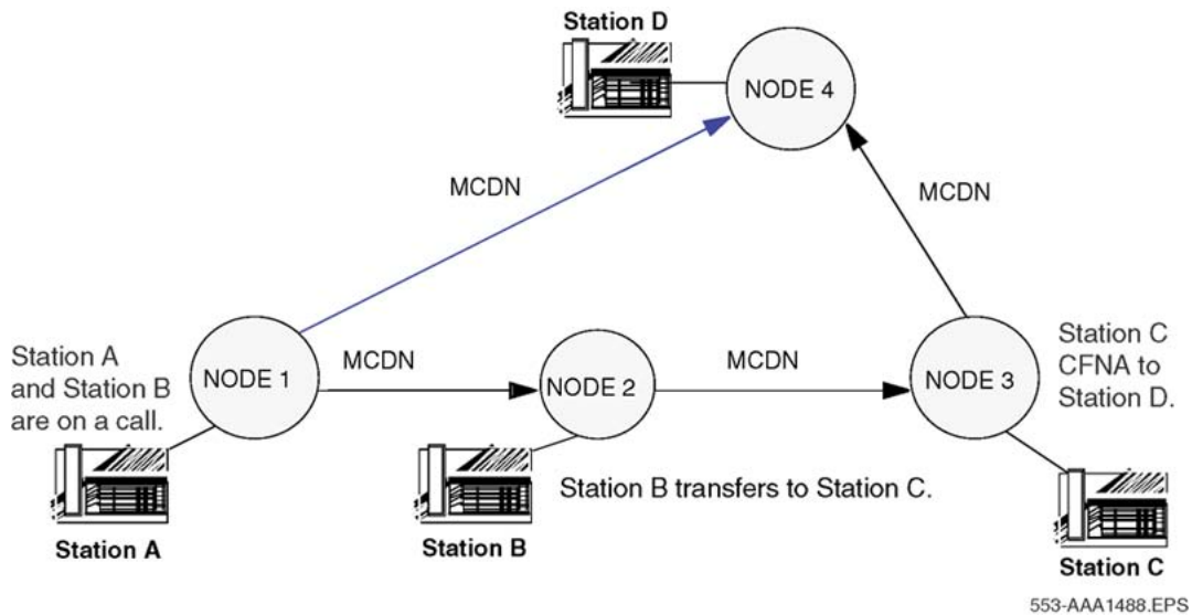
Figure 114: Supervised transfer followed by CFNA
