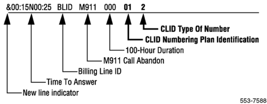
Figure 46: Third line format for CDR ticket
