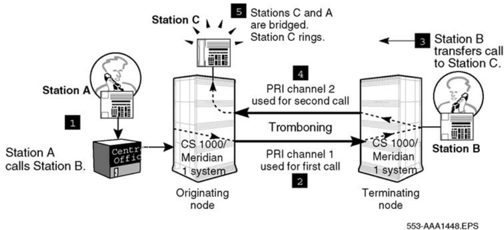
Figure 59: Prior to Trunk Anti-Tromboning operation
