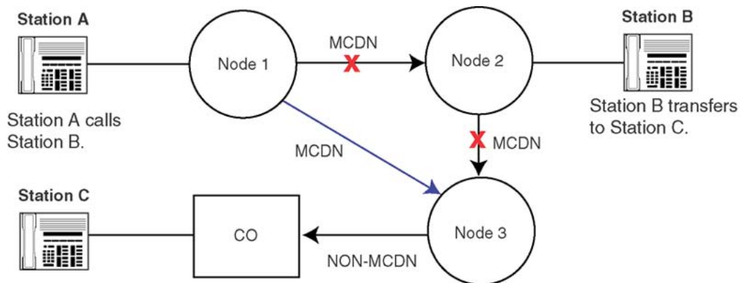
Figure 88: TRO-CM successful at an interworking node
