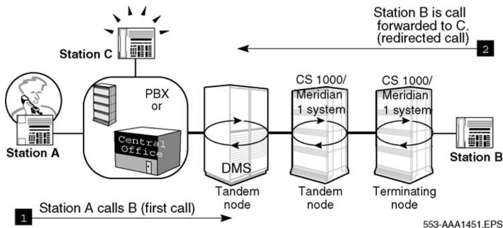
Figure 75: Anti-Tromboning for NCRD (case 1), PBX/DMS
