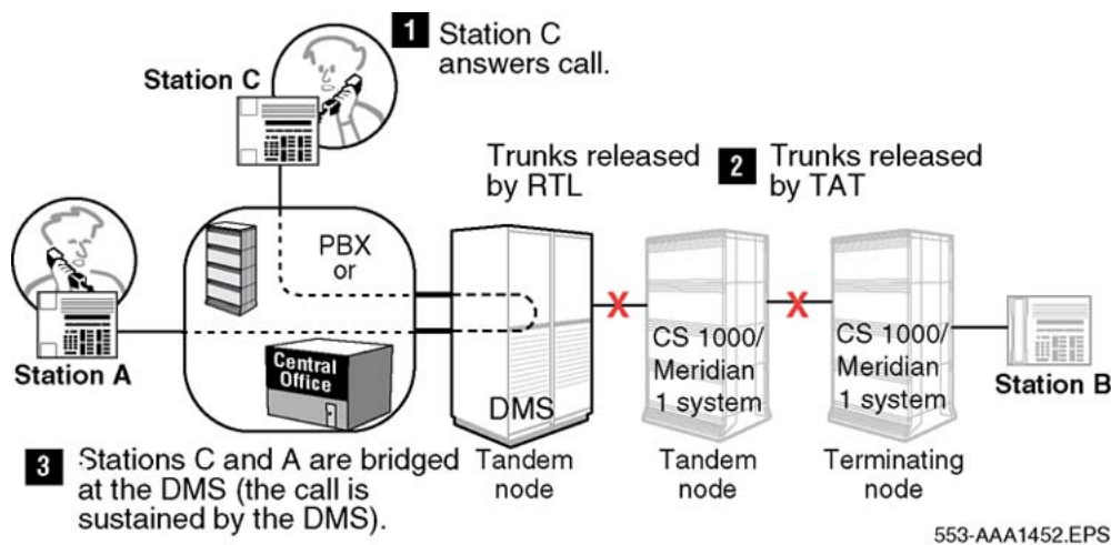
Figure 76: Results of anti-tromboning for NCRD (case 1), PBX/DMS
