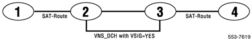
Figure 33: A scenario involving two SAT-Routes where VSIG = YES and SIGO is set to STD
