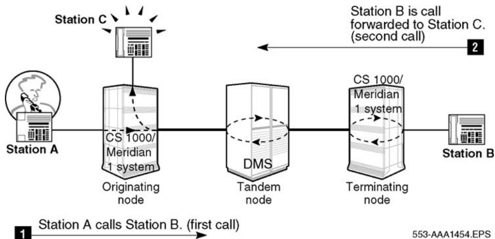
Figure 79: Anti-tromboning for Call Modification - DMS/System
