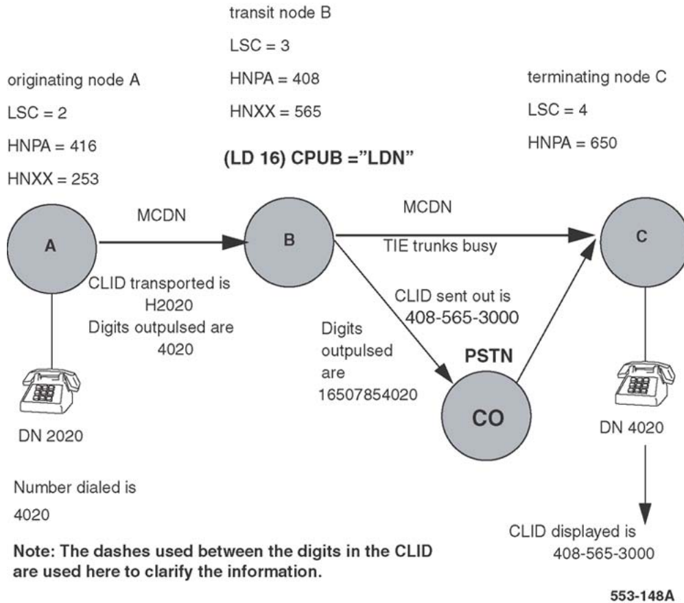
Figure 53: Private network to Public network hopoff, LDN conversion functionality for CDP dialing
