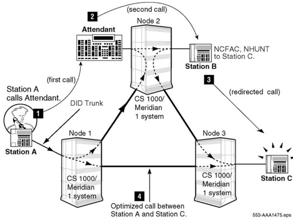
Figure 93: Attendant extended call
