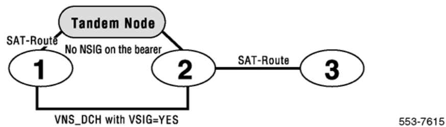
Figure 29: A scenario involving two SAT-Routes where VSIG = NO and SIGO is not set to STD
