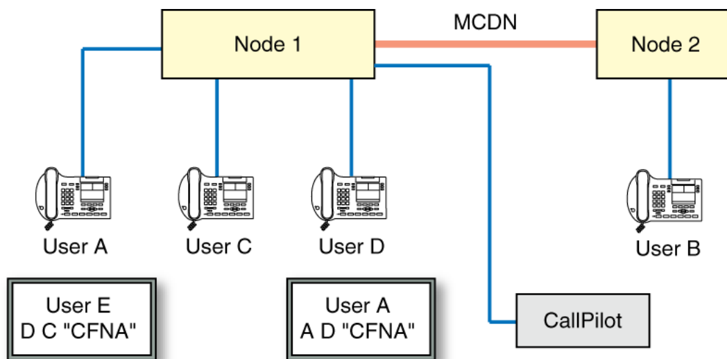
Figure 118: Example of TRO-BA in operation when ARDN = YES or NO
