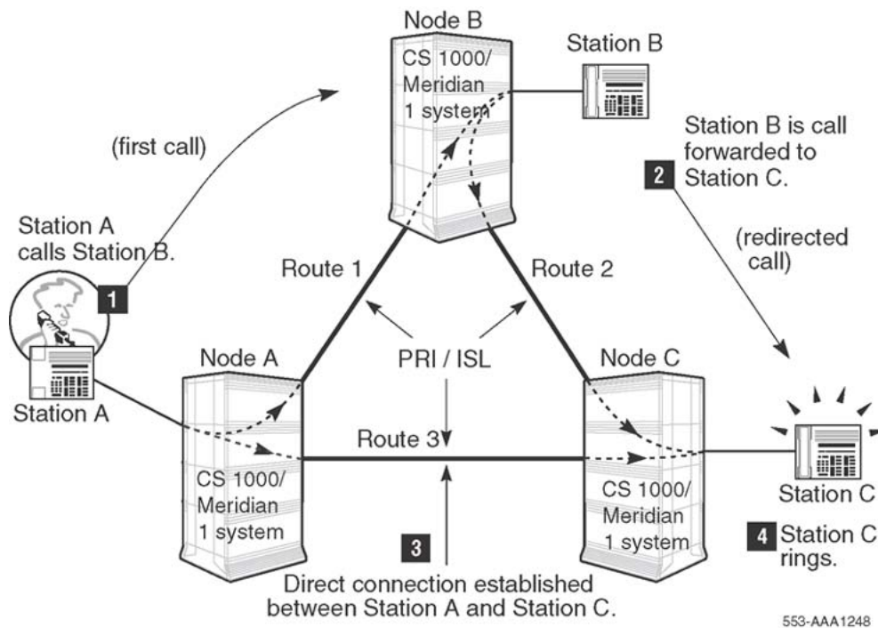
Figure 57: Example of TRO-BA when NCRD is enabled on each node
