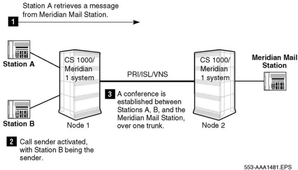
Figure 102: Call Sender operation with Network Message Services active
