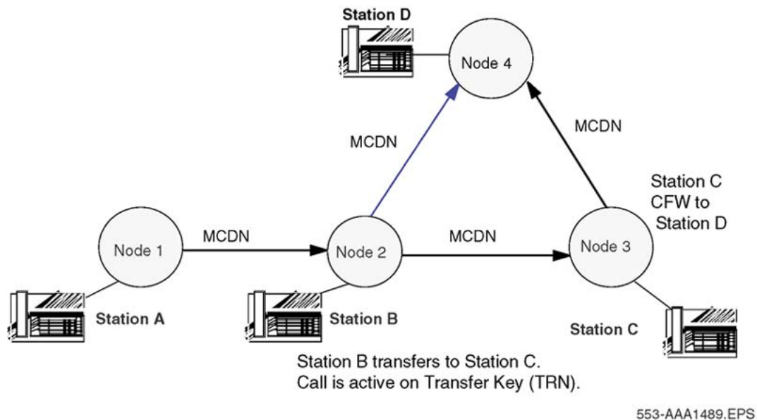
Figure 115: Trunk Route Optimization before transfer
