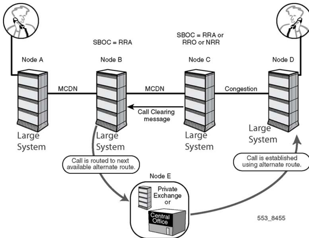
Figure 2: Transit node RRA operation
