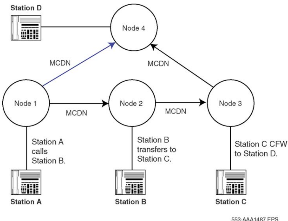
Figure 113: Trunk Route Optimization after transfer
