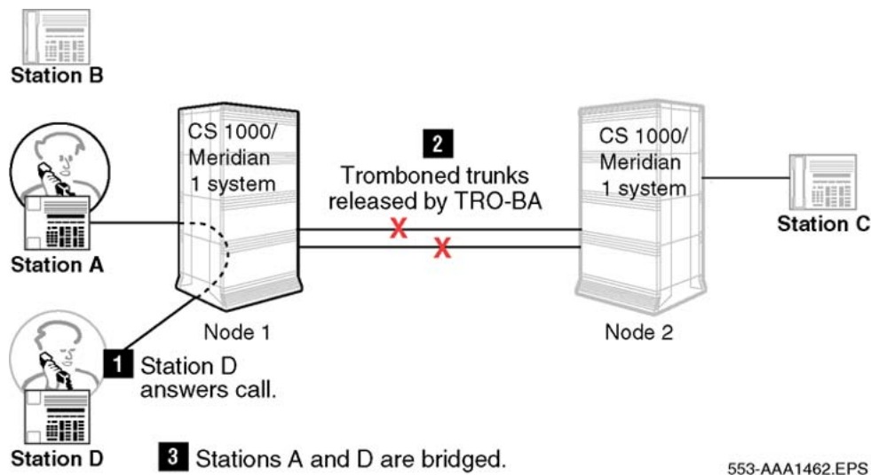
Figure 67: Tromboned trunks released by TAT
