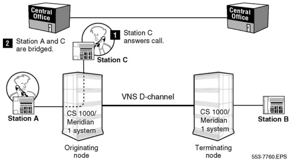
Figure 108: VNS before TAT
