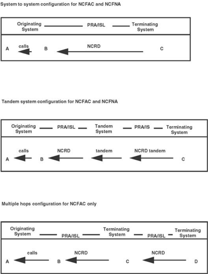
Figure 18: Network configurations for NCFAC and NCFNA
