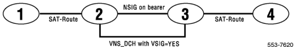
Figure 31: A scenario involving two SAT-Routes where VSIG = YES and SIGO is not set to STD
