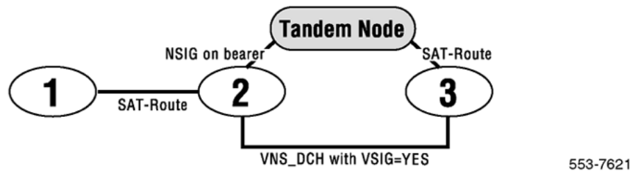
Figure 32: A scenario involving two SAT-Routes where VSIG = YES and SIGO is not set to STD
