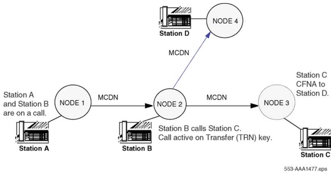
Figure 96: TRO-BA on TRN key
