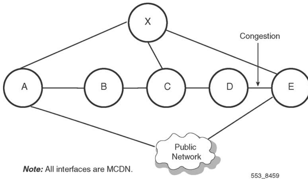
Figure 4: Example of multi node network
