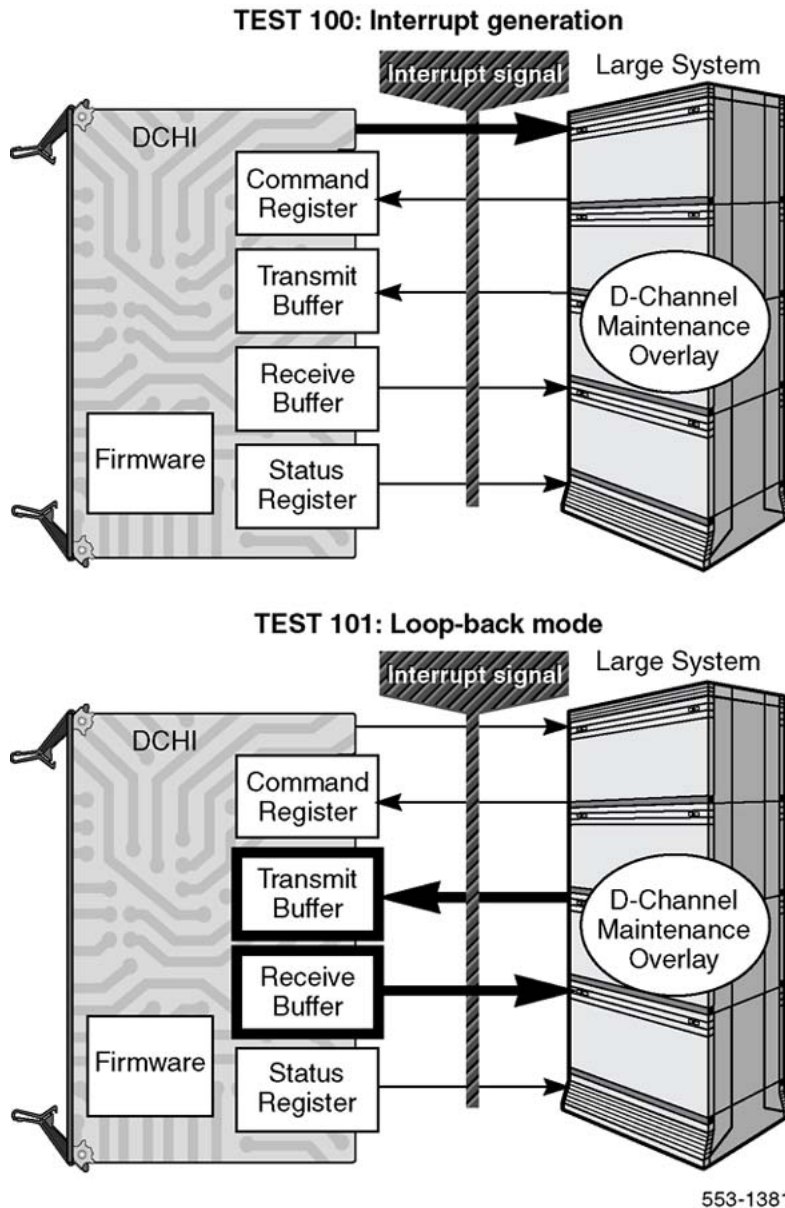
Figure 130: DCH tests 100 and 101
