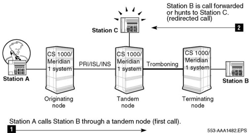
Figure 106: NCRD before TAT
