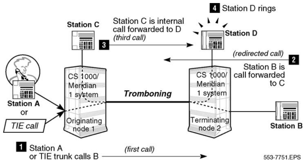
Figure 100: Internal Call Forward before TAT
