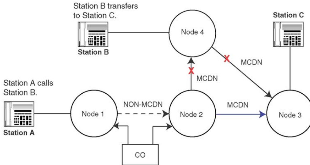
Figure 88: TRO-CM successful at an interworking node
