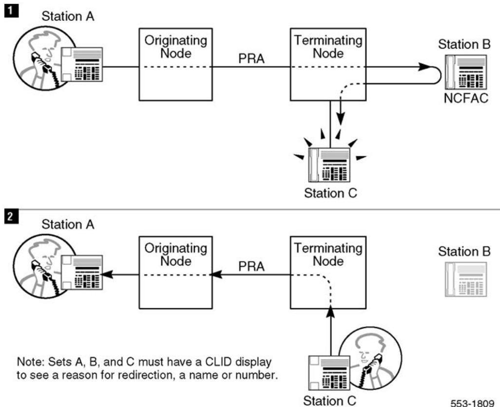
Figure 23: NCFAC intranode redirection
