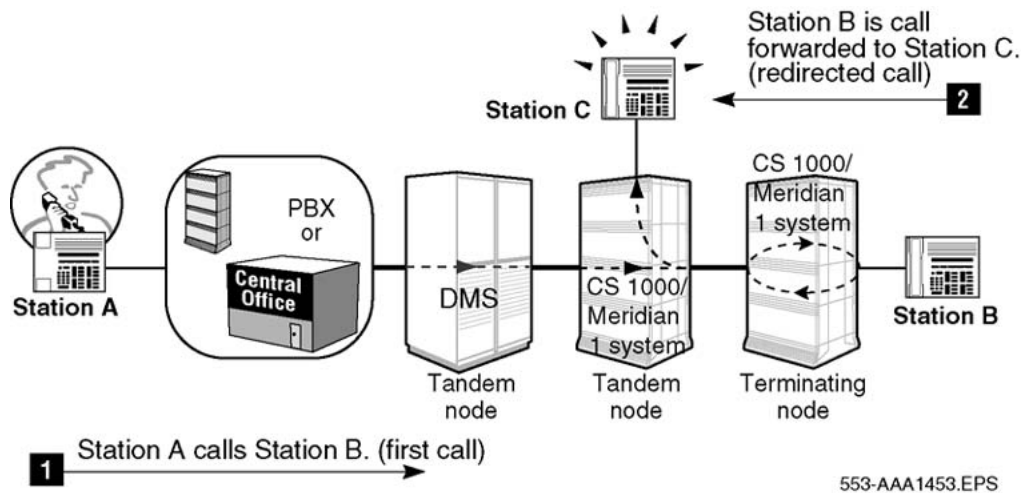
Figure 77: Anti-tromboning for NCRD (case 2), system/DMS
