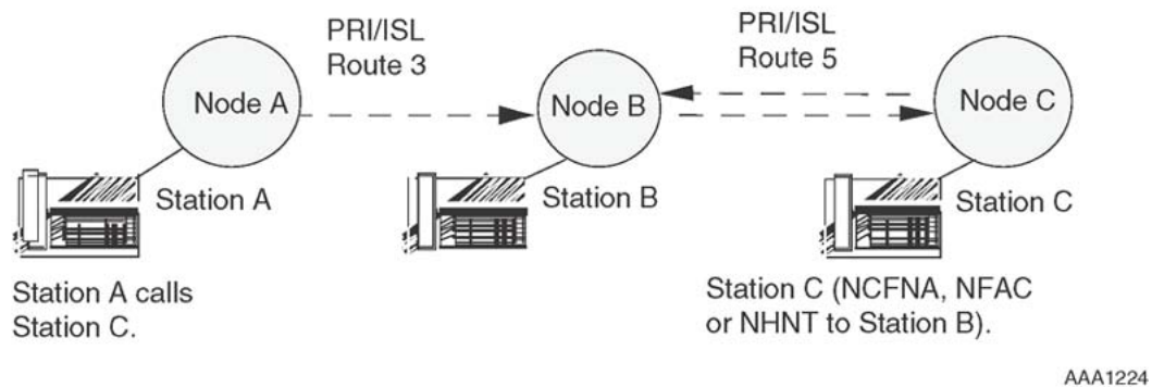
Figure 58: Example 2 of TRO-BA when NCRD is enabled on each node
