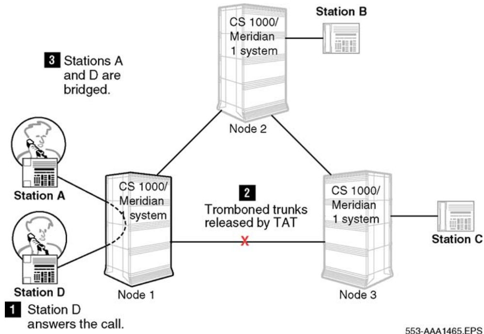
Figure 71: Tromboned trunks released by TAT
