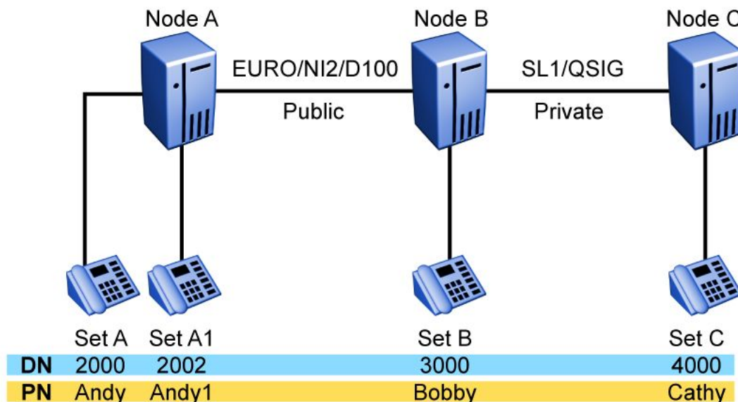
Figure 135: Name display for CFNA over public-private network with EURO interface
