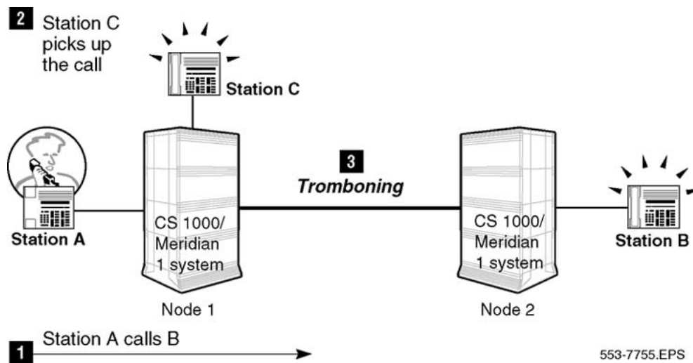
Figure 104: Network Call Pickup before TAT
