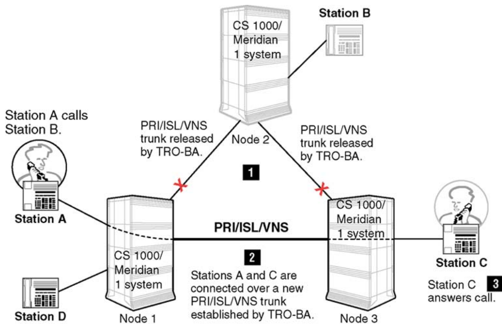
Figure 69: Call path after TRO-BA is applied
