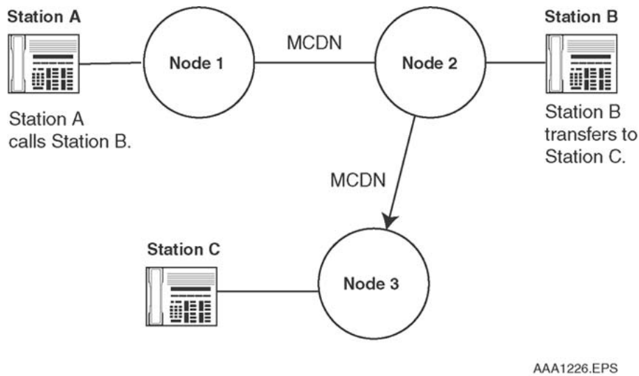
Figure 111: Before TRO-CM operation
