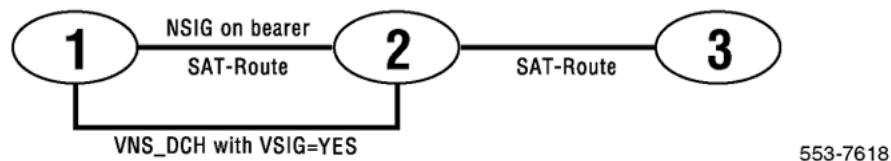
Figure 30: A scenario involving two SAT-Routes where VSIG = YES and SIGO is not set to STD
