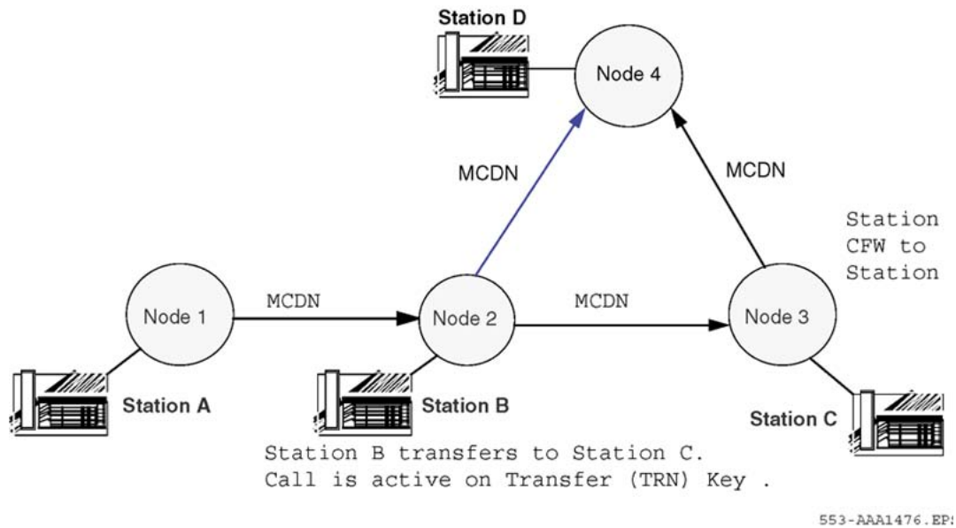
Figure 95: Trunk Route Optimization before transfer
