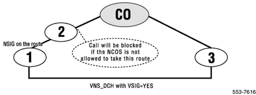
Figure 36: A scenario where the call is blocked, as NCOS is insufficient (VSIG = YES and SIGO is not set to STD)
