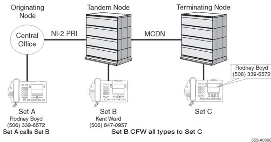
Figure 42: Call Forward (all types) in a networking environment
