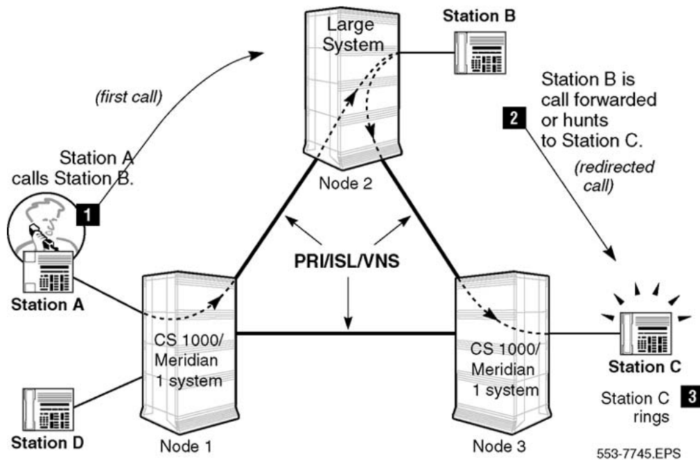
Figure 68: Call path before TRO-BA is applied
