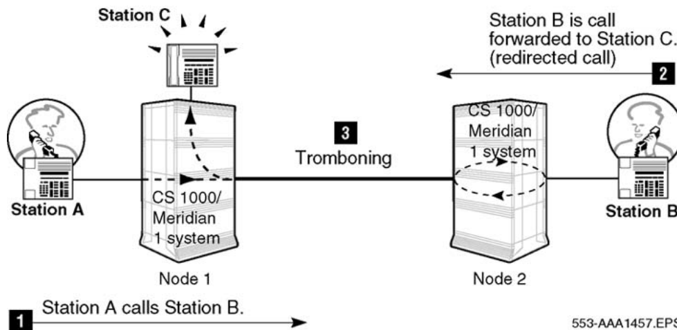
Figure 61: TRO-BA and TAT operating together before optimization in a Call Forward scenario
