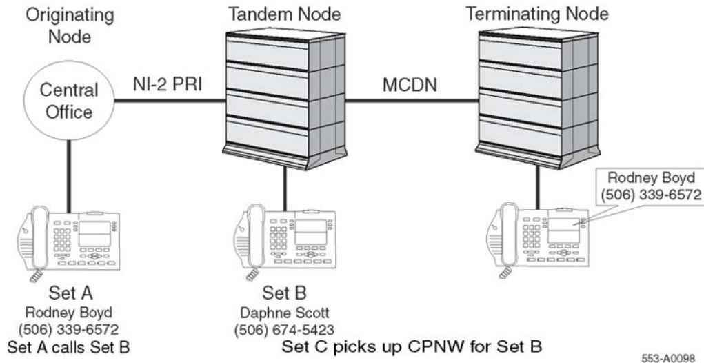
Figure 44: Call Pickup Network Wide
