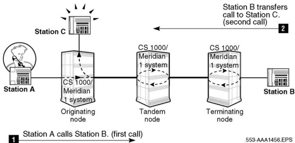
Figure 81: Anti-tromboning for Network Call Transfer - system/system
