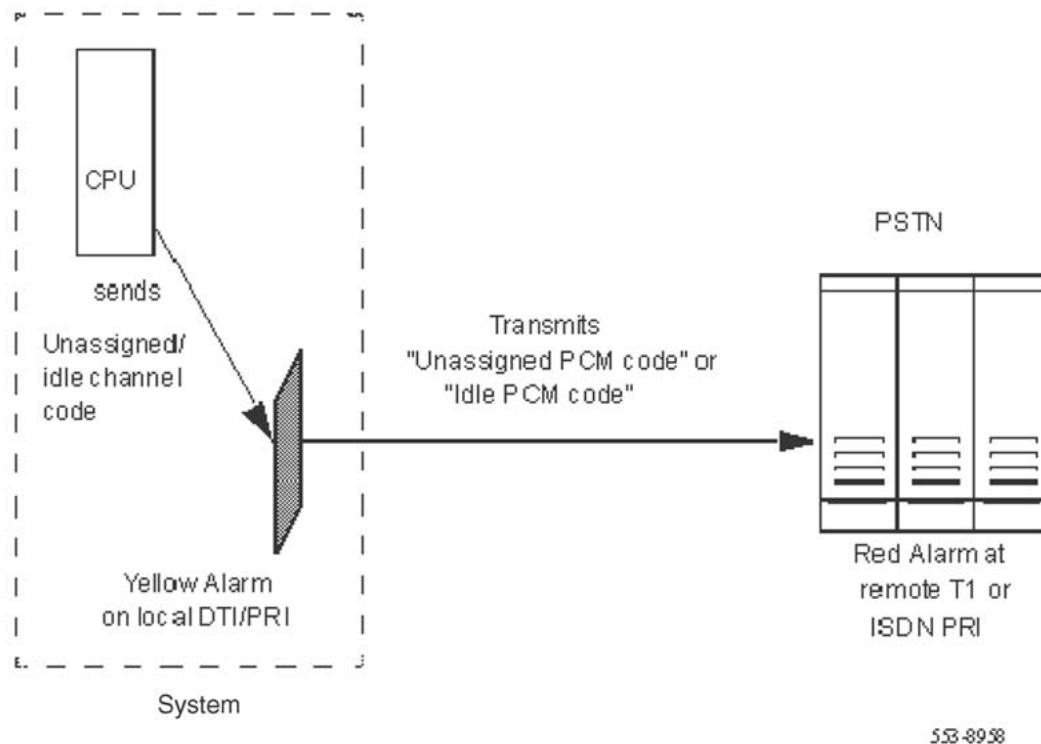
Figure 11: System with Idle Code Selection feature responding to Yellow Alarm condition
