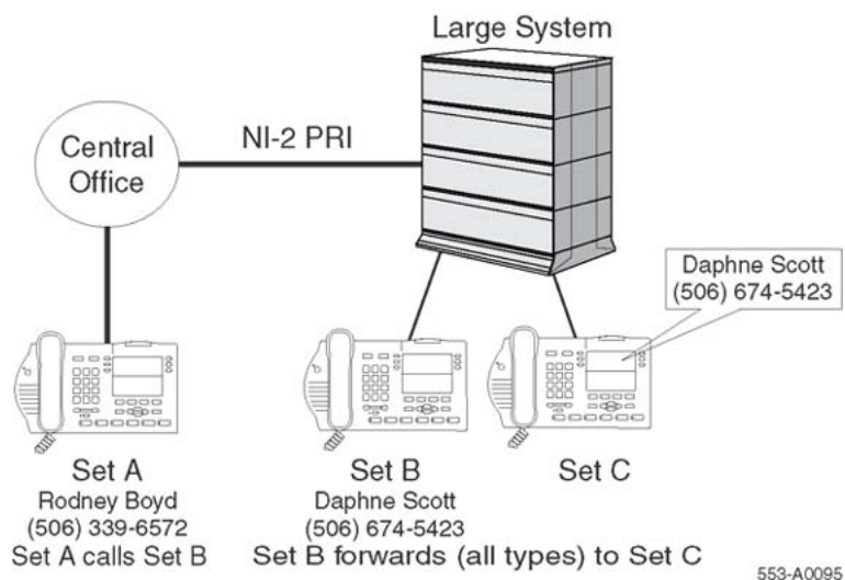
Figure 41: Call Forward (all types) in a stand-alone environment
