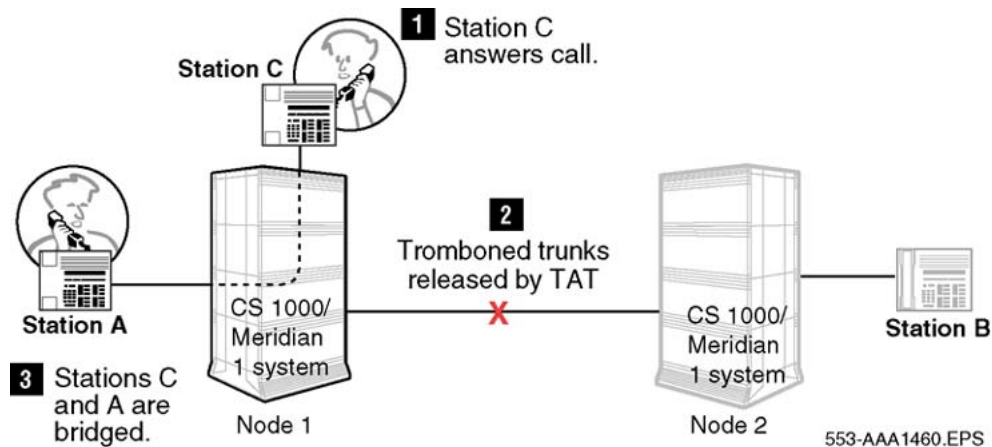
Figure 64: After TAT applied to tromboned trunks due to a call transfer
