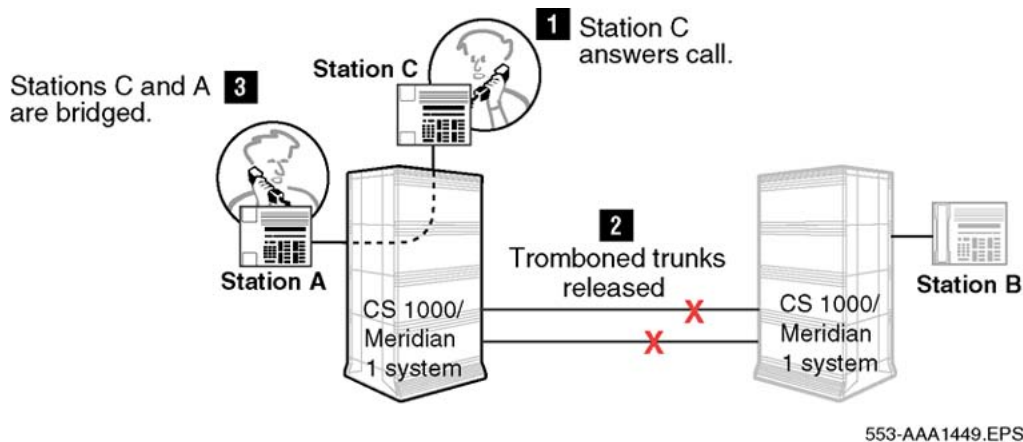
Figure 60: After Trunk Anti-Tromboning operation
