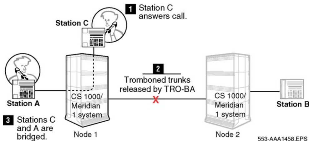
Figure 62: After TRO-BA applies optimization
