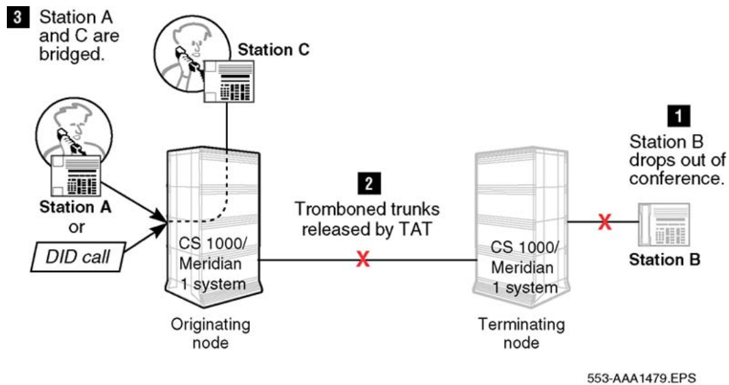
Figure 99: Conference call after TAT
