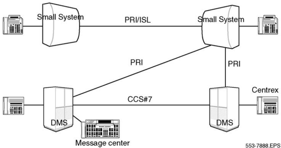
Figure 9: Private corporate network with DMS hosting the Message Center
