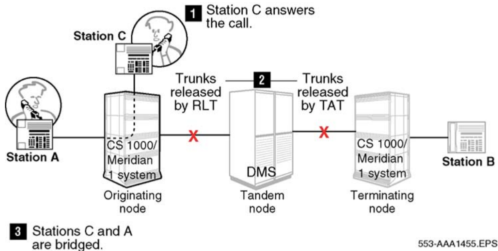
Figure 80: Results of anti-tromboning for Network Call Transfer - DMS/System
