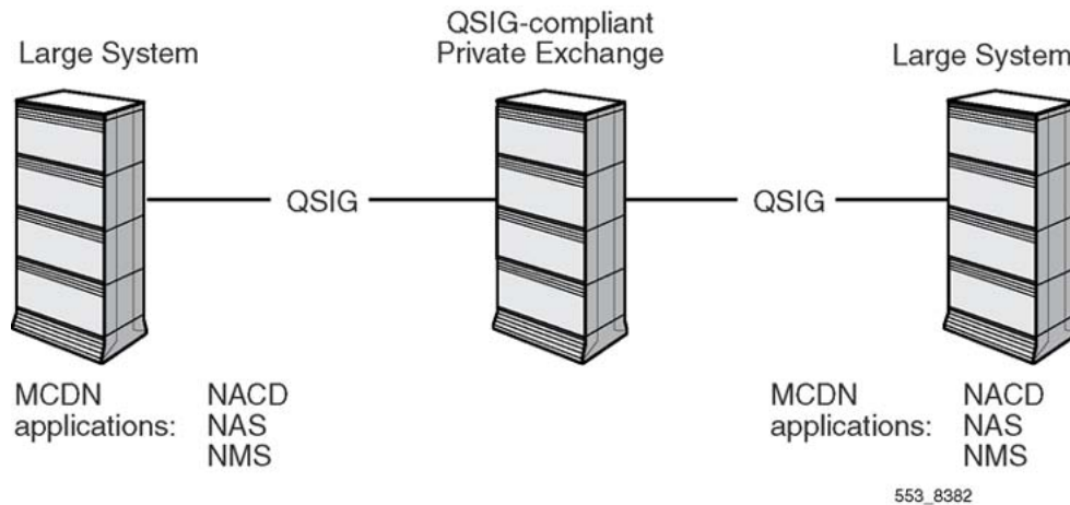
Figure 6: MCDN End-to-End Transparency
