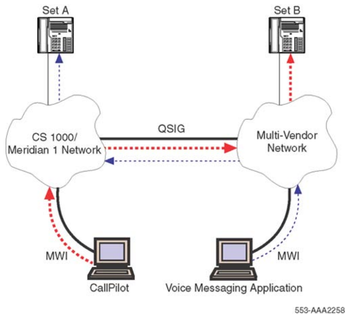
Figure 54: MWI message transport between a system network and a multi-vendor network
