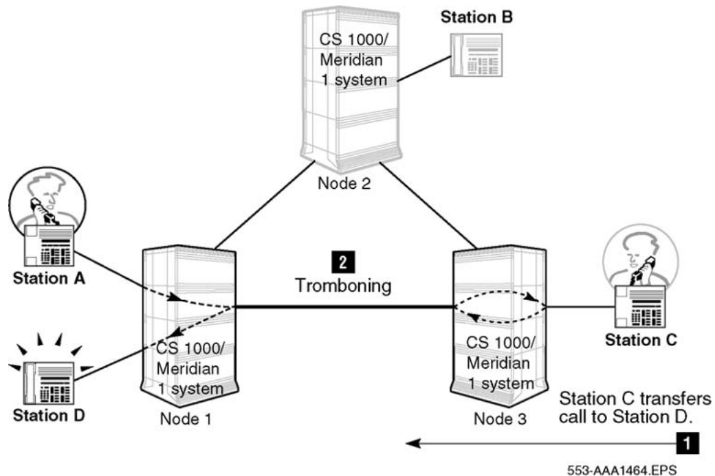
Figure 70: Tromboning of trunks after TRO-BA is applied
