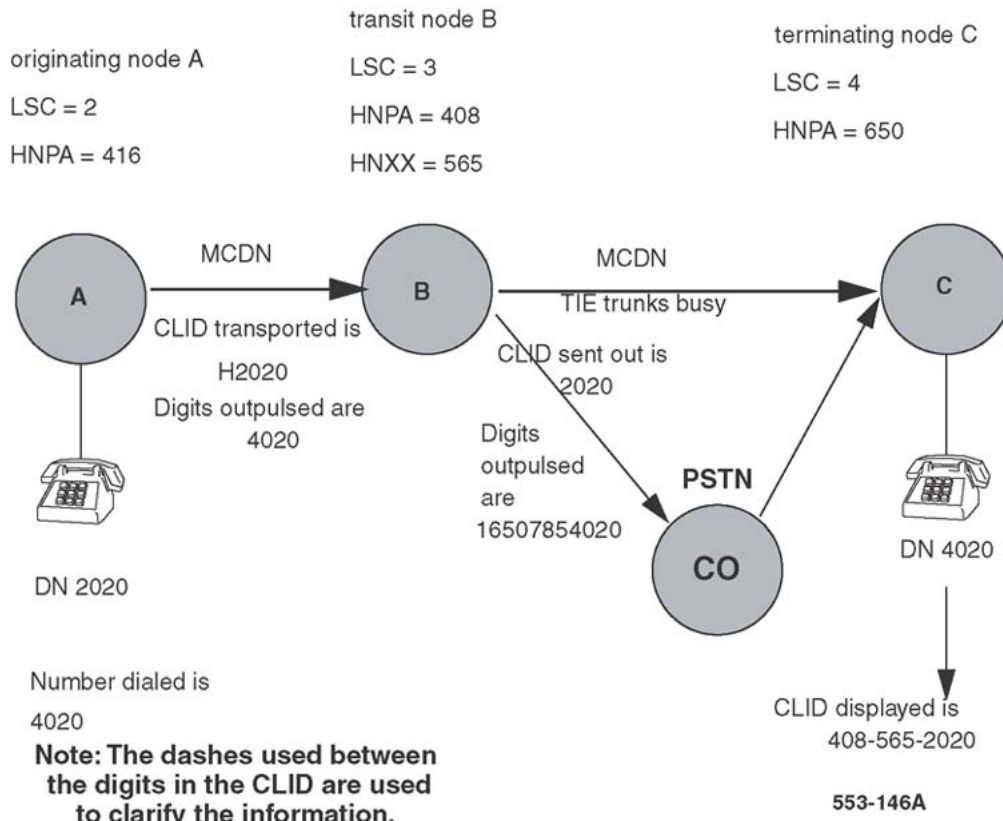
Figure 51: Private network to Public network hopoff, prior functionality for CDP dialing
