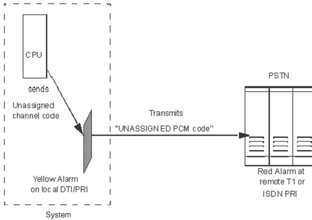
Figure 10: System response to Yellow Alarm condition prior to Idle Code Selection feature
