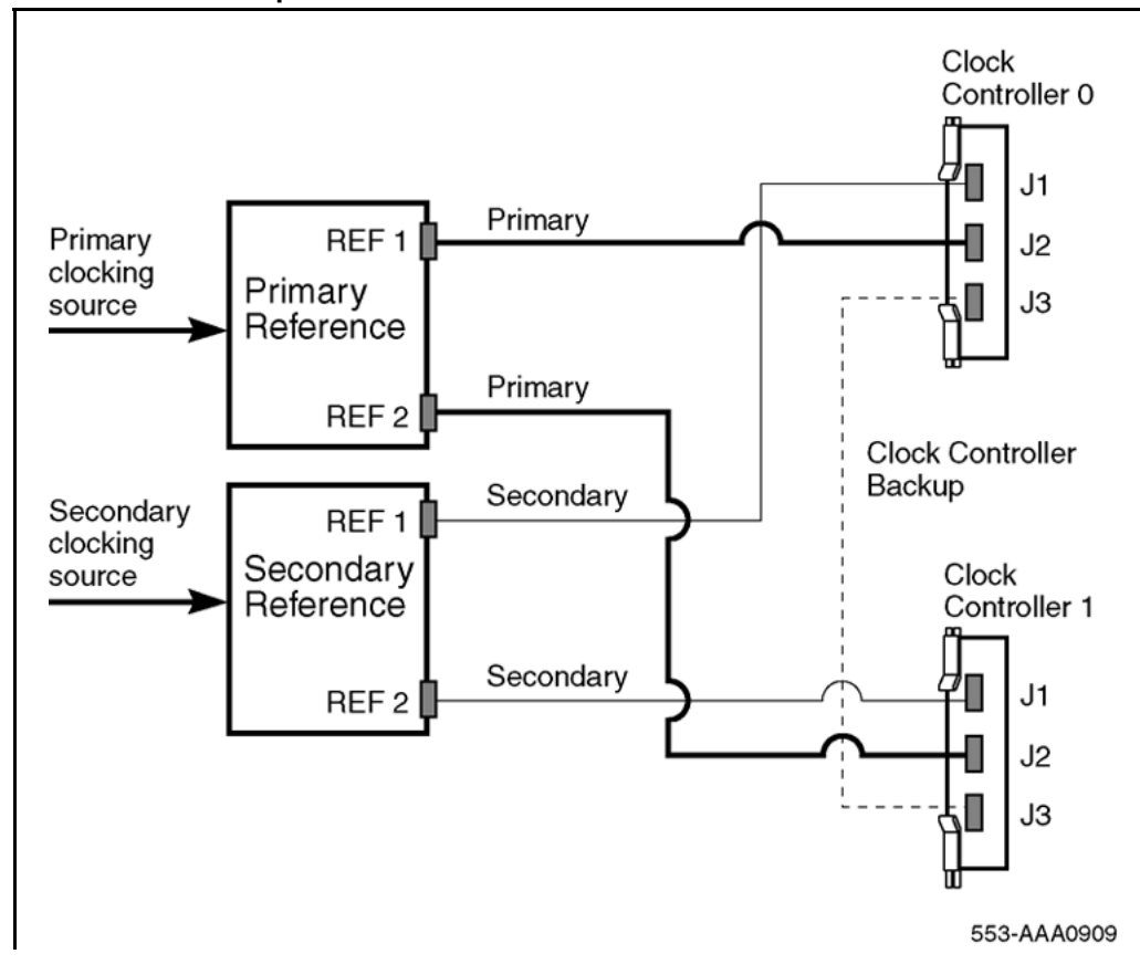
Figure 56 Clock Controller Option 1
