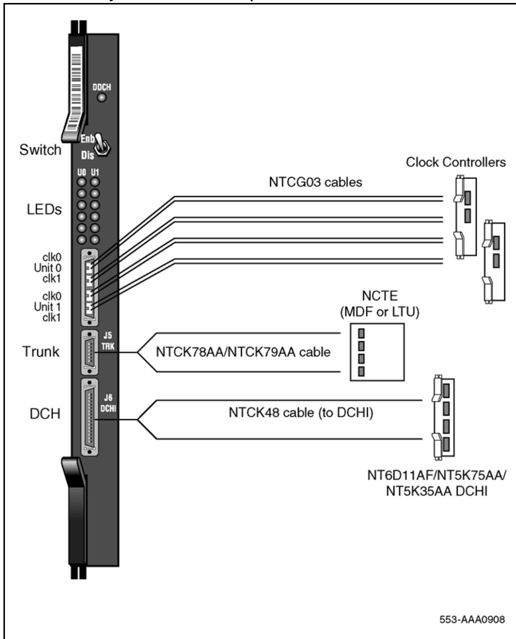
Figure 54 DDP2 cable for systems without an I/O panel
