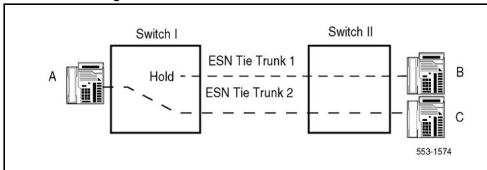
Figure 7 Connection after NXFER
