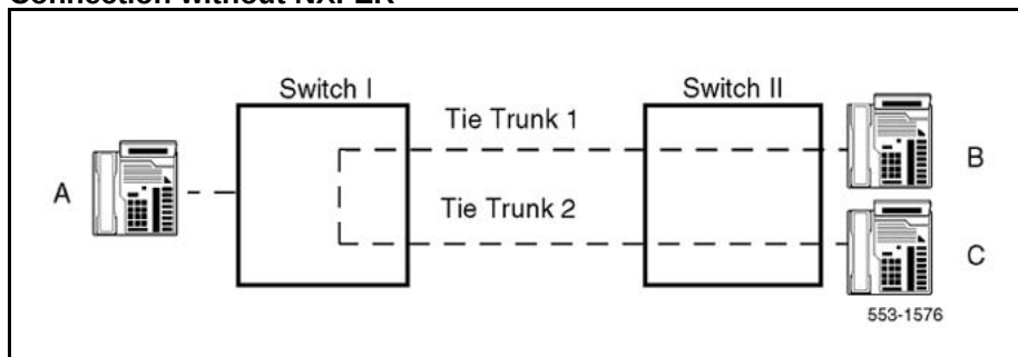
Figure 5 Connection without NXFER
