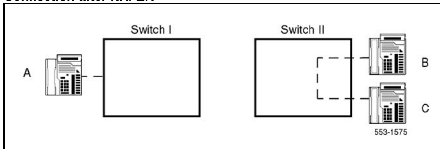
Figure 7 Connection after NXFER
