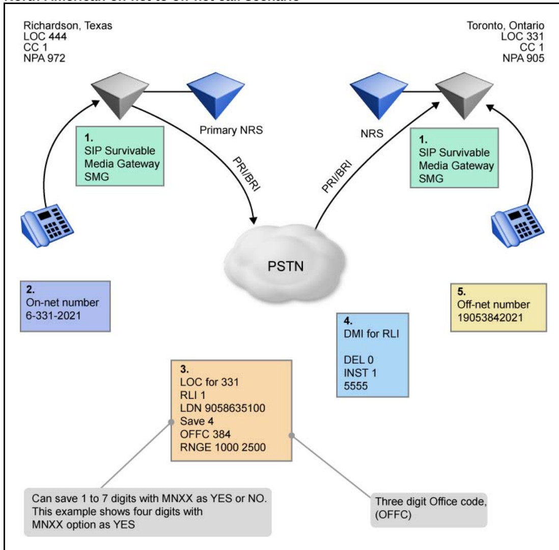
Figure 2 North American on-net to off-net call scenario
