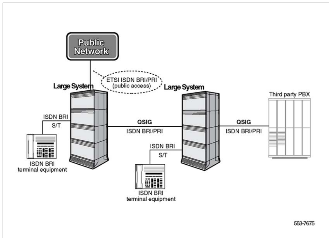
Figure 13 QSIG ISDN BRI trunk connectivity
