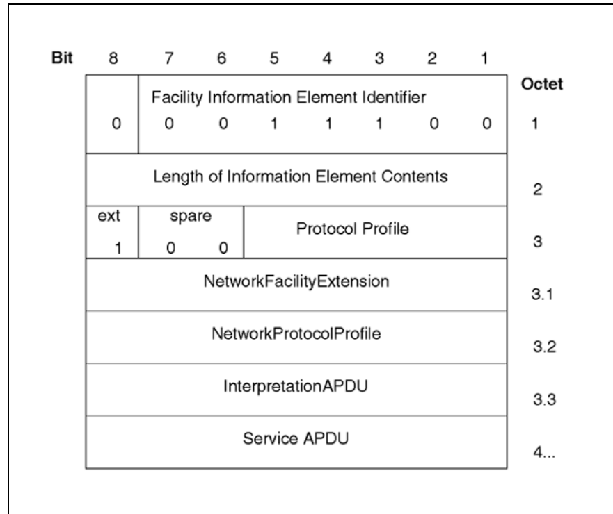
Figure 81 Facility IE layout
