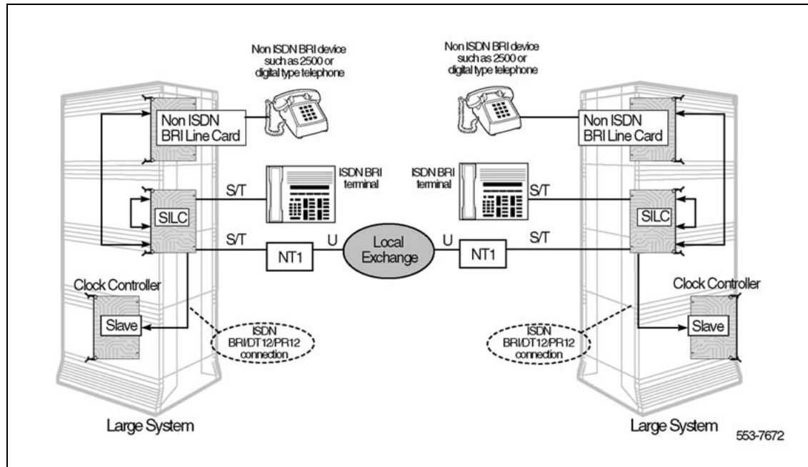
Figure 10 ISDN BRI trunk access TIE trunk connectivity - first configuration
