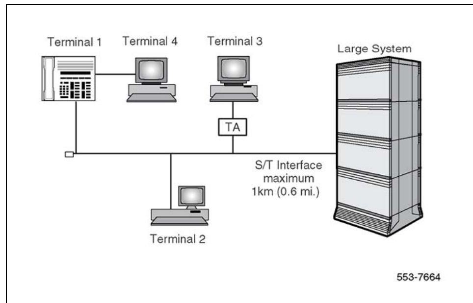
Figure 2 ISDN Basic Rate Interface S/T interface configured as a line
