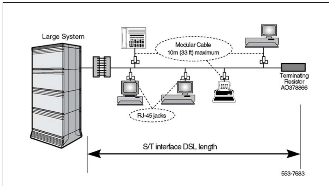
Figure 21 Short passive SILC DSL
