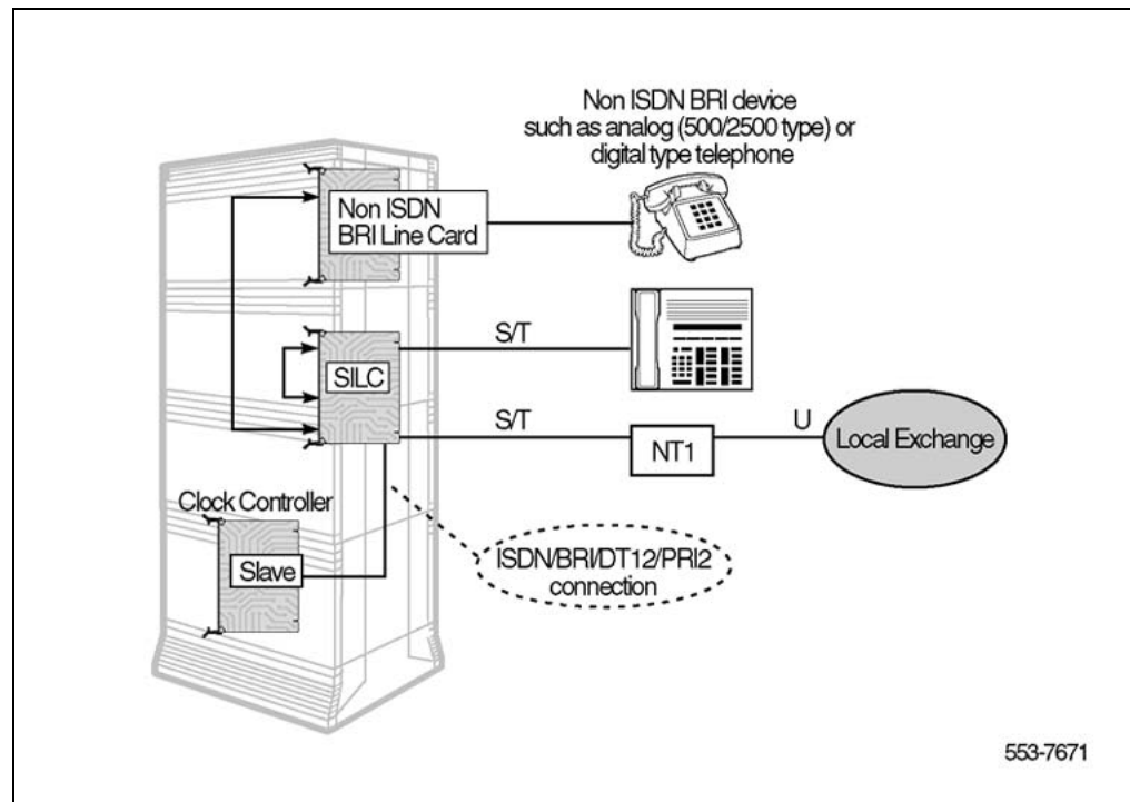
Figure 9 ISDN BRI trunk access for local exchange connectivity
