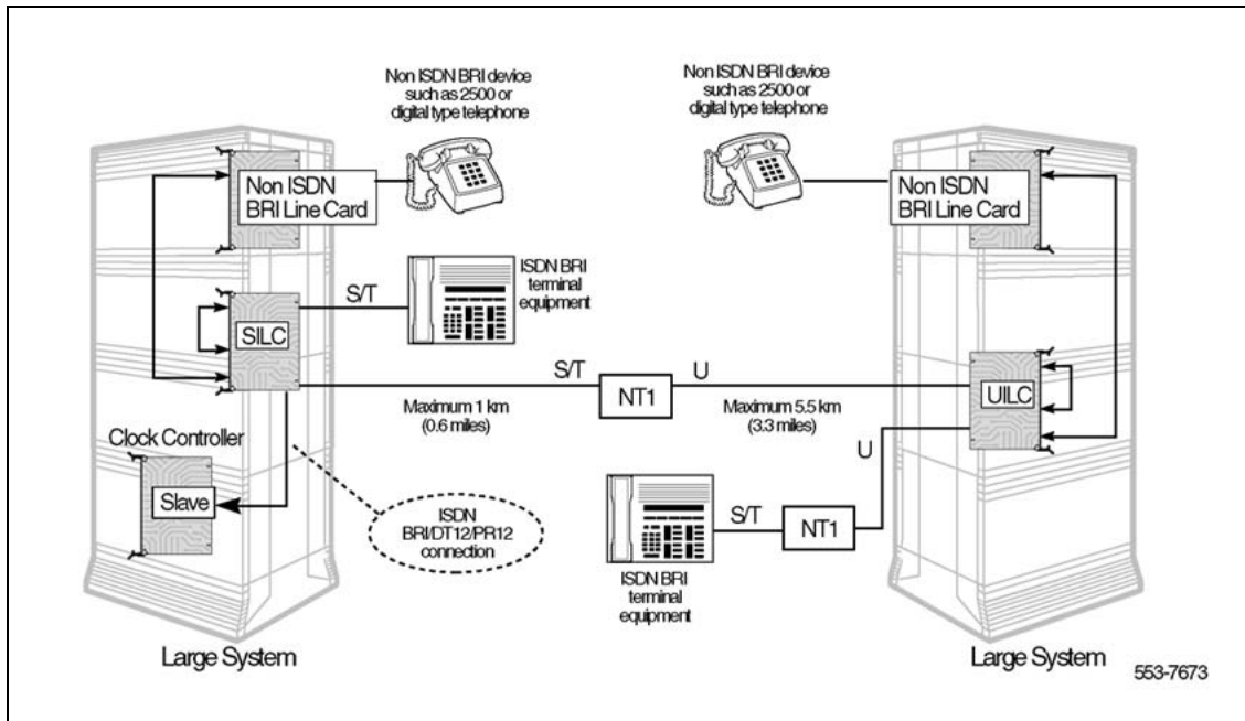
Figure 11 ISDN BRI TIE trunk connectivity - second configuration
