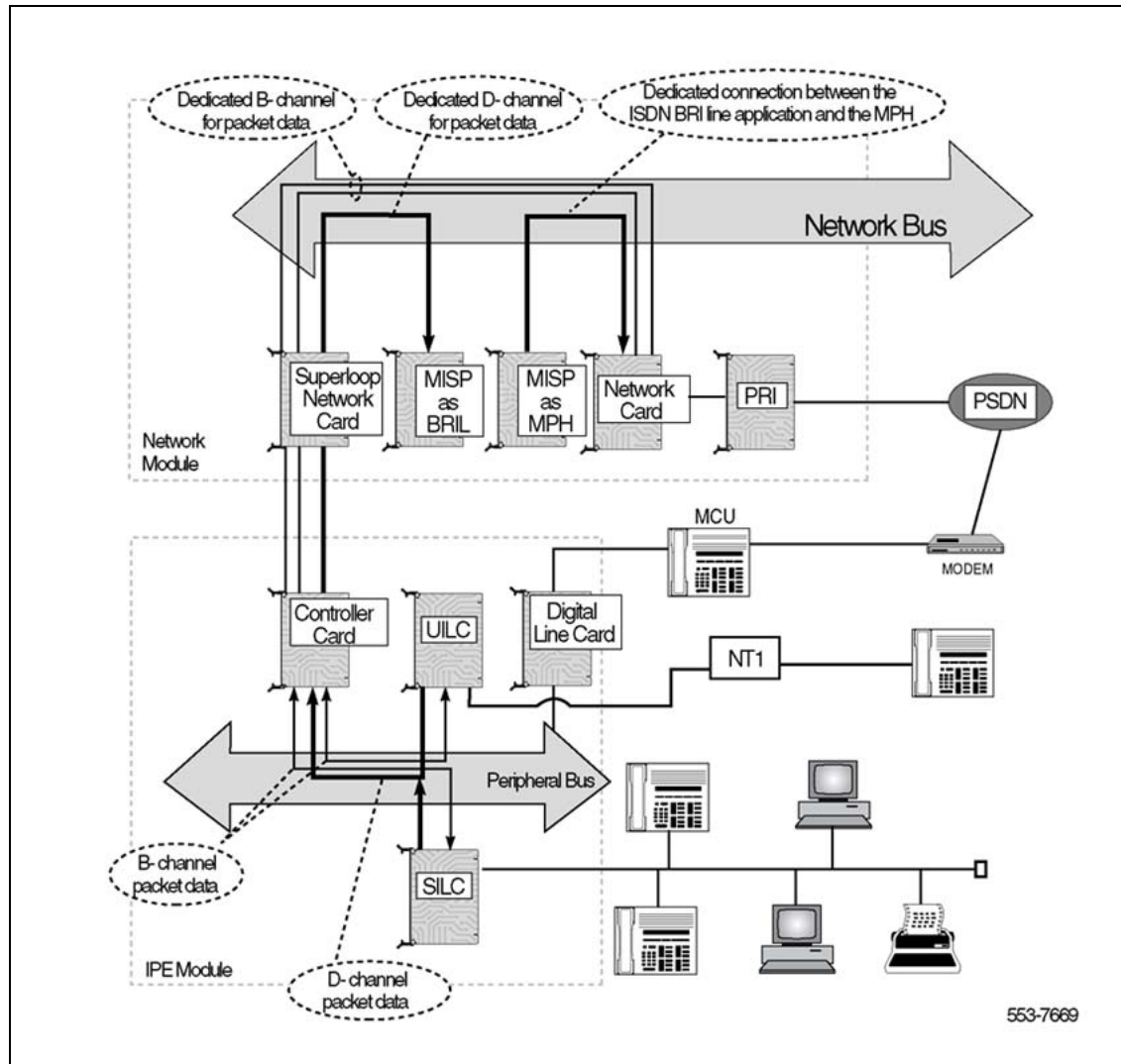
Figure 7 Packet data transmission using the MPH
