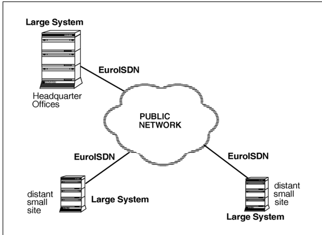
Figure 55 Example of a network where BNE is useful
