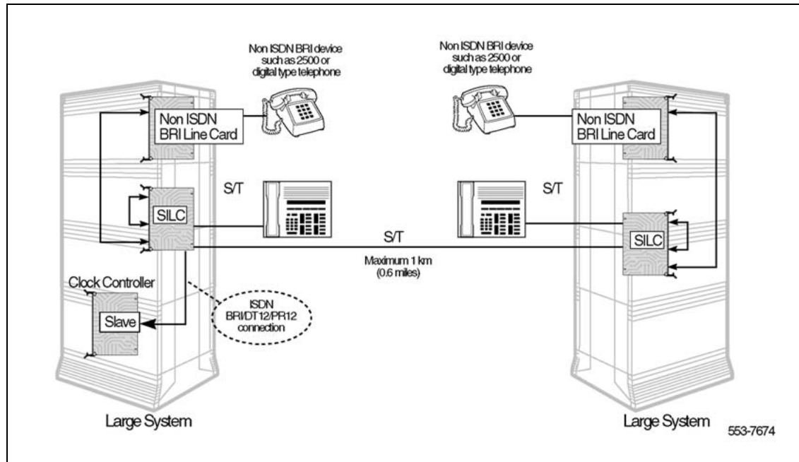
Figure 12 ISDN BRI TIE trunk connectivity - third configuration, as described above
