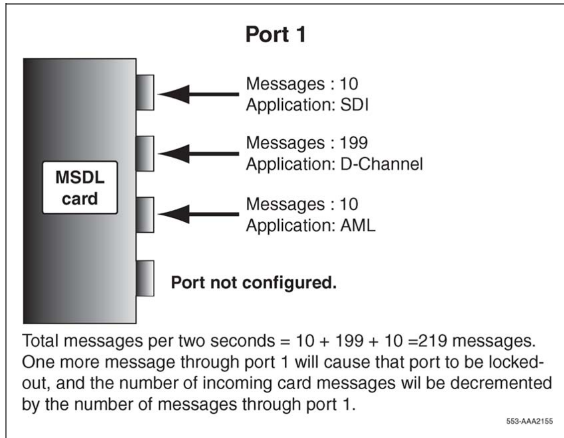
Figure 102 MSDL port overload check preceding card overload check
