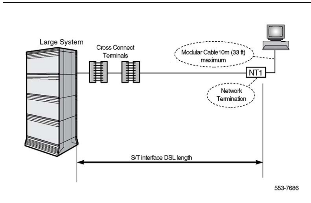
Figure 24 Point-to-Point UILC DSL
