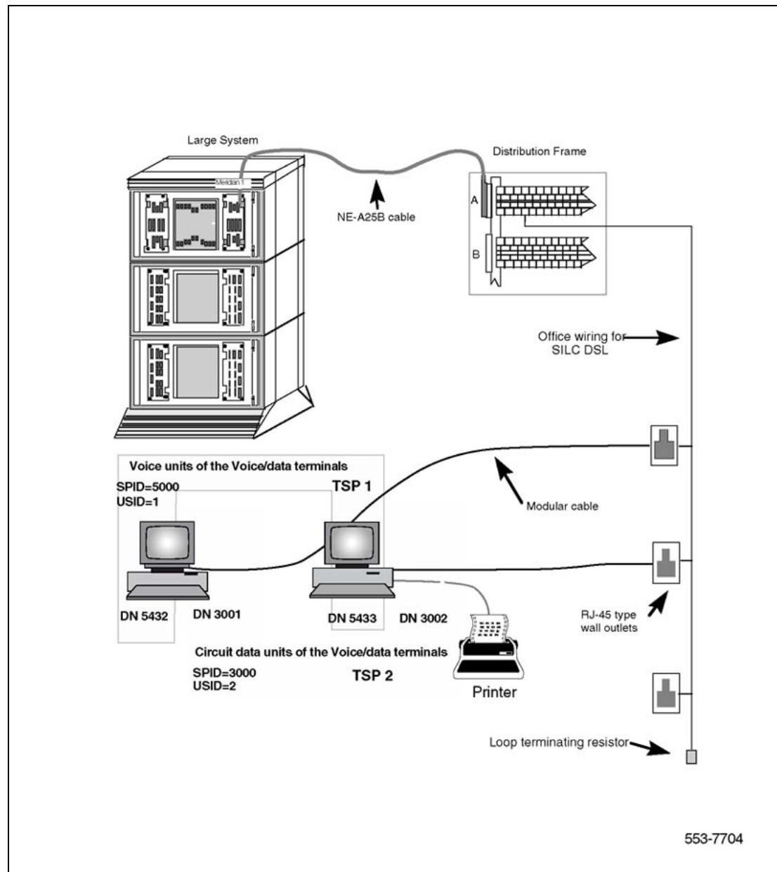
Figure 28 DSL terminal configuration
