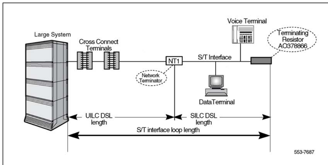
Figure 25 UILC DSL used as an extension for an S/T interface loop
