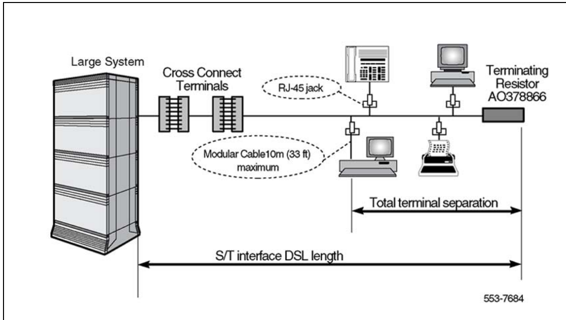
Figure 22 Extended passive SILC DSL
