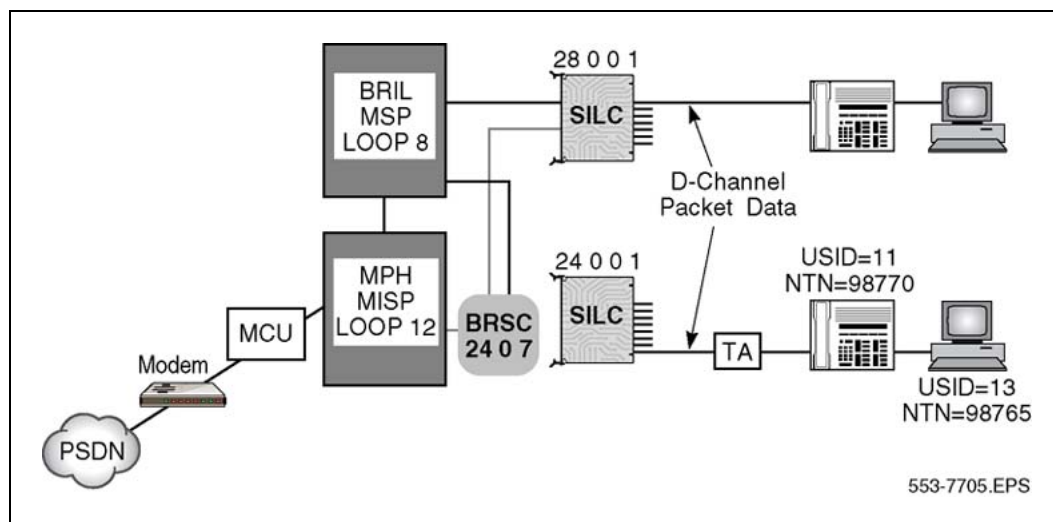
Figure 29 DSL terminal configuration with D-channel and B-channel packet data
