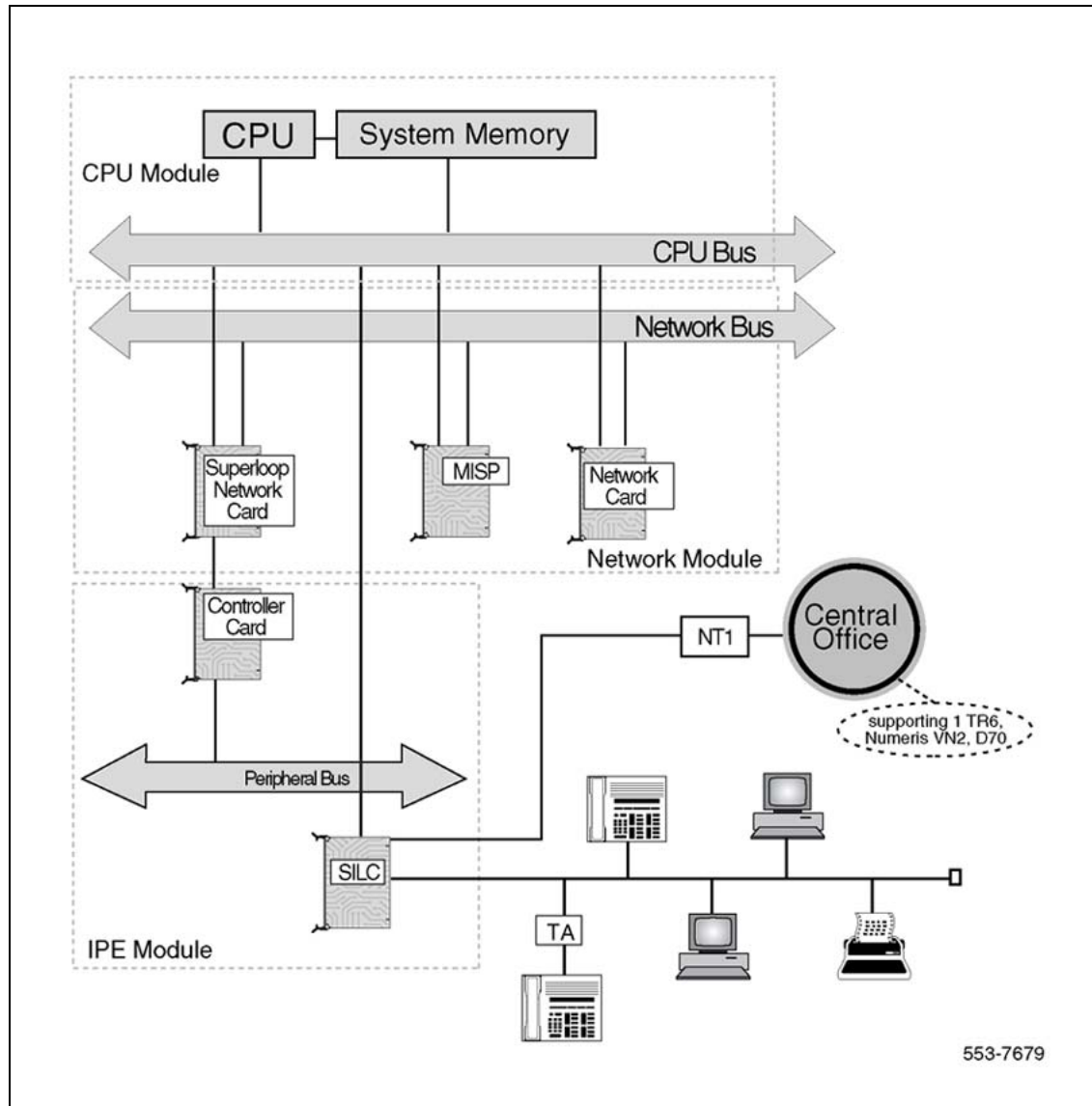
Figure 17 A basic ISDN BRI trunking architecture (CO connectivity)
