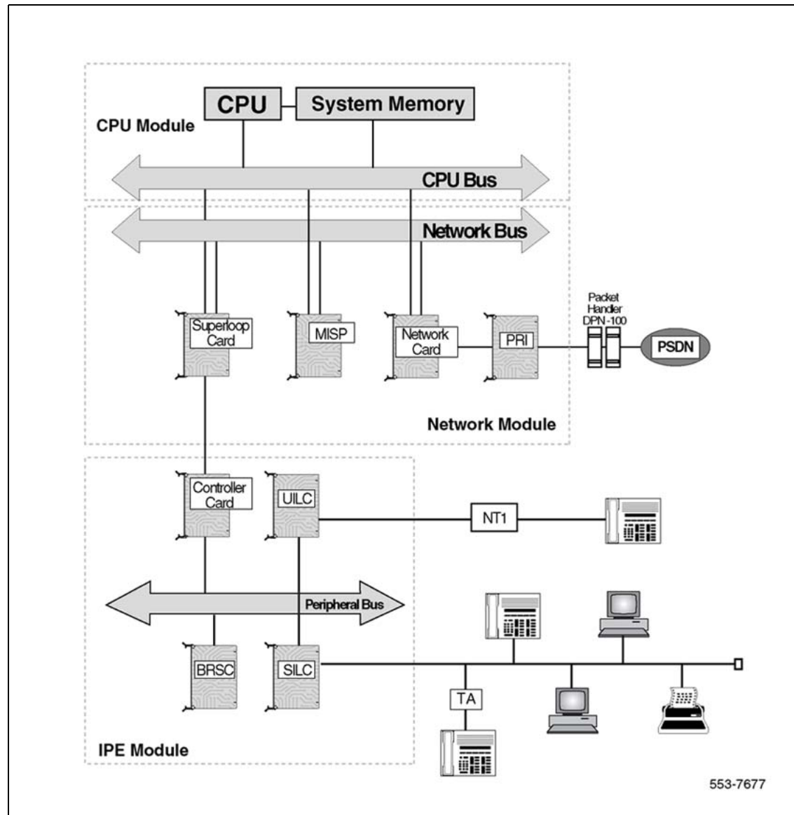
Figure 15 A basic ISDN BRI DPN-100 packet data architecture, with a BRSC
