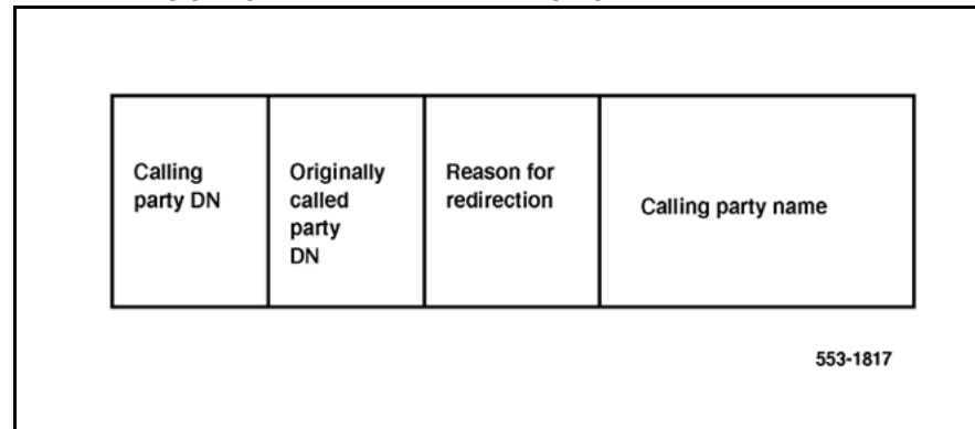
Terminating party CLID redirection display
