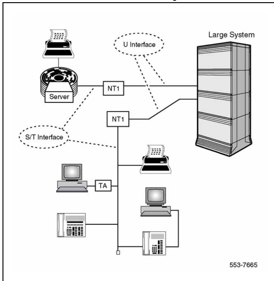
Figure 3 ISDN Basic Rate Interface U interface configured as a line
