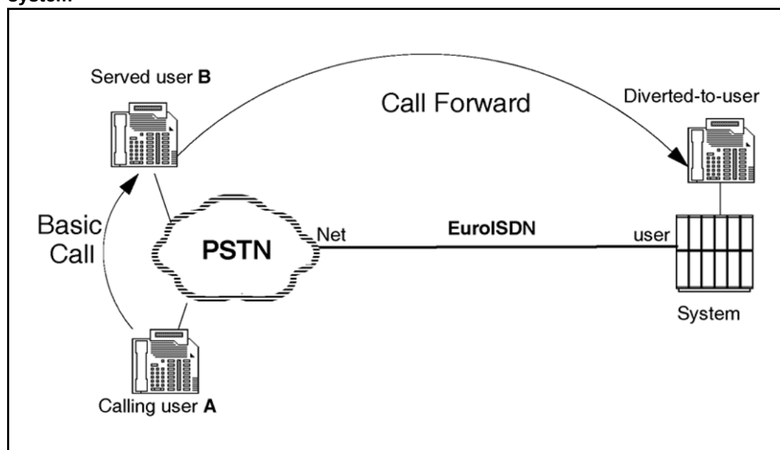
Figure 36 The calling and served users are in the public network and the diverted-to-user is on the system
