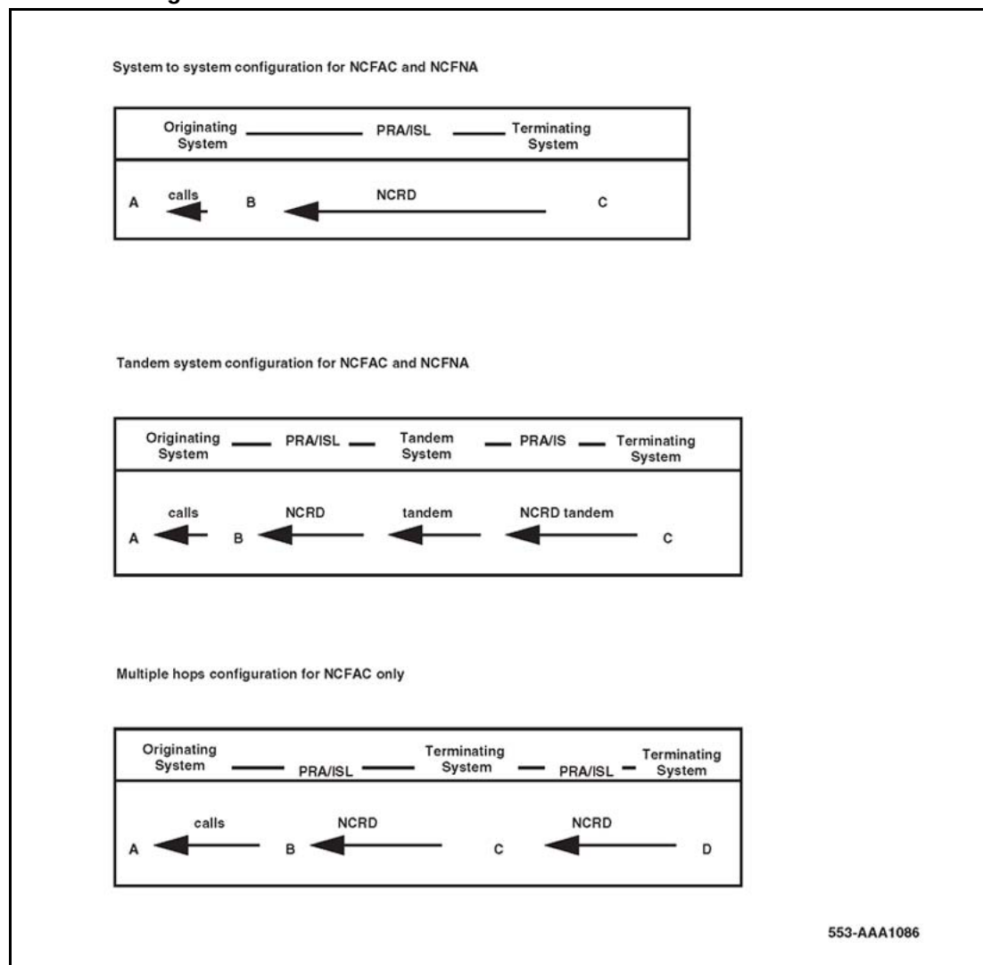
Figure 106 Network configurations for NCFAC and NCFNA
