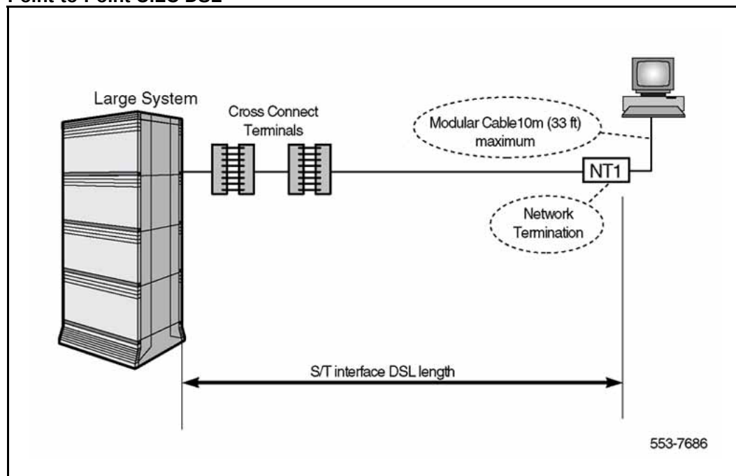
Figure 24 Point-to-Point ULC DSL
