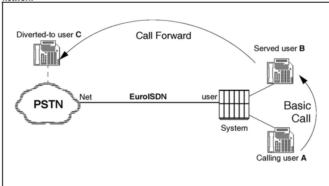
Figure 37 The calling and served users are on the system and the diverted-to-user is in the public network
