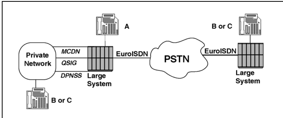
Figure 48 User A and user B or C are in the system private network.
