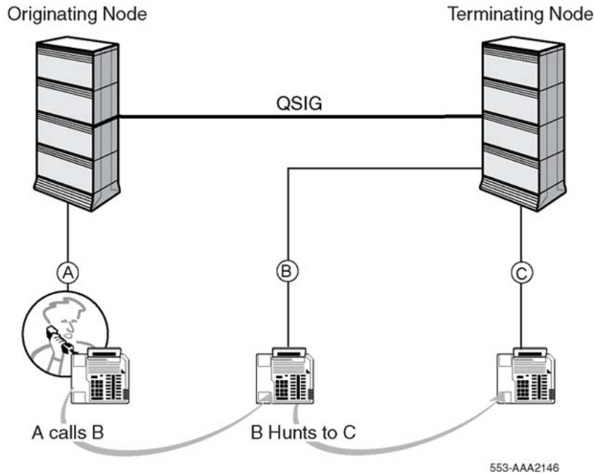
Figure 88: Hunt over a QSIG link
