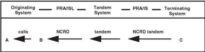
Tandem system configuration for NCFAC and NCFNA
