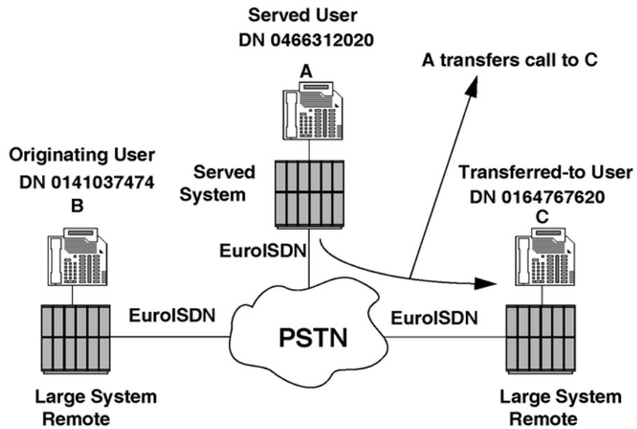
Figure 51: User B calls user A. User A transfers call to user C.
