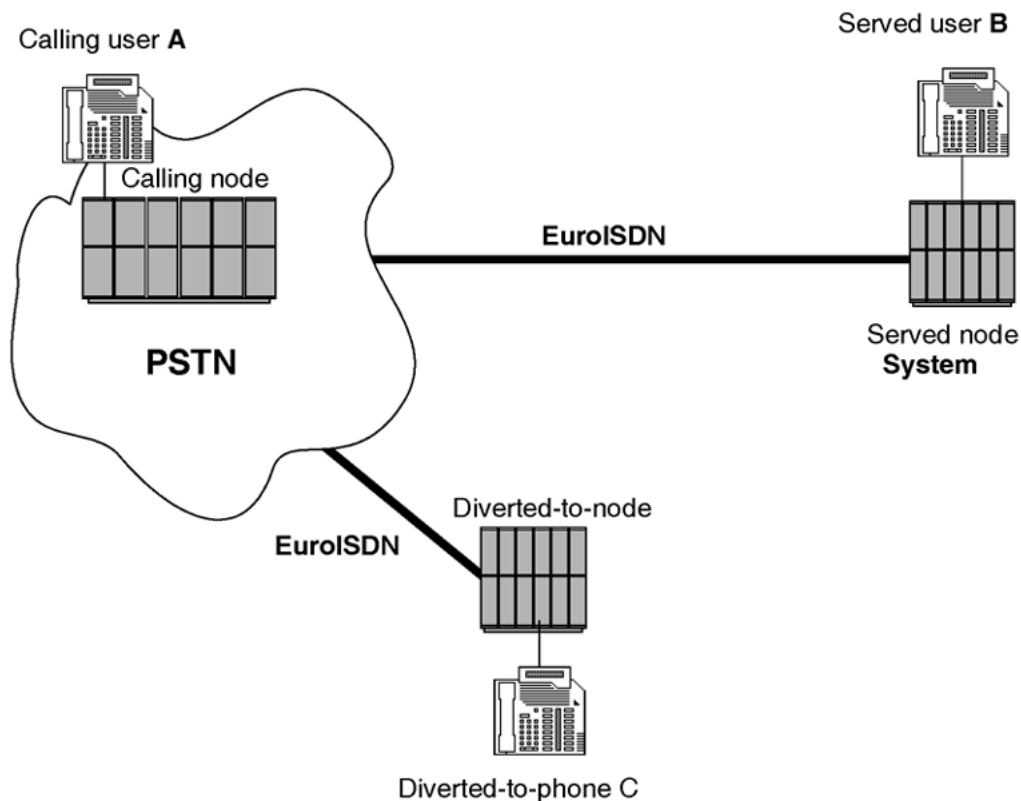
Figure 32: Call Diversion environment
