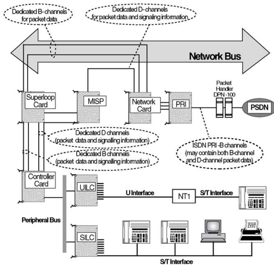
Figure 5: Packet data transmission using the external packet handler
