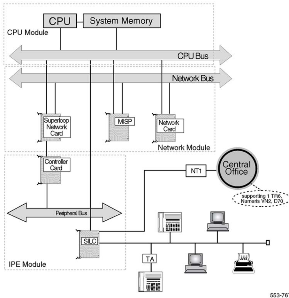
Figure 17: A basic ISDN BRI trunking architecture (CO connectivity)
