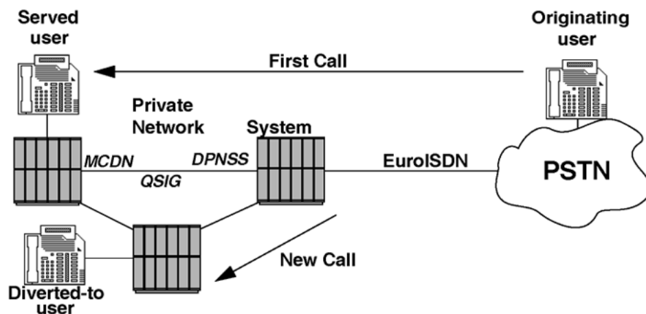
Figure 42: Call rerouting request processed at the gateway node.
