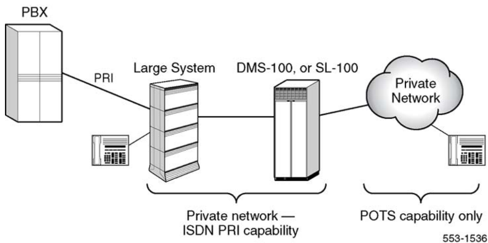
Figure 68: Private Network Hopoff
