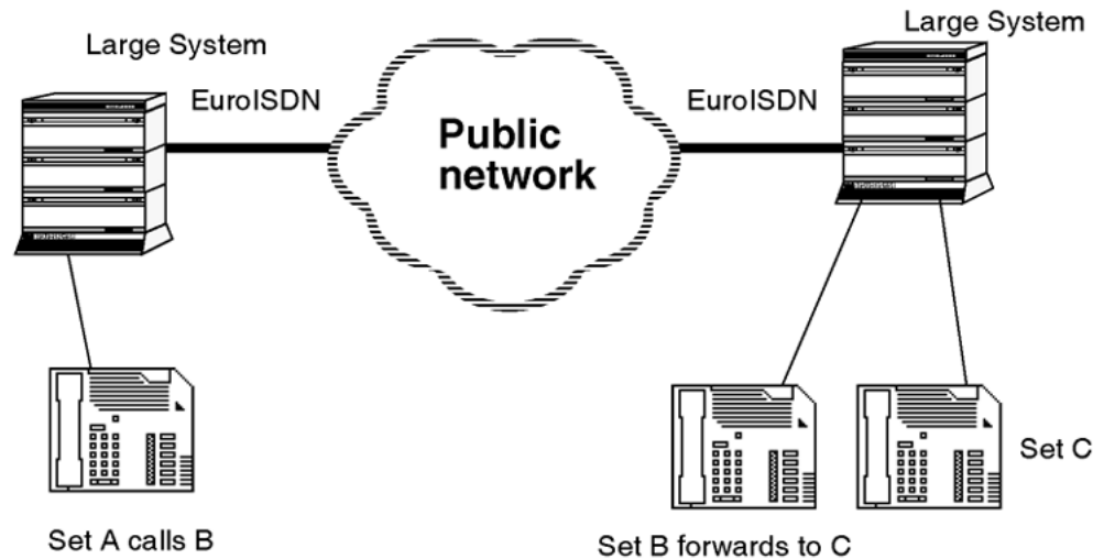
Figure 60: Local Call Forward
