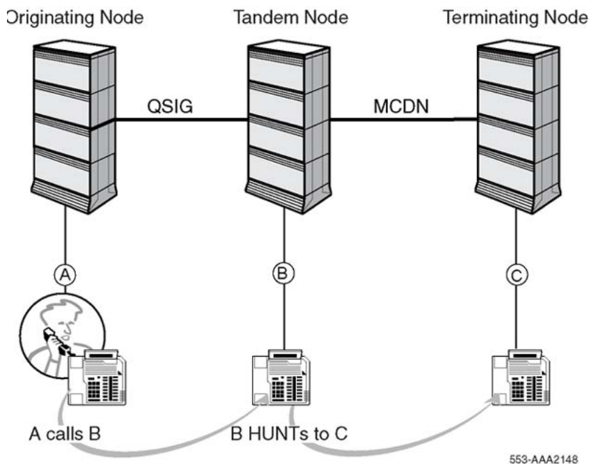
Figure 91: Hunt over a QSIG/MCDN link
