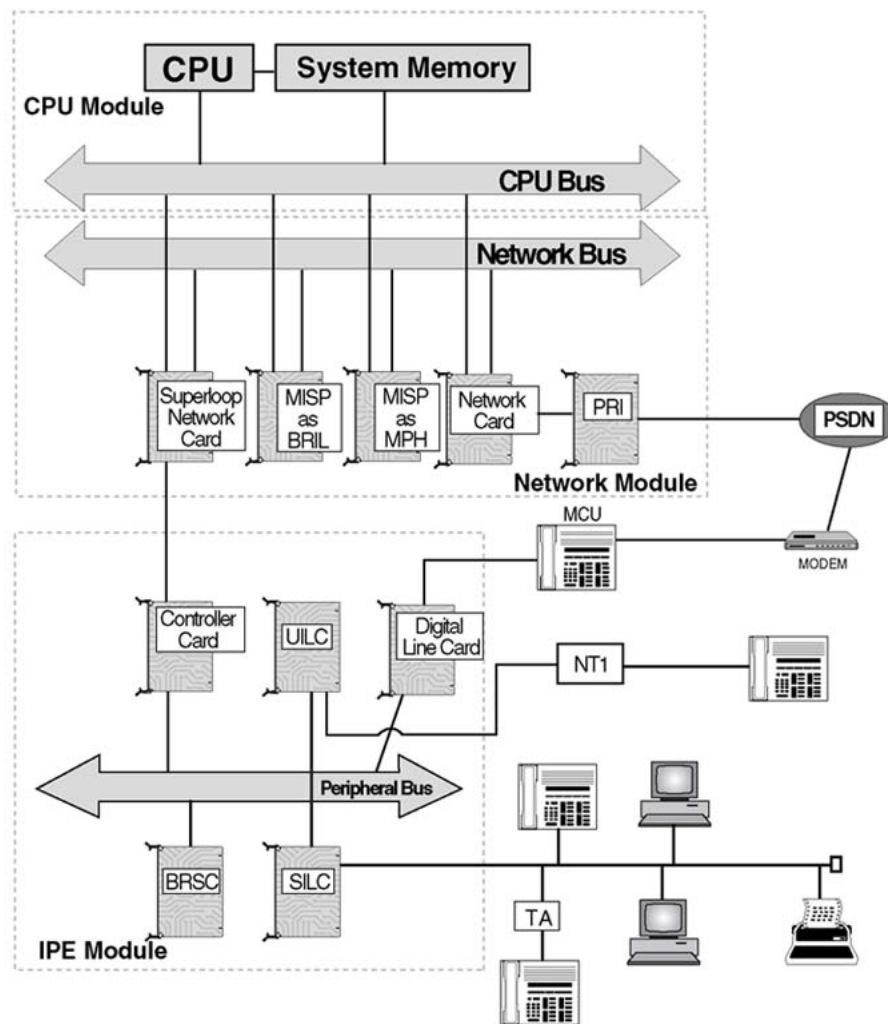
Figure 16: A basic ISDN BRI MPH packet data architecture, with a BRSC and an MCU
