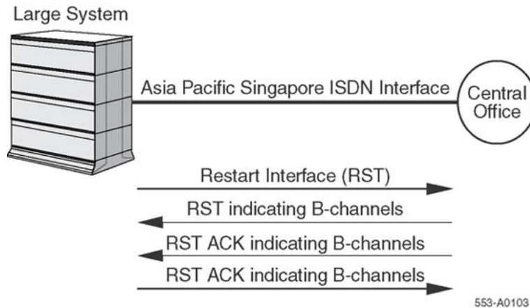
Figure 121: Restart messaging sequence for the Singapore ISDN Restart Message Enhancement
