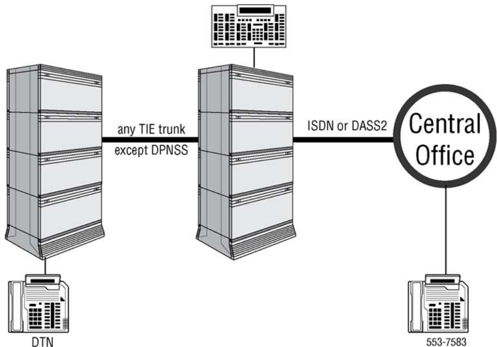
Figure 67: Attendant Through Dialing Networkwide
