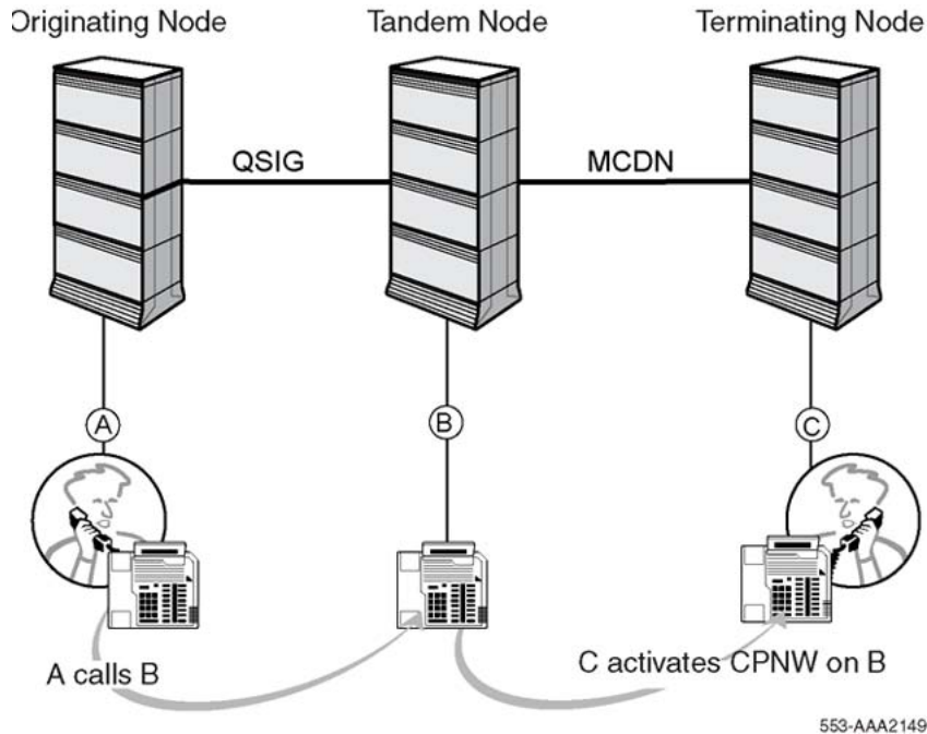
Figure 92: Call Pickup Network Wide over a QSIG/MCDN link
