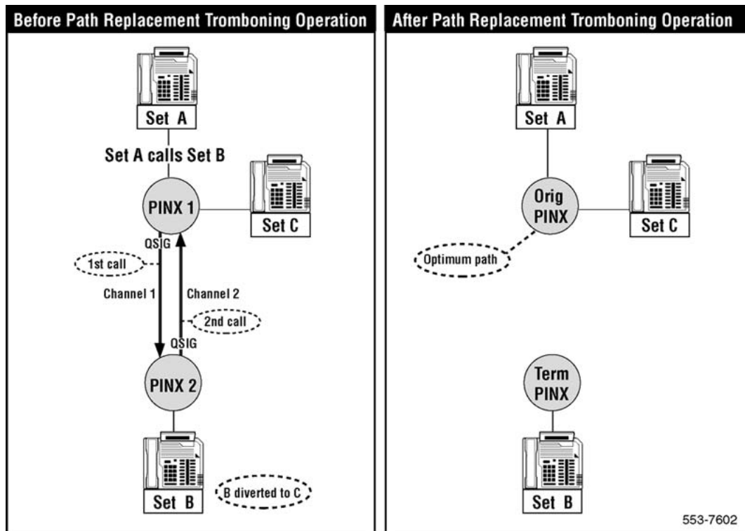
Figure 98: Tromboning Path Replacement
