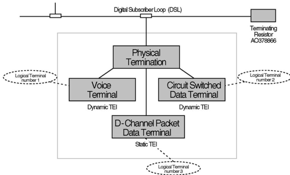
Figure 26: Multiple logical terminals on one physical termination
