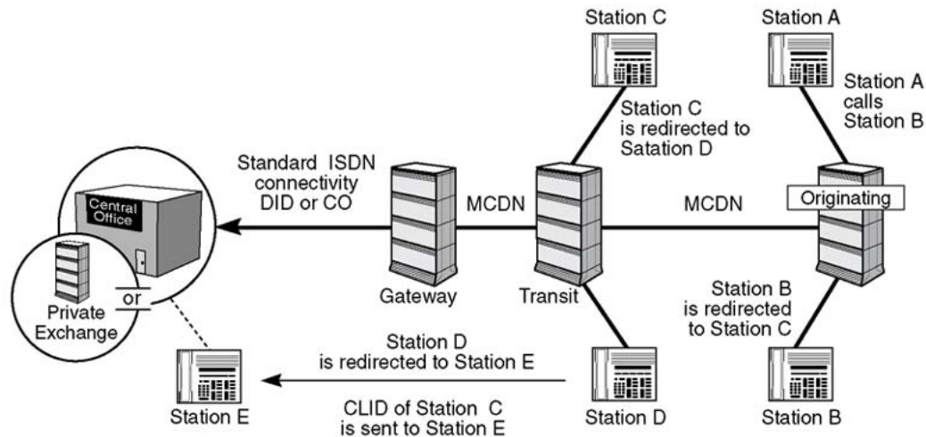
Figure 73: MCDN call redirected to the Public Network/PBX from a non-gateway node
