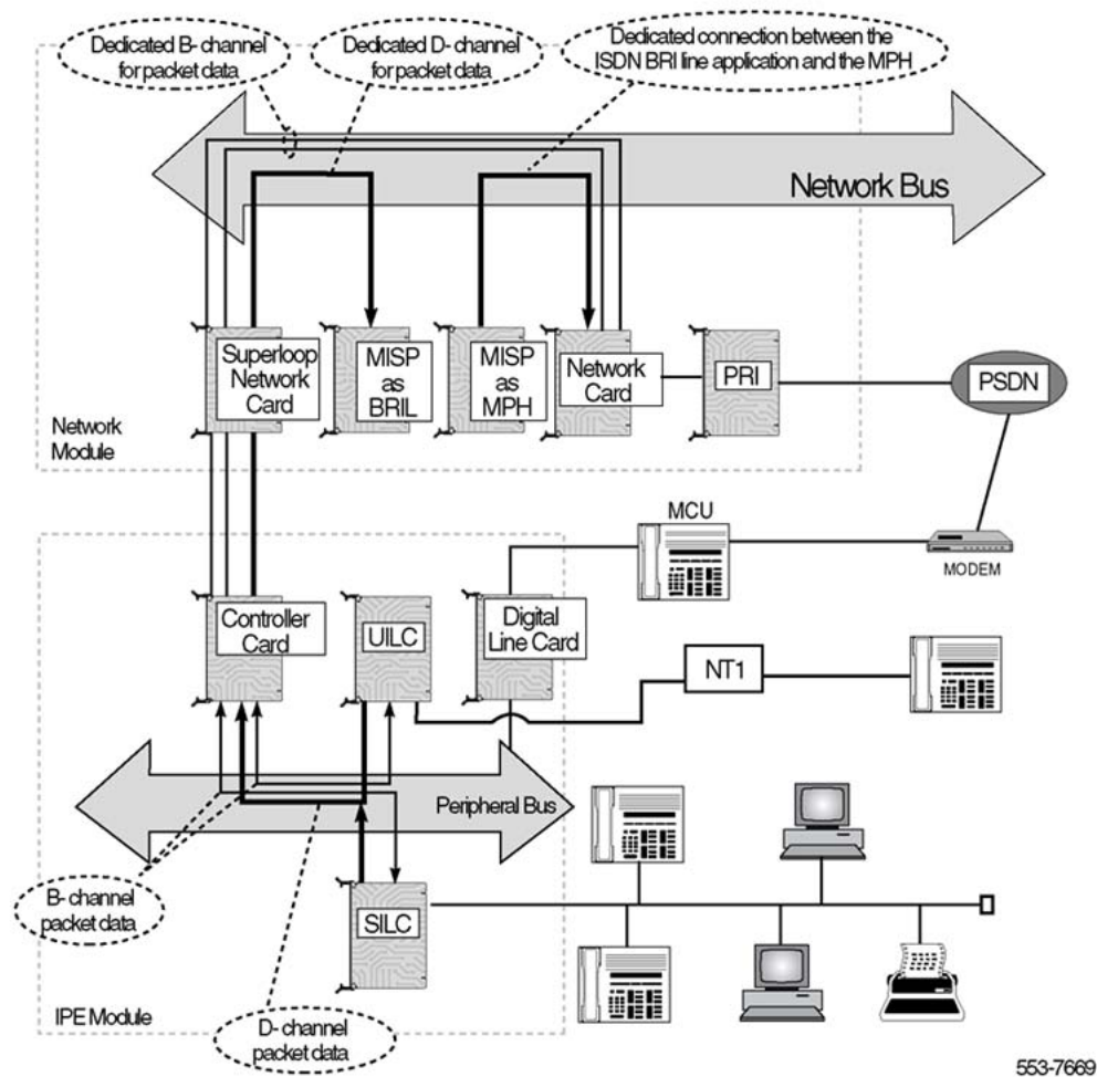
Figure 7: Packet data transmission using the MPH
