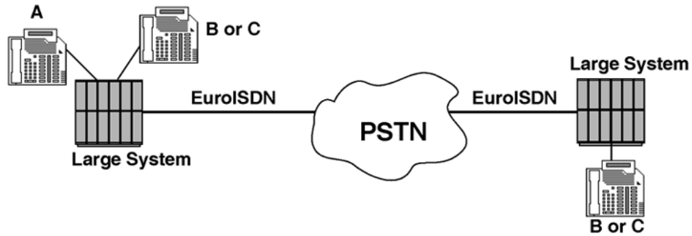
Figure 46: User A and user B or C are in the system private network
