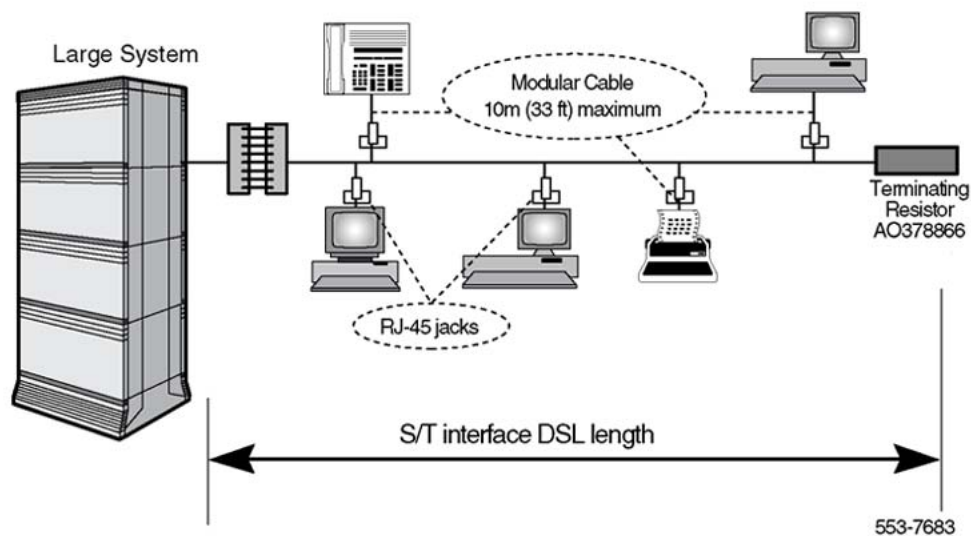
Figure 21: Short passive SILC DSL
