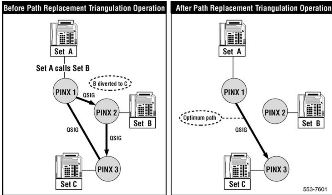
Figure 97: Triangulation Path Replacement
