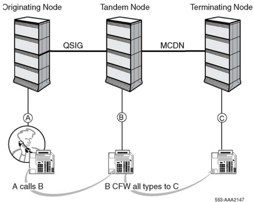
Figure 90: Call Forward All Calls over a QSIG/MCDN link
