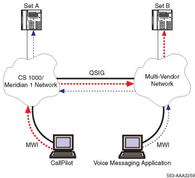
Figure 119: MWI message transport between a system network and a multi-vendor network
