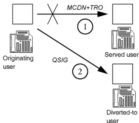
Figure 83: Call from MCDN TRO Diverted to QSIG
