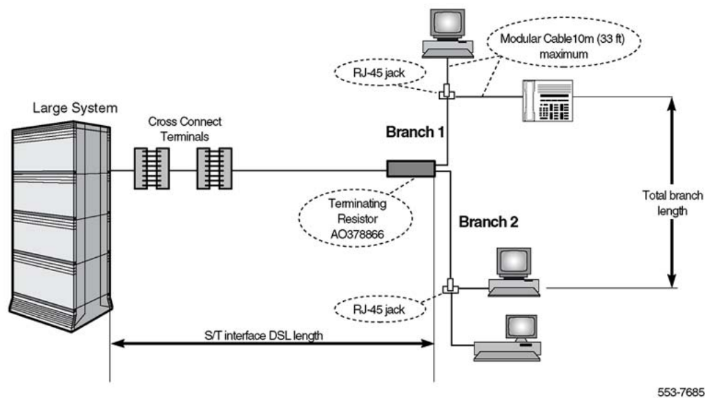
Figure 23: Branched passive SILC DSL
