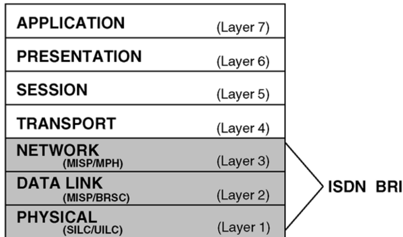
Figure 1: OSI model
