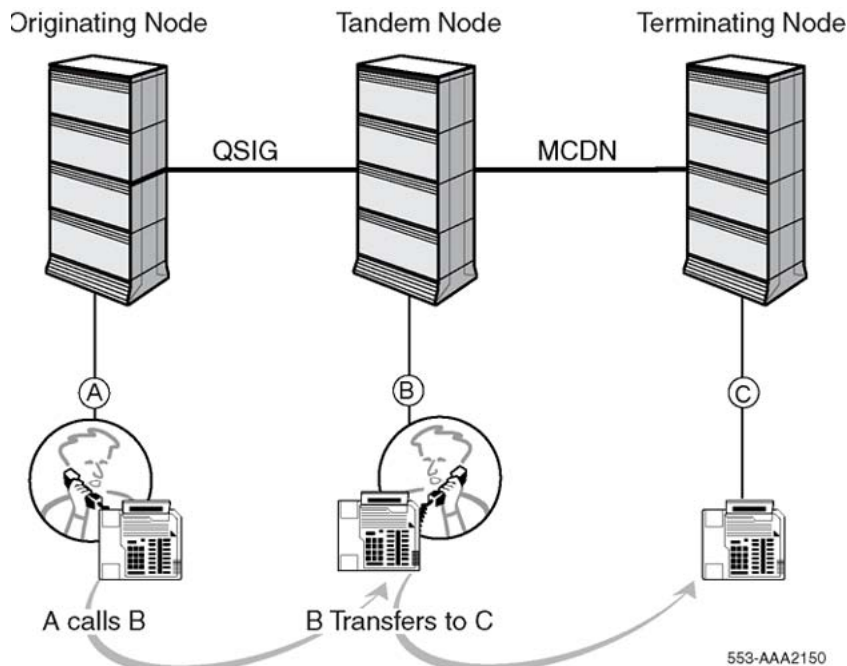
Figure 93: Call Transfer over a QSIG/MCDN link
