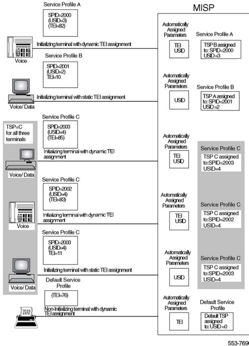
Figure 27: Terminal initialization and service profile assignment examples
