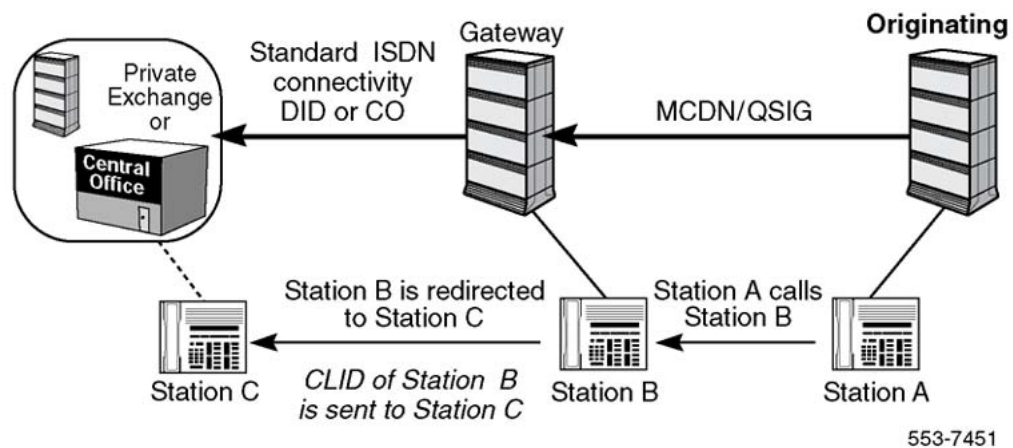
Figure 71: MCDN/QSIG call redirected to the Public Network/PBX
