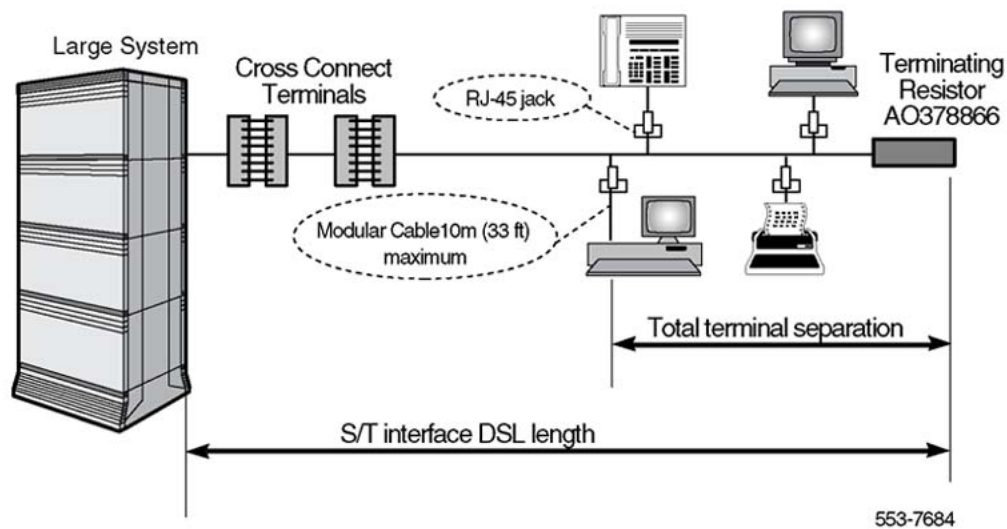
Figure 22: Extended passive SILC DSL
