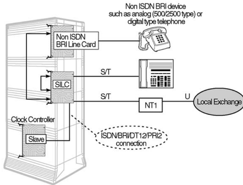
Figure 9: ISDN BRI trunk access for local exchange connectivity
