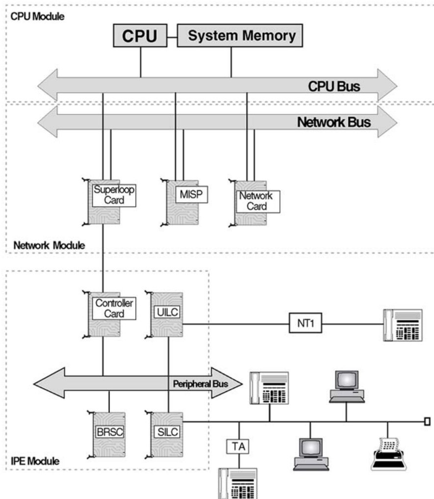
Figure 14: ISDN BRI line application architecture, configured with a BRSC
