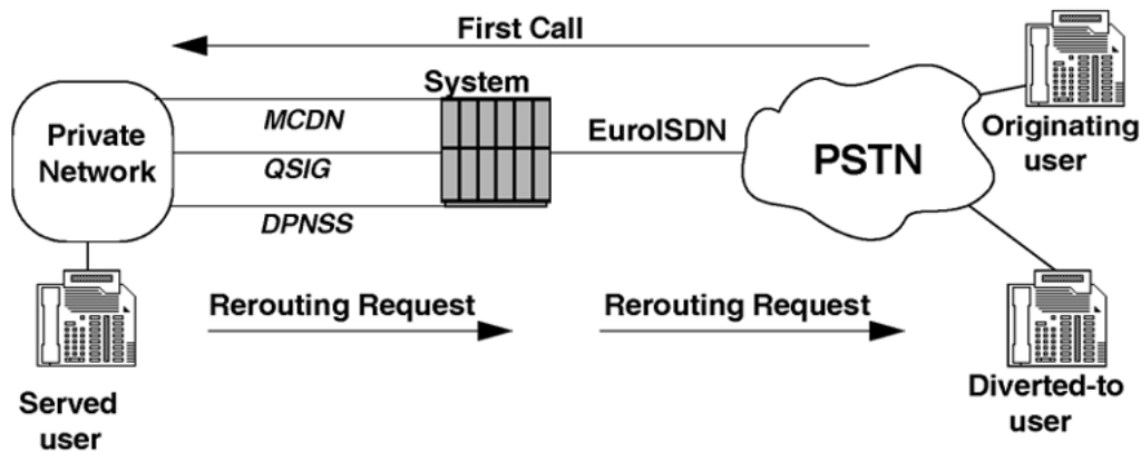
Figure 41: Call rerouting request sent to the CO.
