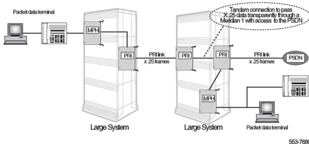
Figure 18: Tandem connections with the MPH
