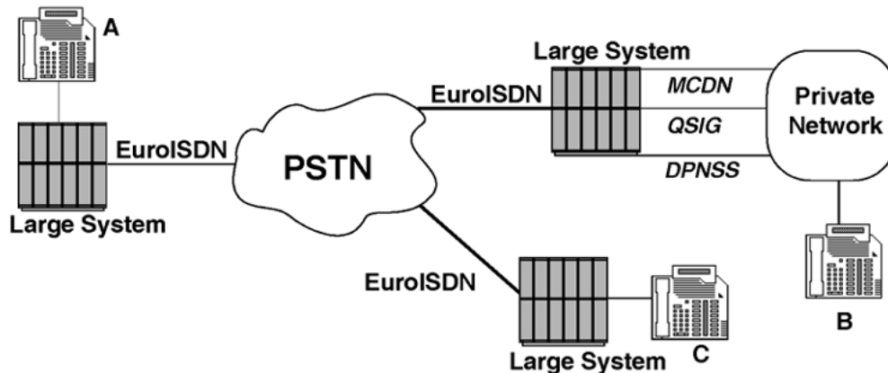
Figure 50: Remote user B or C is in the system private network
