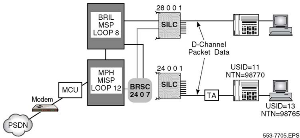
Figure 29: DSL terminal configuration with D-channel and B-channel packet data
