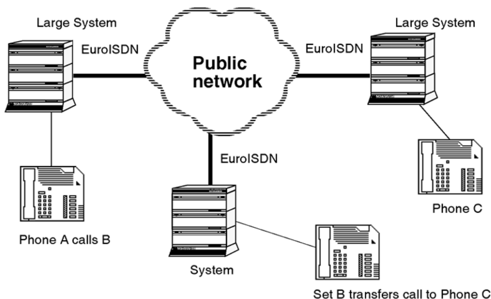
Figure 65: Call Transfer across a network
