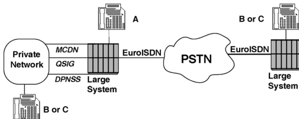
Figure 48: User A and user B or C are in the system private network.
