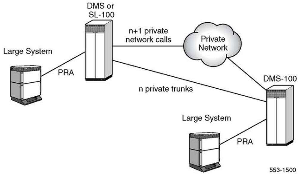
Figure 69: Private Network Overflow
