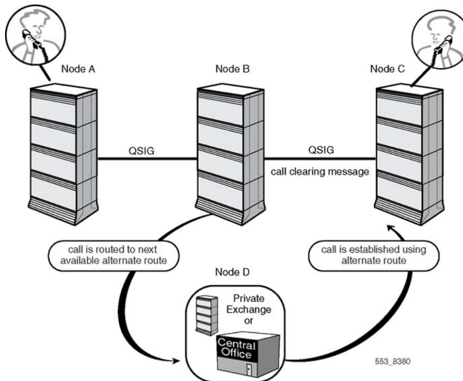
Figure 79: Transit node operation
