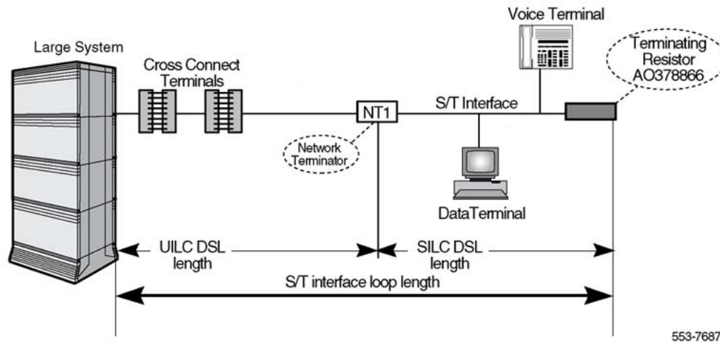
Figure 25: ULC DSL used as an extension for an S/T interface loop
