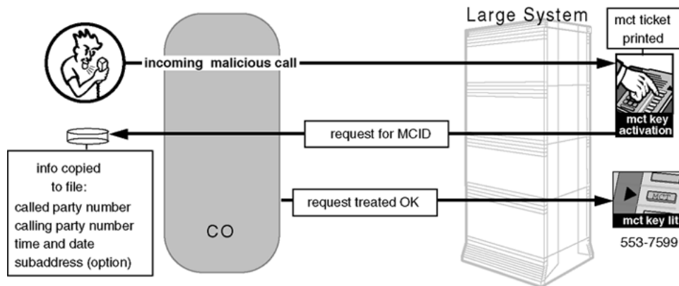
Figure 76: EuroISDN MCID invoked during the active phase of a malicious call
