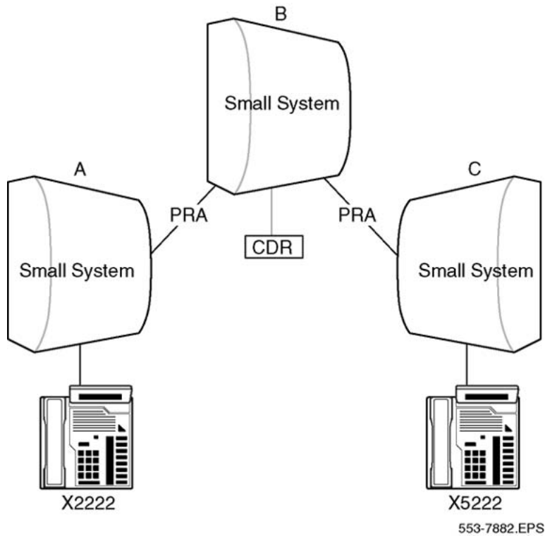
Figure 66: CDR in Multi-site Configuration
