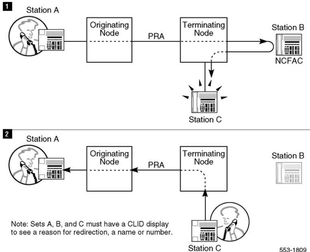
Figure 111: NCFAC intranode redirection
