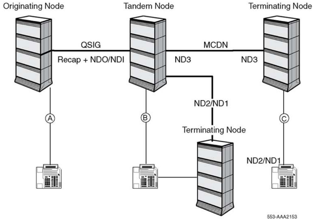
Figure 96: MCDN Name Display features over a QSIG/MCDN link
