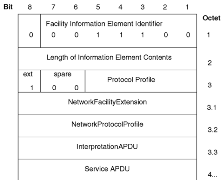
Figure 81: Facility IE layout
