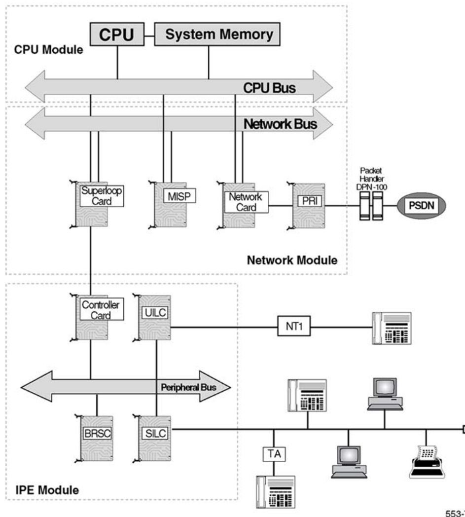
Figure 15: A basic ISDN BRI DPN-100 packet data architecture, with a BRSC
