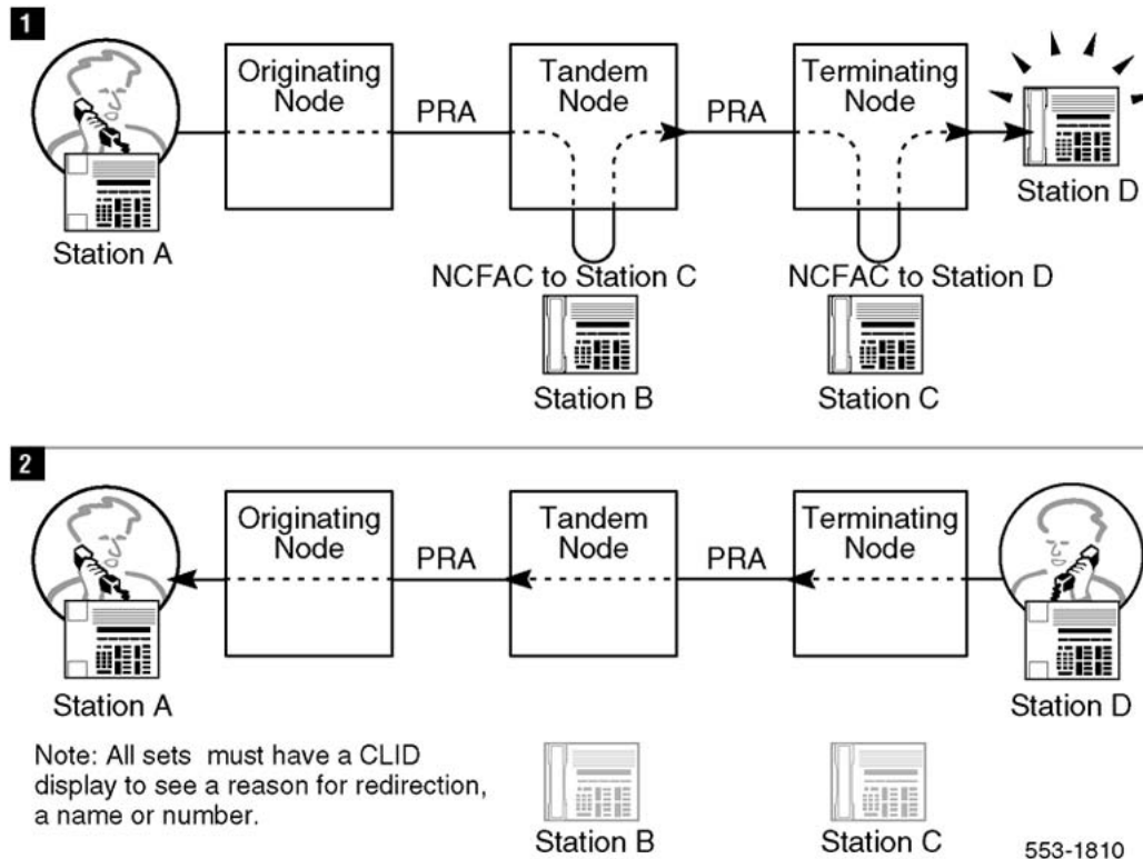
Figure 114: Tandem NCFAC intranode
