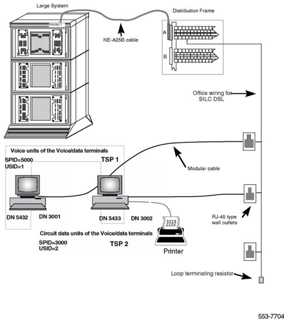
Figure 28: DSL terminal configuration
