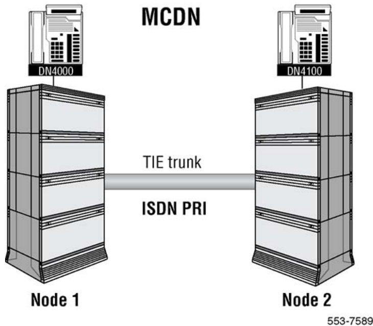
Figure 118: Scenario involving a call over a Meridian Customer Defined Network
