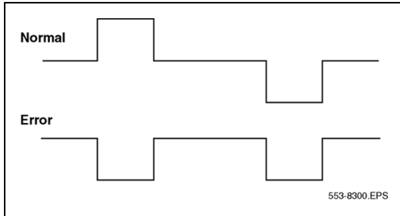
Figure 19 Bipolar violations
