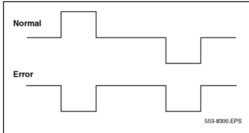
Figure 29 Bipolar violations
