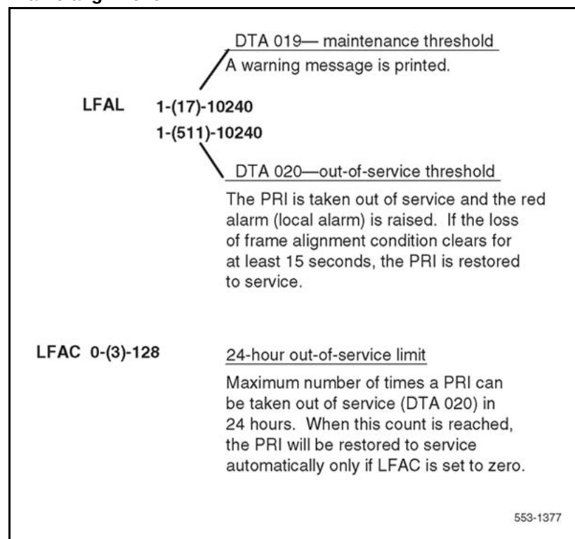
Figure 7 Frame alignment
