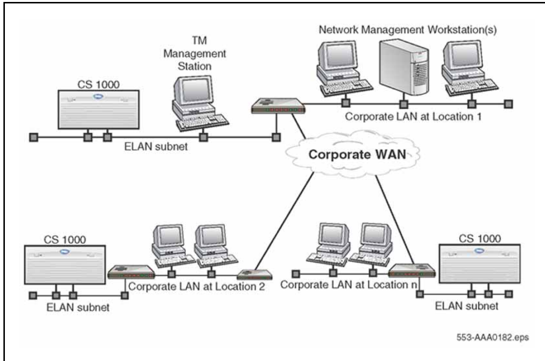
Figure 9 Typical SNMP Ethernet WAN
