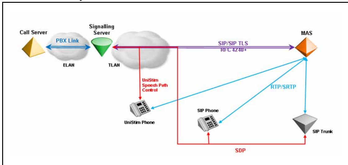
Figure 7 IP Media Services system architecture
