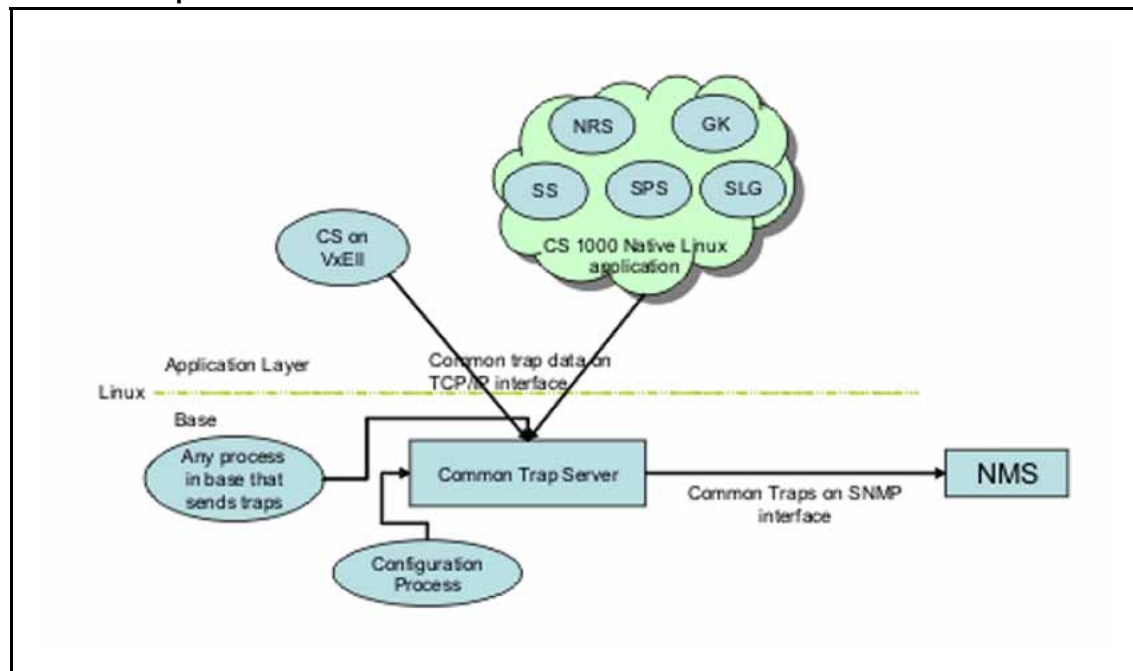
Figure 6 Common Trap Server in Linux
