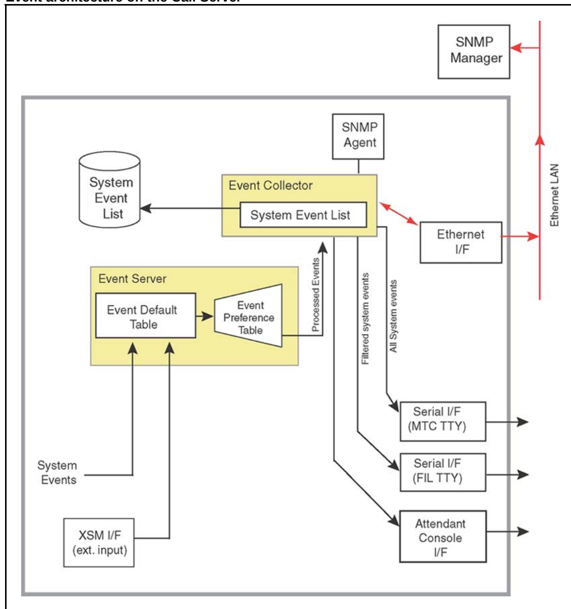
Figure 4 Event architecture on the Call Server
