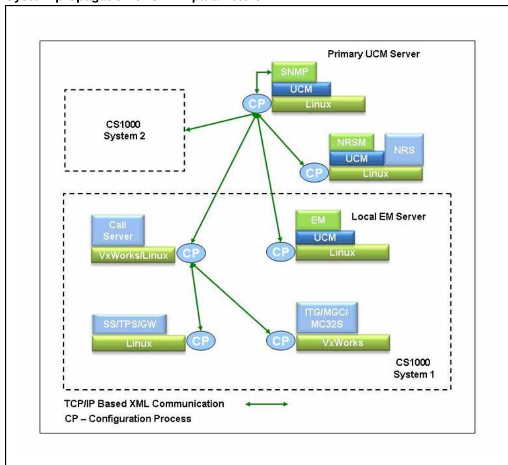
Figure 3 System propagation of SNMP parameters
