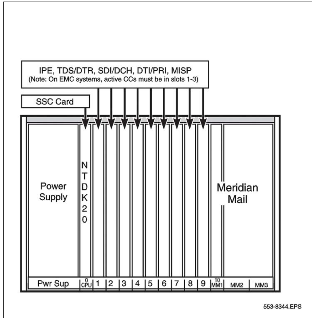
Figure 2 Circuit card assignments in the Main Cabinet
