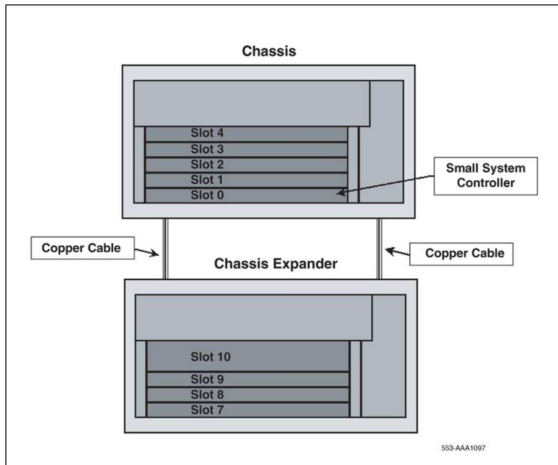
Figure 7 Chassis connected to a Chassis Expander
