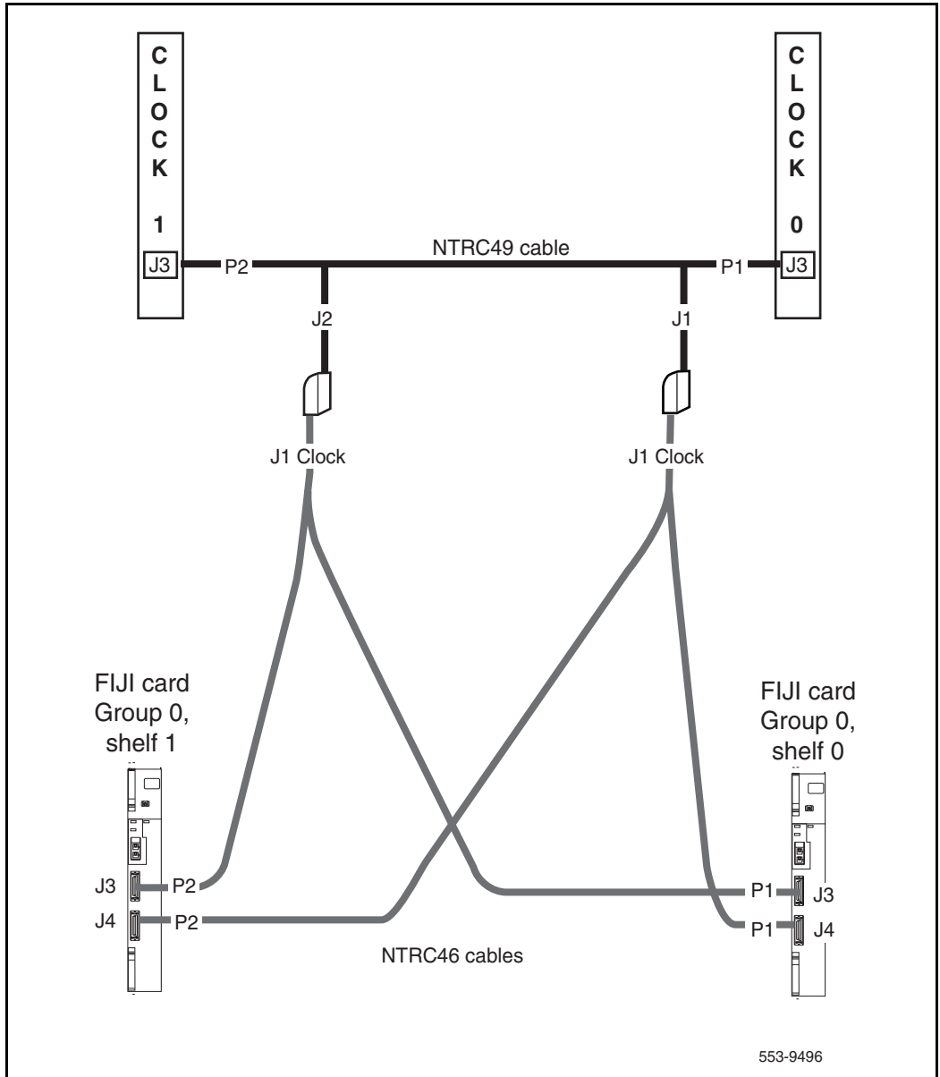
Figure 8 Clock Controller cable configuration
