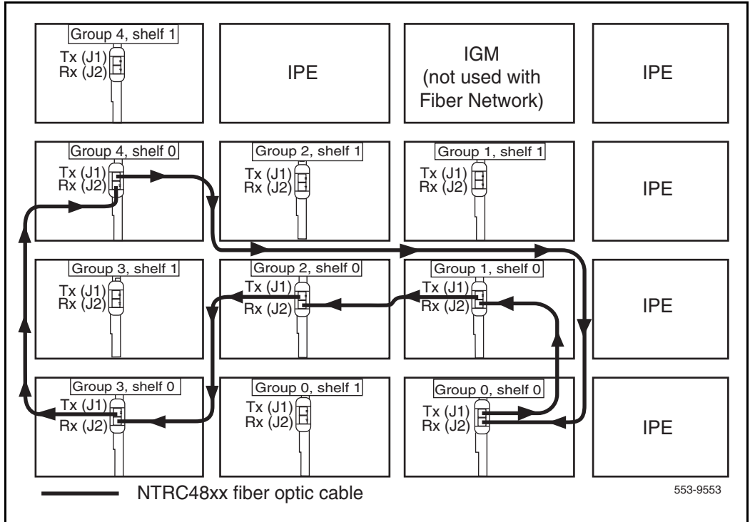
Figure 7 Shelf 0 ascending fiber optic Ring (Meridian 1 Option 81C 5 group example)
