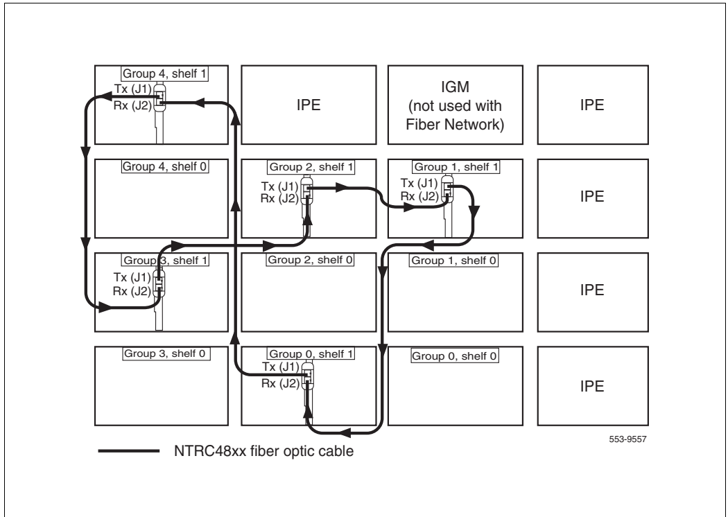
Figure 2 Shelf 1 descending fiber optic Ring (Meridian 1 Option 81C 5 group example)
