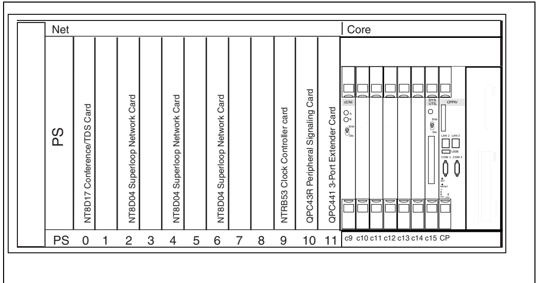
Figure 1 CP Core/Net Module
