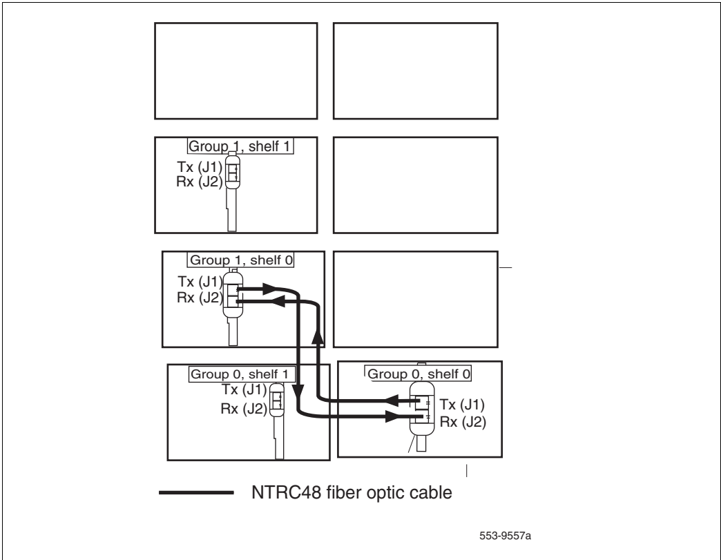
Figure 6 Shelf 0 ascending fiber optic Ring (Meridian 1 Option 81C 2 group example)
