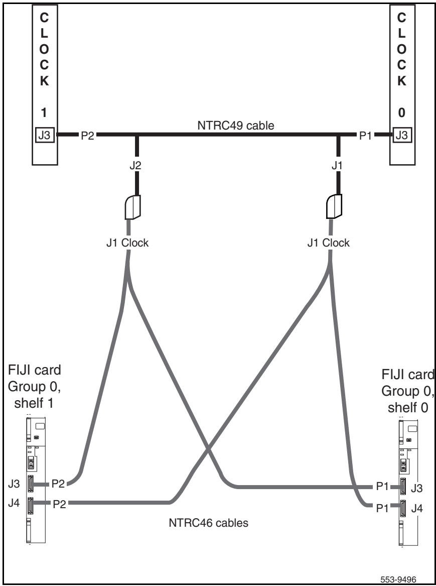
Figure 5 Clock Controller cable configuration
