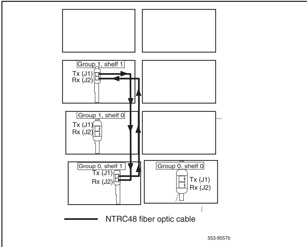
Figure 3 Shelf 1 descending fiber optic Ring (Meridian 1 Option 81C 2 group example)
