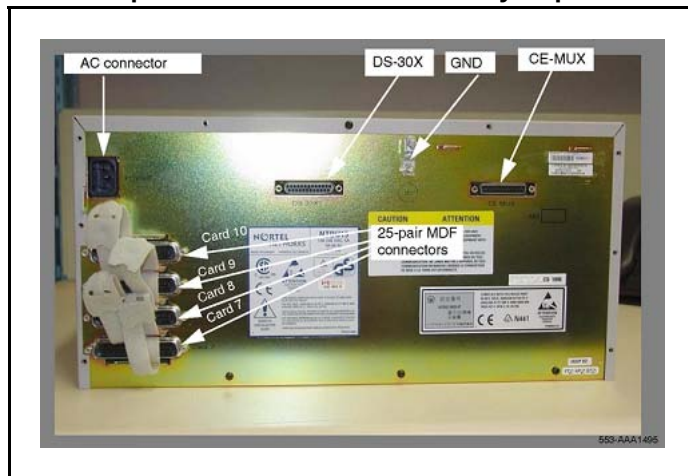
Figure 6 Rear components in the Media Gateway Expander
