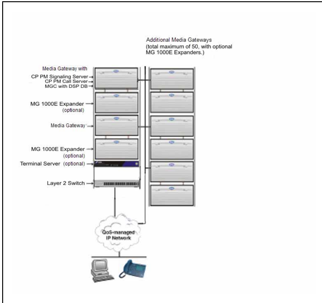
Figure 13 CS 1000E Standard Availability
