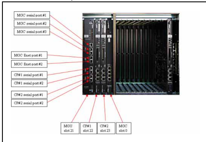
Figure 7 MG 1010 front components
