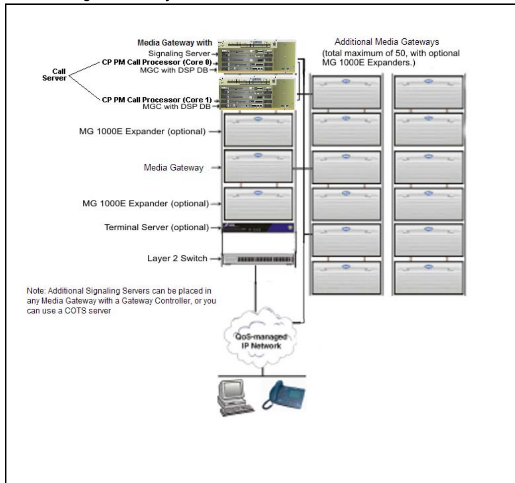
Figure 14 CS 1000E High Availability
