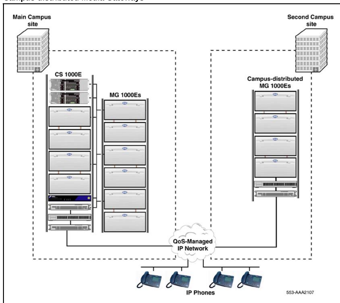
Figure 15 Campus-distributed Media Gateways
