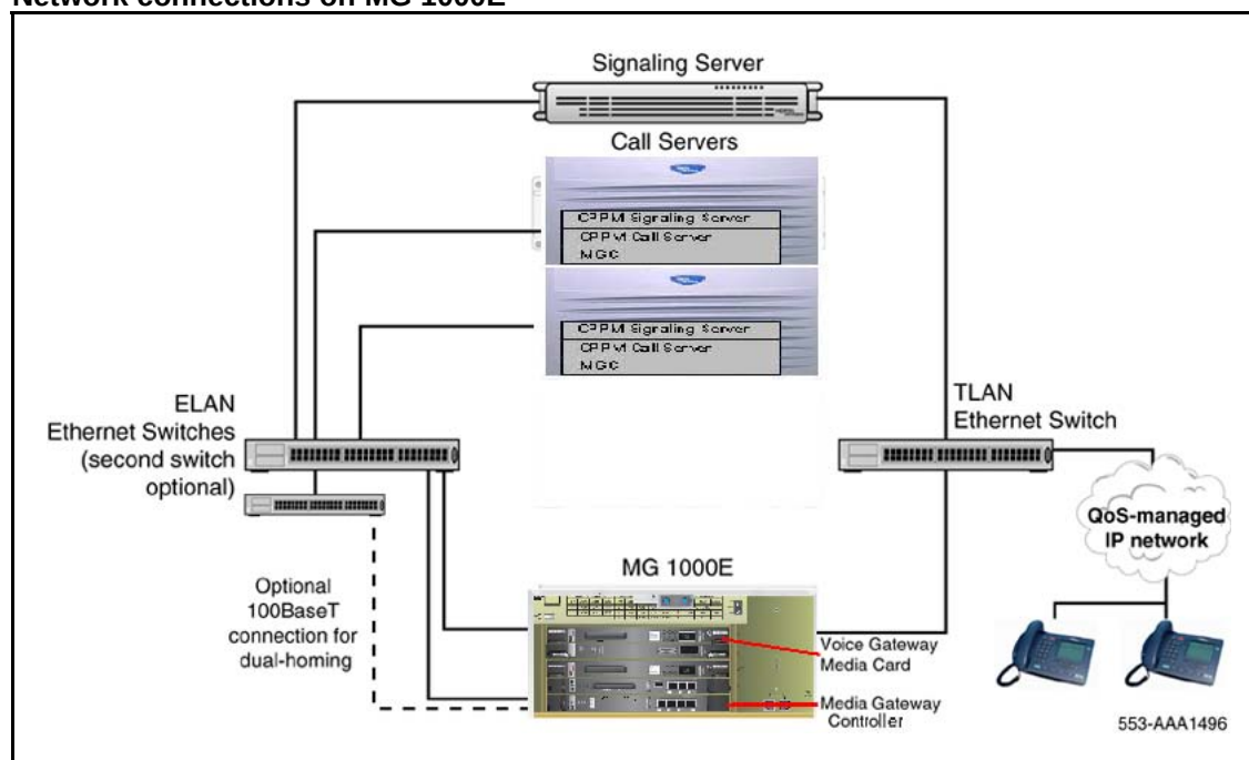
Figure 11 Network connections on MG 1000E
