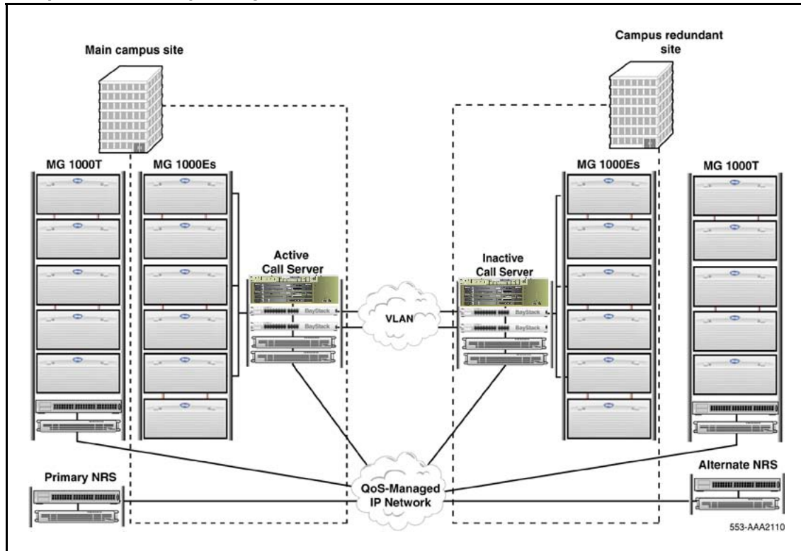
Figure 16 Campus Redundancy configuration
