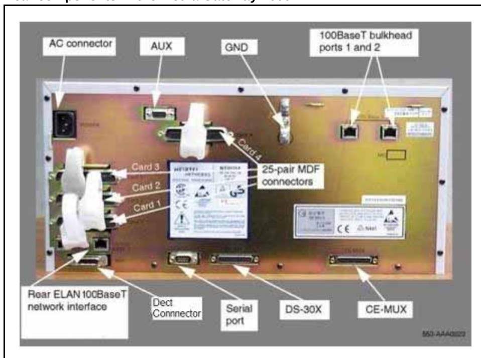
Figure 4 Rear components in the Media Gateway 1000E
