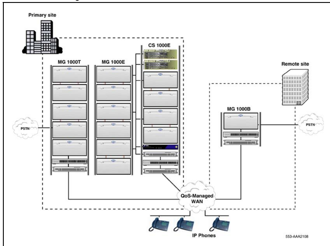
Figure 17 Branch Office configuration
