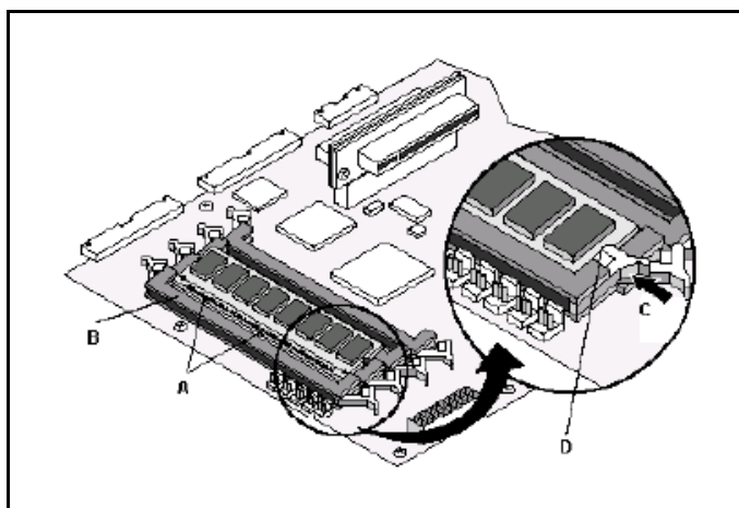
Figure 40 Install DIMM board
