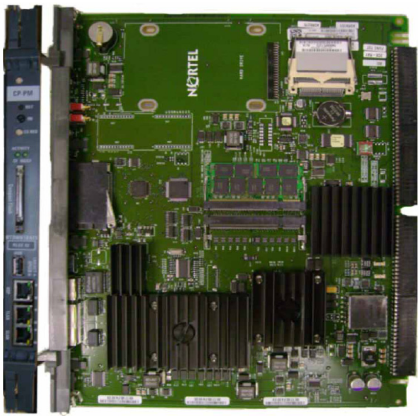
Figure 2 NTDW61 CP PM card
