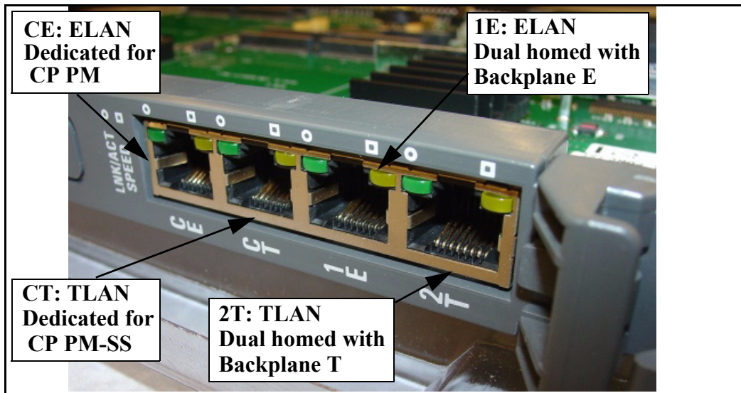
Figure 9 MGC faceplate
