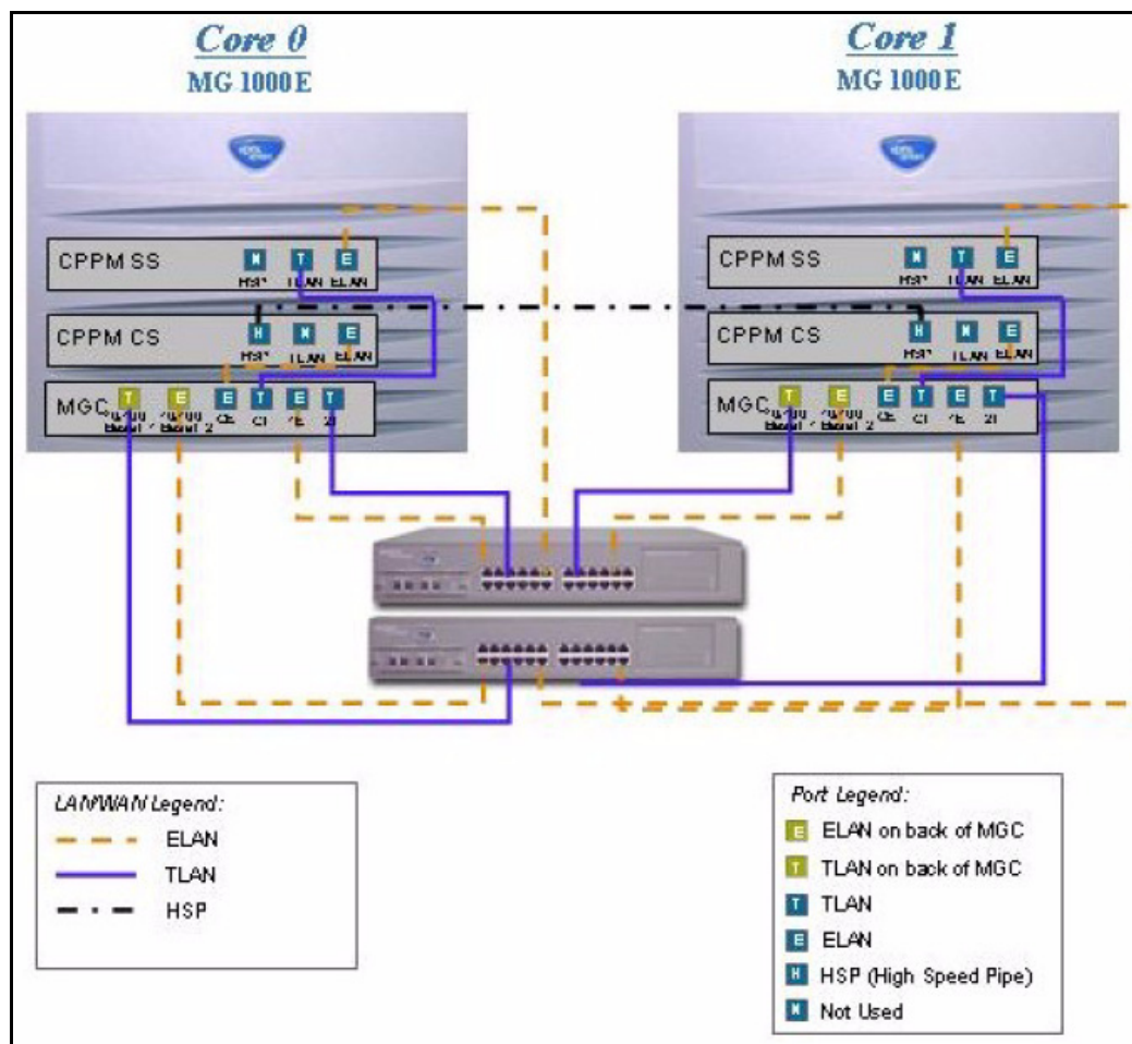
Figure 71 Campus Redundancy with CP PM call servers co-located
