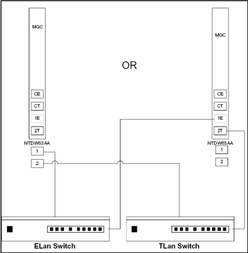
Figure 11 Elan connections (MGC)
