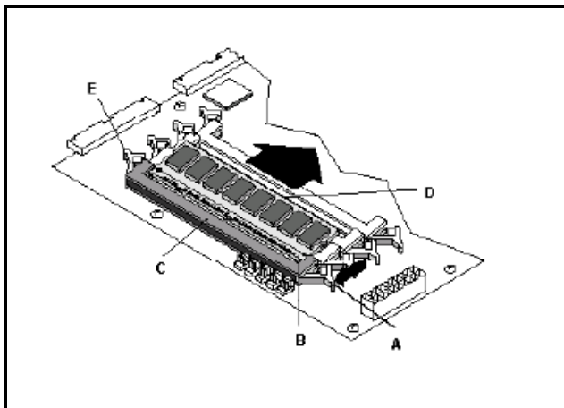
Figure 39 Remove DIMM board
