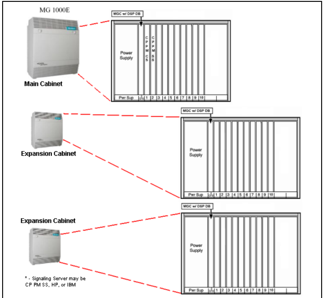
Figure 6 Typical three cabinet SA system
