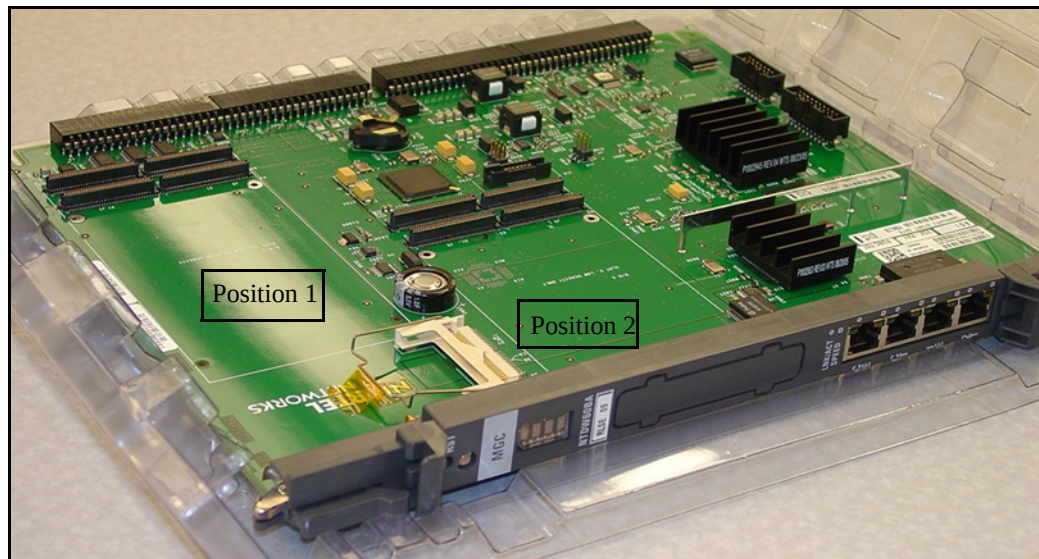
Figure 7 DSP Daughterboard
