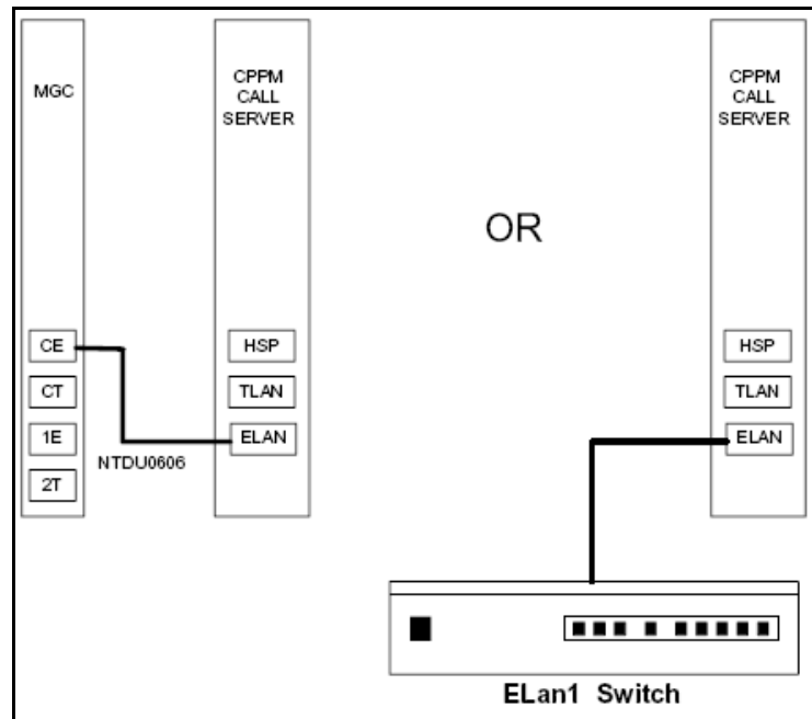
Figure 10 Elan connection (CP PM Call Server)
