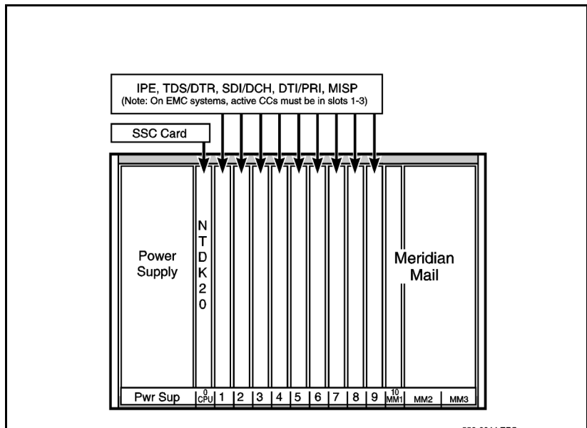
Figure 5 NTAK11 Cabinet with SSC card
