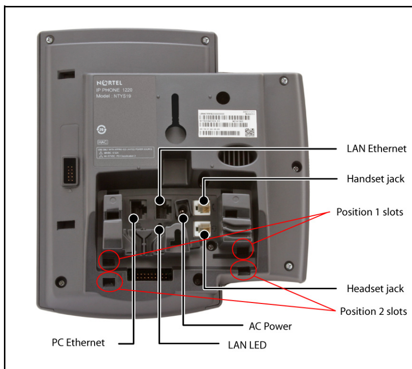
Figure 4: Connections on the IP Phone 1220
