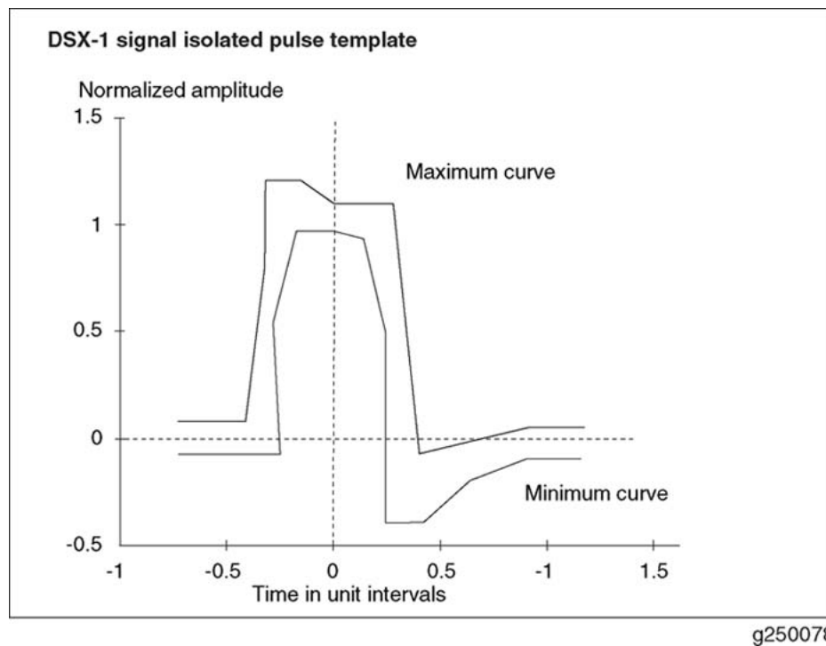
DSX-1 isolated pulse template corner points
