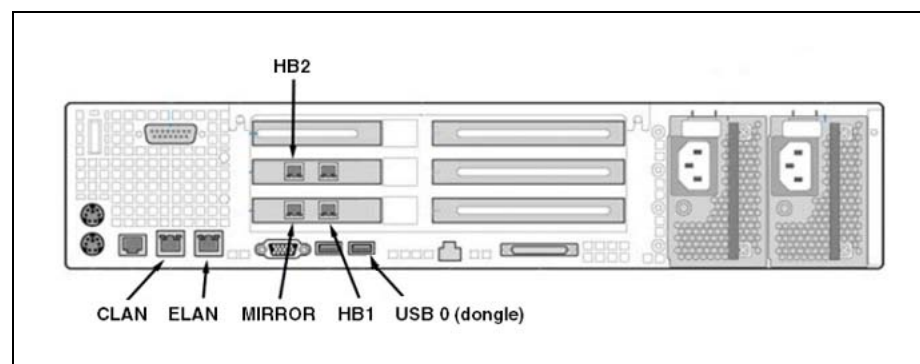
Figure 25 Rear panel of 1005r server showing LAN connections
