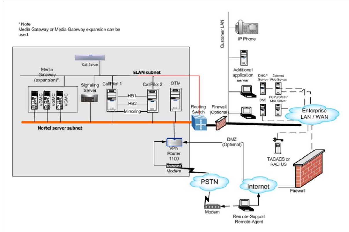
Figure 2 High Availability network
