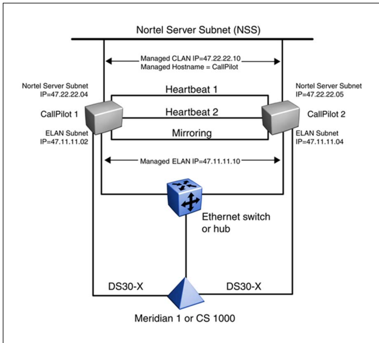
Figure 1 Example of a High Availability system
