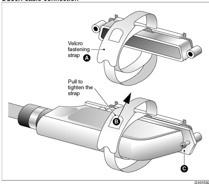
DS30X cable connection
