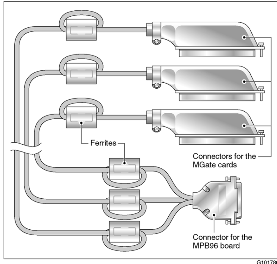
Connectors between MGate and MPB96
