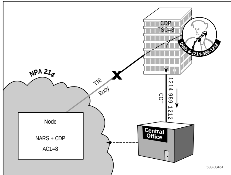
Figure 23- Using Trunk Steering Codes at a remote site
