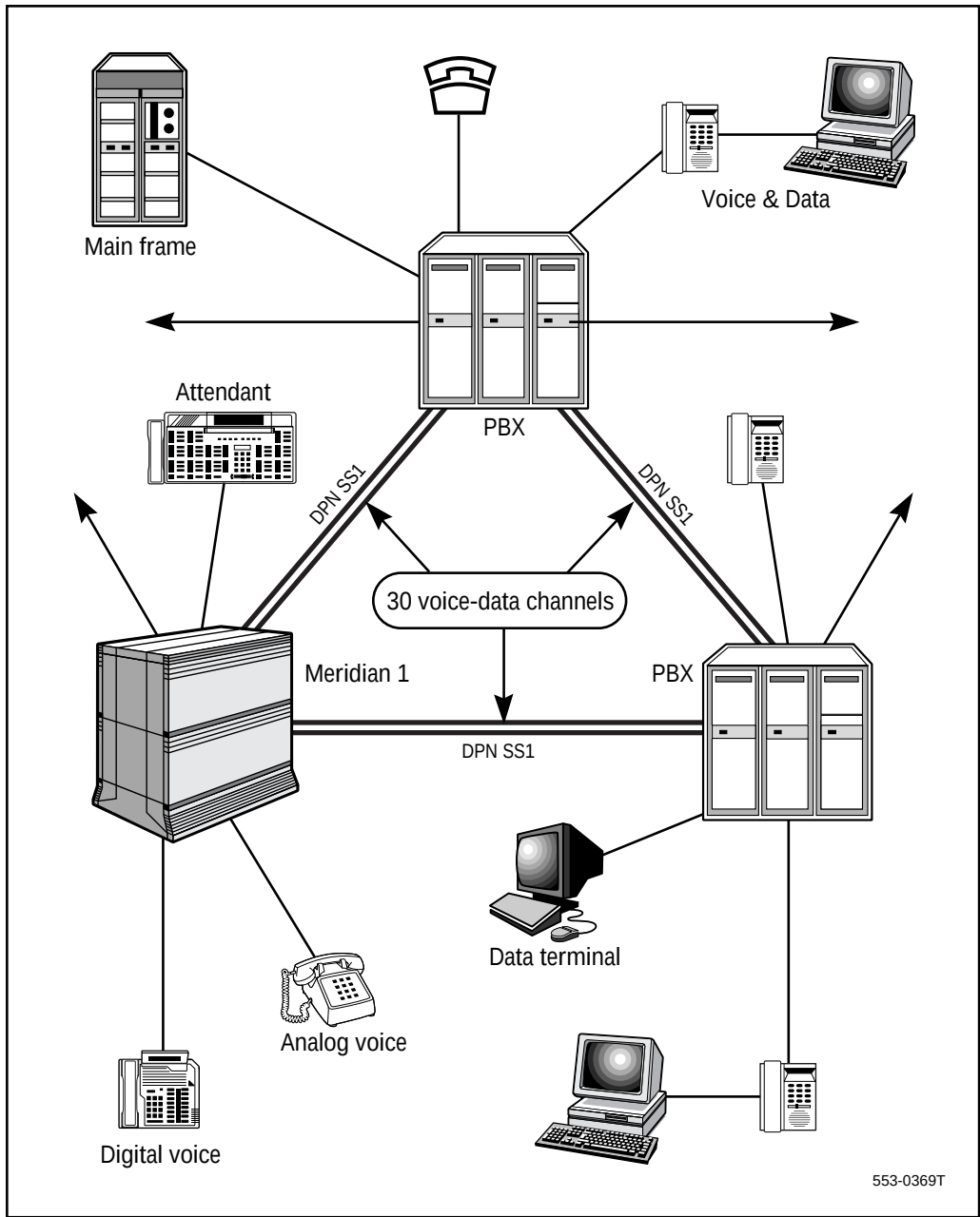
Figure 31- DPNSS1 configured in a network
