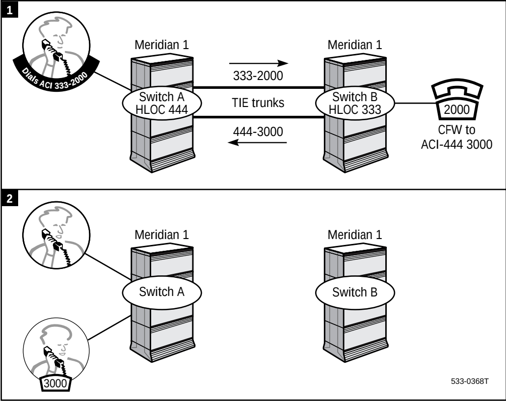
Figure 43 - Trunk Anti-Tromboning
