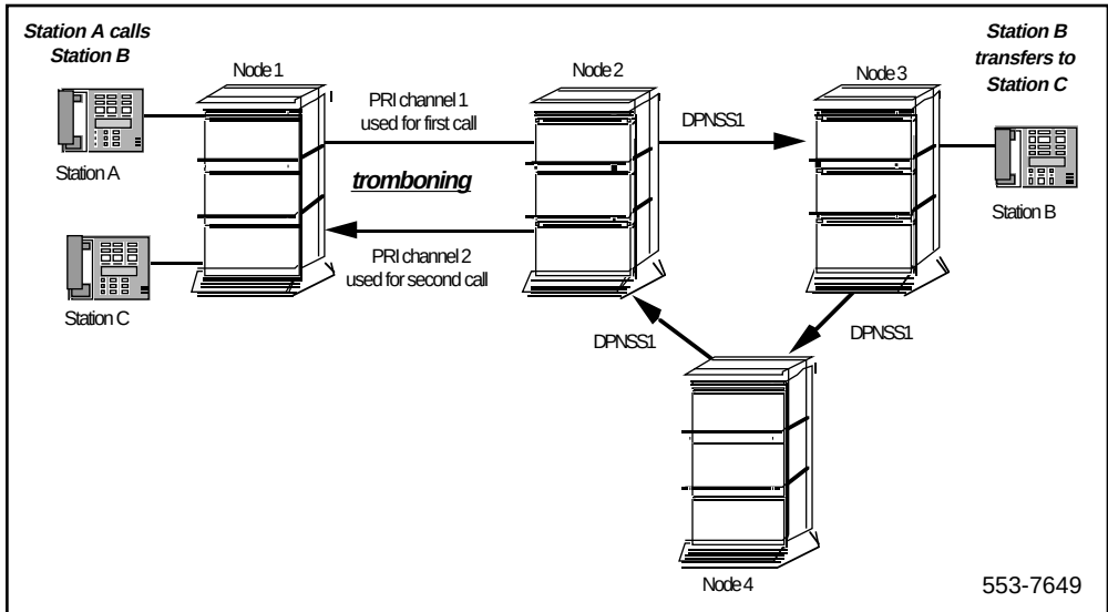
Figure 58 MCDN/DPNSS1 RO/TAT Interworking scenario, before RO has been applied
