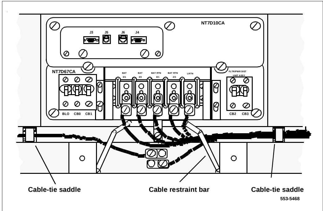
Figure 18 Cable routing in the rear of the pedestal — NT7D67CA PDU
